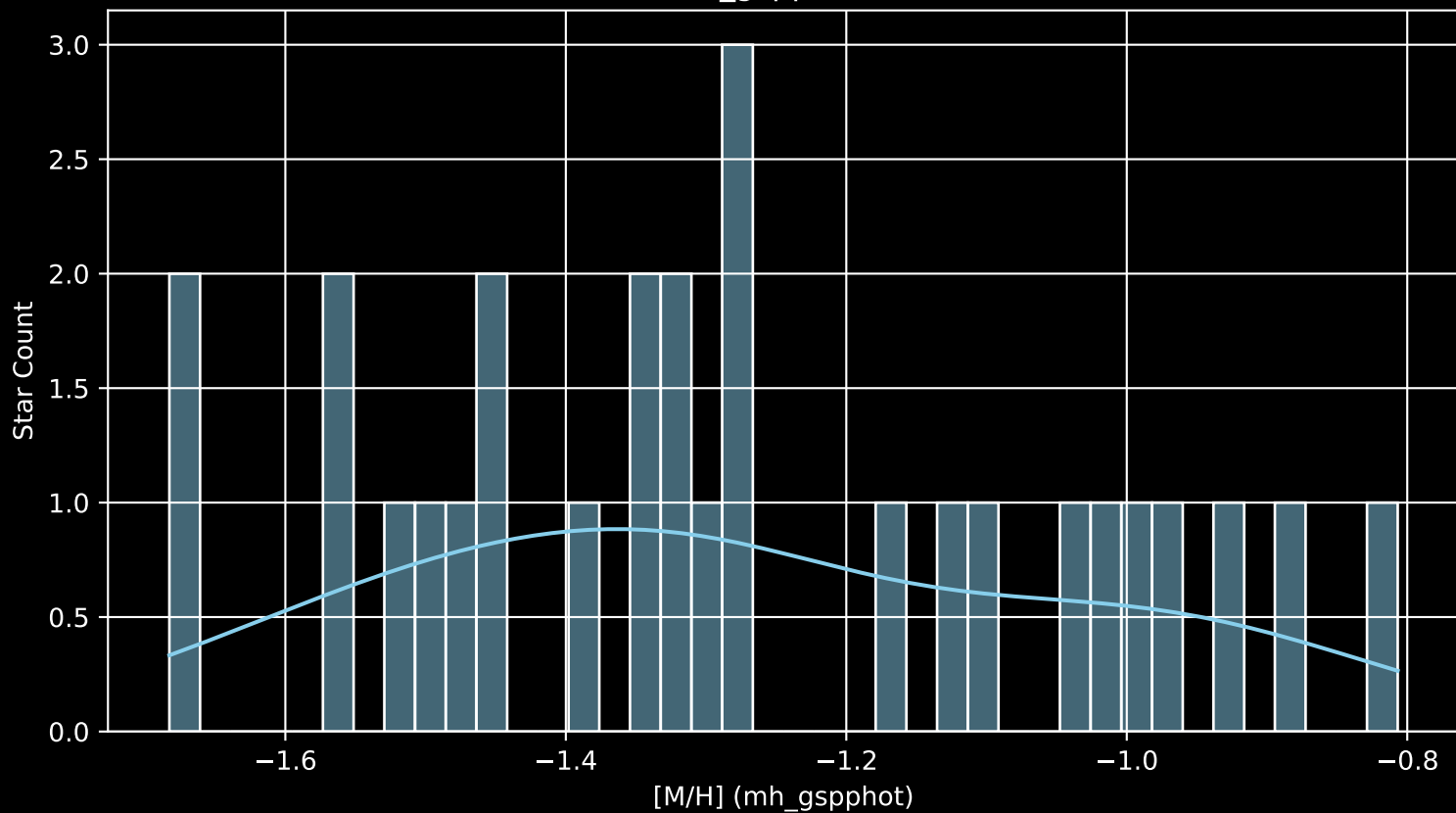
Gaia Stream: [New-10 [M/H] (mh_gspphot) (n= 28)
