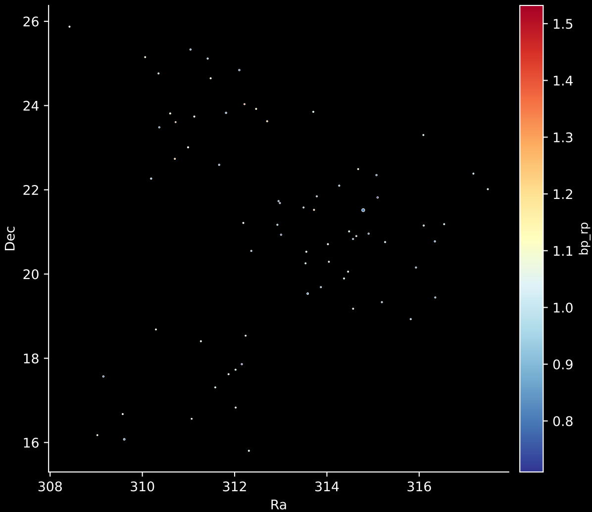
Gaia Stream: [New-18] Stars: 90
