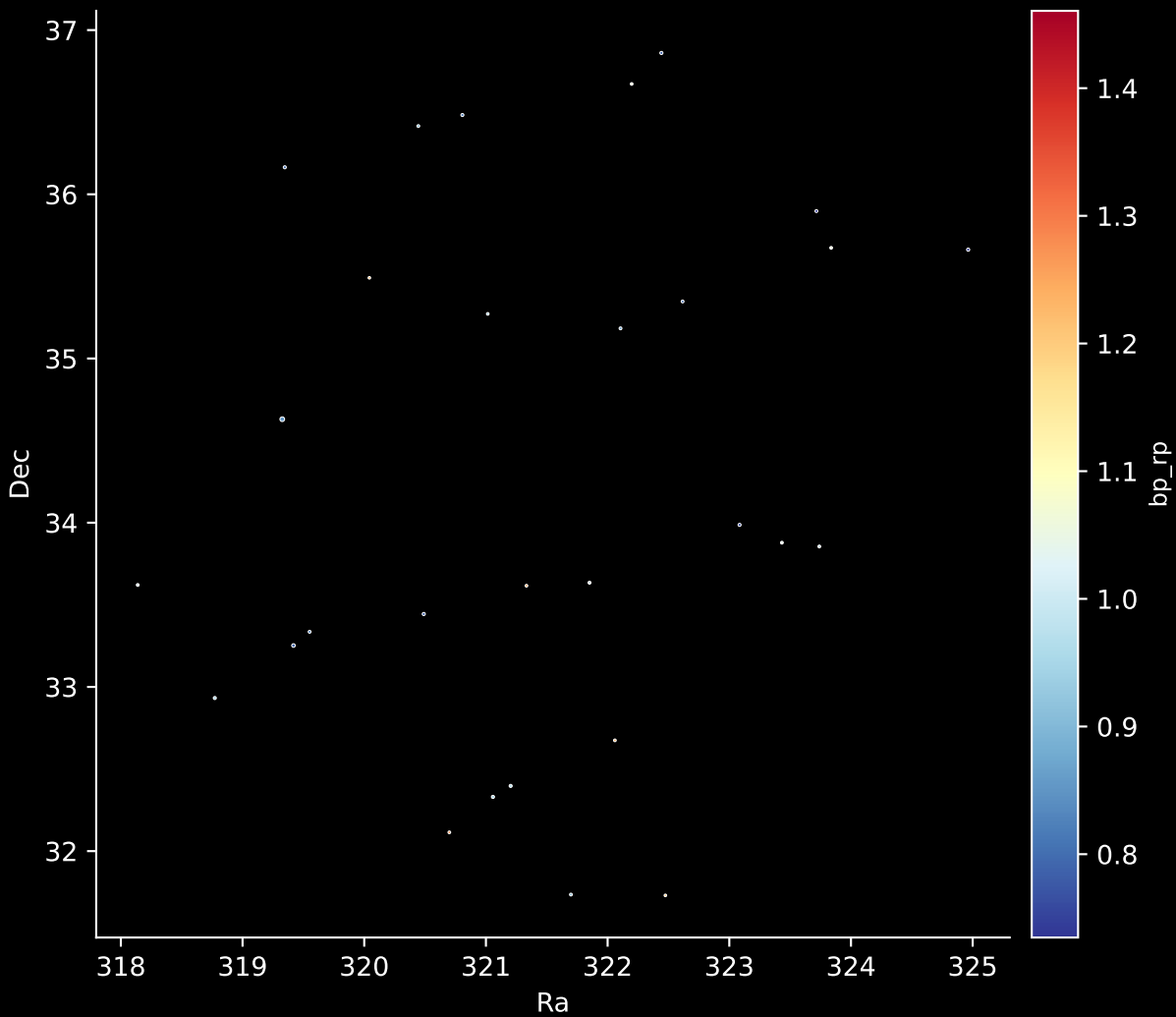
Gaia Stream: [New-19] Stars: 39
