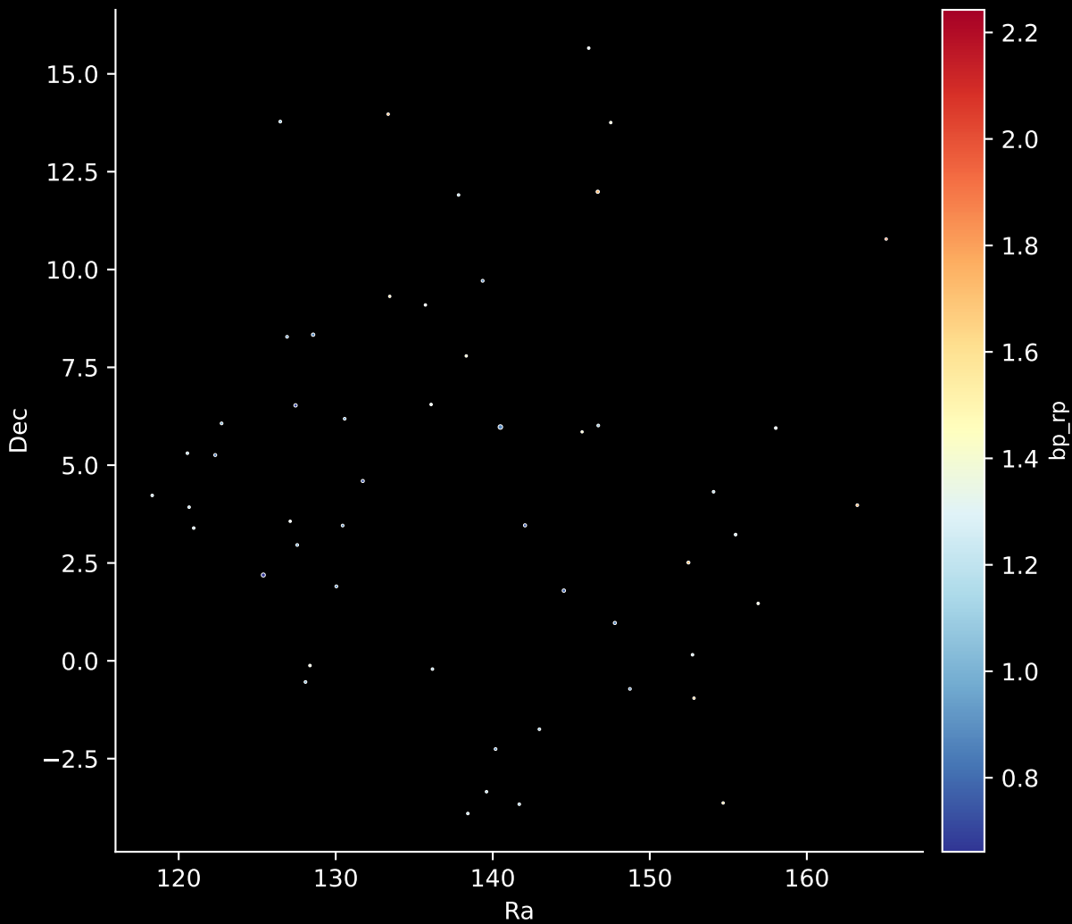
Gaia Stream: [New-2] Stars: 85
