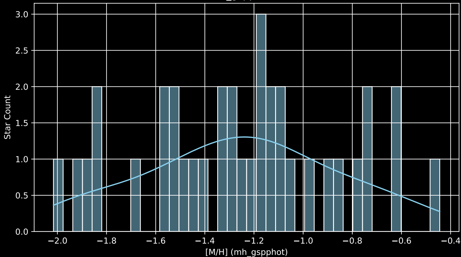
Gaia Stream: [New-24 [M/H] (mh_gspphot) (n= 36)
