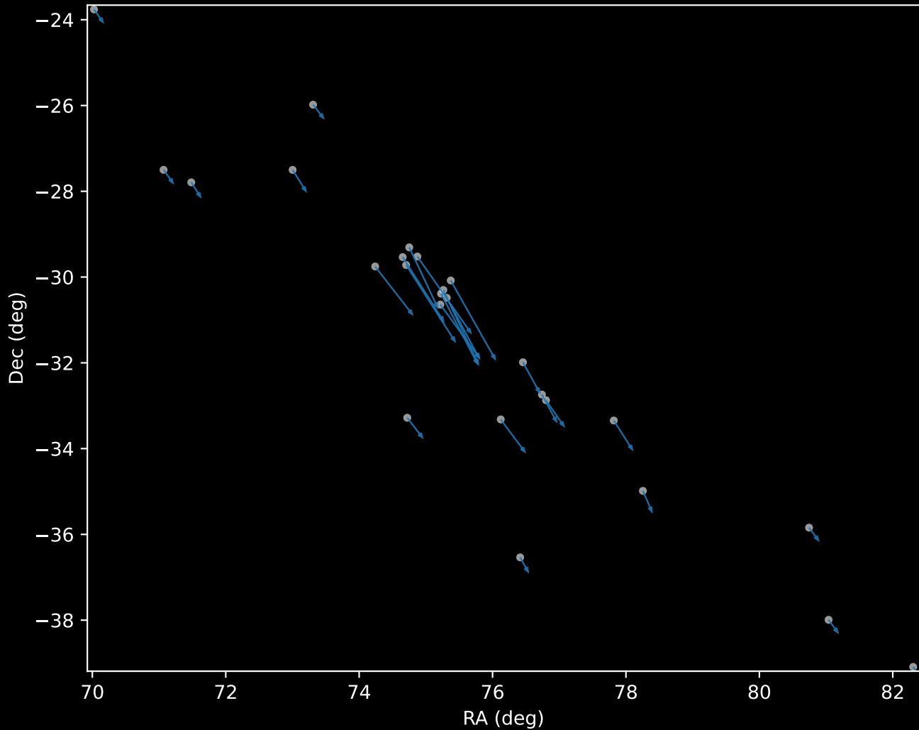
Gaia DR3 Cluster 0 Proper Motion Vectors (n=26)
