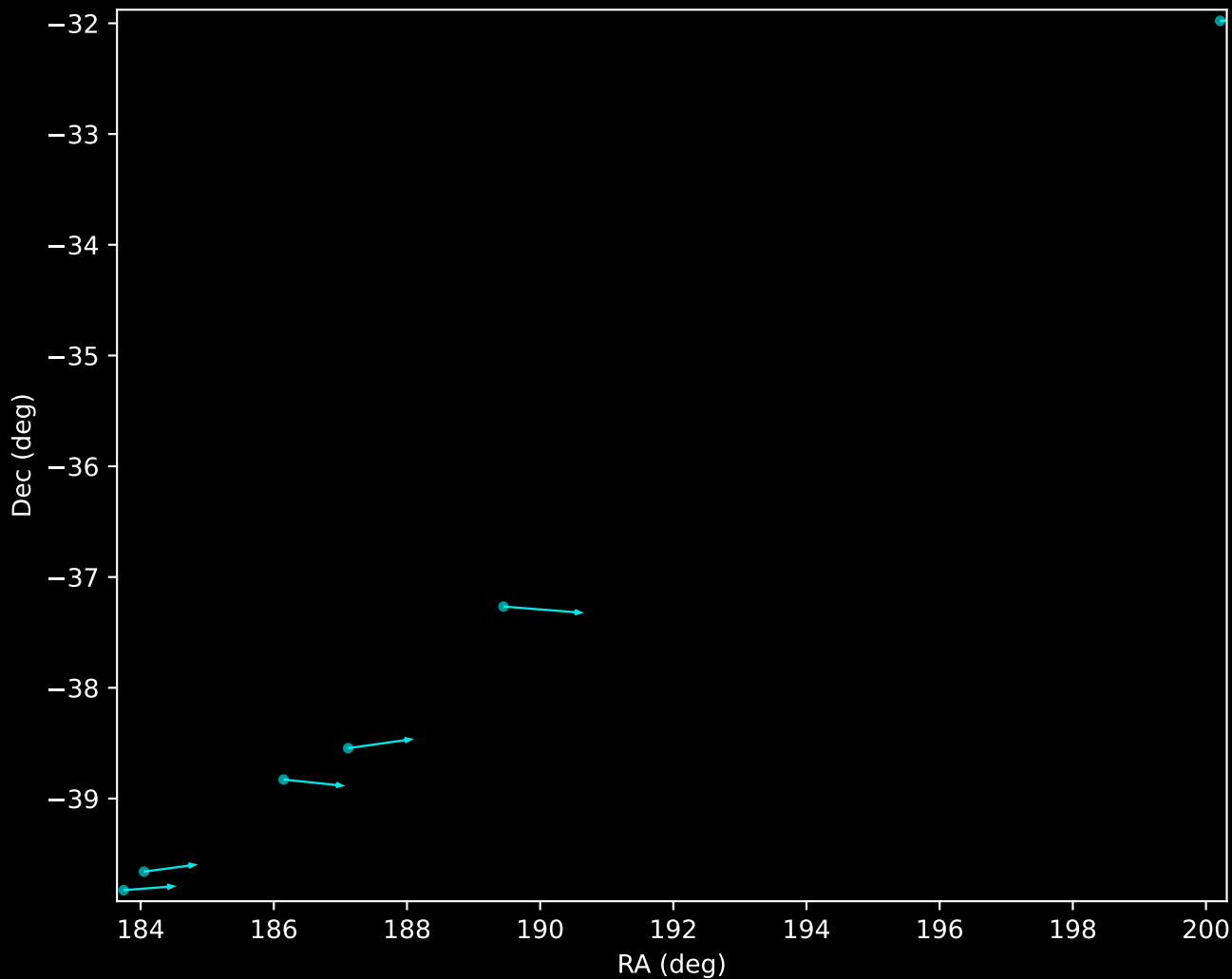
Gaia DR3 Noise Stream Proper Motion Vectors (n=6)
