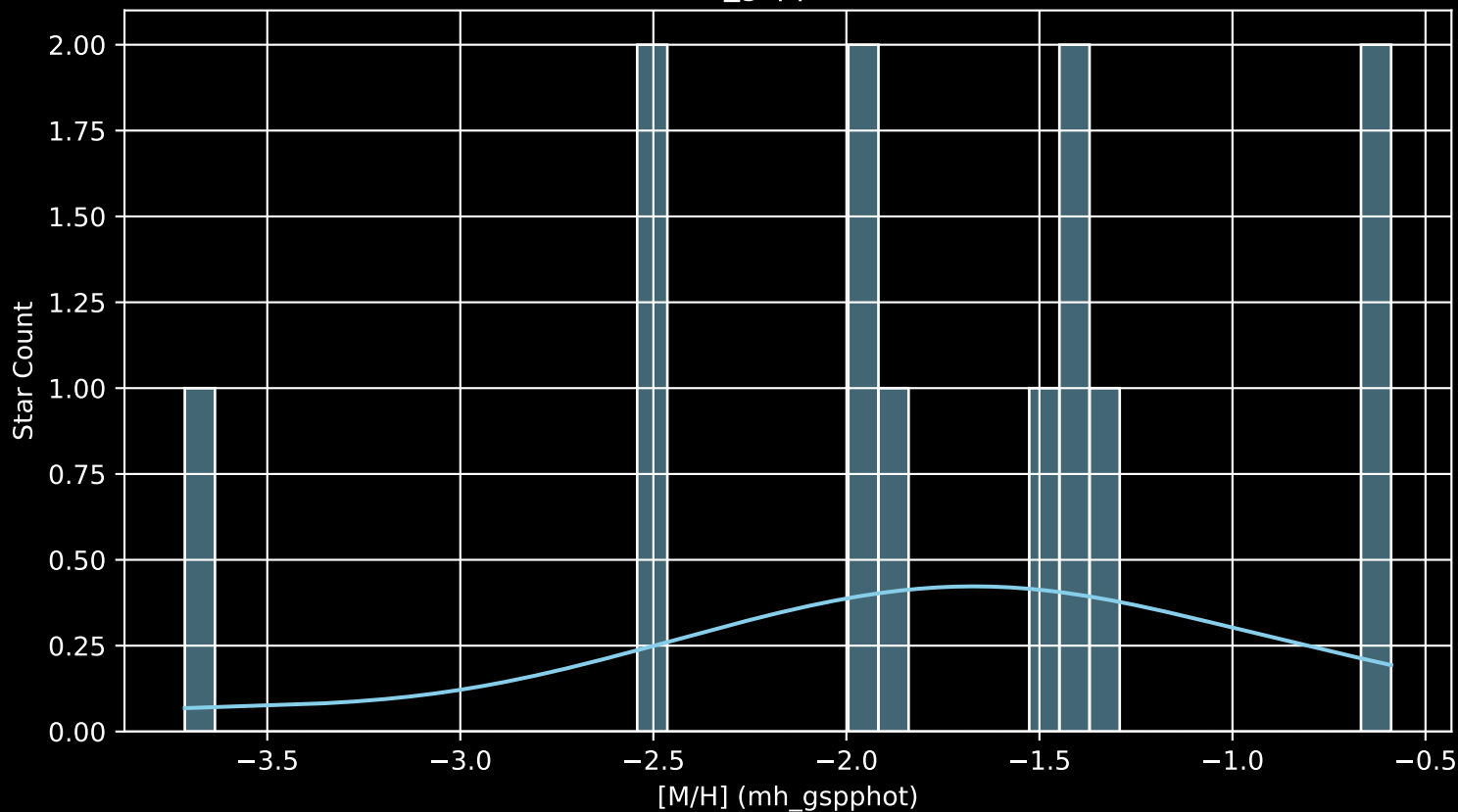
Gaia Stream: [New-4 [M/H] (mh_gspphot) (n= 12)
