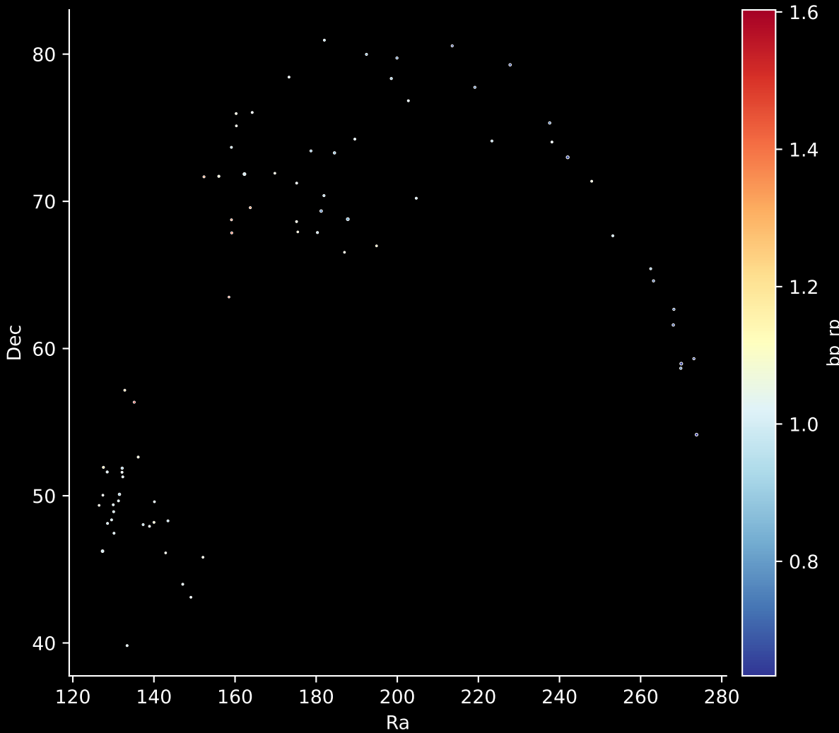
Gaia Stream: [New-6] Stars: 127
