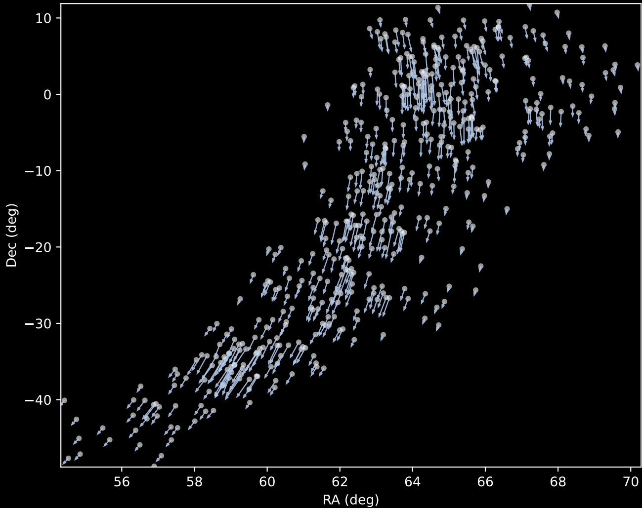
Gaia DR3 Cluster 1 Proper Motion Vectors (n=475)
