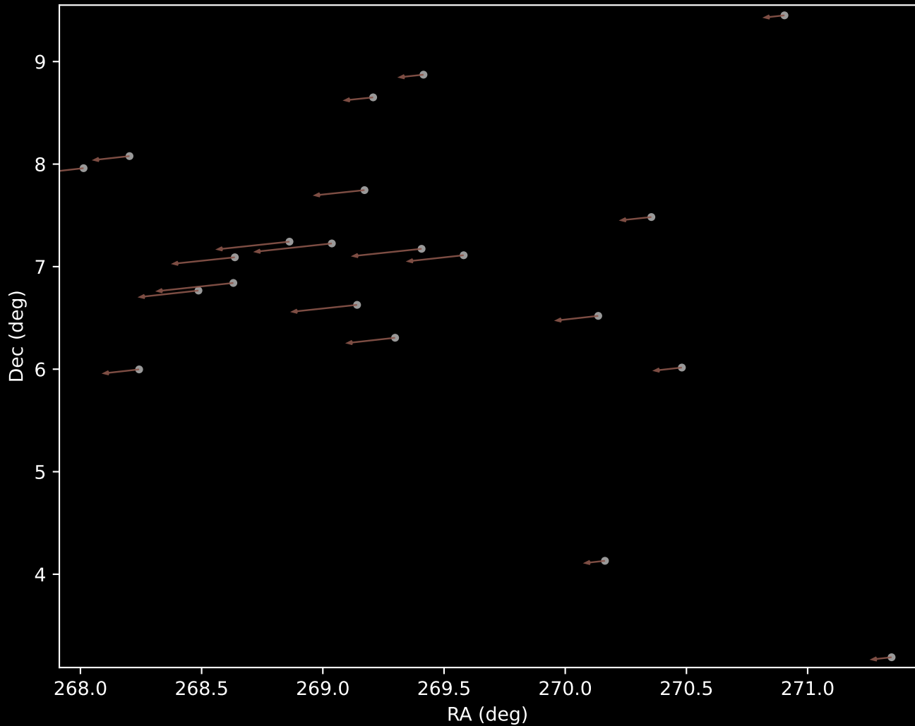
Gaia DR3 Cluster 10 Proper Motion Vectors (n=21)
