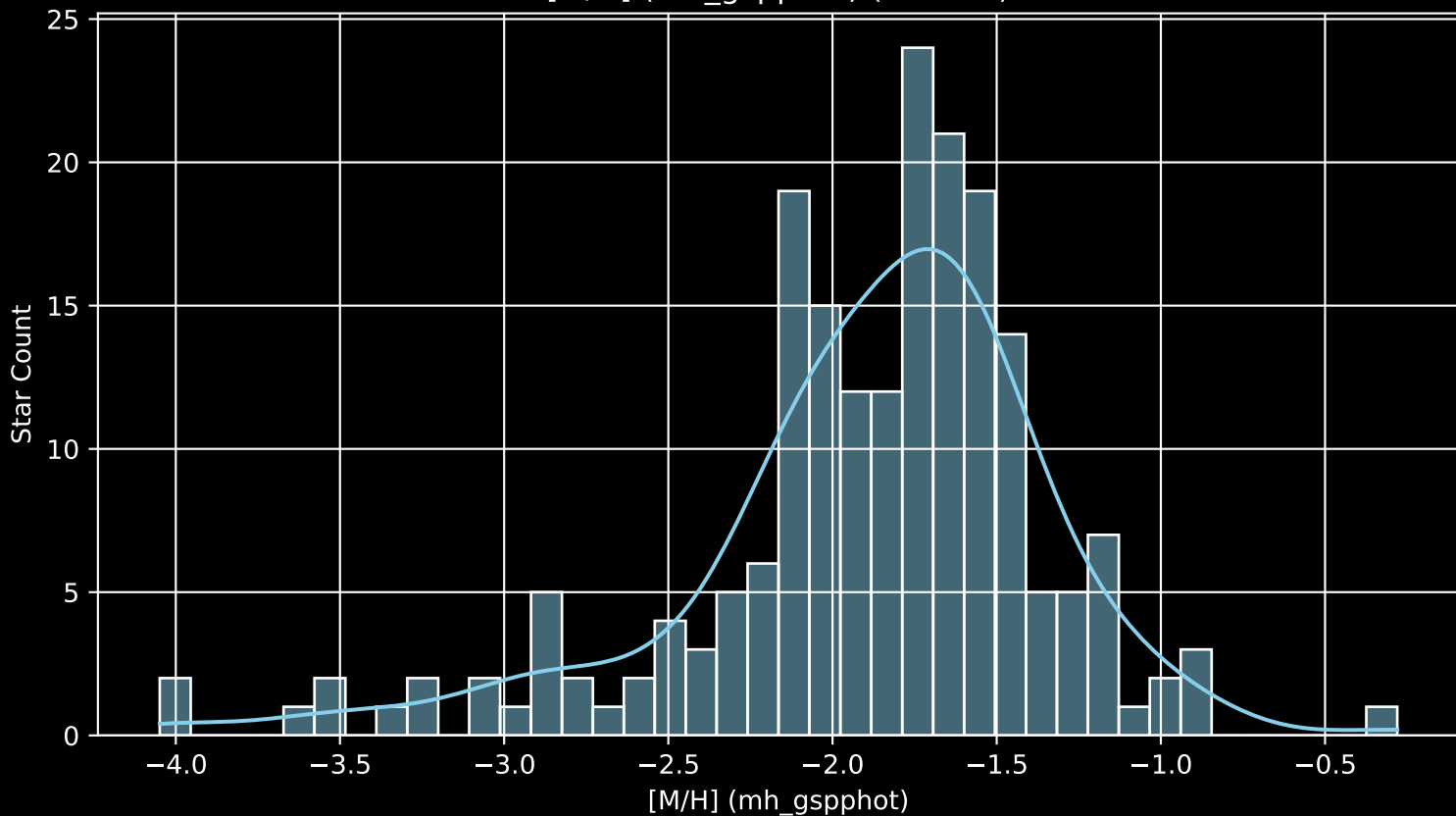
Gaia Stream: [Slidr [M/H] (mh_gspphot) (n= 199)
