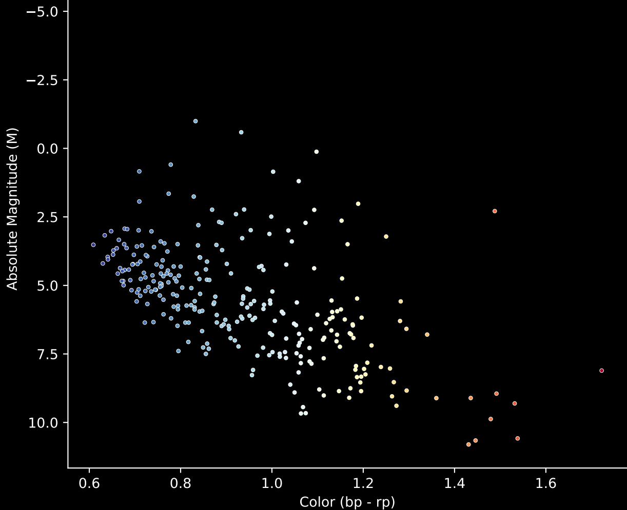
Gaia Stream: [Slidr] Stream (n= 278) Hertzsprung-Russel Diagram
