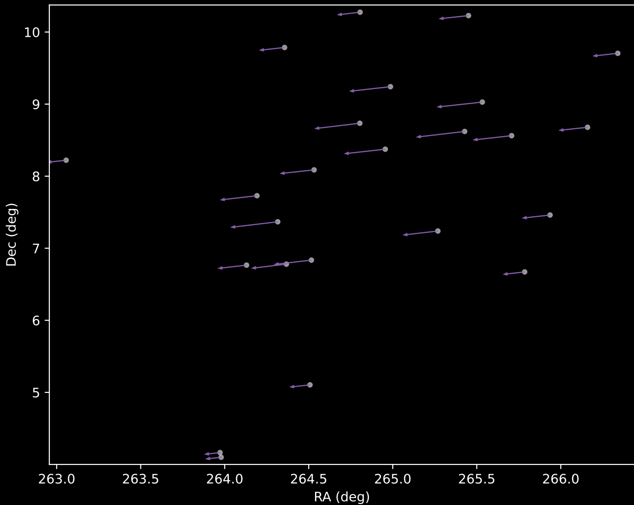
Gaia DR3 Cluster 8 Proper Motion Vectors (n=24)
