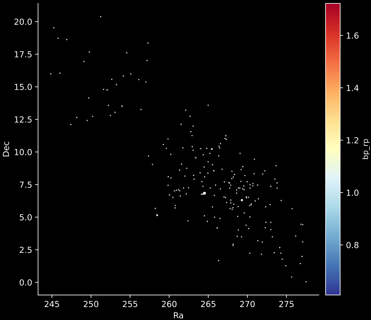
Gaia Stream: [Slidr] Stars: 278
