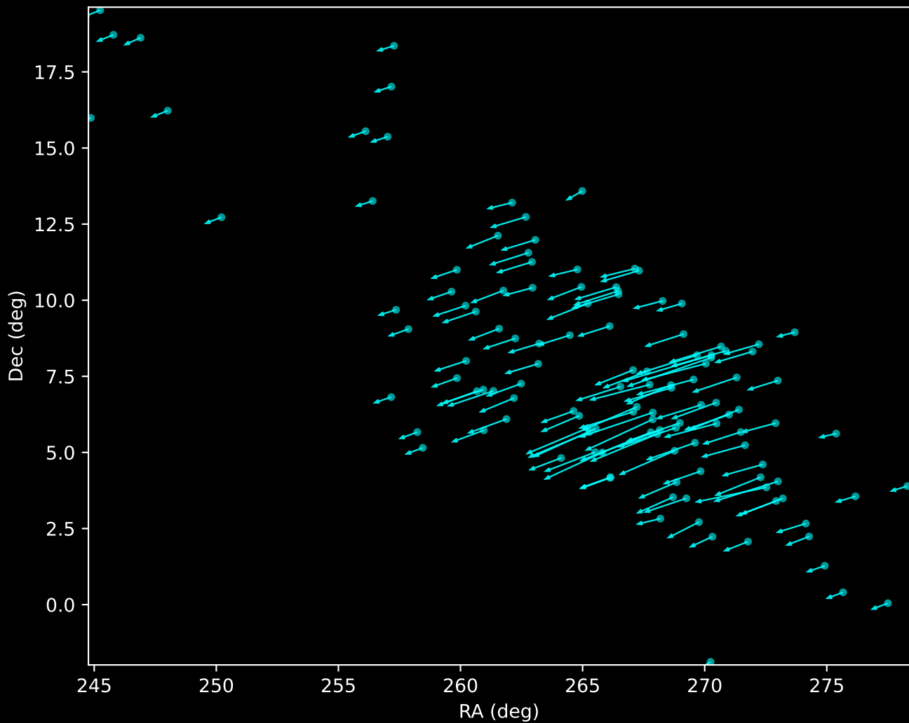
Gaia DR3 Noise Stream Proper Motion Vectors (n=125)
