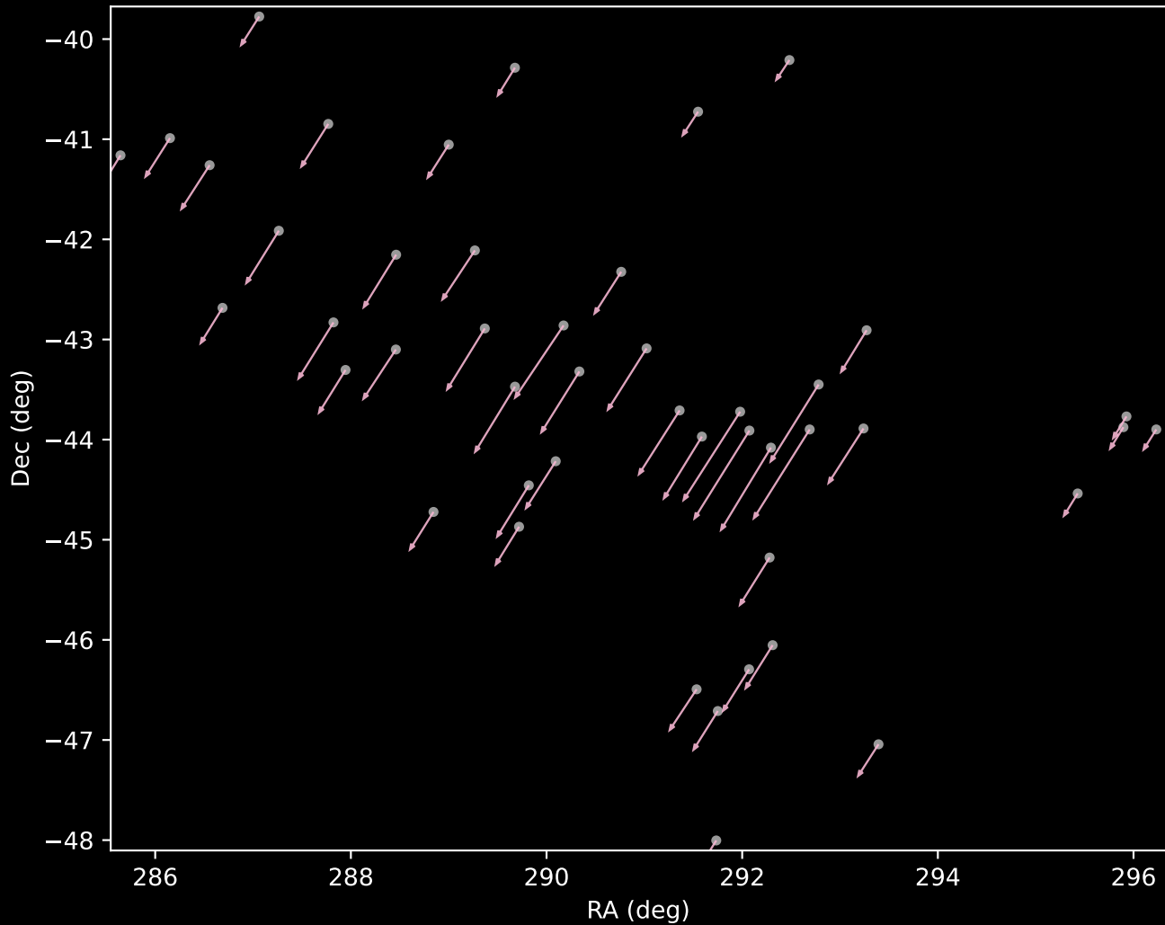
Gaia DR3 Cluster 153 Proper Motion Vectors (n=46)
