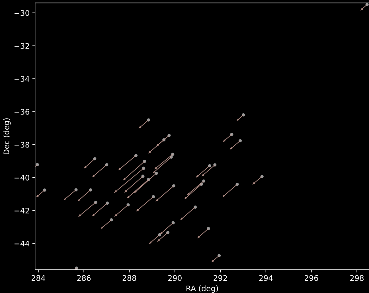
Gaia DR3 Cluster 111 Proper Motion Vectors (n=40)
