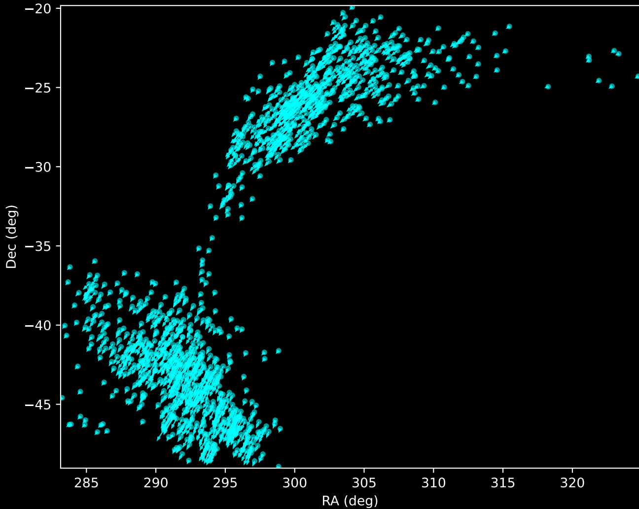
Gaia DR3 Noise Stream Proper Motion Vectors (n=1144)
