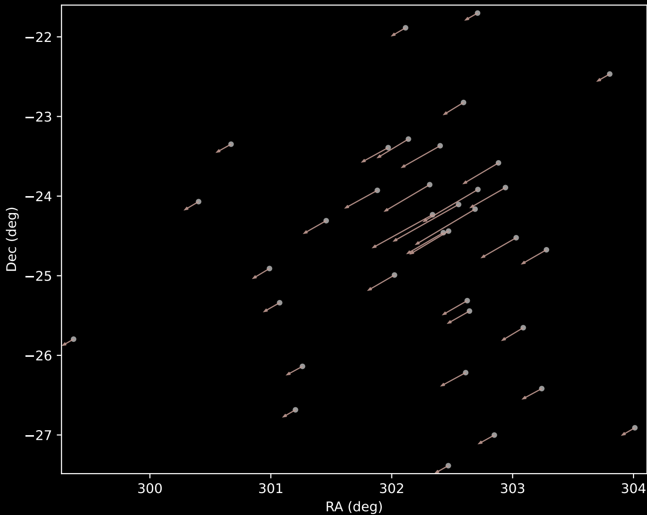
Gaia DR3 Cluster 51 Proper Motion Vectors (n=36)
