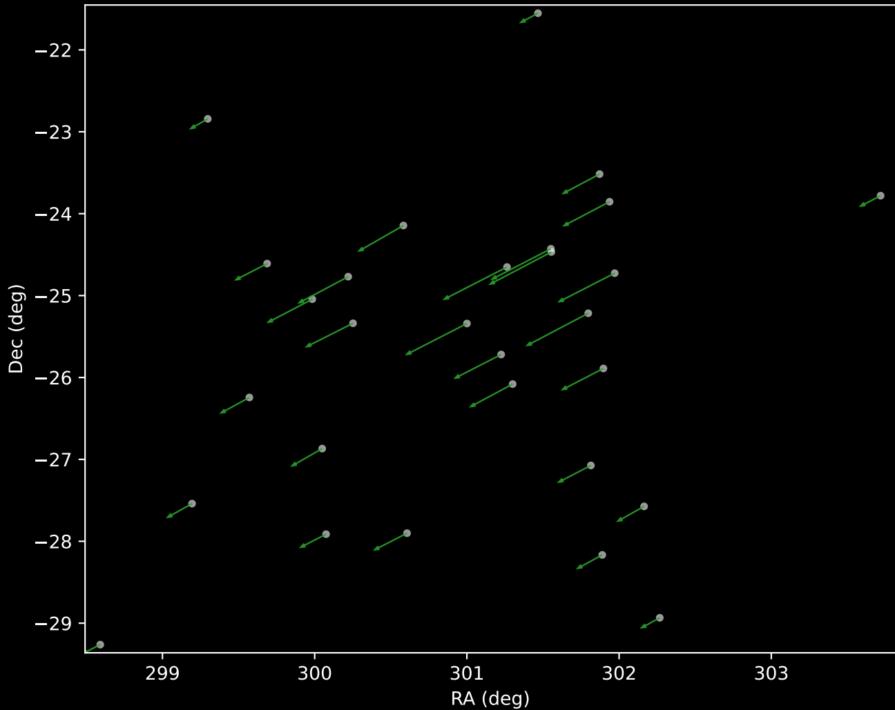
Gaia DR3 Cluster 24 Proper Motion Vectors (n=29)
