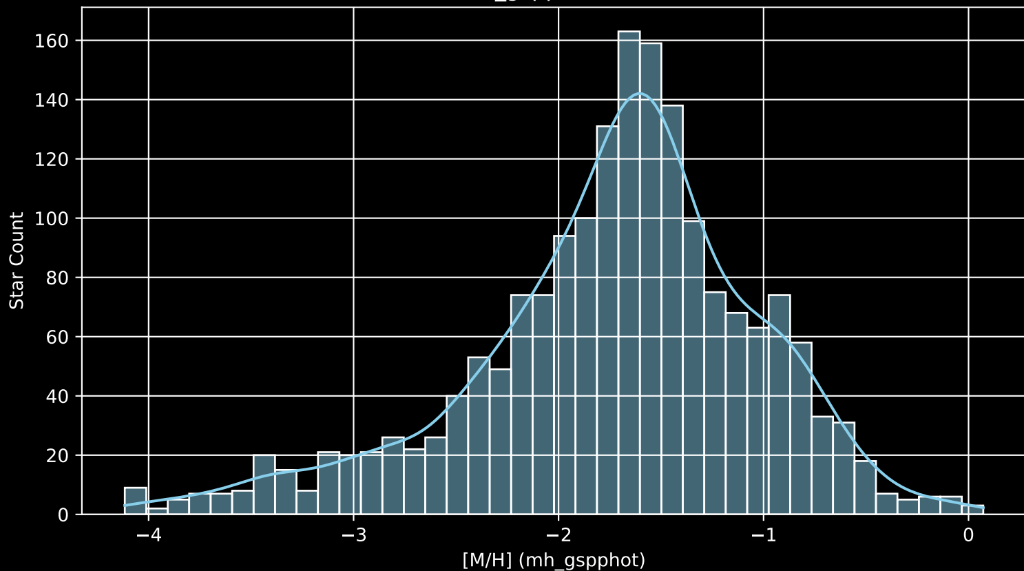
Gaia Stream: [Svol [M/H] (mh_gspphot) (n= 1838)
