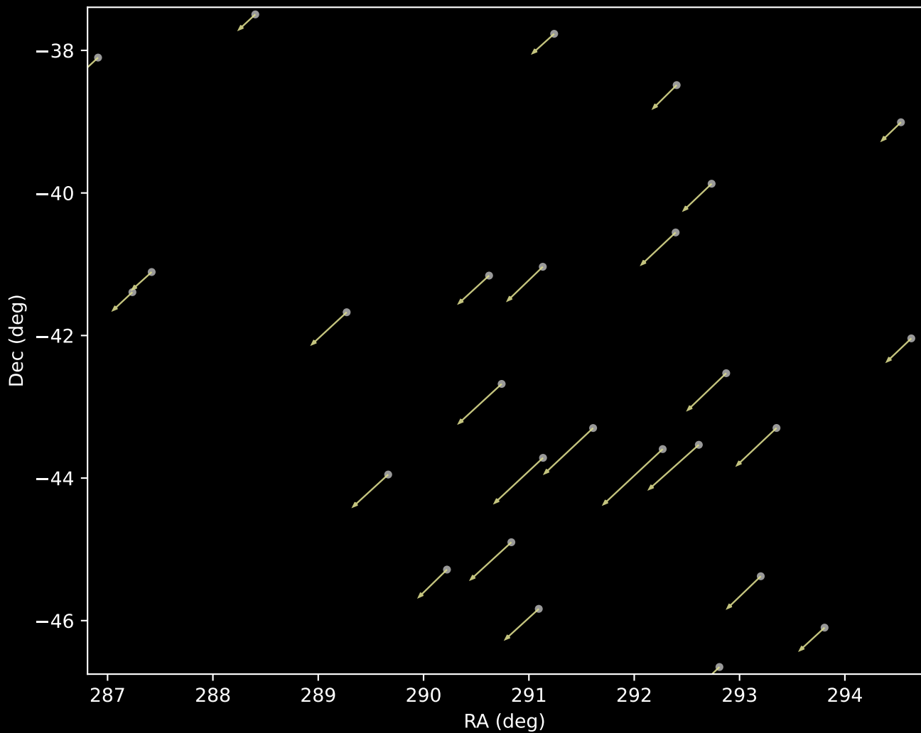
Gaia DR3 Cluster 137 Proper Motion Vectors (n=27)
