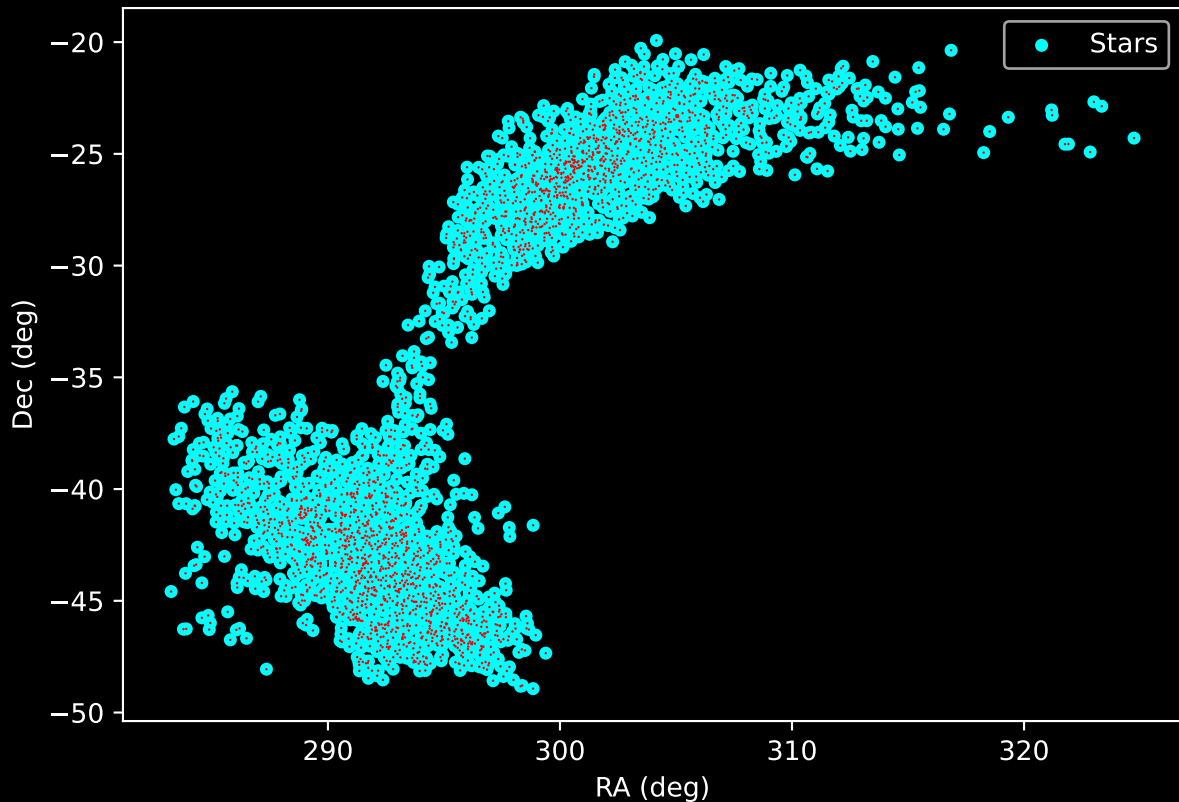
Gaia Stream: [Svol] Proper Motion Vectors for Gaia Star Field (n= 2874)
