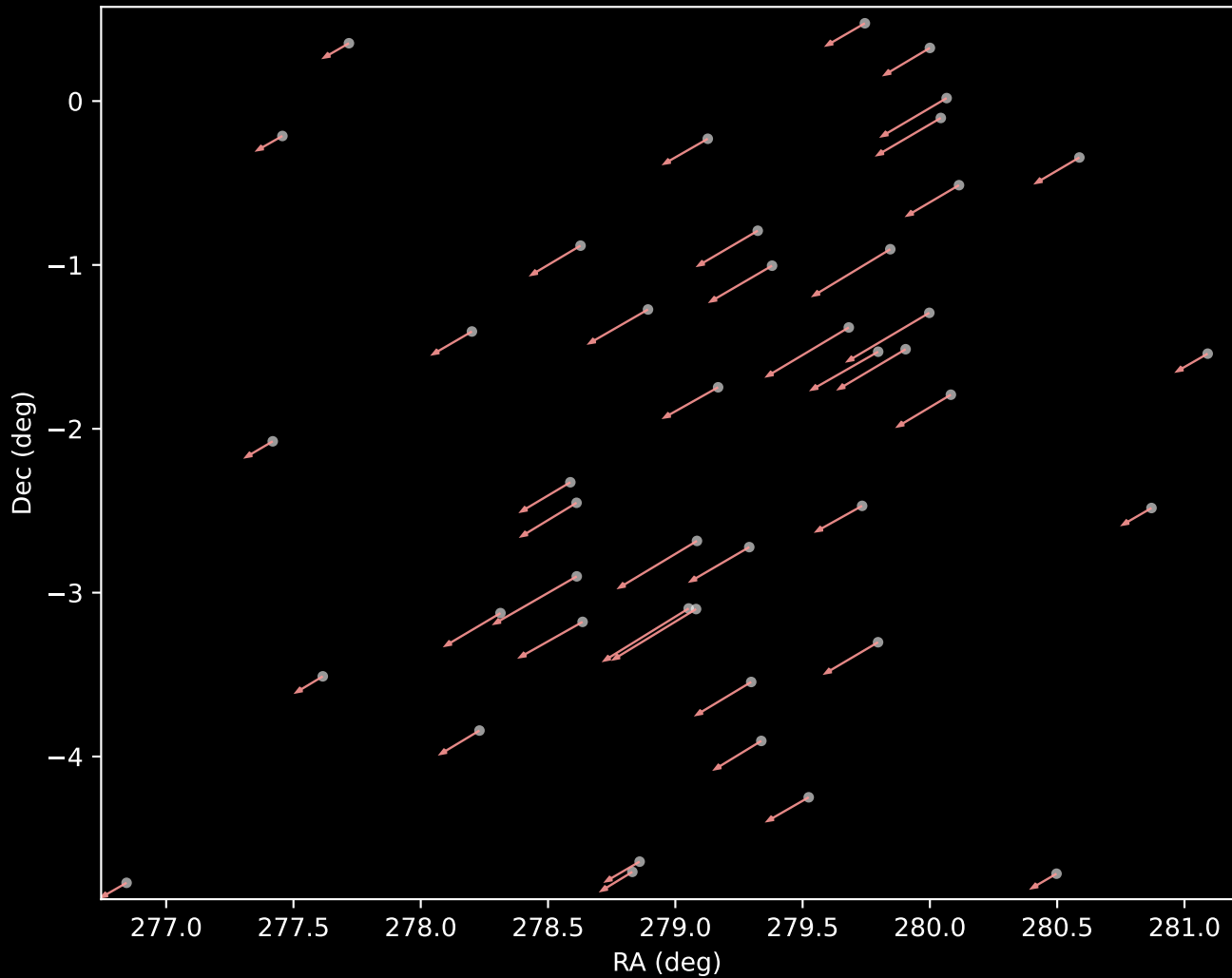
Gaia DR3 Cluster 7 Proper Motion Vectors (n=44)
