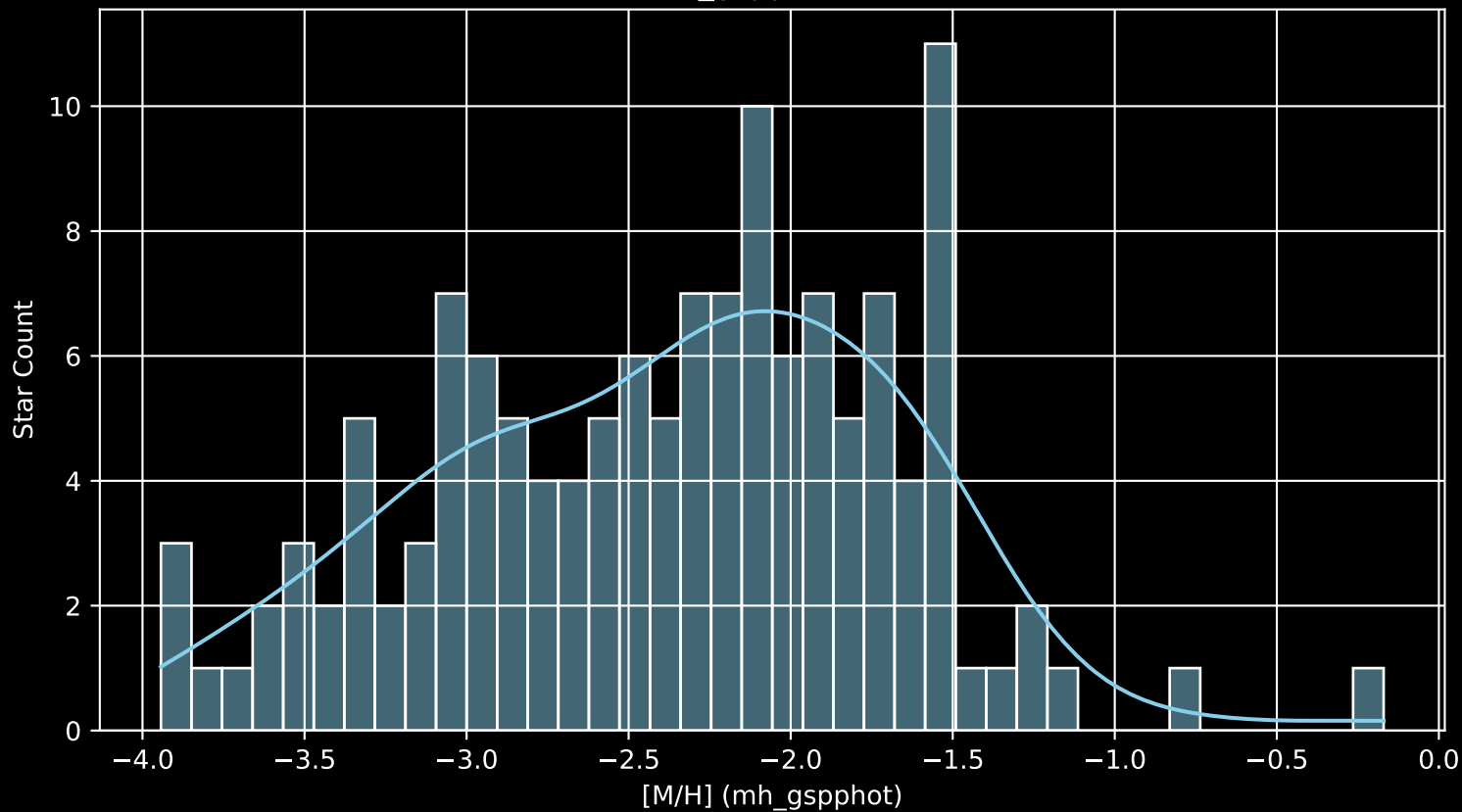
Gaia Stream: [Sylgr [M/H] (mh_gspphot) (n= 135)
