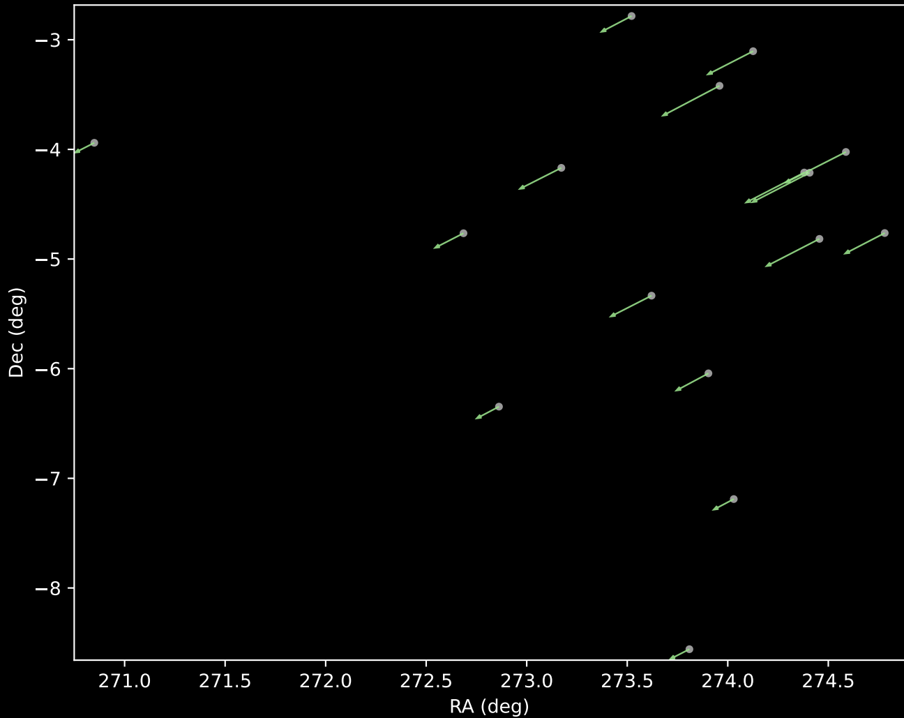
Gaia DR3 Cluster 5 Proper Motion Vectors (n=16)
