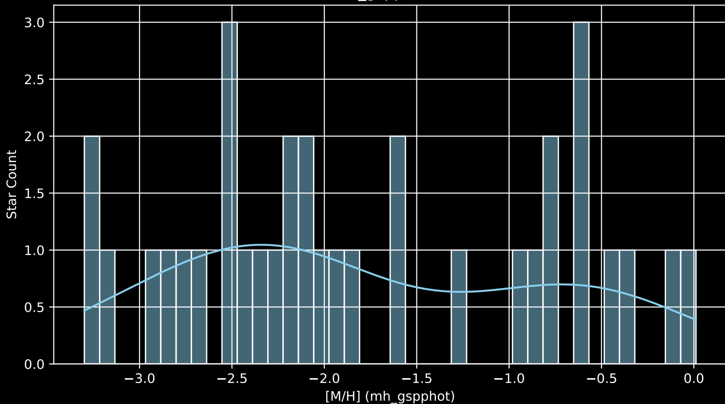
Gaia Stream: [Tuc-3 [M/H] (mh_gspphot) (n= 34)
