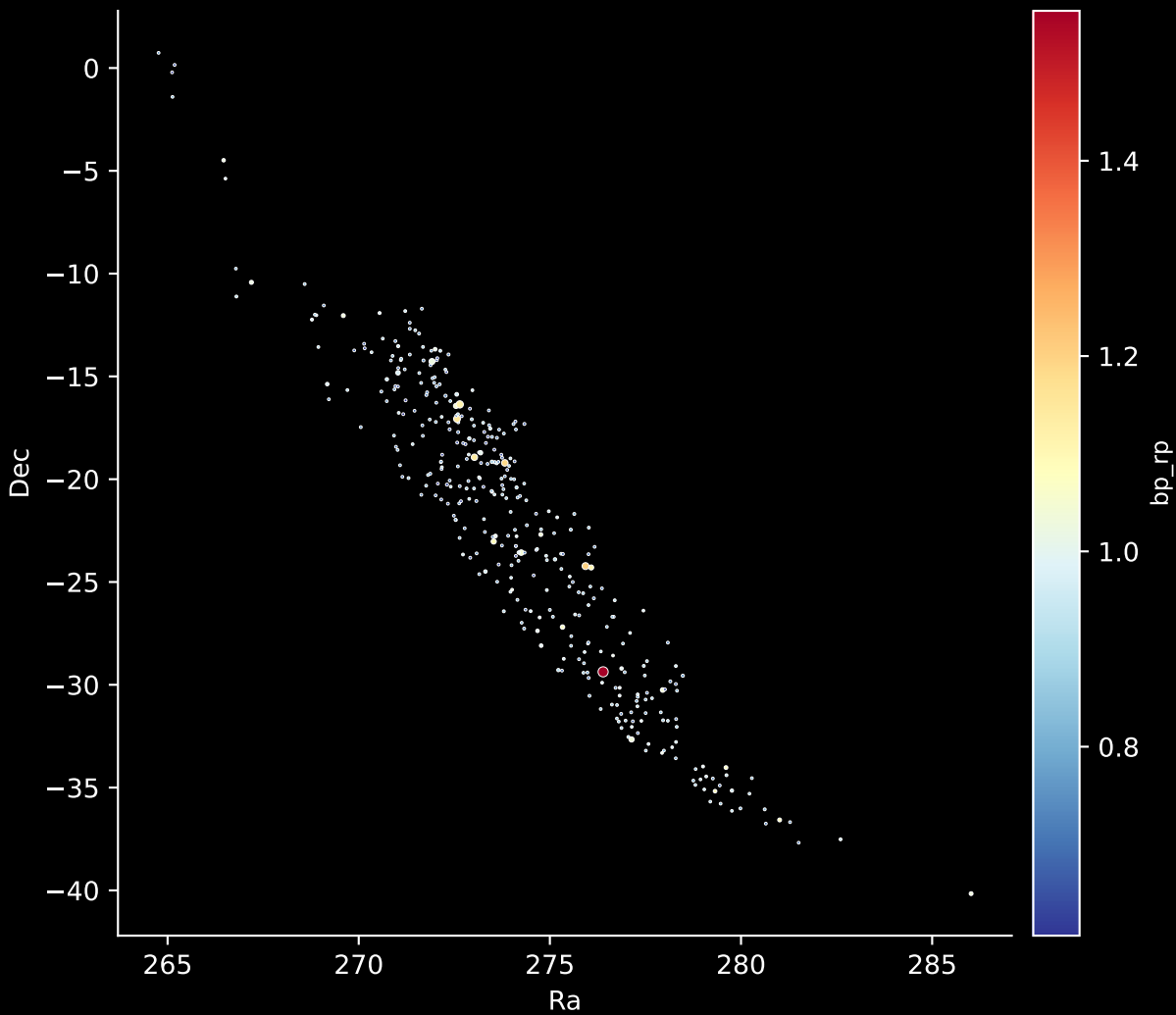
Gaia Stream: [Ylgr] Stars: 628
