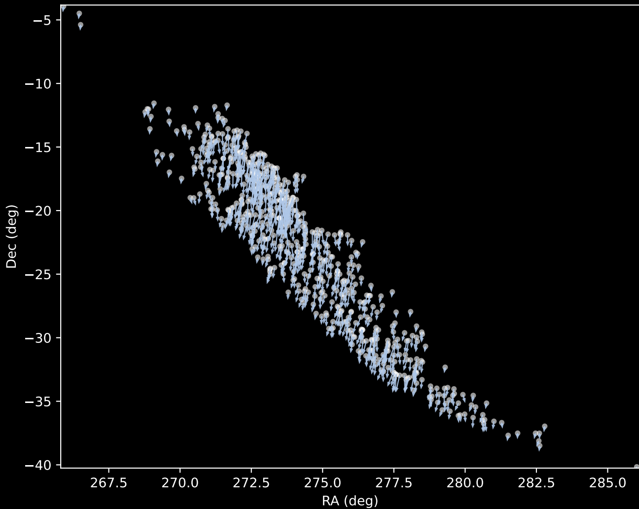
Gaia DR3 Cluster 1 Proper Motion Vectors (n=609)
