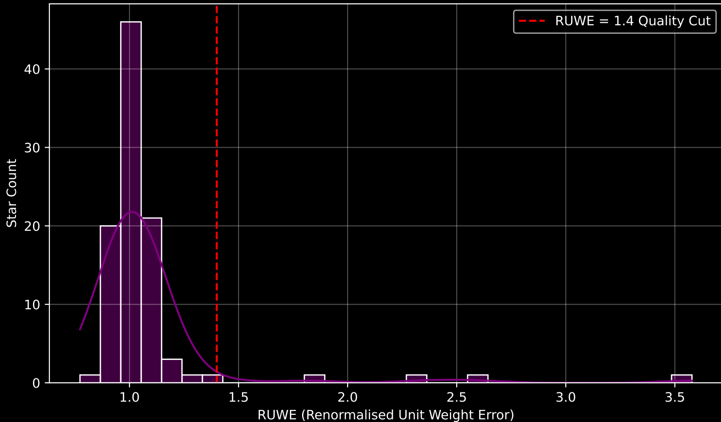
Gaia Cluster: [ASCC_10] RUWE Distribution (n= 97)
