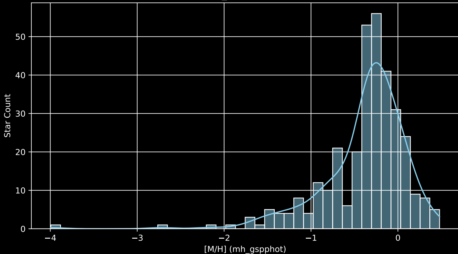
Gaia Cluster: [ASCC_111 [M/H] (mh_gspphot) (n= 329)
