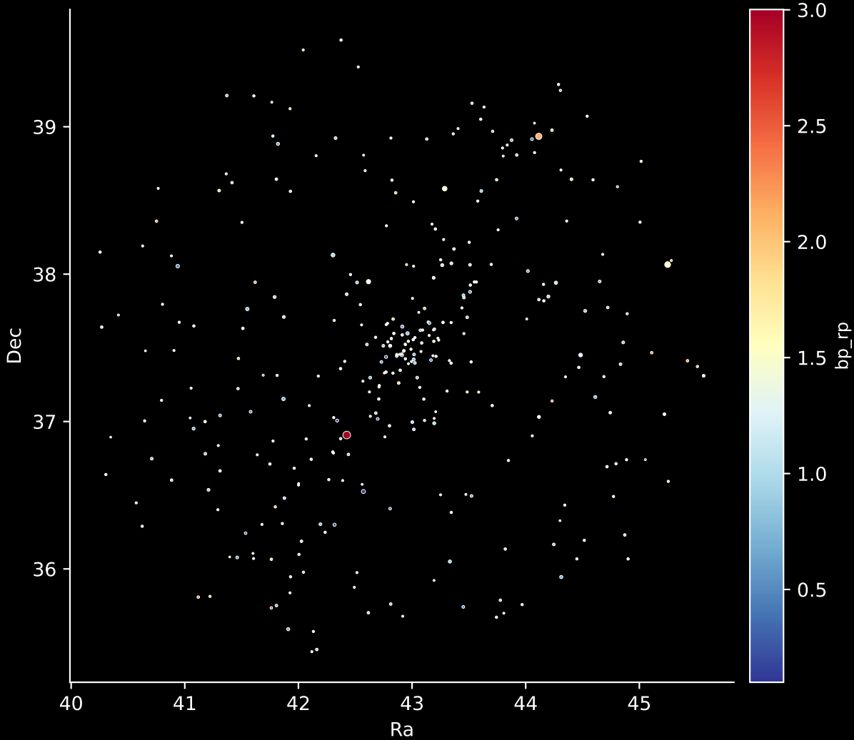
Gaia Cluster: [ASCC_111] Stars: 329
