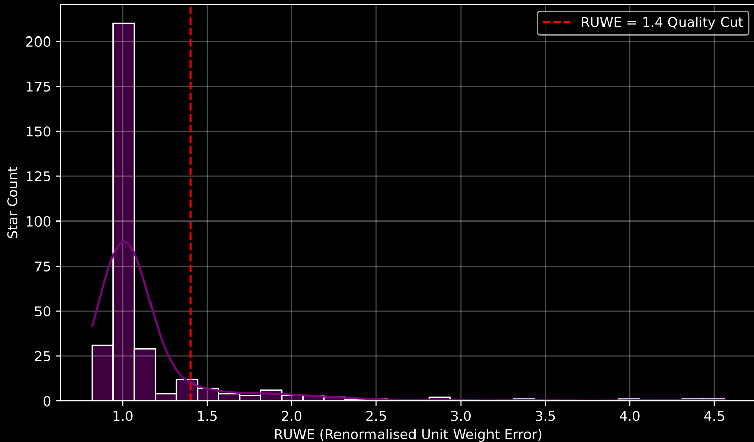
Gaia Cluster: [ASCC_111] RUWE Distribution (n= 322)
