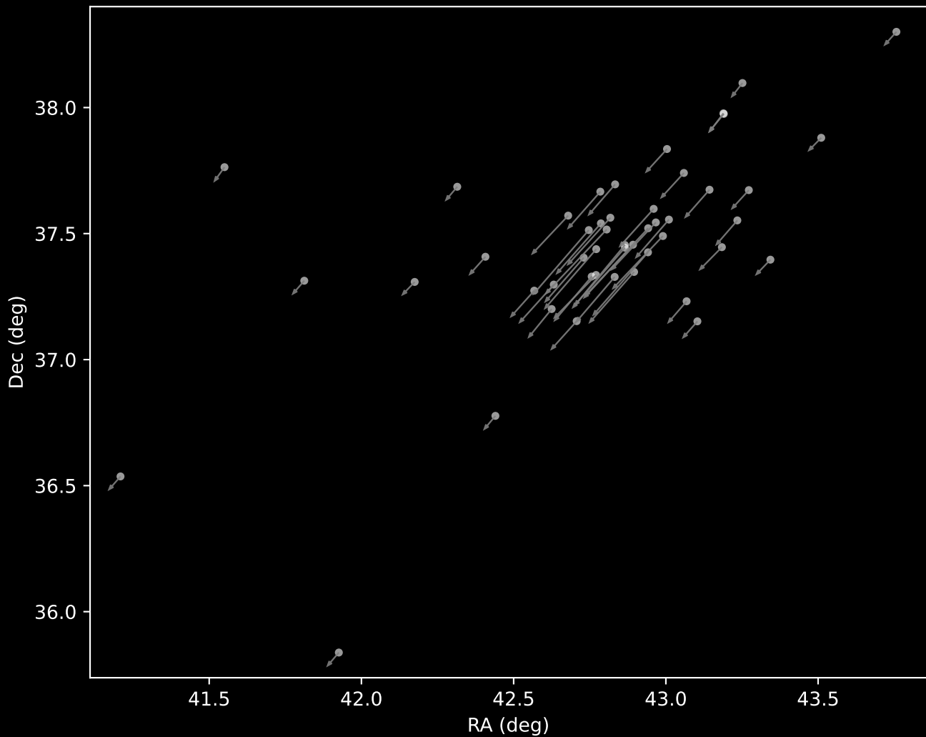
Gaia DR3 Cluster 14 Proper Motion Vectors (n=48)
