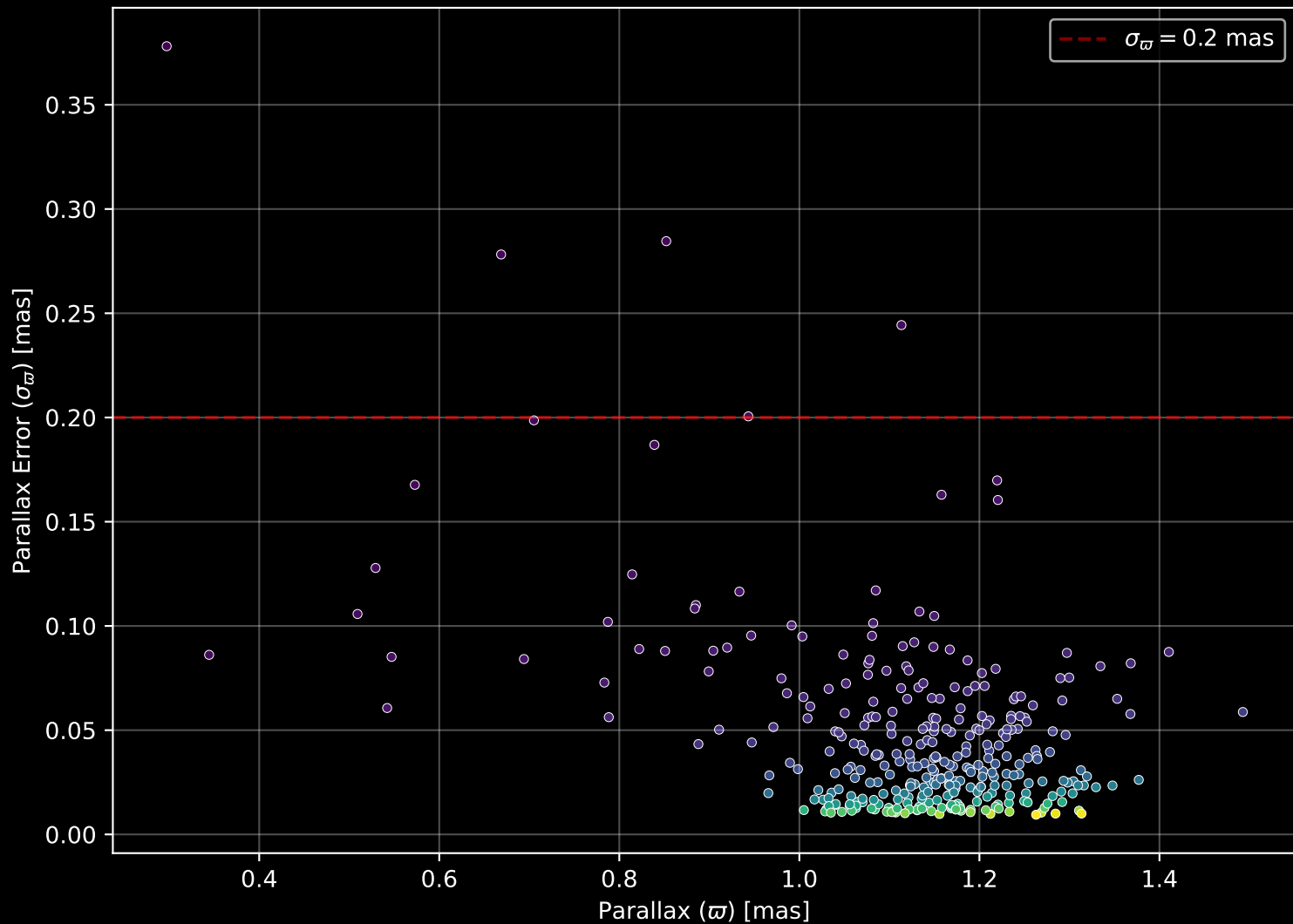
Gaia Cluster: [ASCC_111] Parallax Quality (n= 329)
