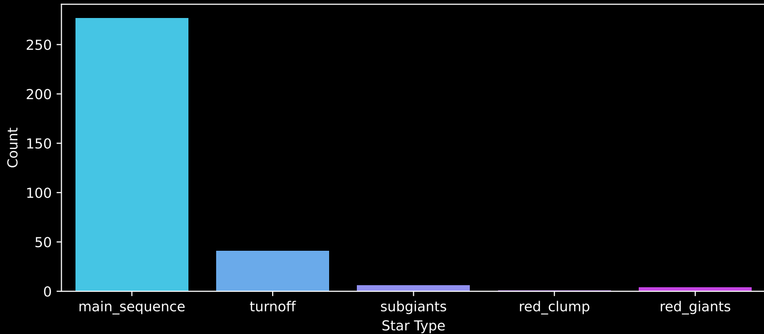
Gaia Cluster: [ASCC_111] Count plot of Star Type
