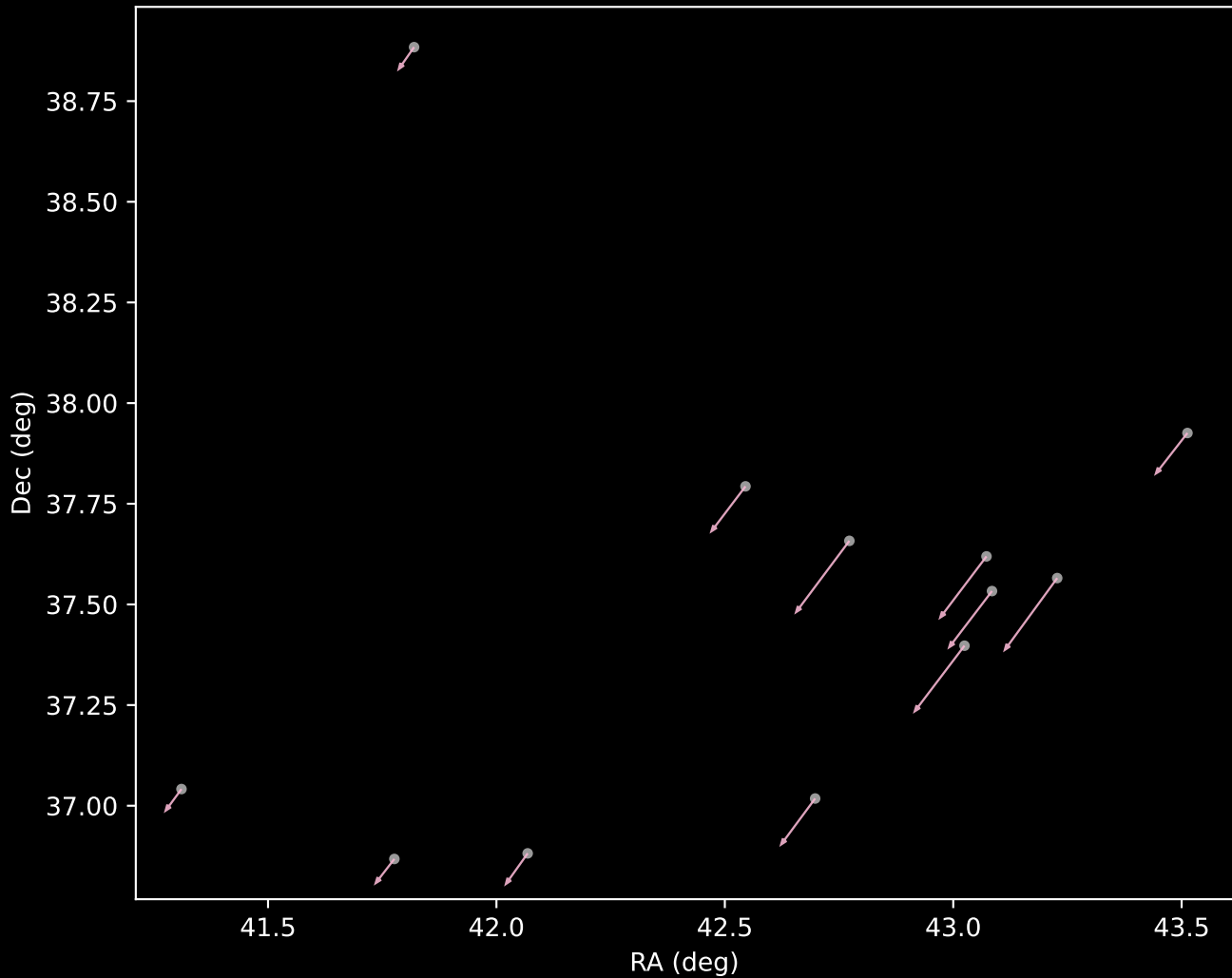
Gaia DR3 Cluster 13 Proper Motion Vectors (n=12)
