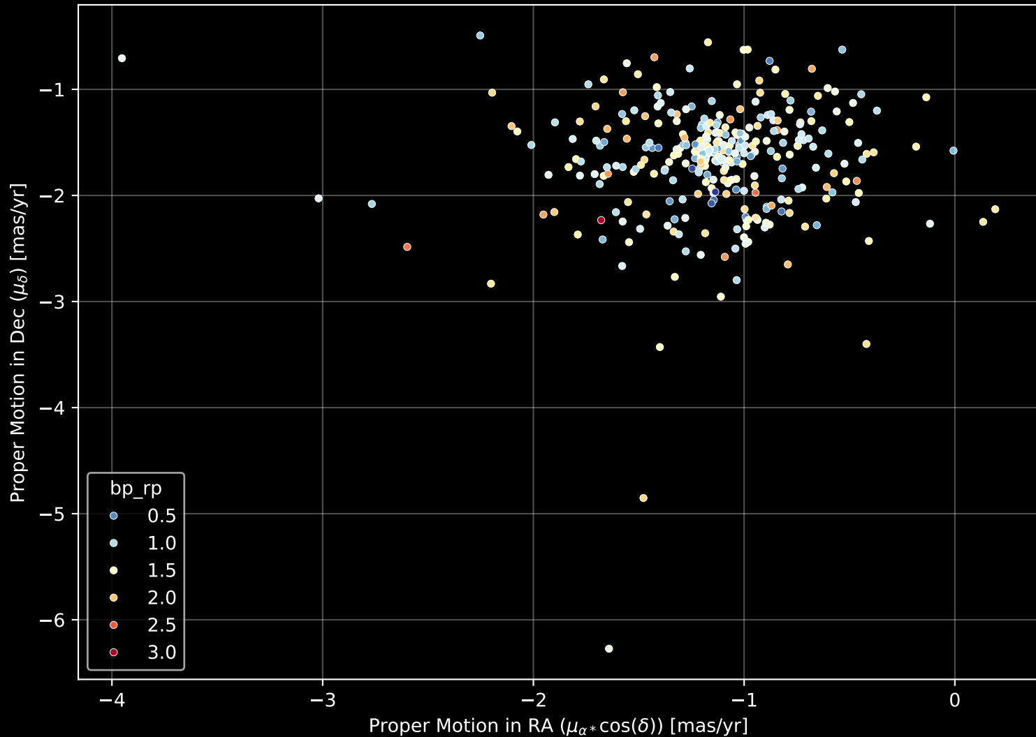
Gaia Cluster: [ASCC_111] Proper Motion Diagram (n= 329)
