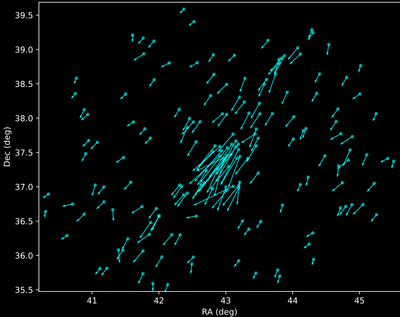
Gaia DR3 Noise Stream Proper Motion Vectors (n=167)
