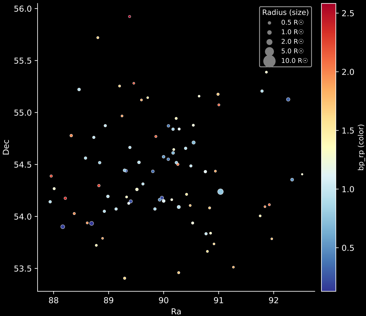
Gaia Cluster: [ASCC_128] Stars: 84
