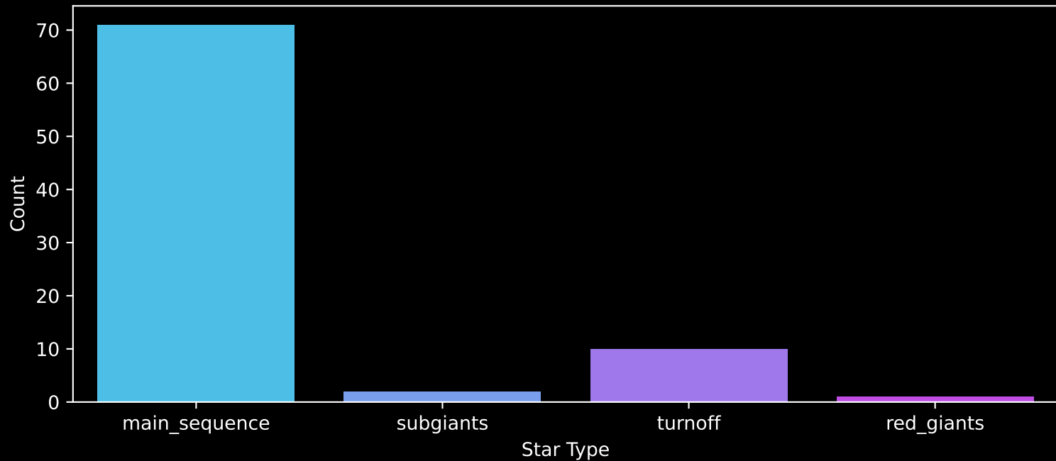
Gaia Cluster: [ASCC_128] Count plot of Star Type
