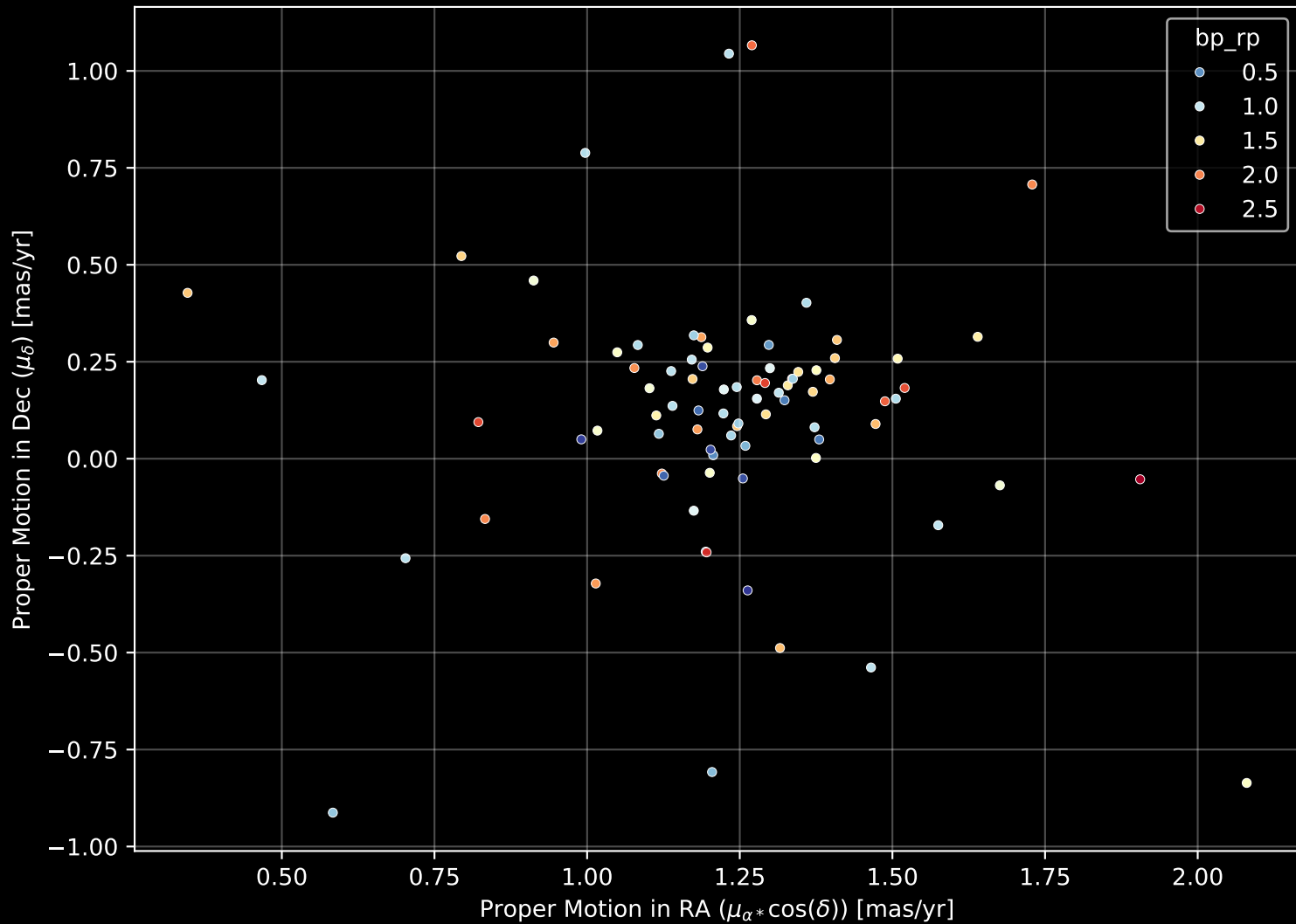
Gaia Cluster: [ASCC_128] Proper Motion Diagram (n= 84)
