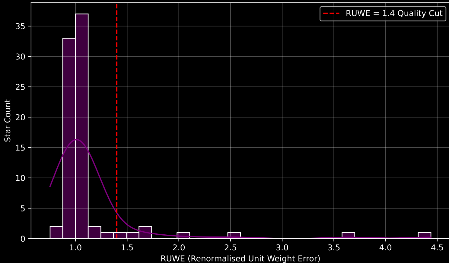
Gaia Cluster: [ASCC_128] RUWE Distribution (n= 83)
