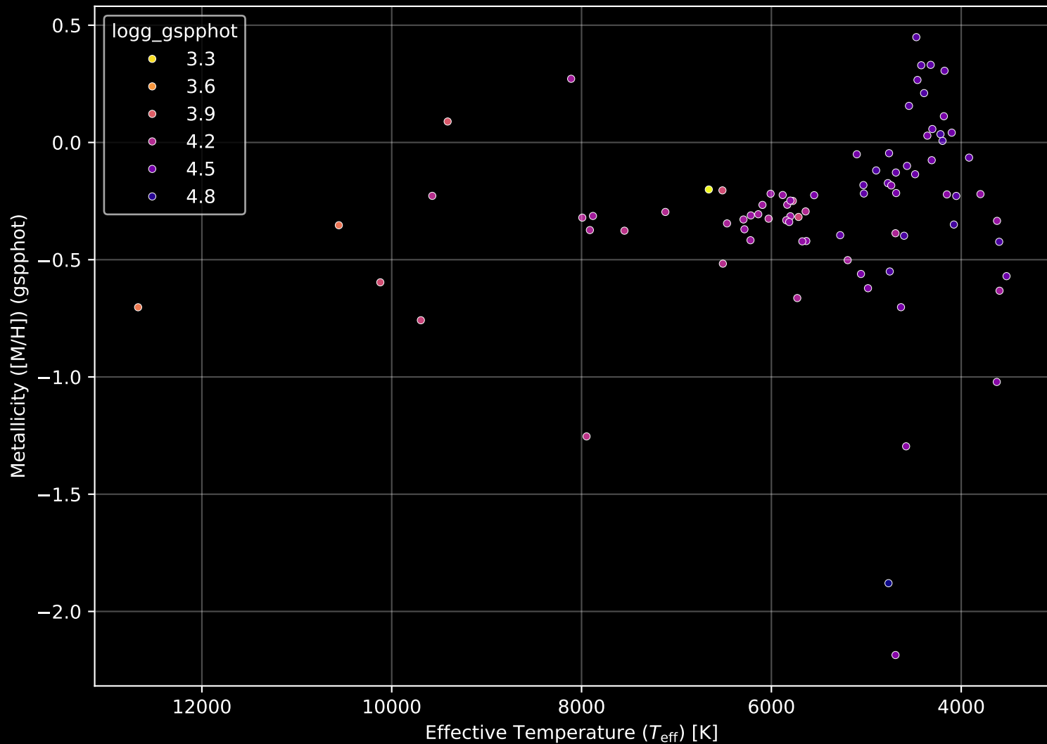
Gaia Cluster: [ASCC_128] Stellar Population Parameters (n= 84)
