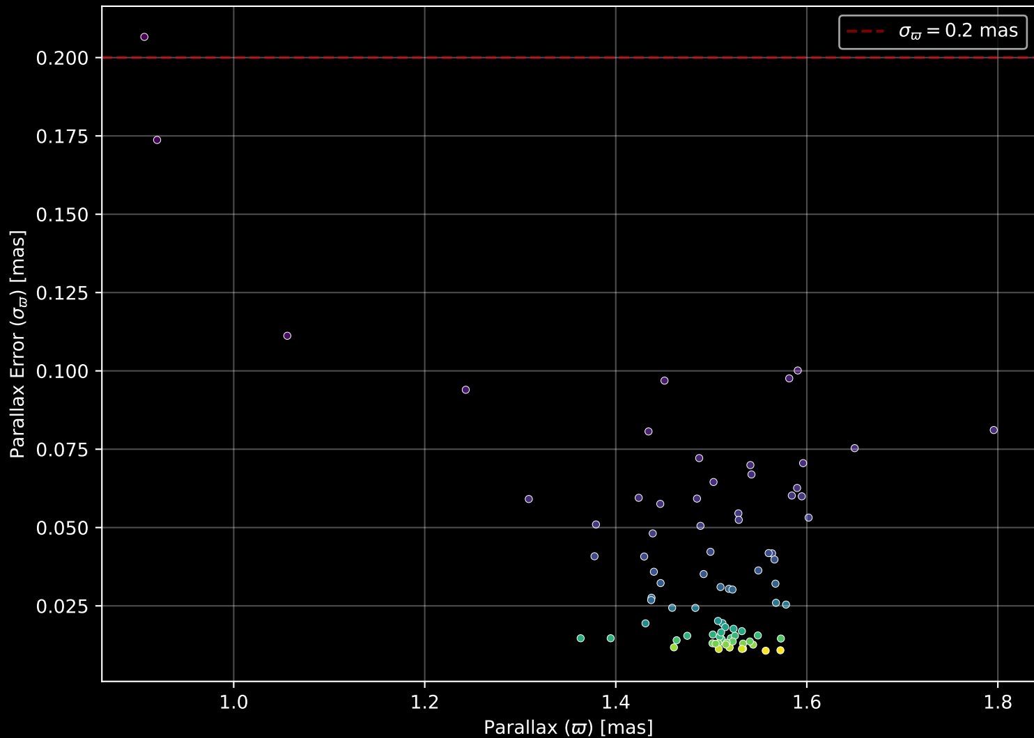
Gaia Cluster: [ASCC_128] Parallax Quality (n= 84)
