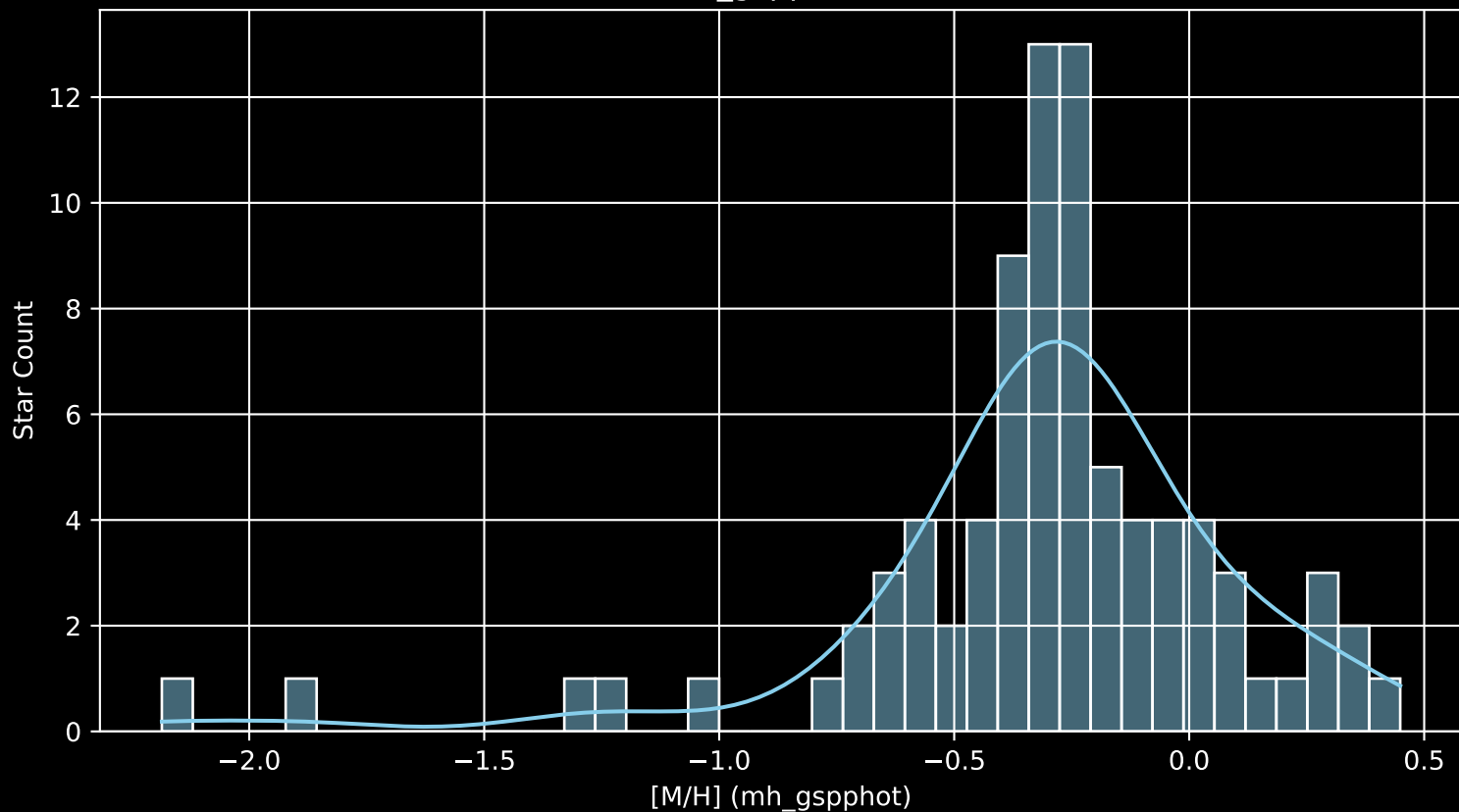
Gaia Cluster: [ASCC_128 [M/H] (mh_gspphot) (n= 84)
