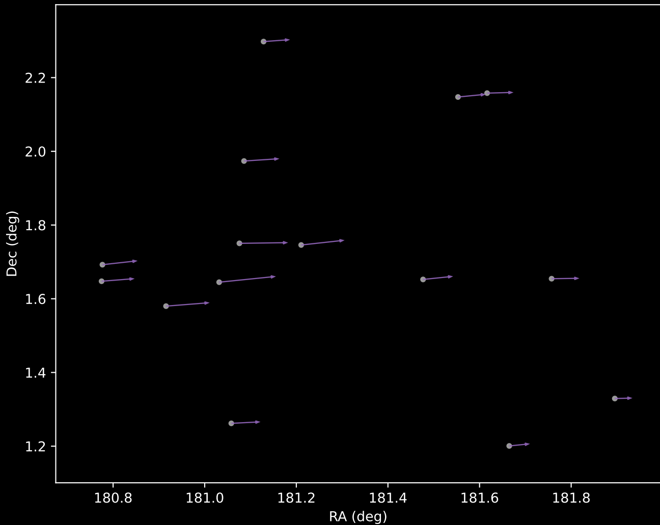
Gaia DR3 Cluster 8 Proper Motion Vectors (n=15)
