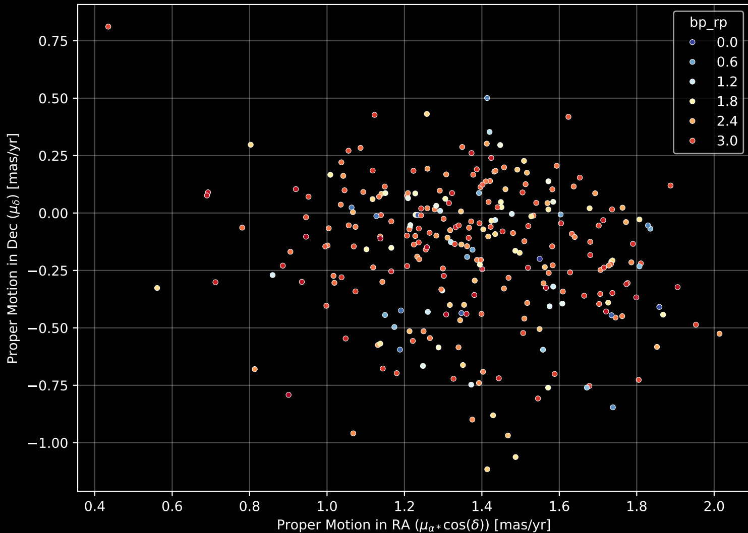
Gaia Cluster: [ASCC_16] Proper Motion Diagram (n= 276)
