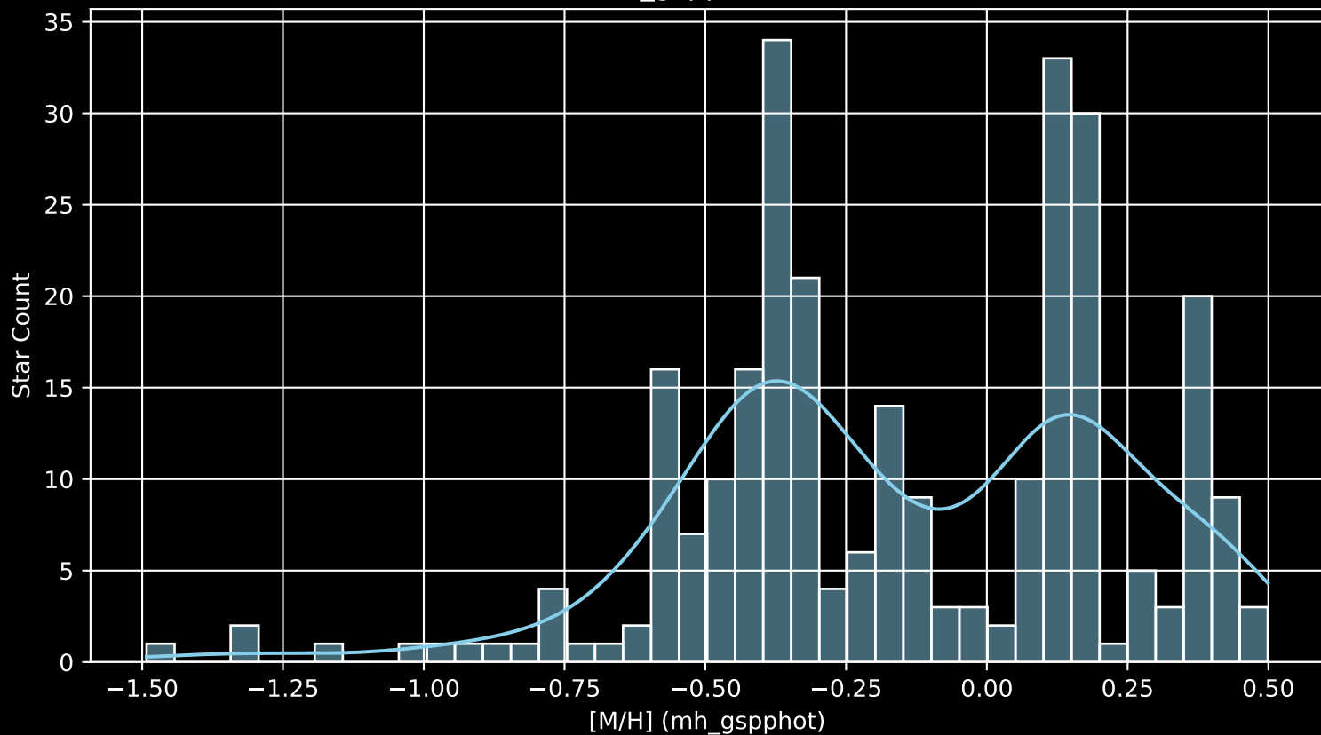
Gaia Cluster: [ASCC_16 [M/H] (mh_gspphot) (n= 276)
