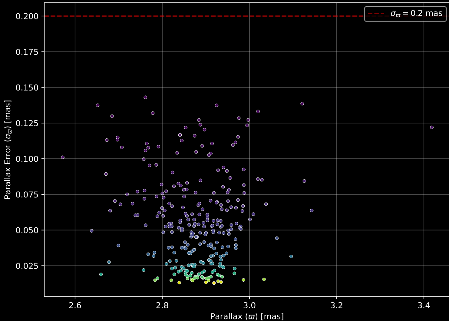
Gaia Cluster: [ASCC_16] Parallax Quality (n= 276)
