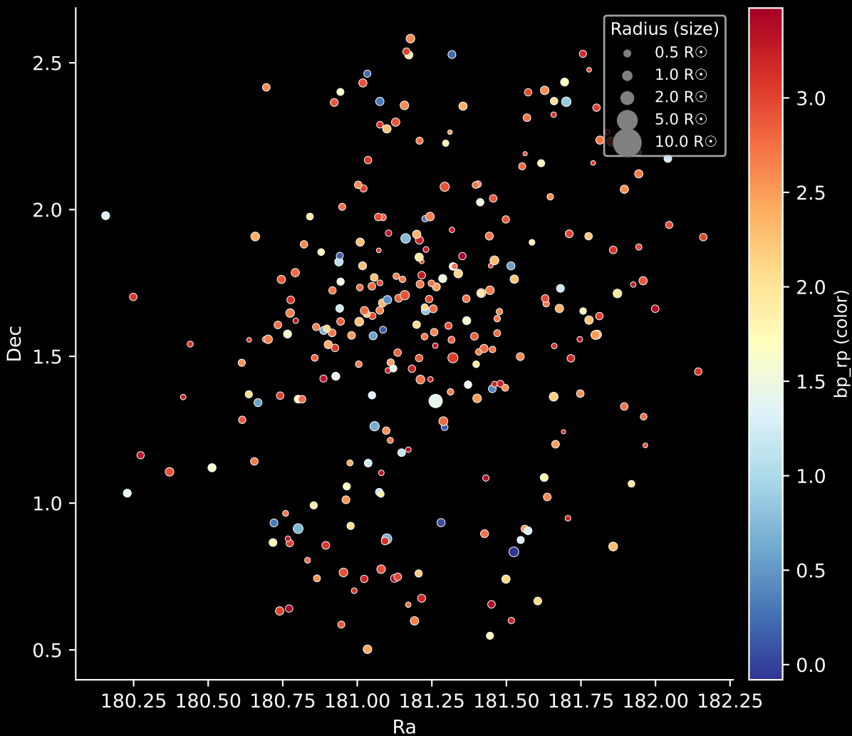
Gaia Cluster: [ASCC_16] Stars: 276
