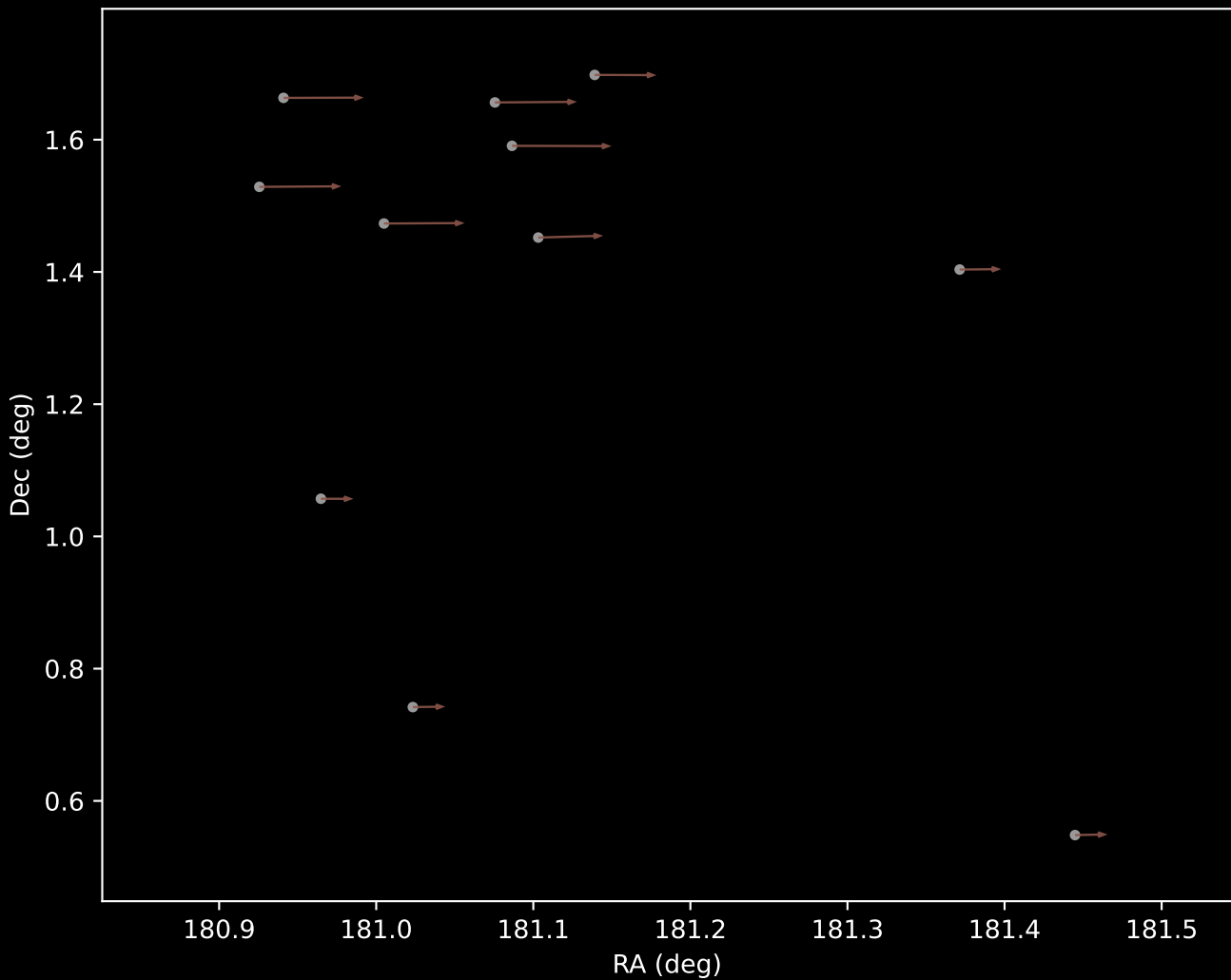
Gaia DR3 Cluster 10 Proper Motion Vectors (n=11)
