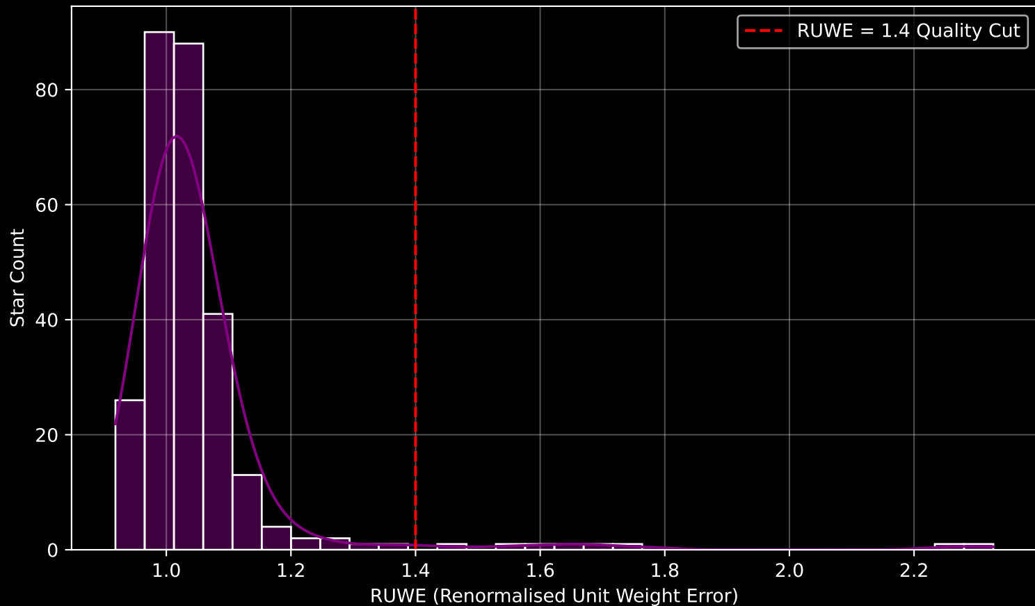
Gaia Cluster: [ASCC_16] RUWE Distribution (n= 276)
