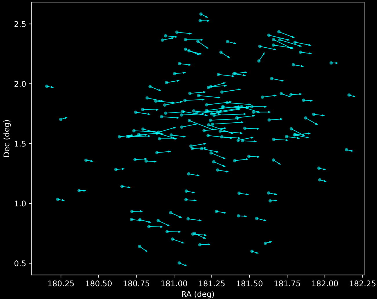
Gaia DR3 Noise Stream Proper Motion Vectors (n=141)
