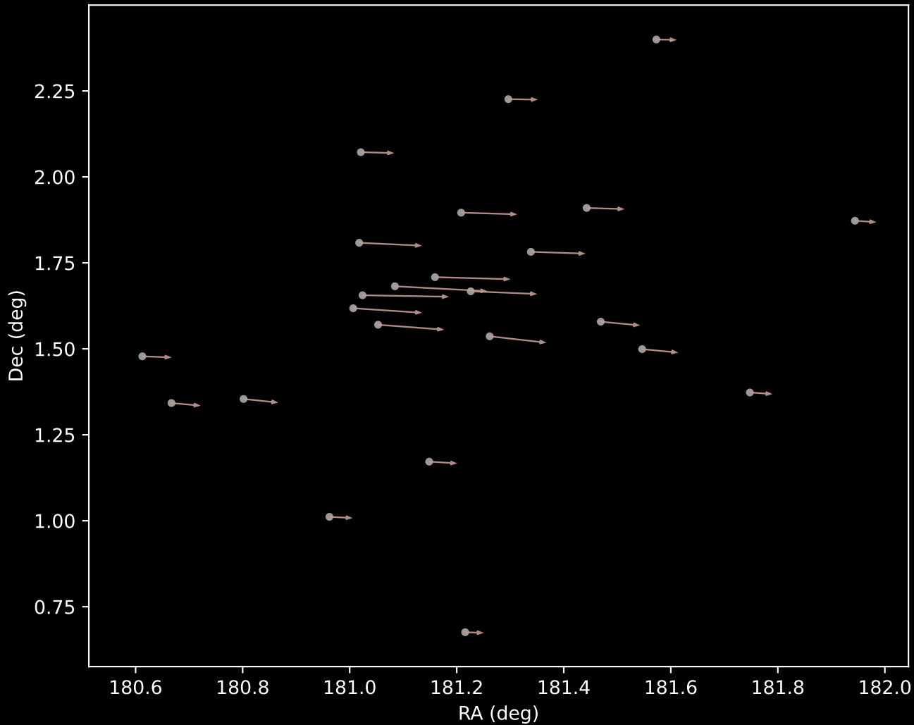
Gaia DR3 Cluster 11 Proper Motion Vectors (n=24)
