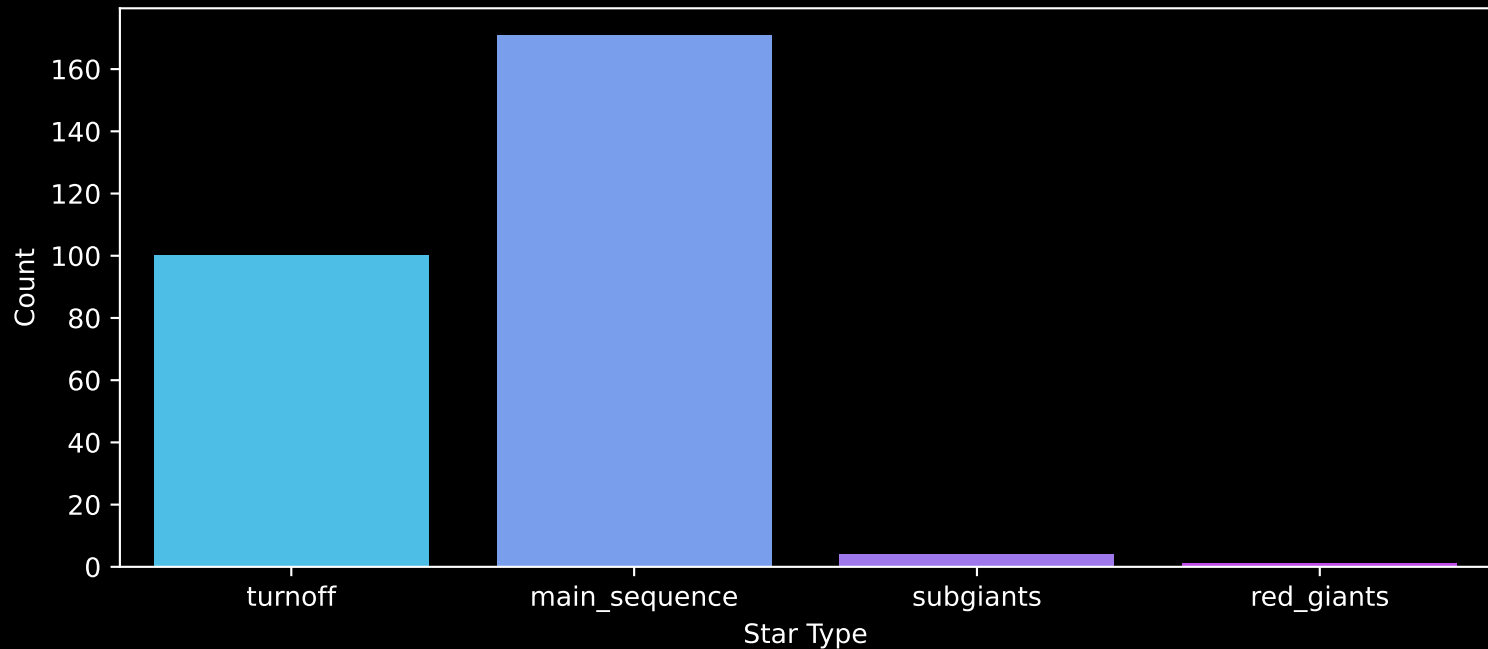
Gaia Cluster: [ASCC_16] Count plot of Star Type
