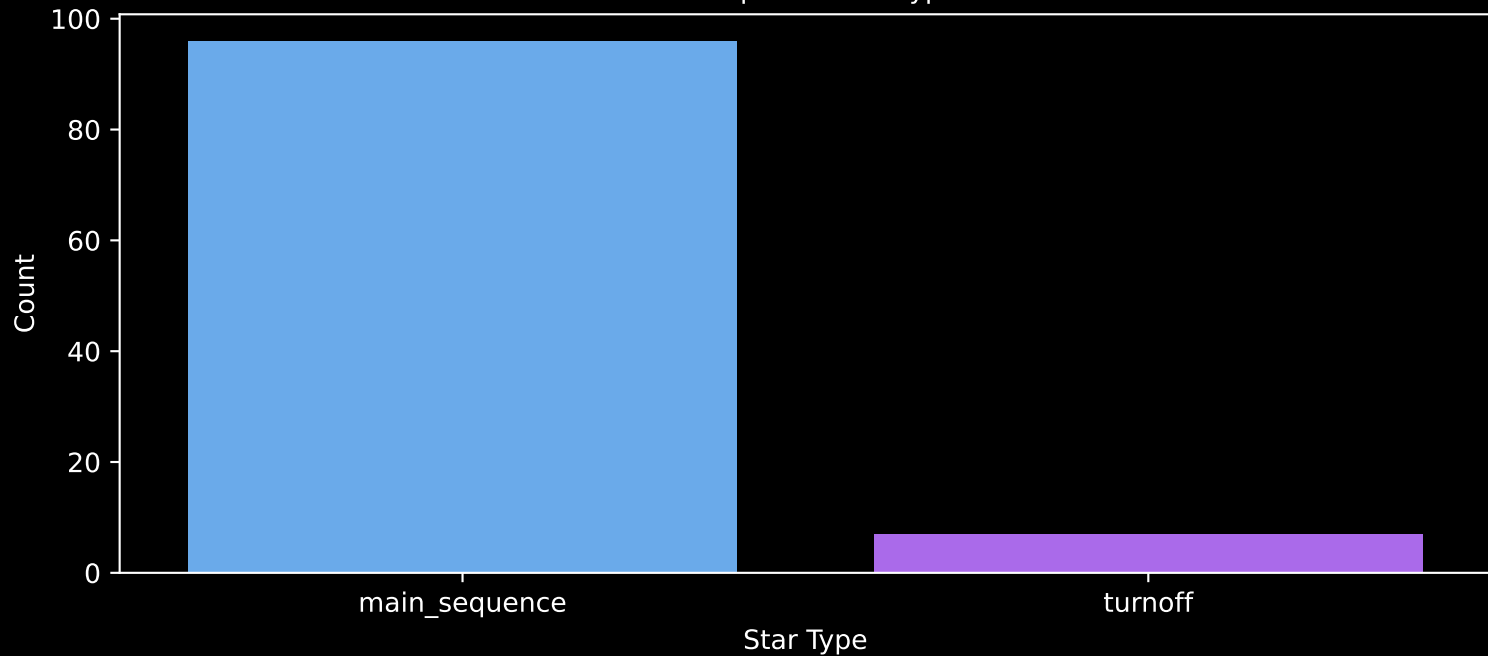
Gaia Cluster: [ASCC_41] Count plot of Star Type
