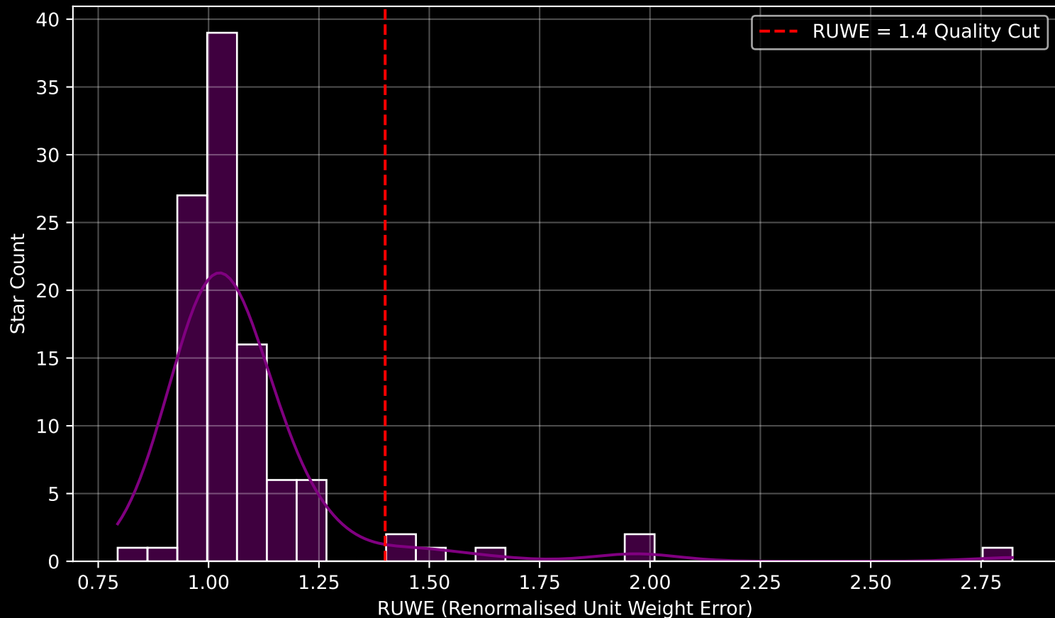
Gaia Cluster: [ASCC_41] RUWE Distribution (n= 103)
