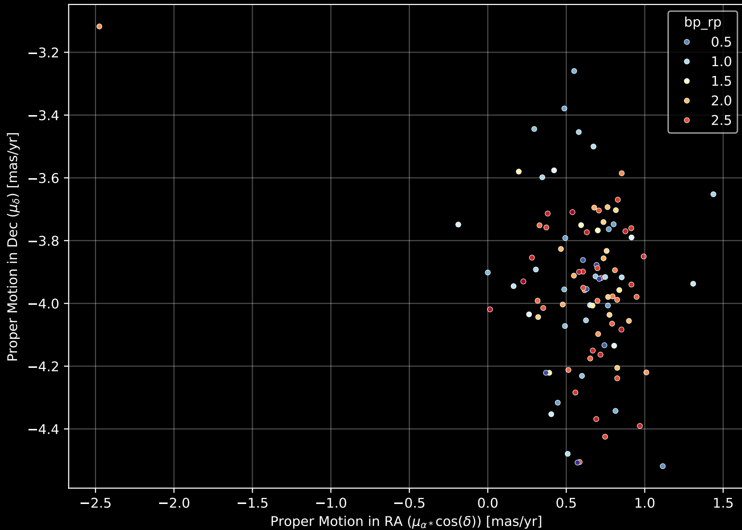
Gaia Cluster: [ASCC_41] Proper Motion Diagram (n= 103)
