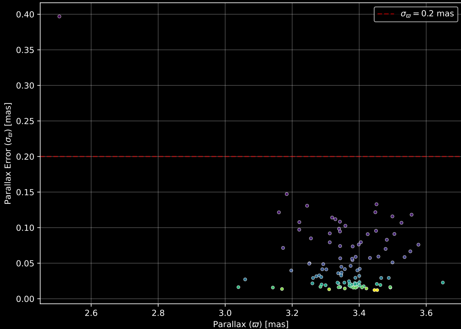
Gaia Cluster: [ASCC_41] Parallax Quality (n= 103)
