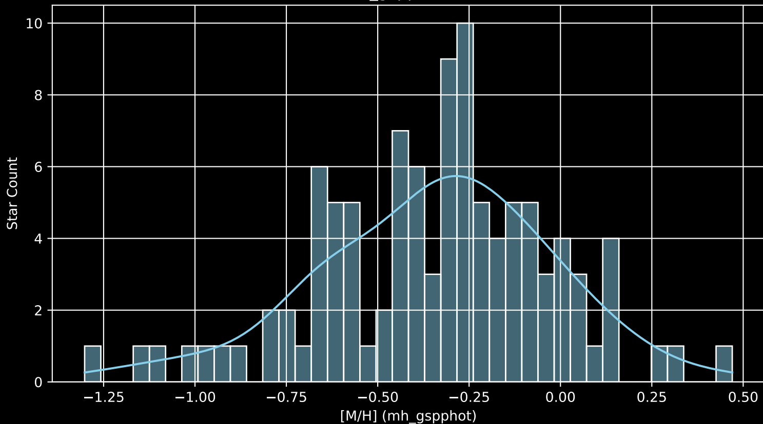
Gaia Cluster: [ASCC_41 [M/H] (mh_gspphot) (n= 103)
