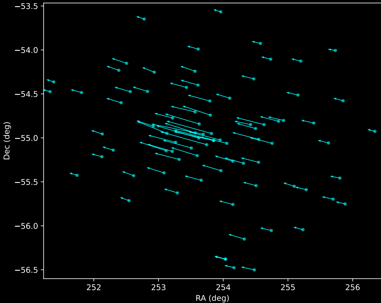
Gaia DR3 Noise Stream Proper Motion Vectors (n=82)
