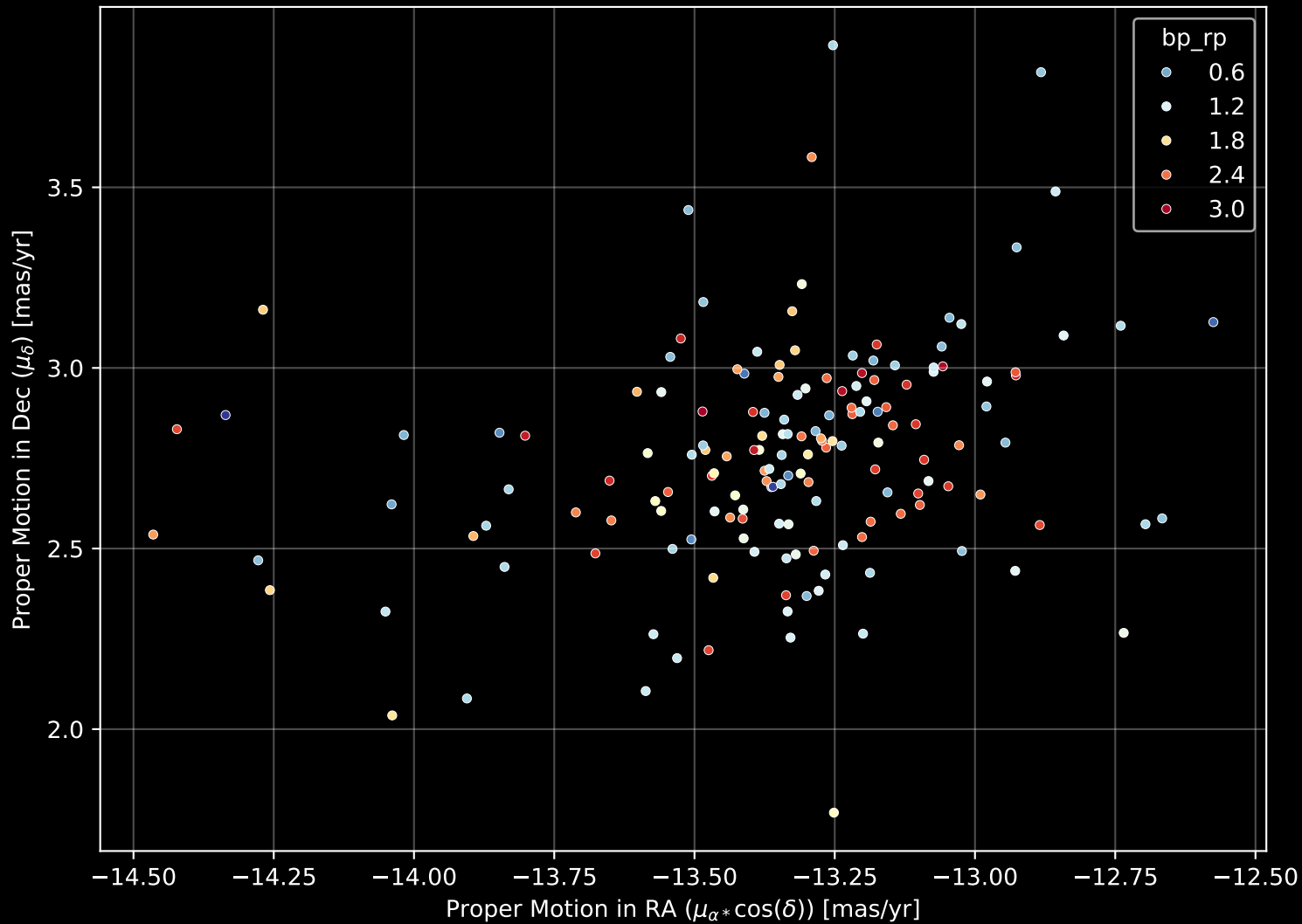
Gaia Cluster: [ASCC_58] Proper Motion Diagram (n= 161)
