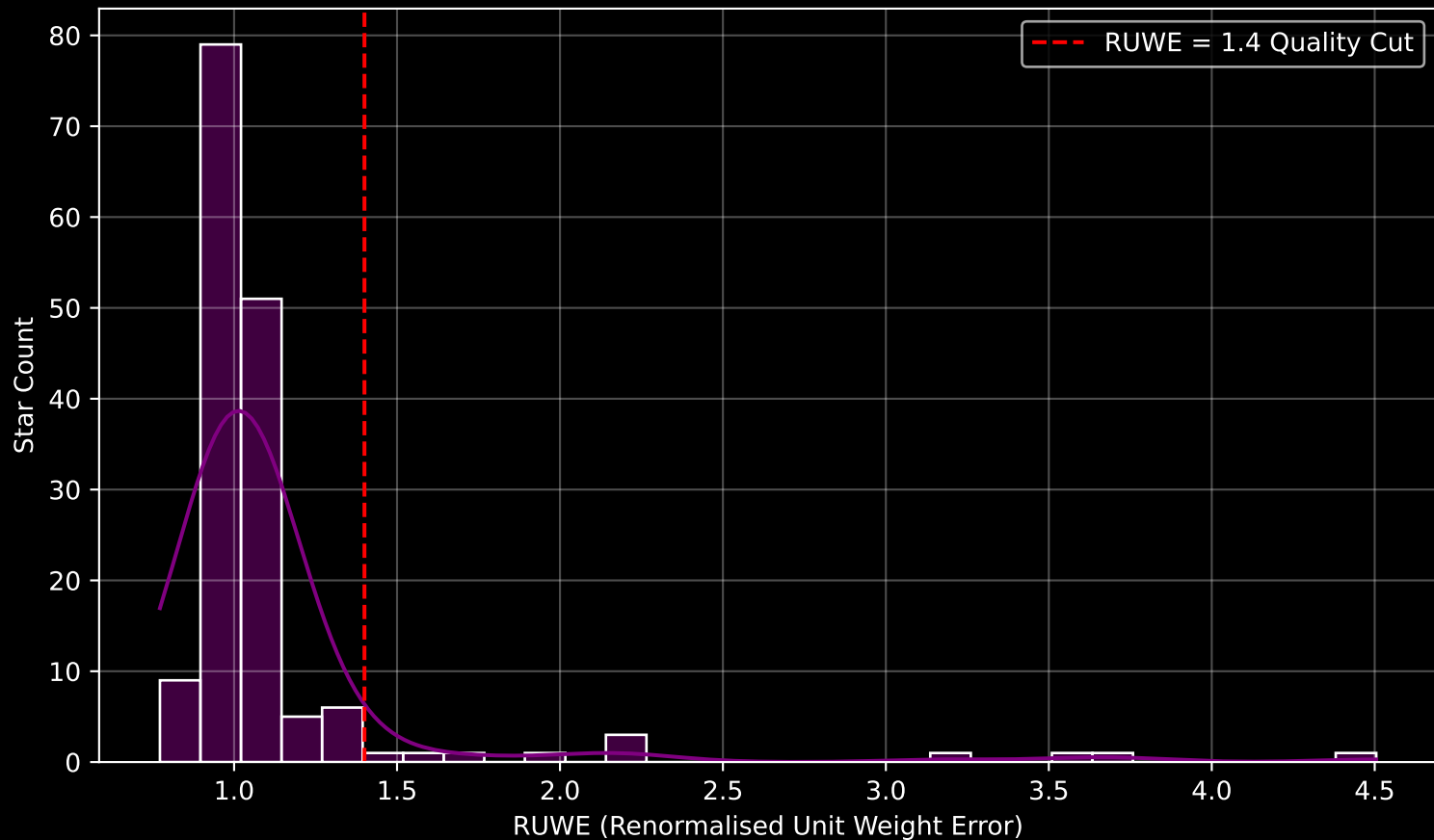
Gaia Cluster: [ASCC_58] RUWE Distribution (n= 161)
