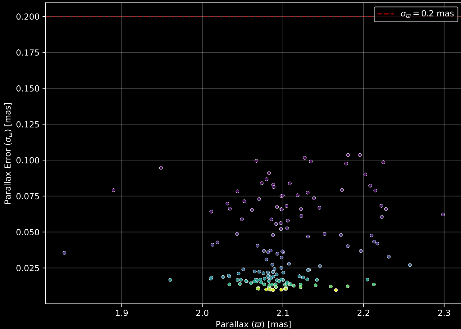
Gaia Cluster: [ASCC_58] Parallax Quality (n= 161)
