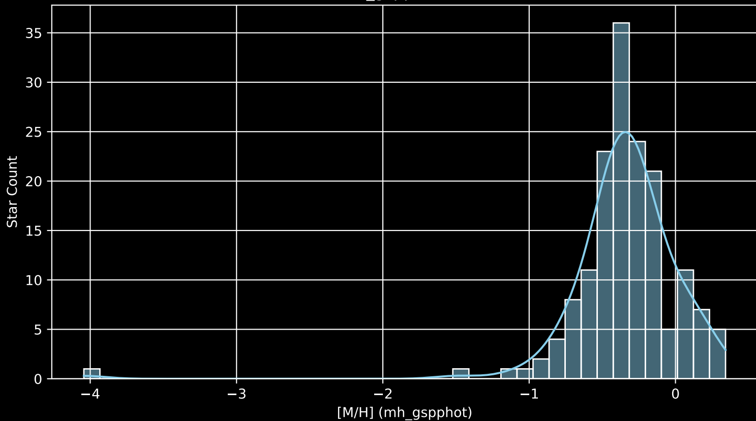
Gaia Cluster: [ASCC_58 [M/H] (mh_gspphot) (n= 161)
