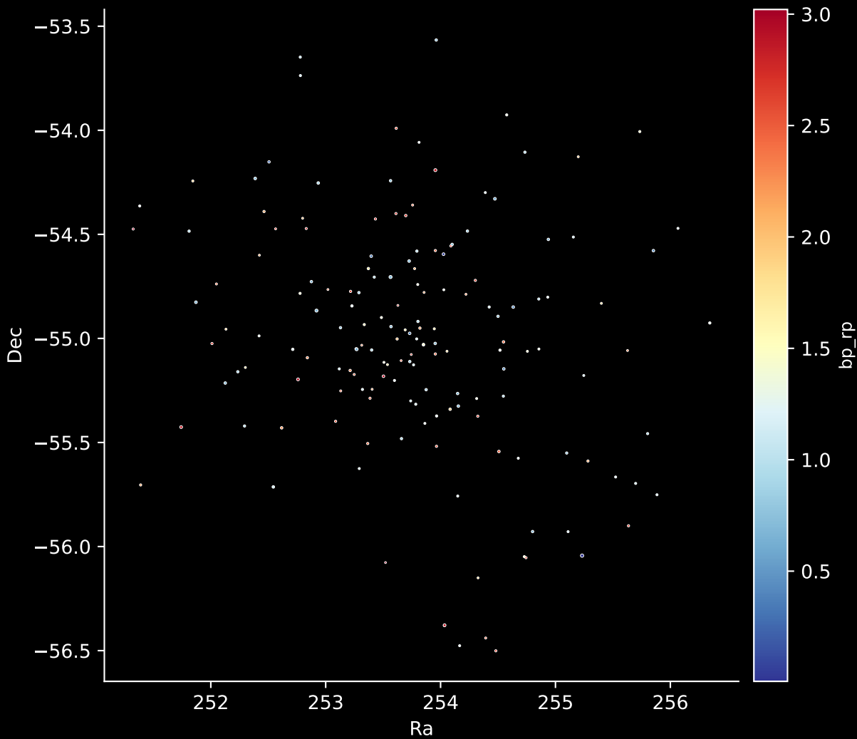
Gaia Cluster: [ASCC_58] Stars: 161
