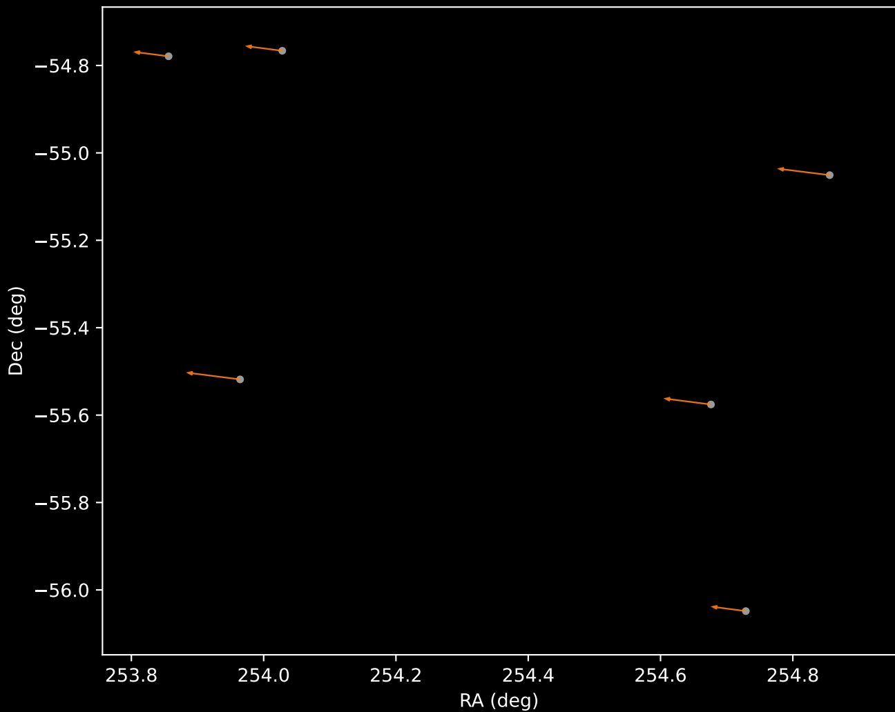
Gaia DR3 Cluster 2 Proper Motion Vectors (n=6)
