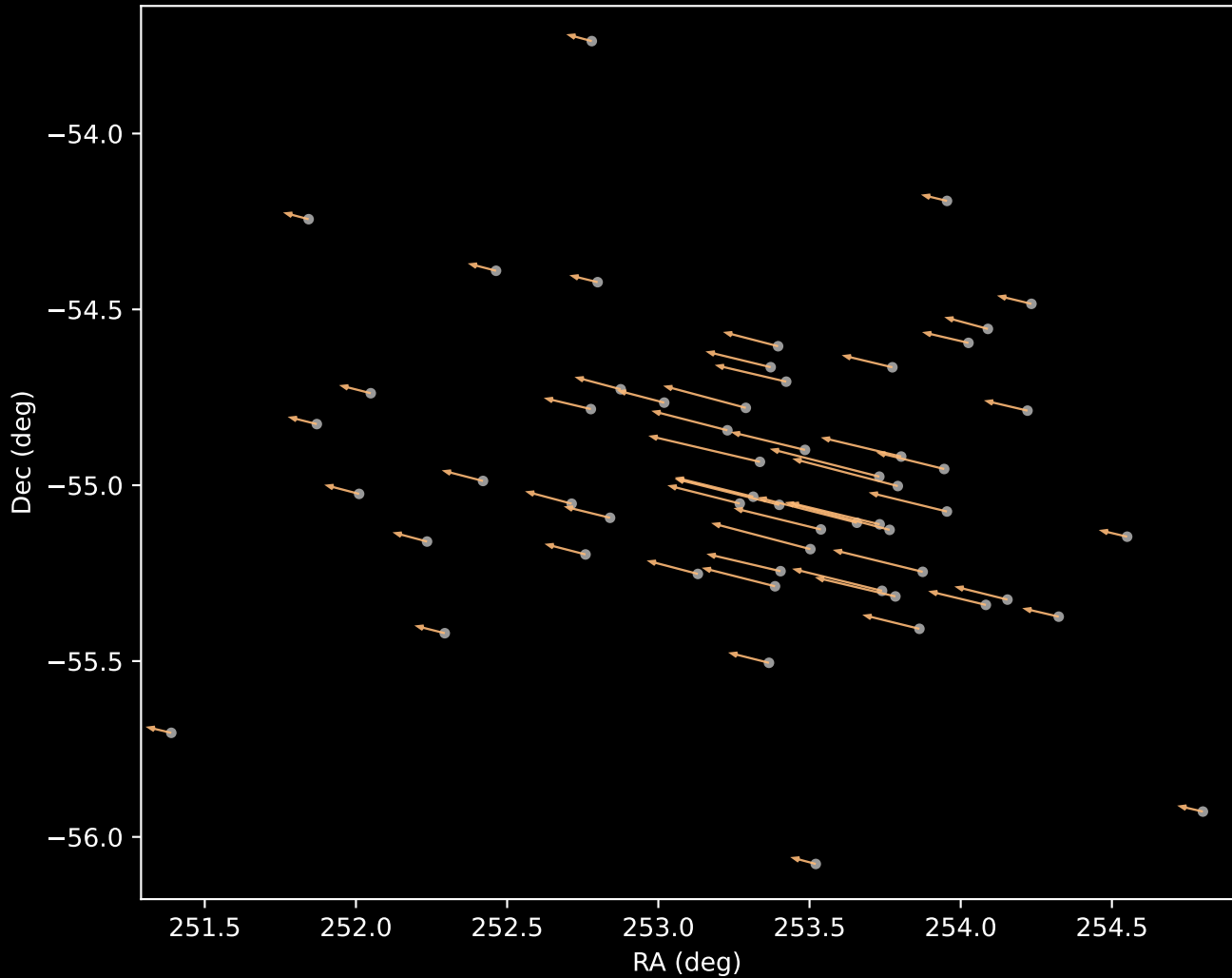
Gaia DR3 Cluster 3 Proper Motion Vectors (n=57)
