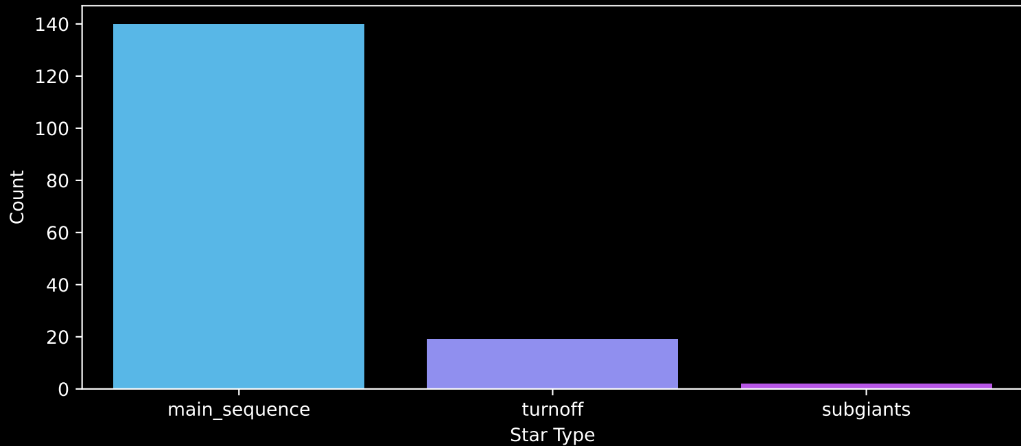
Gaia Cluster: [ASCC_58] Count plot of Star Type
