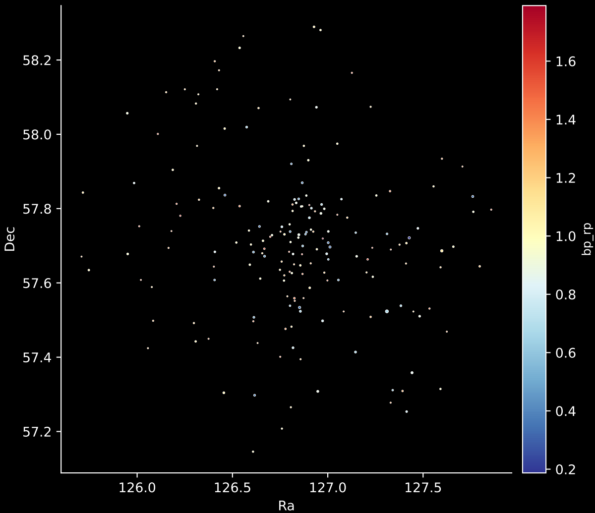
Gaia Cluster: [ASCC_6] Stars: 183
