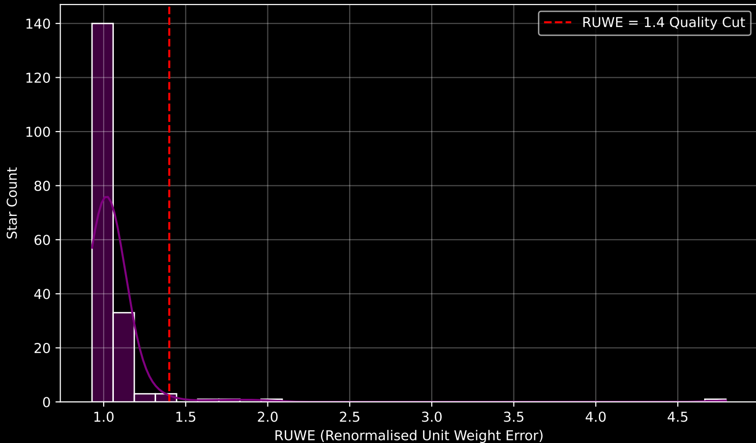
Gaia Cluster: [ASCC_6] RUWE Distribution (n= 183)
