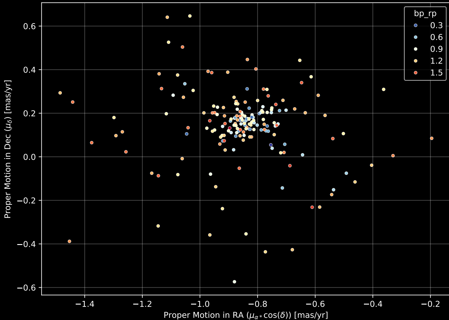
Gaia Cluster: [ASCC_6] Proper Motion Diagram (n= 183)
