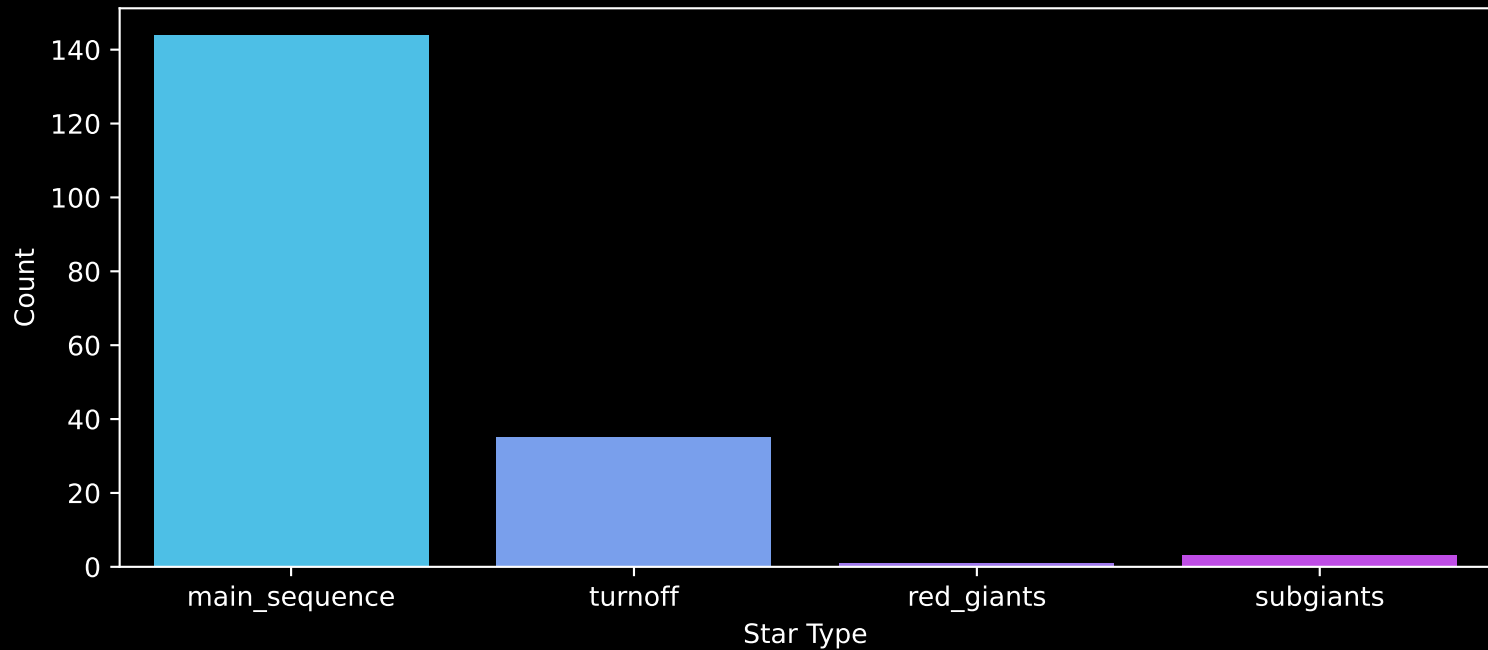
Gaia Cluster: [ASCC_6] Count plot of Star Type
