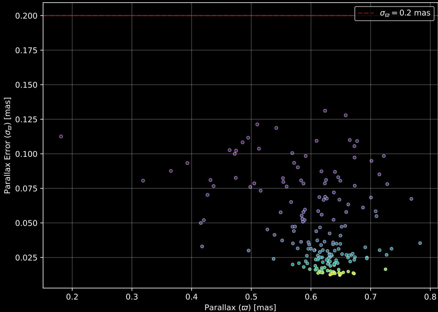
Gaia Cluster: [ASCC_6] Parallax Quality (n= 183)
