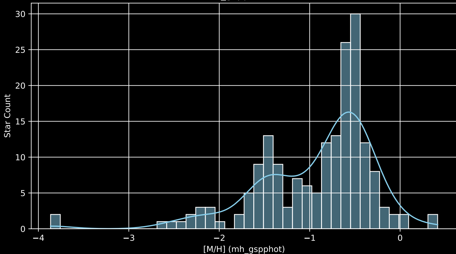
Gaia Cluster: [ASCC_6 [M/H] (mh_gspphot) (n= 183)
