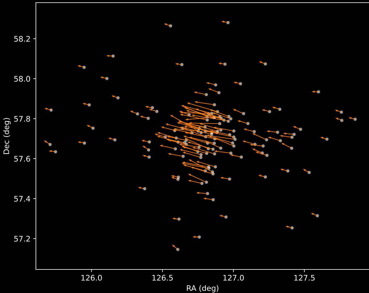
Gaia DR3 Cluster 2 Proper Motion Vectors (n=129)
