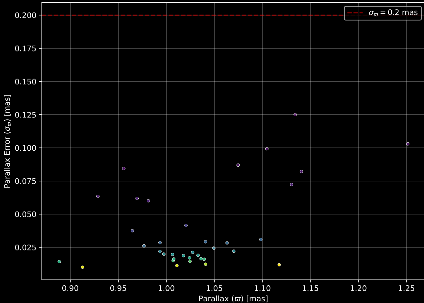
Gaia Cluster: [ASCC_66] Parallax Quality (n= 36)
