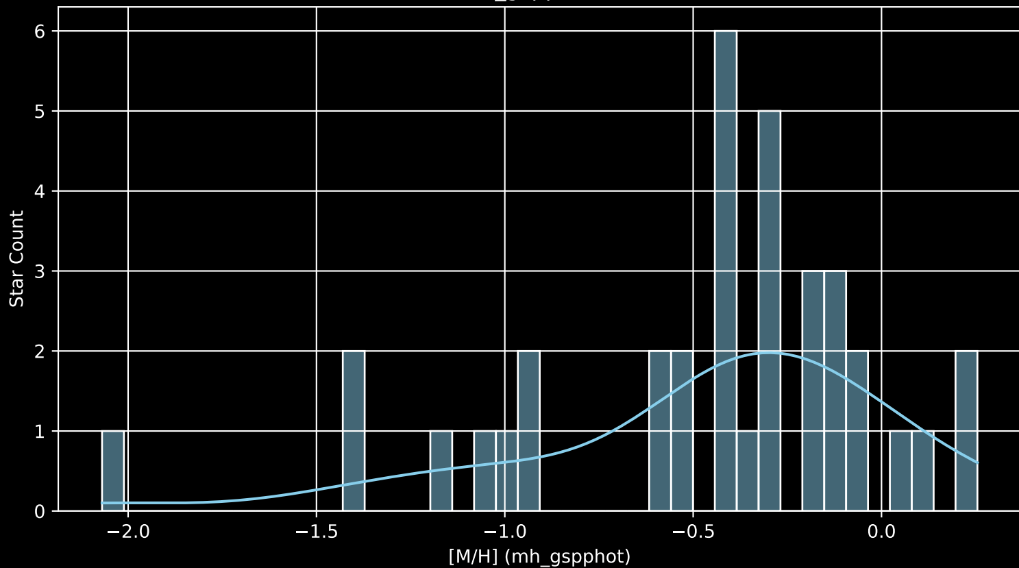
Gaia Cluster: [ASCC_66 [M/H] (mh_gspphot) (n= 36)
