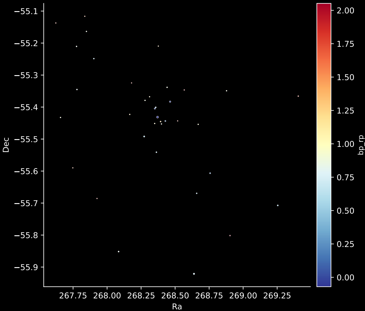
Gaia Cluster: [ASCC_66] Stars: 36
