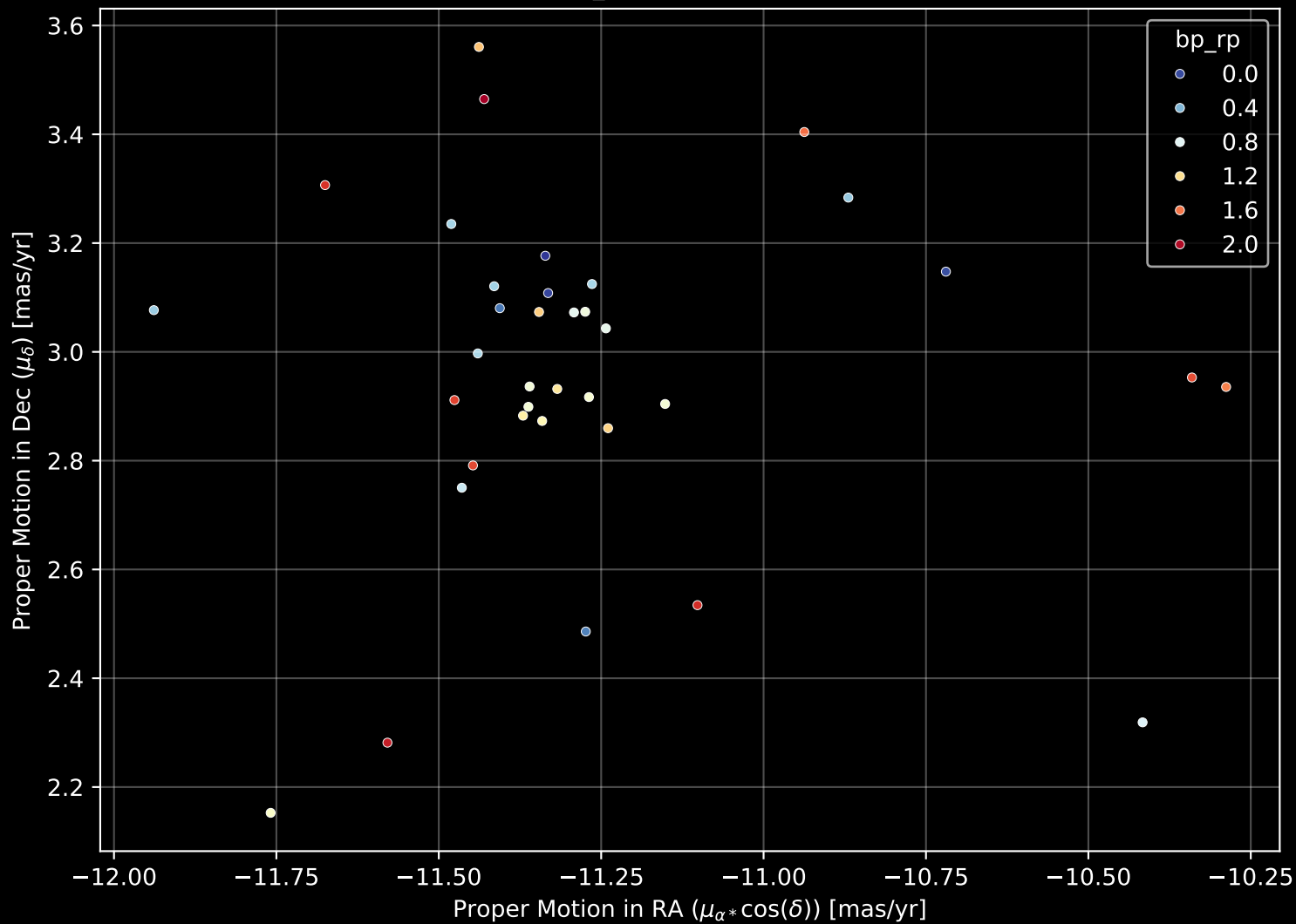
Gaia Cluster: [ASCC_66] Proper Motion Diagram (n= 36)
