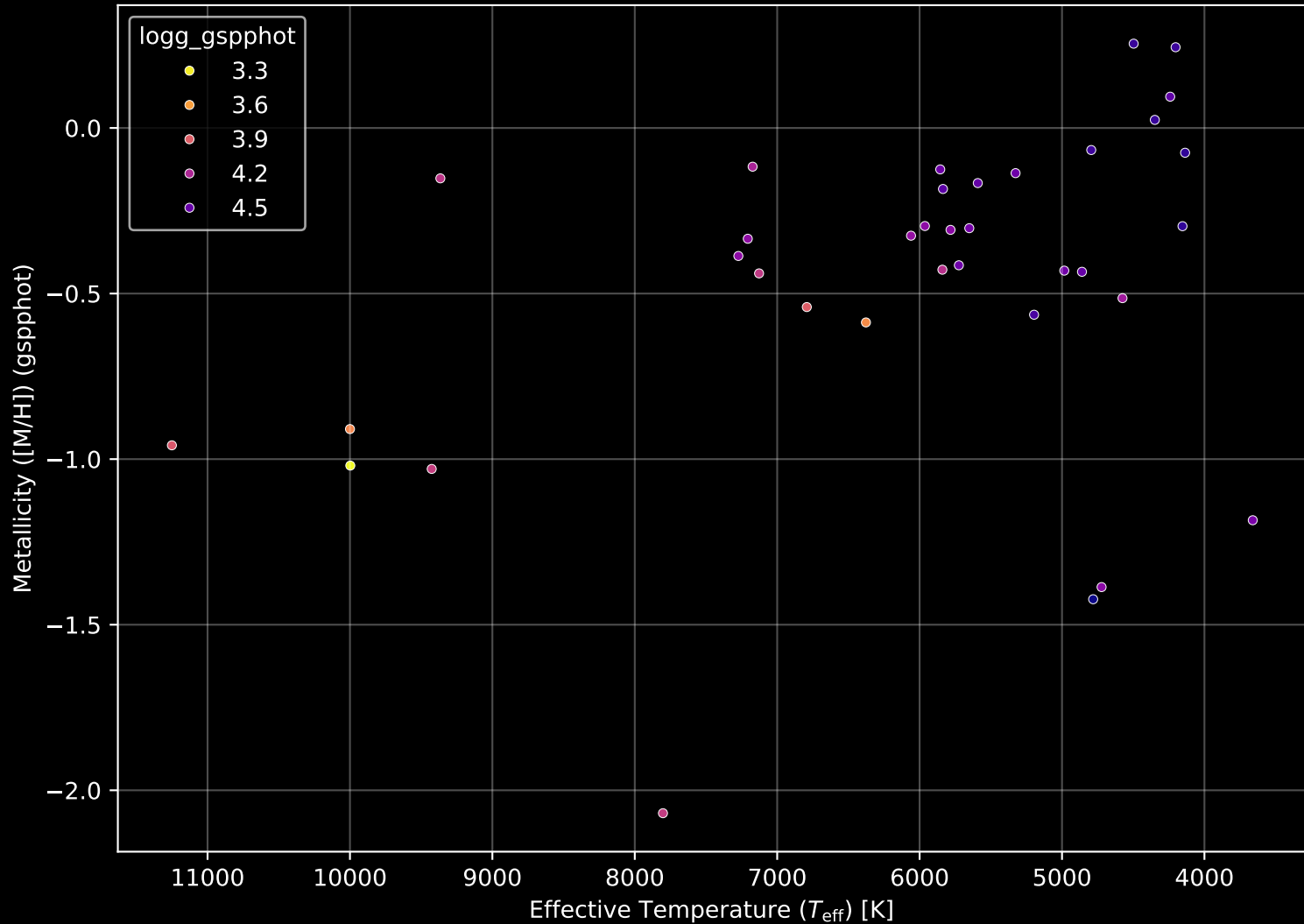
Gaia Cluster: [ASCC_66] Stellar Population Parameters (n= 36)
