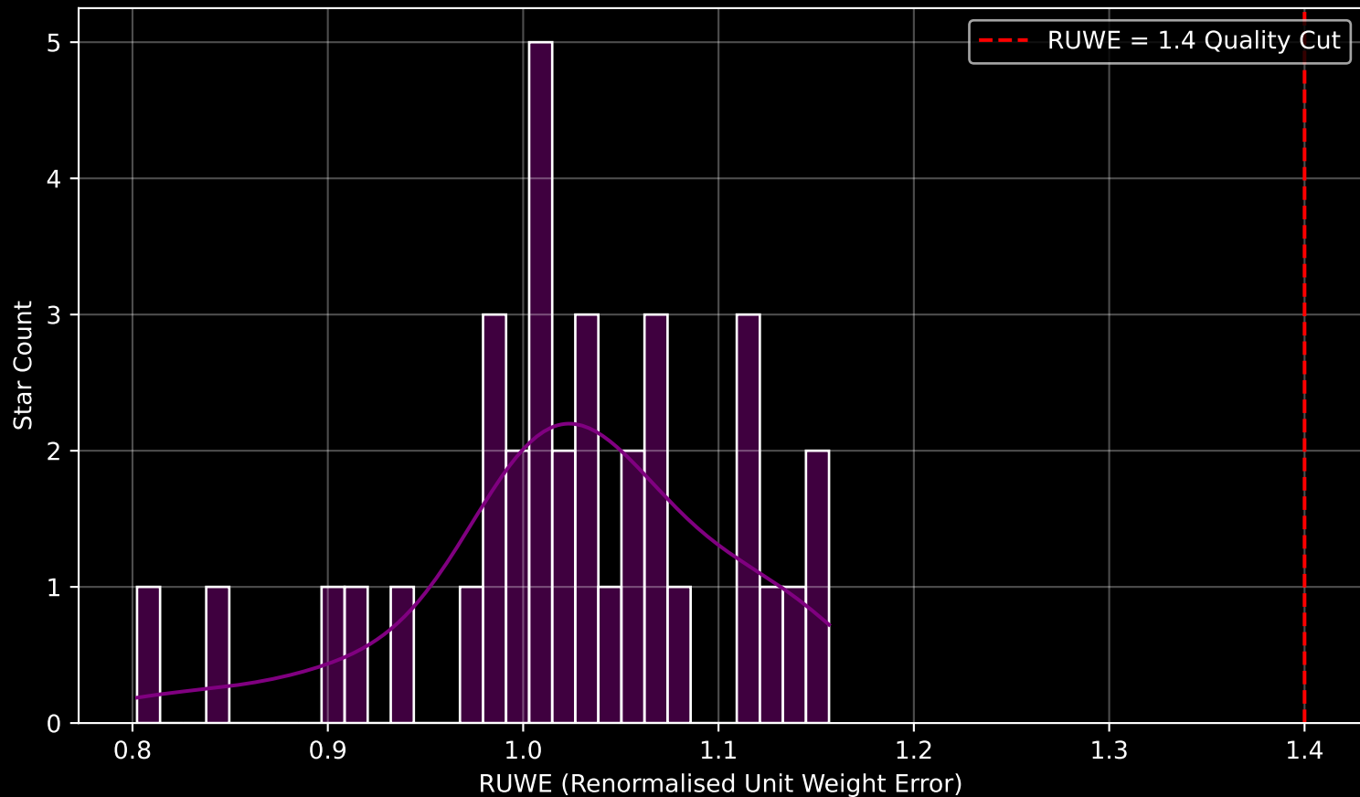
Gaia Cluster: [ASCC_66] RUWE Distribution (n= 35)
