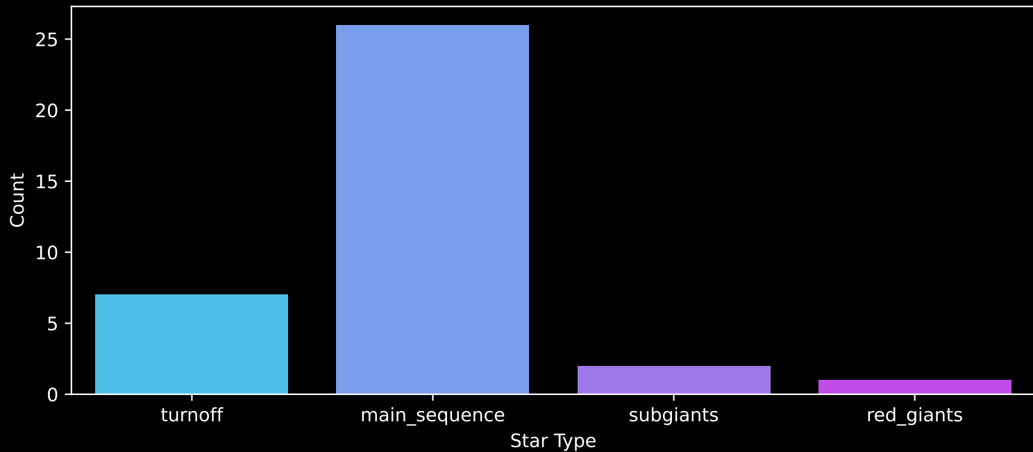
Gaia Cluster: [ASCC_66] Count plot of Star Type
