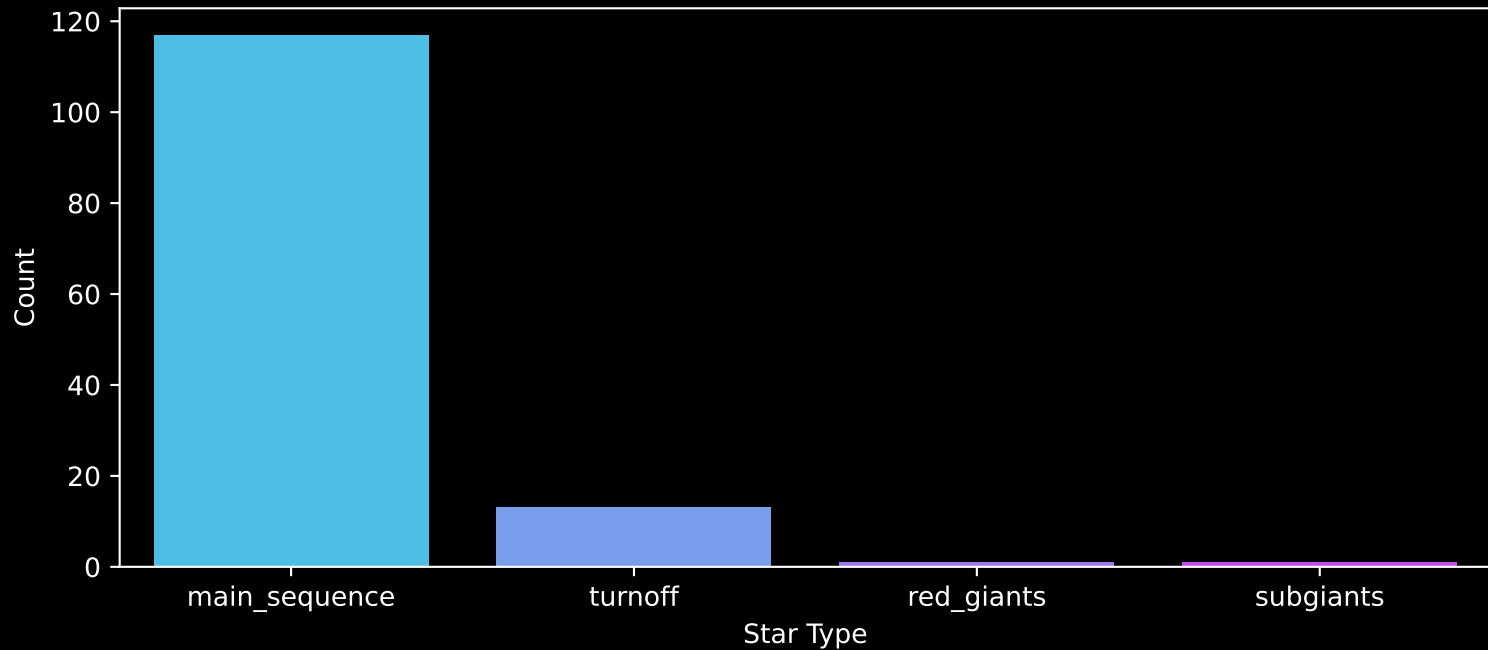
Gaia Cluster: [ASCC_73] Count plot of Star Type
