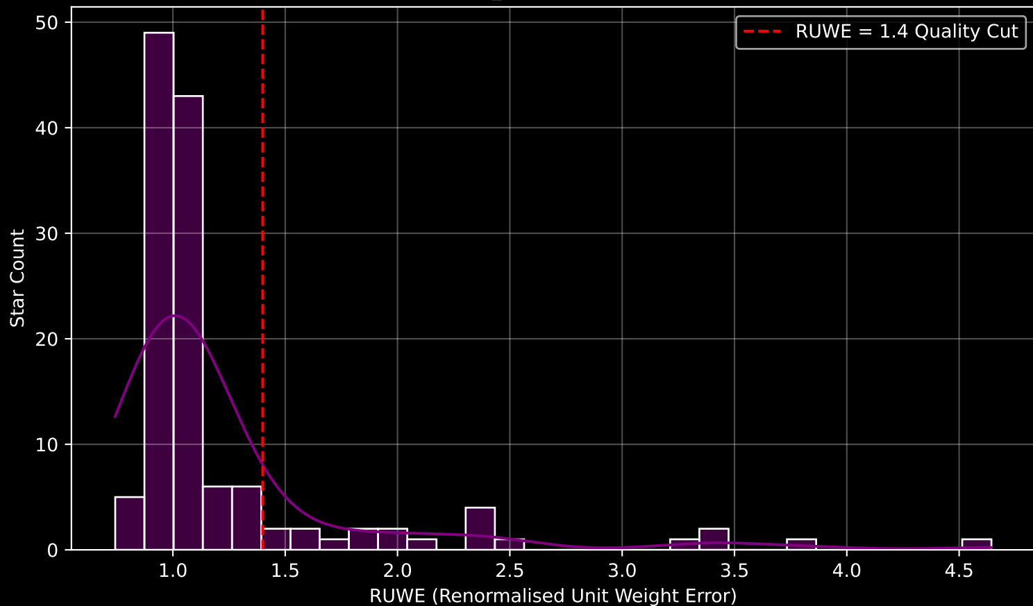
Gaia Cluster: [ASCC_73] RUWE Distribution (n= 129)
