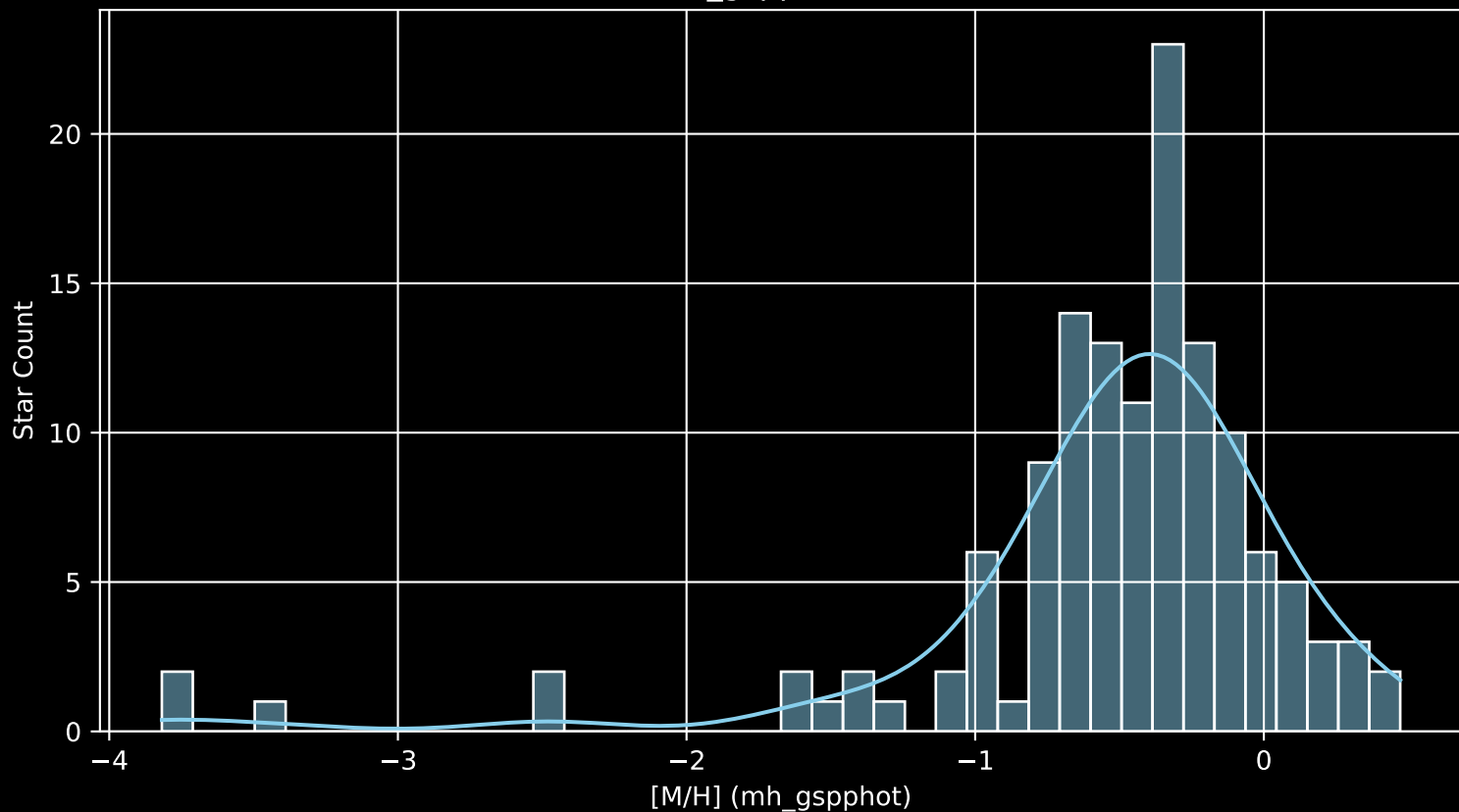
Gaia Cluster: [ASCC_73 [M/H] (mh_gspphot) (n= 132)
