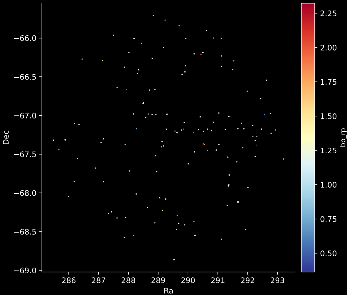
Gaia Cluster: [ASCC_73] Stars: 132
