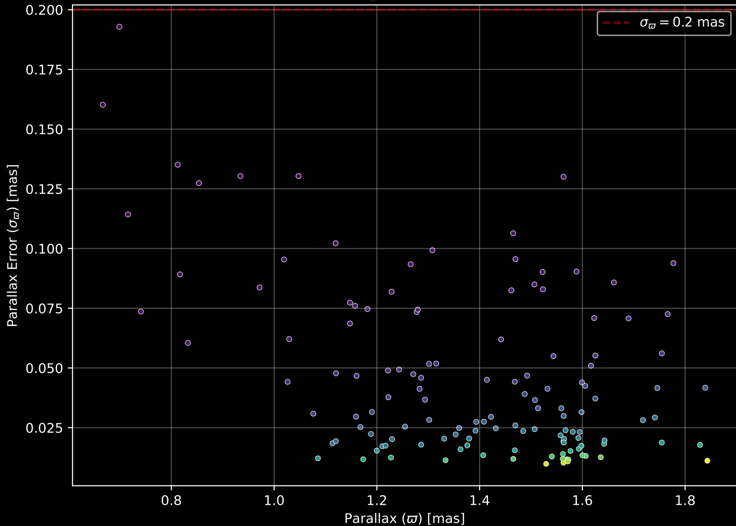
Gaia Cluster: [ASCC_73] Parallax Quality (n= 132)
