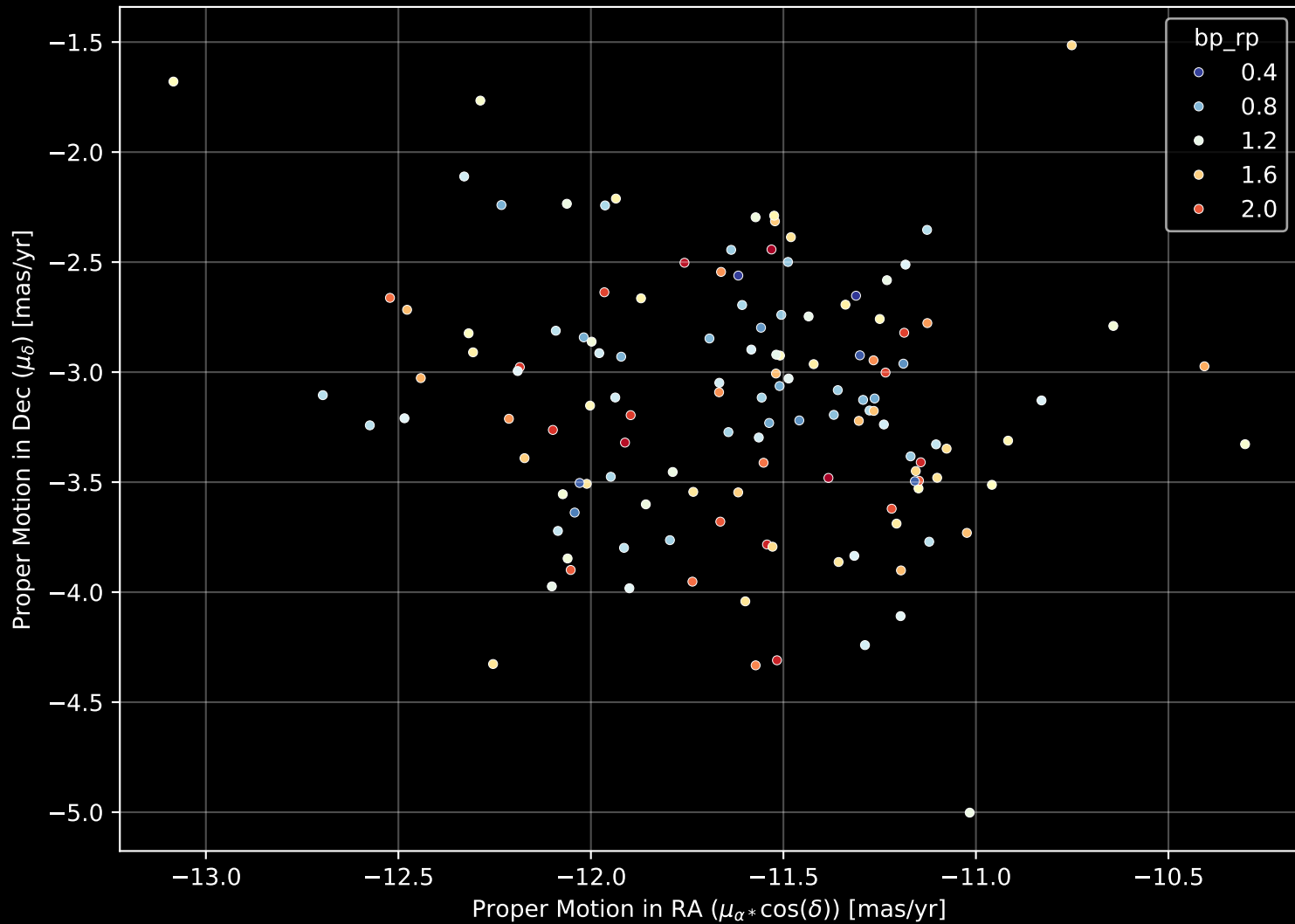
Gaia Cluster: [ASCC_73] Proper Motion Diagram (n= 132)
