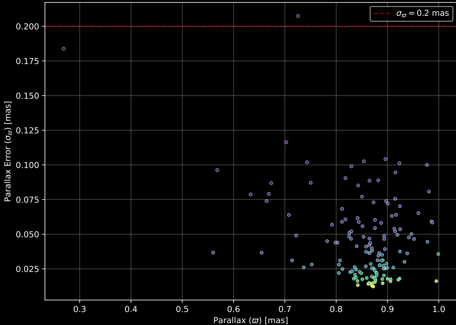
Gaia Cluster: [ASCC_77] Parallax Quality (n= 142)
