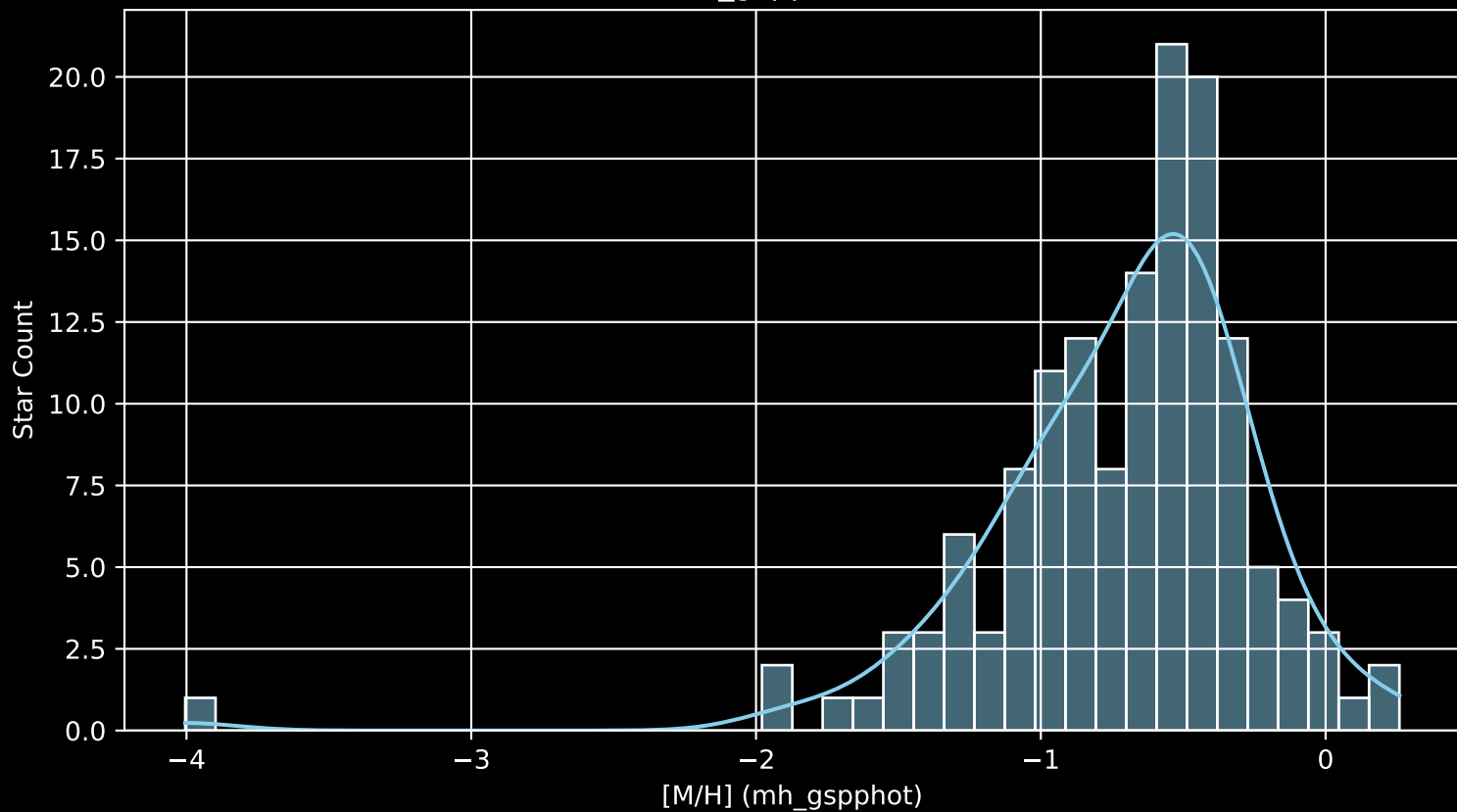
Gaia Cluster: [ASCC_77 [M/H] (mh_gspphot) (n= 141)
