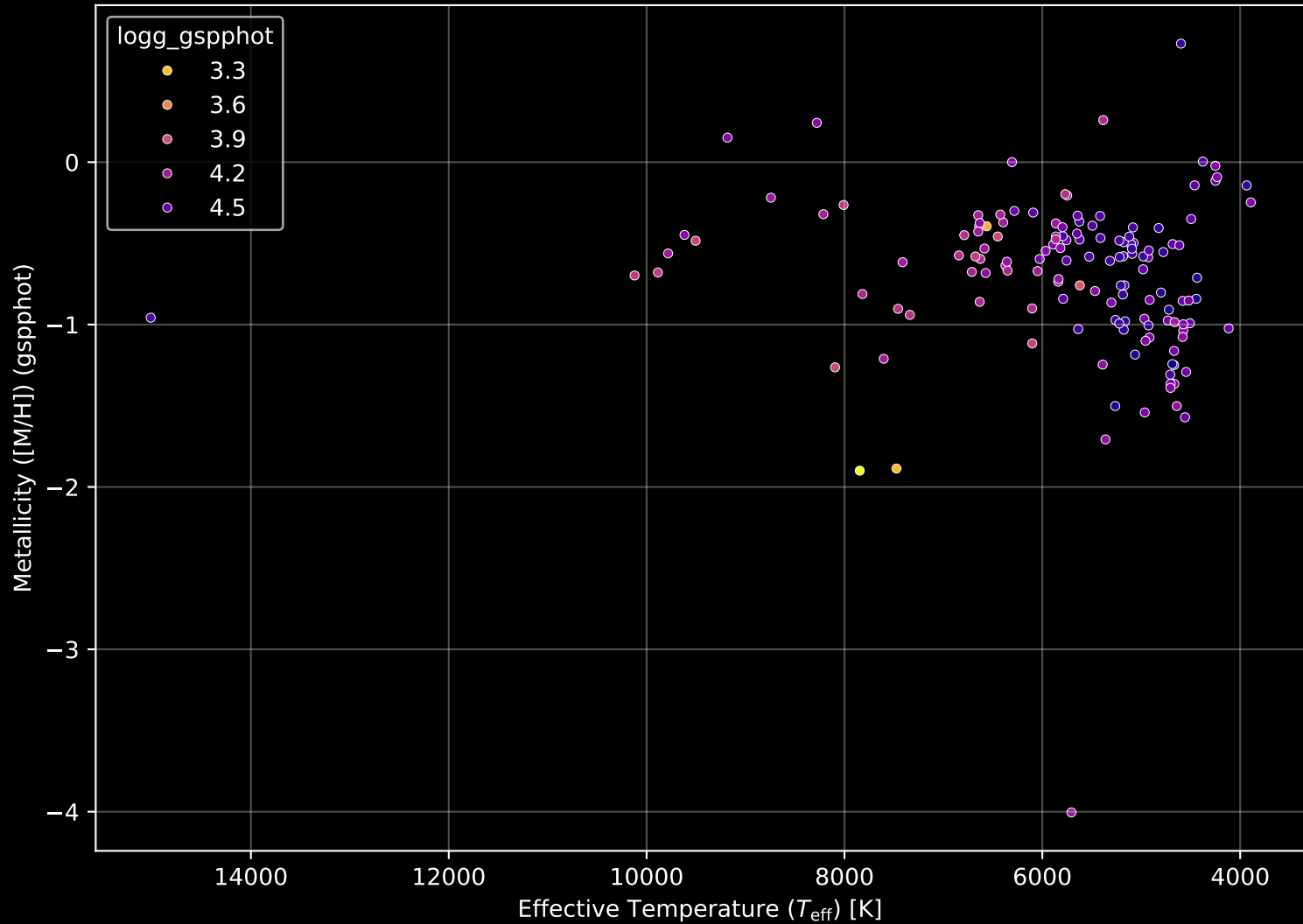
Gaia Cluster: [ASCC_77] Stellar Population Parameters (n= 142)
