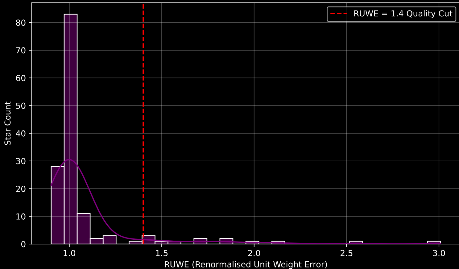
Gaia Cluster: [ASCC_77] RUWE Distribution (n= 141)
