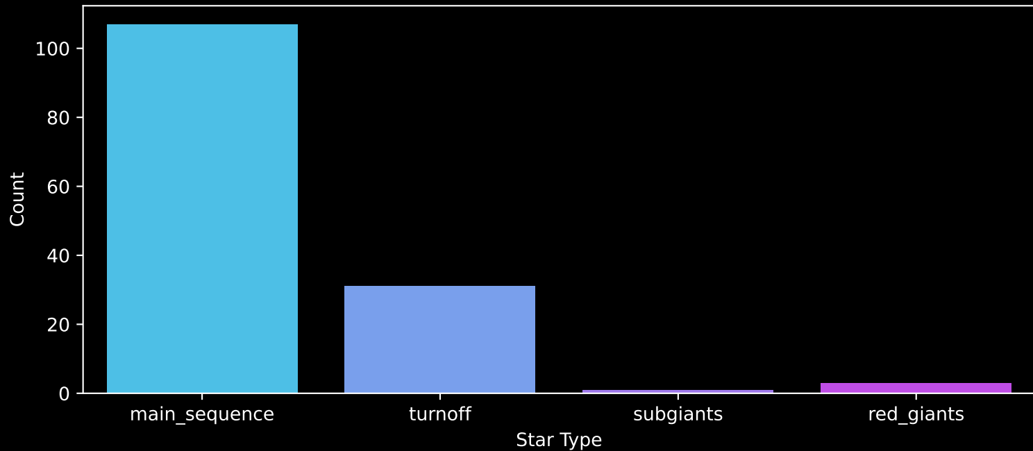
Gaia Cluster: [ASCC_77] Count plot of Star Type
