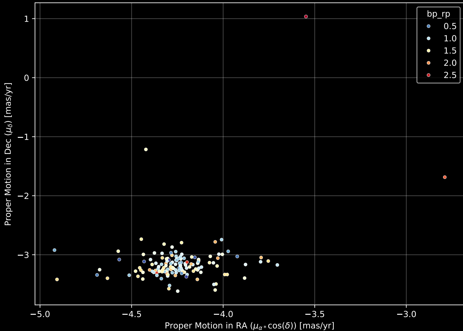
Gaia Cluster: [ASCC_77] Proper Motion Diagram (n= 142)
