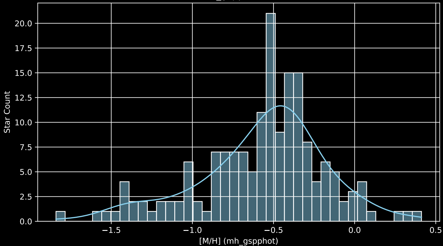
Gaia Cluster: [ASCC_85 [M/H] (mh_gspphot) (n= 168)
