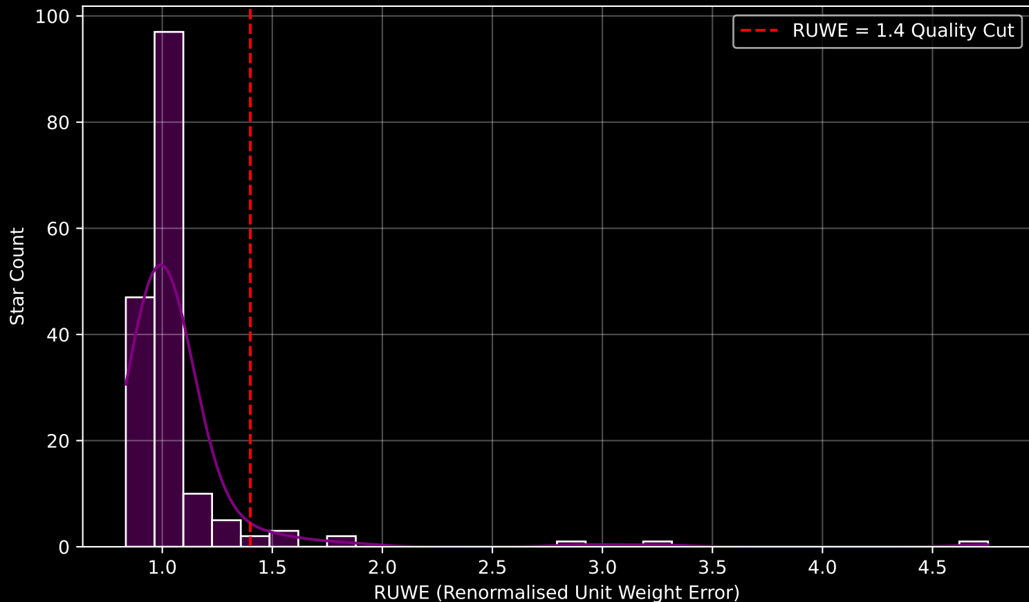
Gaia Cluster: [ASCC_85] RUWE Distribution (n= 169)
