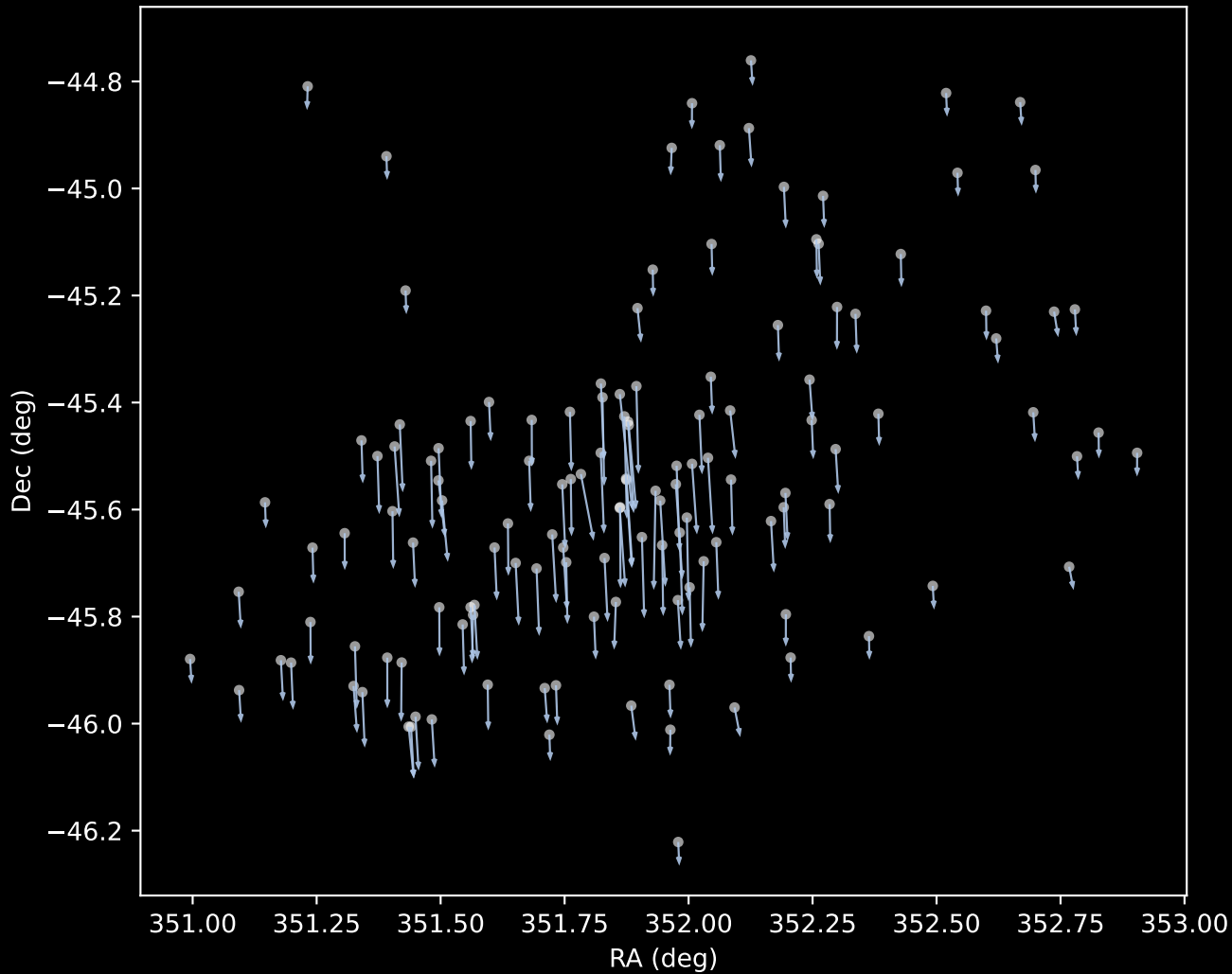
Gaia DR3 Cluster 1 Proper Motion Vectors (n=134)
