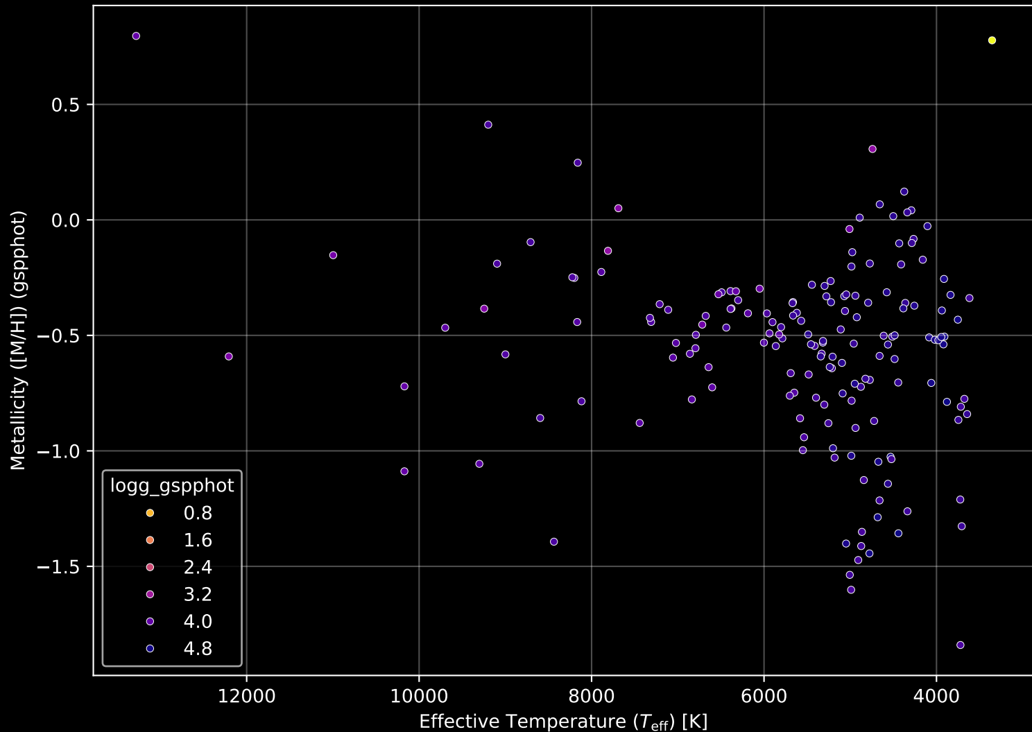
Gaia Cluster: [ASCC_85] Stellar Population Parameters (n= 170)
