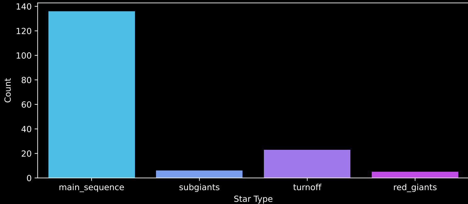
Gaia Cluster: [ASCC_85] Count plot of Star Type
