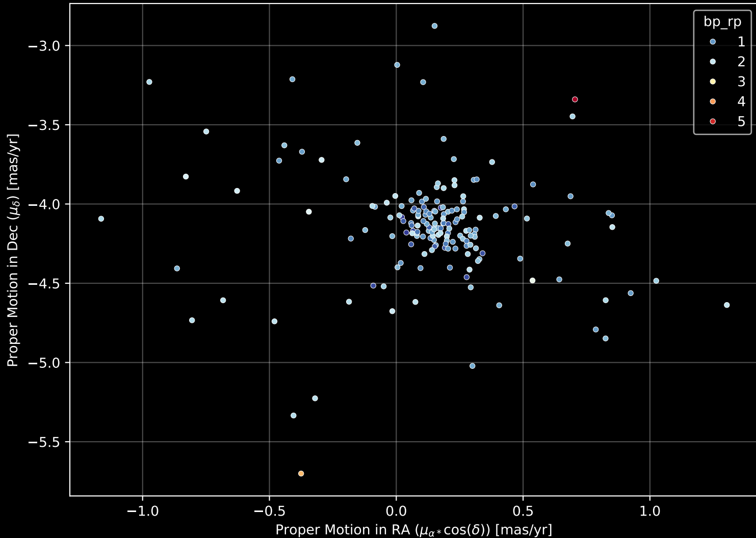
Gaia Cluster: [ASCC_85] Proper Motion Diagram (n= 170)
