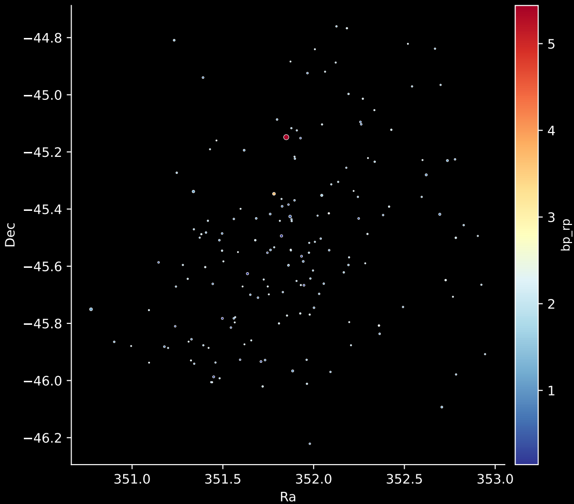
Gaia Cluster: [ASCC_85] Stars: 170
