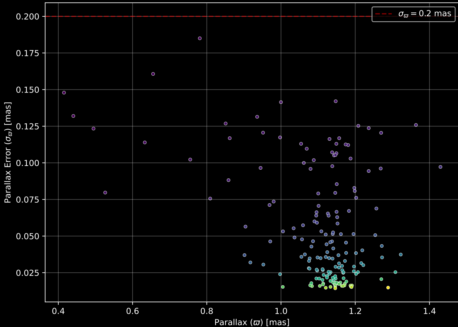
Gaia Cluster: [ASCC_85] Parallax Quality (n= 170)
