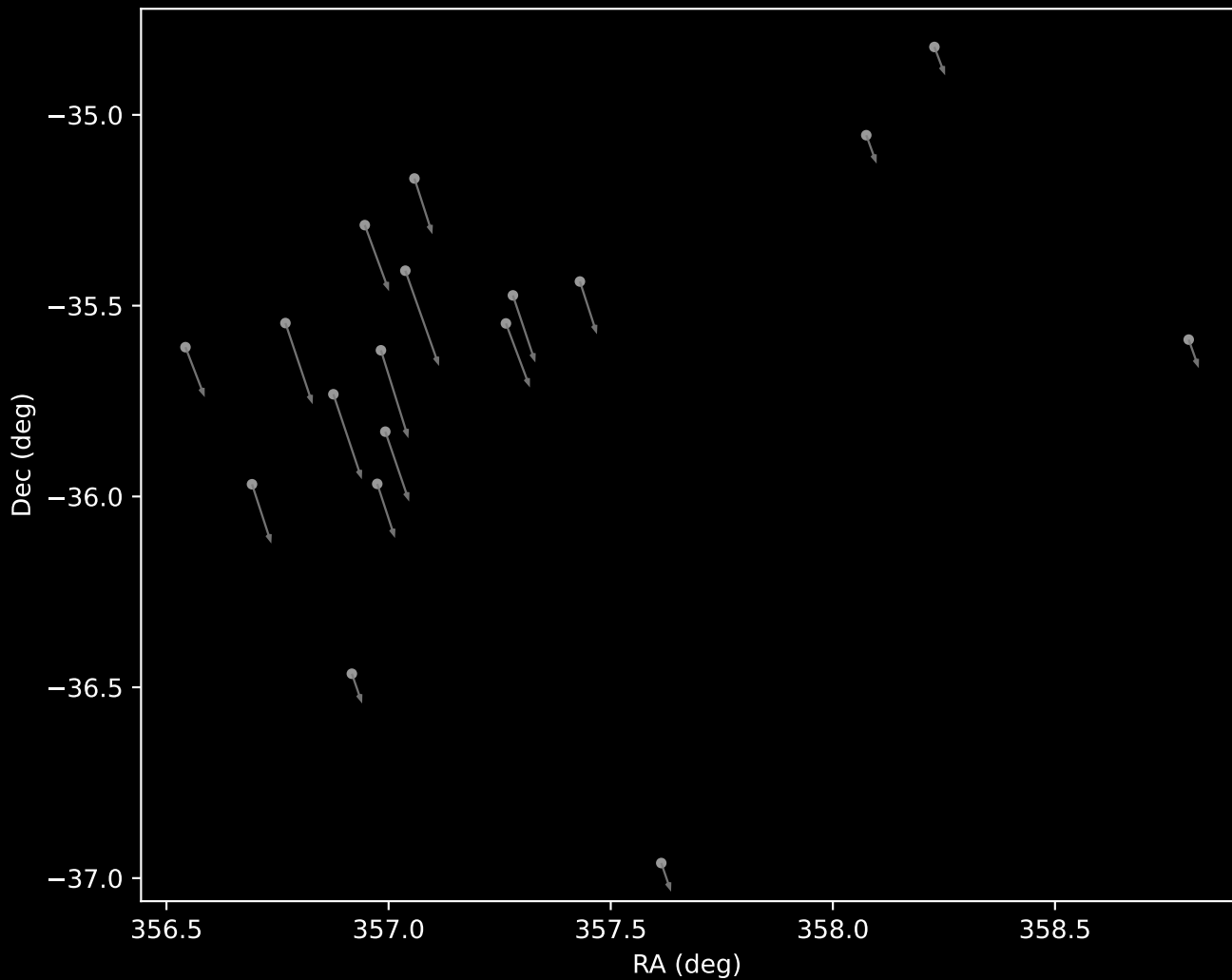
Gaia DR3 Cluster 14 Proper Motion Vectors (n=18)
