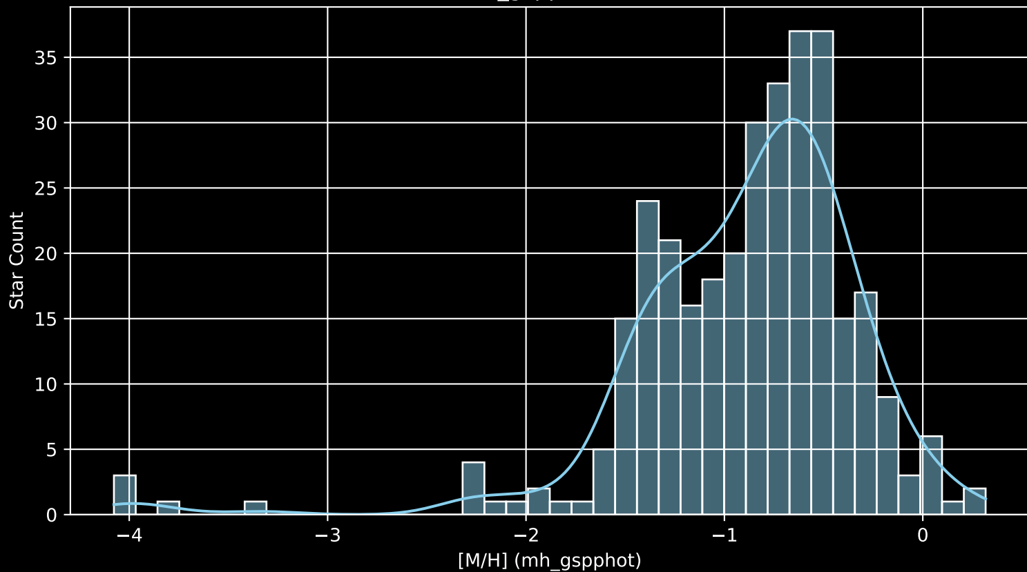
Gaia Cluster: [ASCC_88 [M/H] (mh_gspphot) (n= 324)
