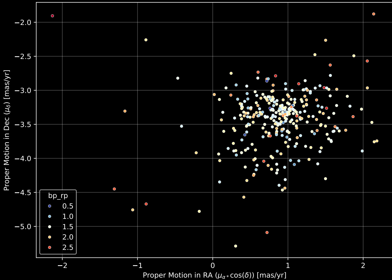
Gaia Cluster: [ASCC_88] Proper Motion Diagram (n= 324)
