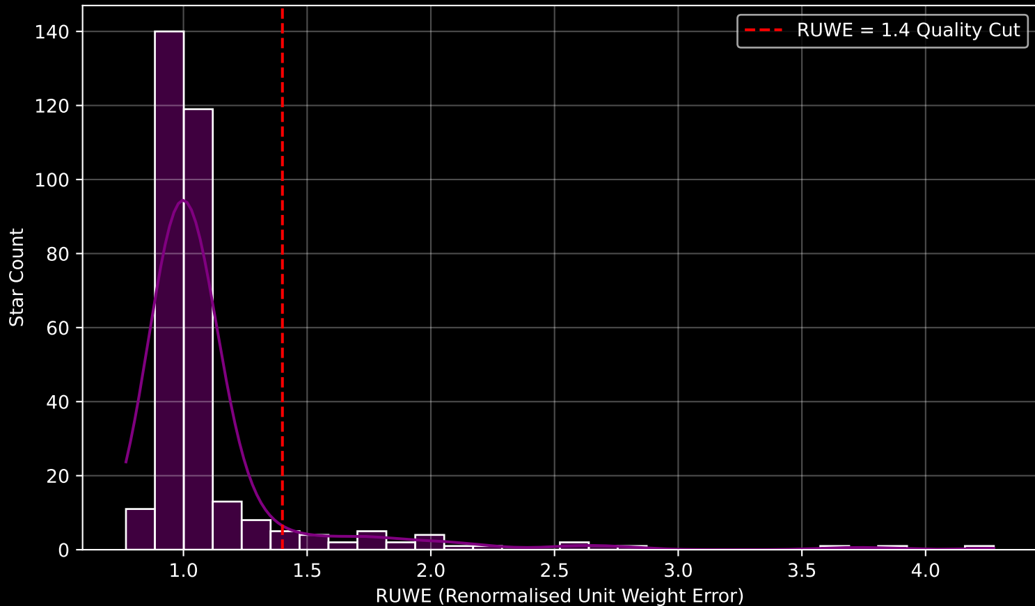
Gaia Cluster: [ASCC_88] RUWE Distribution (n= 322)
