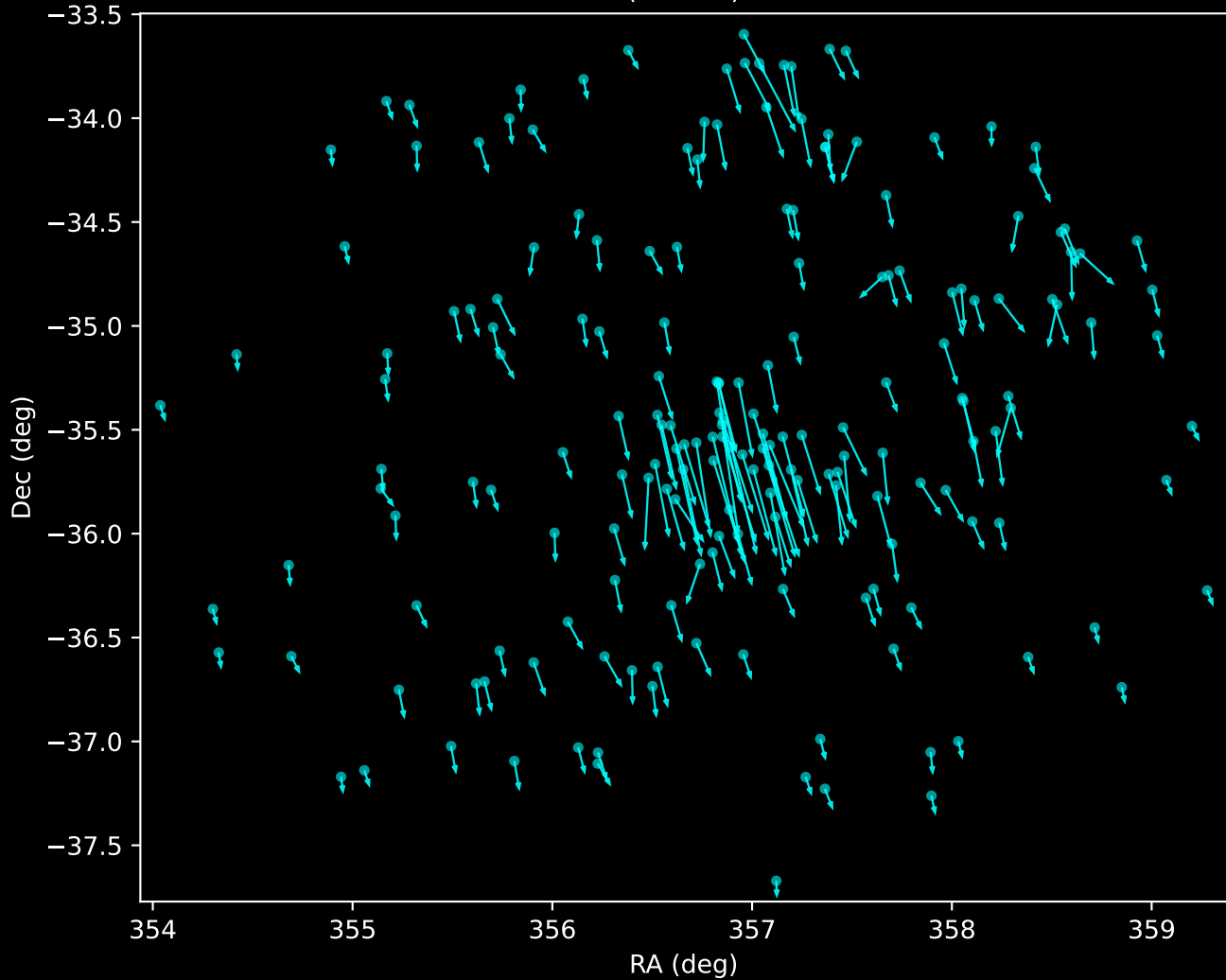
Gaia DR3 Noise Stream Proper Motion Vectors (n=189)
