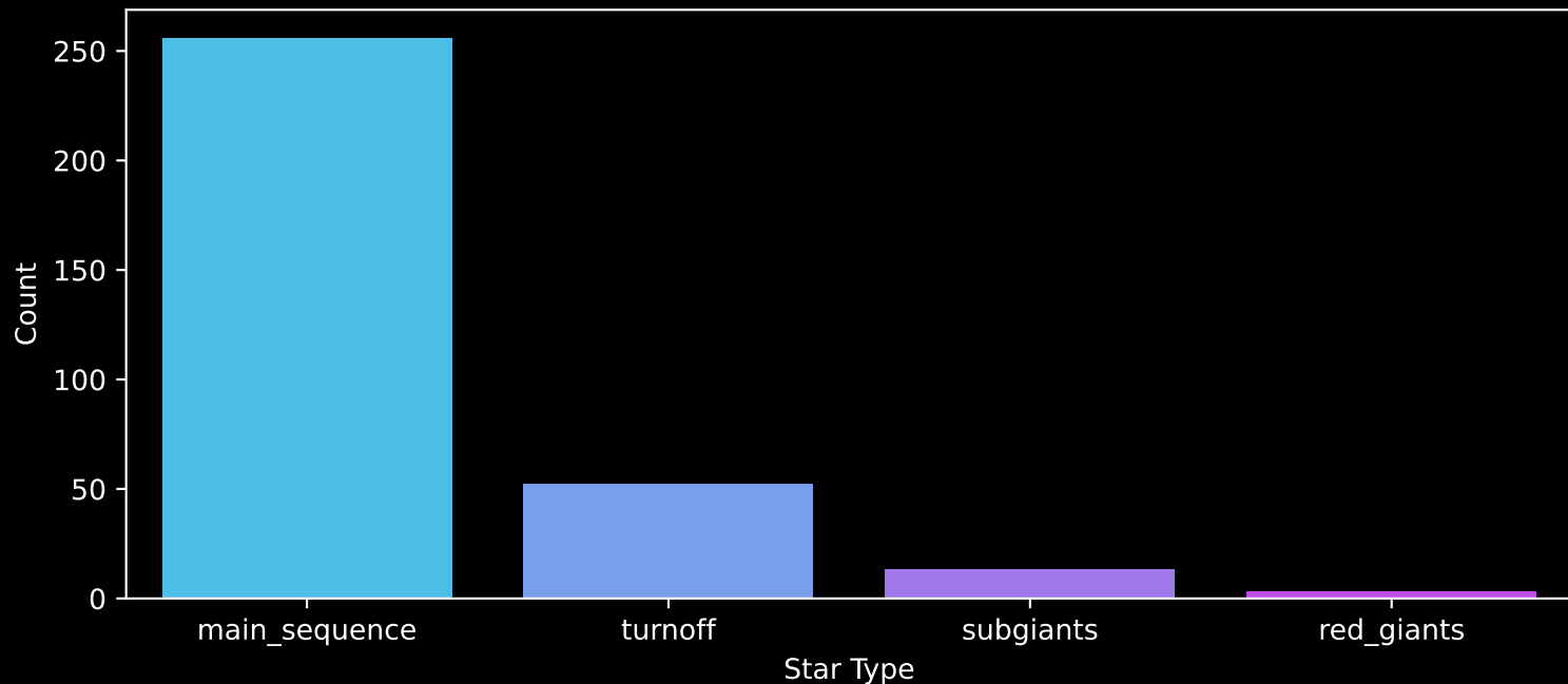
Gaia Cluster: [ASCC_88] Count plot of Star Type
