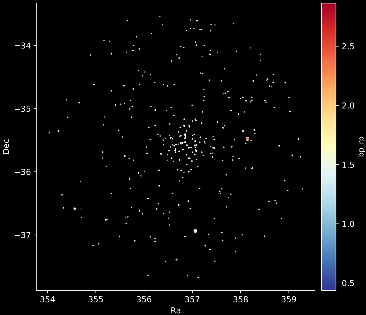
Gaia Cluster: [ASCC_88] Stars: 324
