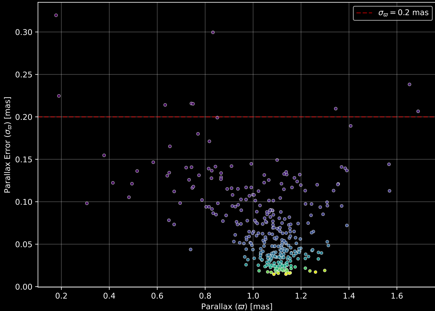
Gaia Cluster: [ASCC_88] Parallax Quality (n= 324)
