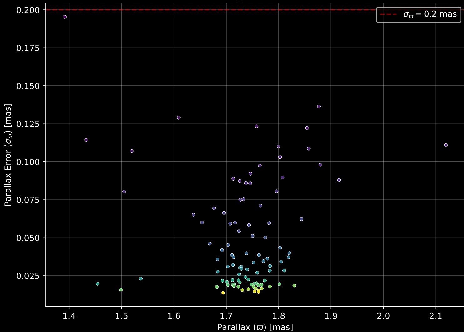
Gaia Cluster: [ASCC_97] Parallax Quality (n= 98)
