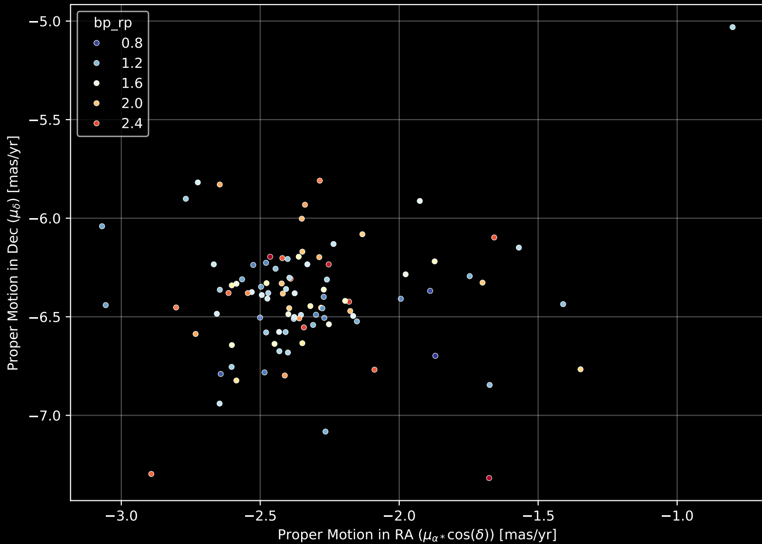
Gaia Cluster: [ASCC_97] Proper Motion Diagram (n= 98)
