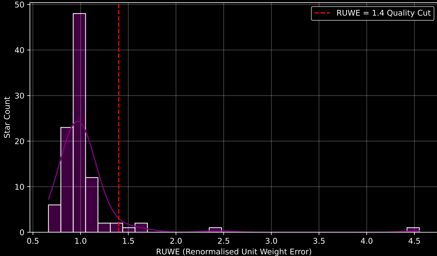
Gaia Cluster: [ASCC_97] RUWE Distribution (n= 98)
