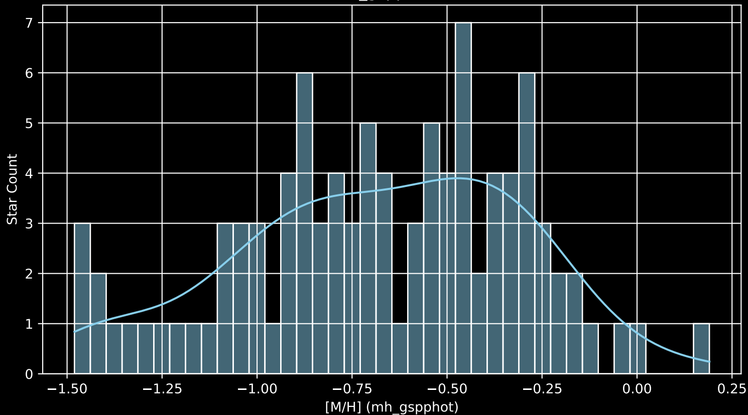
Gaia Cluster: [ASCC_97 [M/H] (mh_gspphot) (n= 98)
