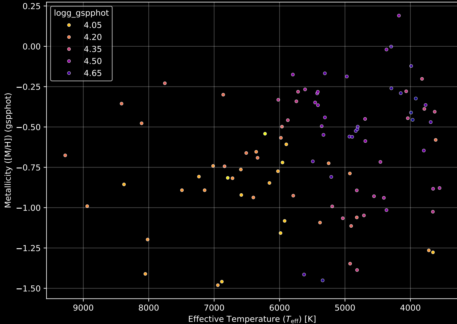
Gaia Cluster: [ASCC_97] Stellar Population Parameters (n= 98)
