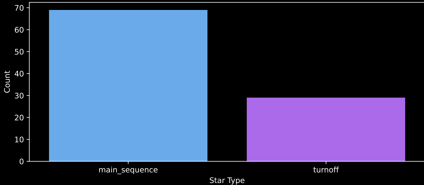
Gaia Cluster: [ASCC_97] Count plot of Star Type
