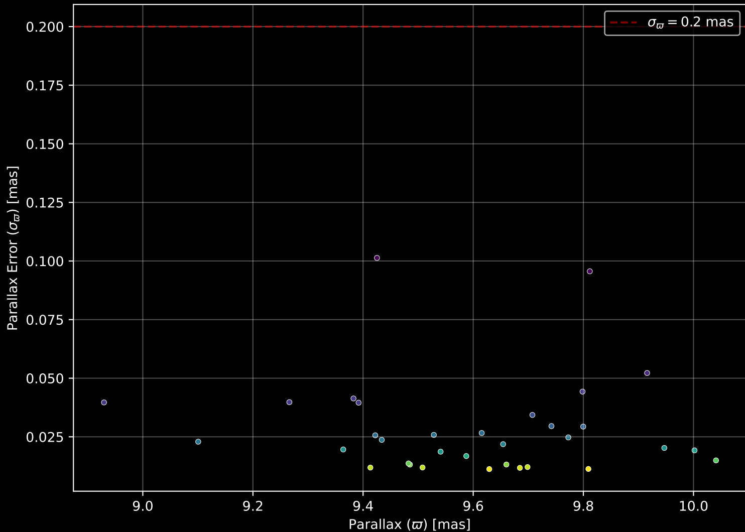
Gaia Cluster: [Alessi_13] Parallax Quality (n= 33)
