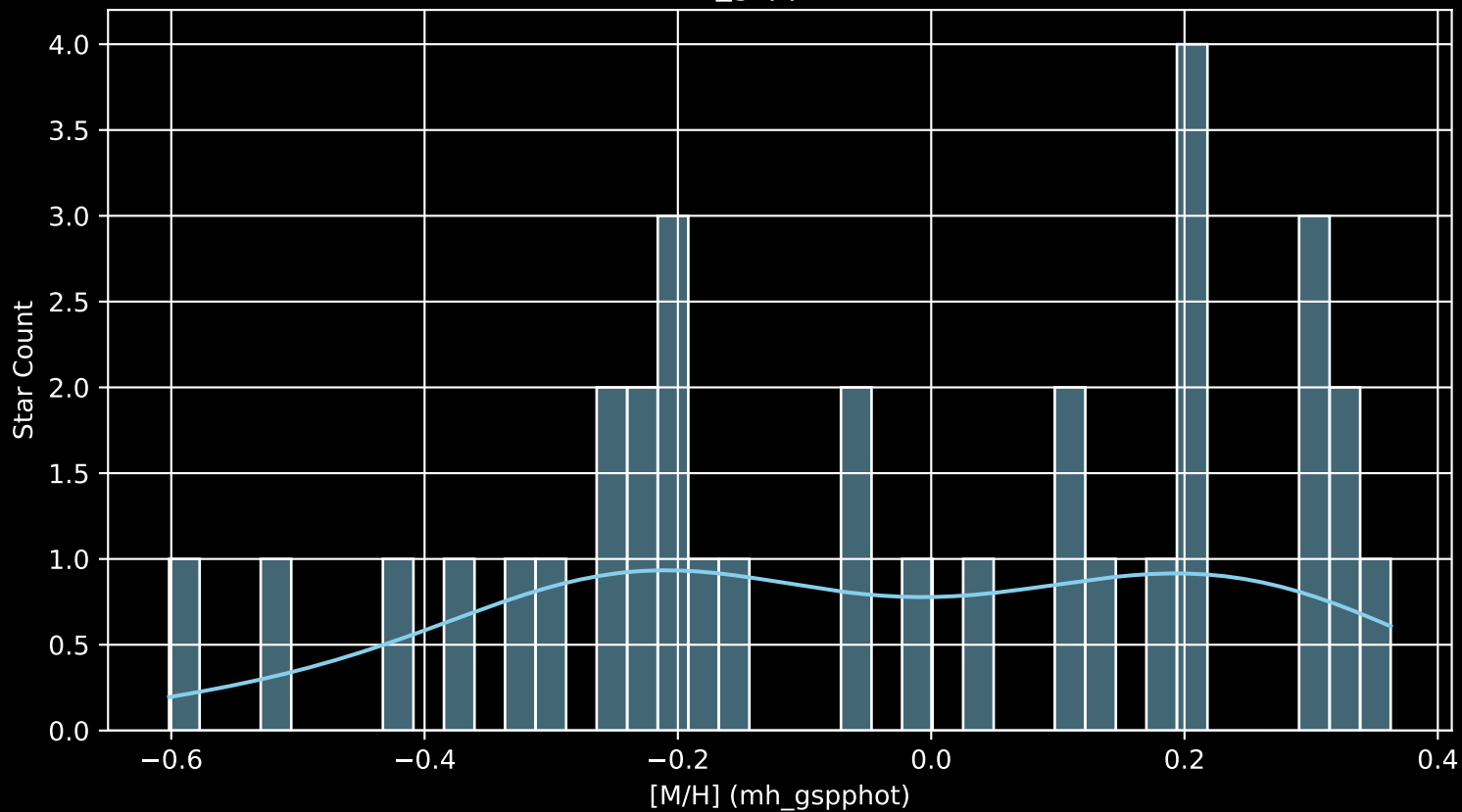
Gaia Cluster: [Alessi_13 [M/H] (mh_gspphot) (n= 33)
