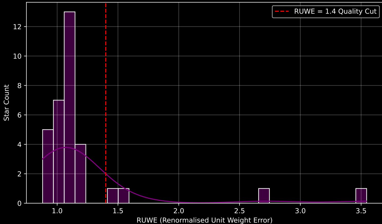
Gaia Cluster: [Alessi_13] RUWE Distribution (n= 33)
