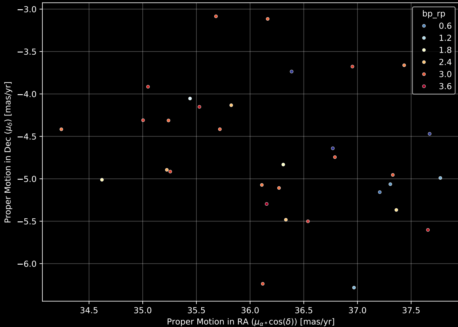
Gaia Cluster: [Alessi_13] Proper Motion Diagram (n= 33)
