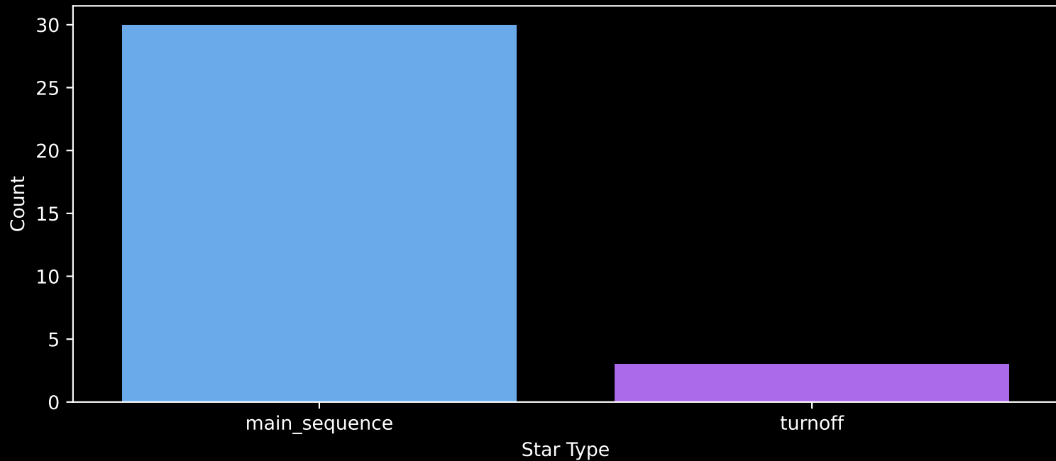
Gaia Cluster: [Alessi_13] Count plot of Star Type
