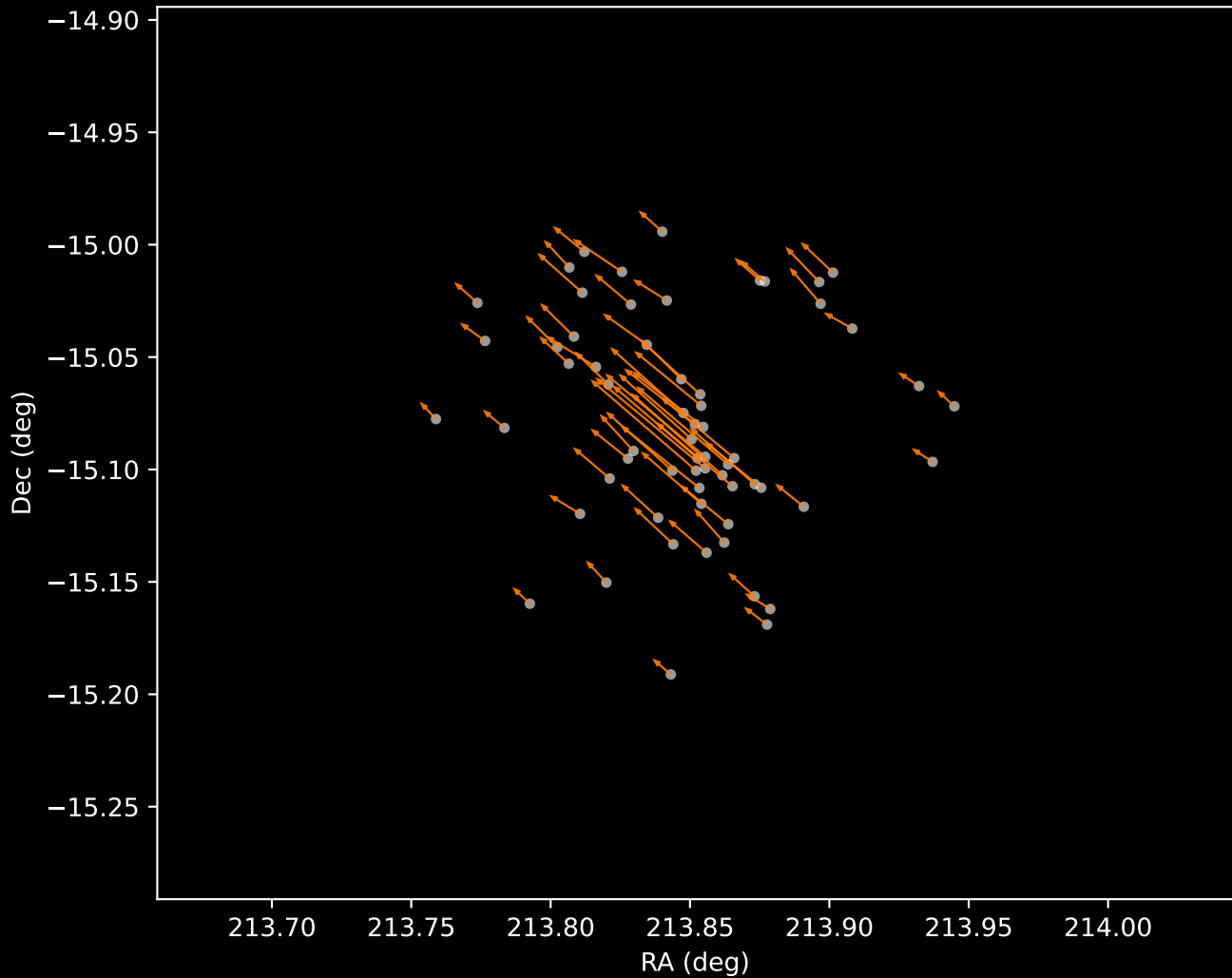
Gaia DR3 Cluster 2 Proper Motion Vectors (n=62)
