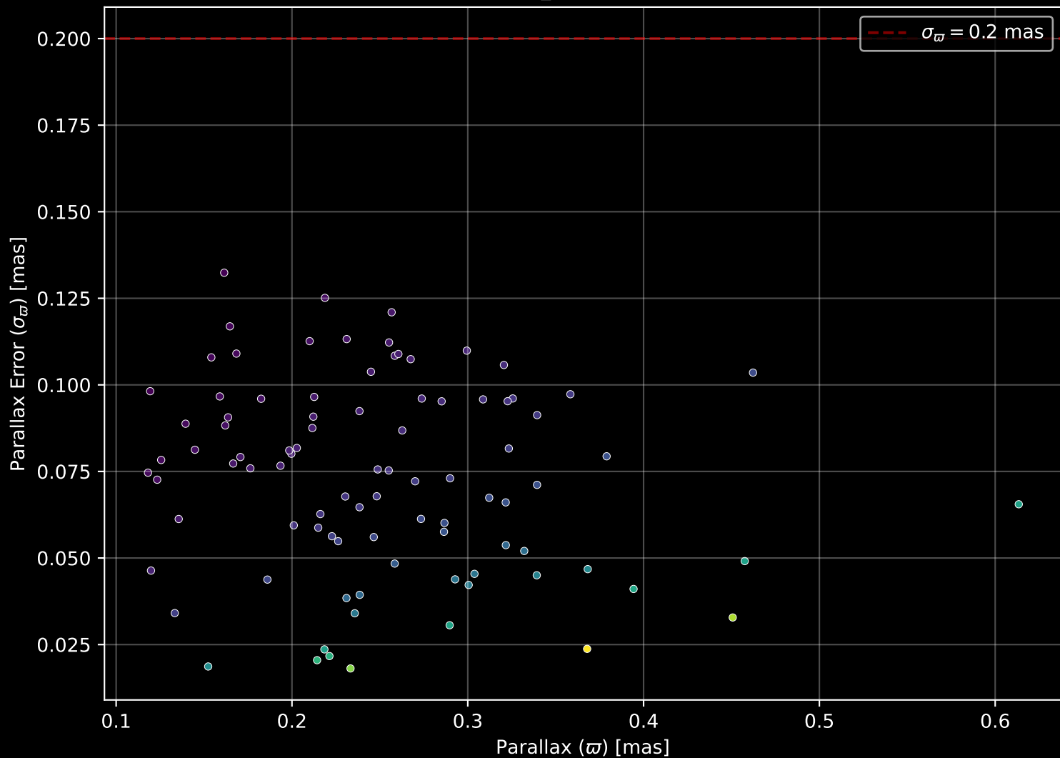
Gaia Cluster: [Alessi_17] Parallax Quality (n= 92)
