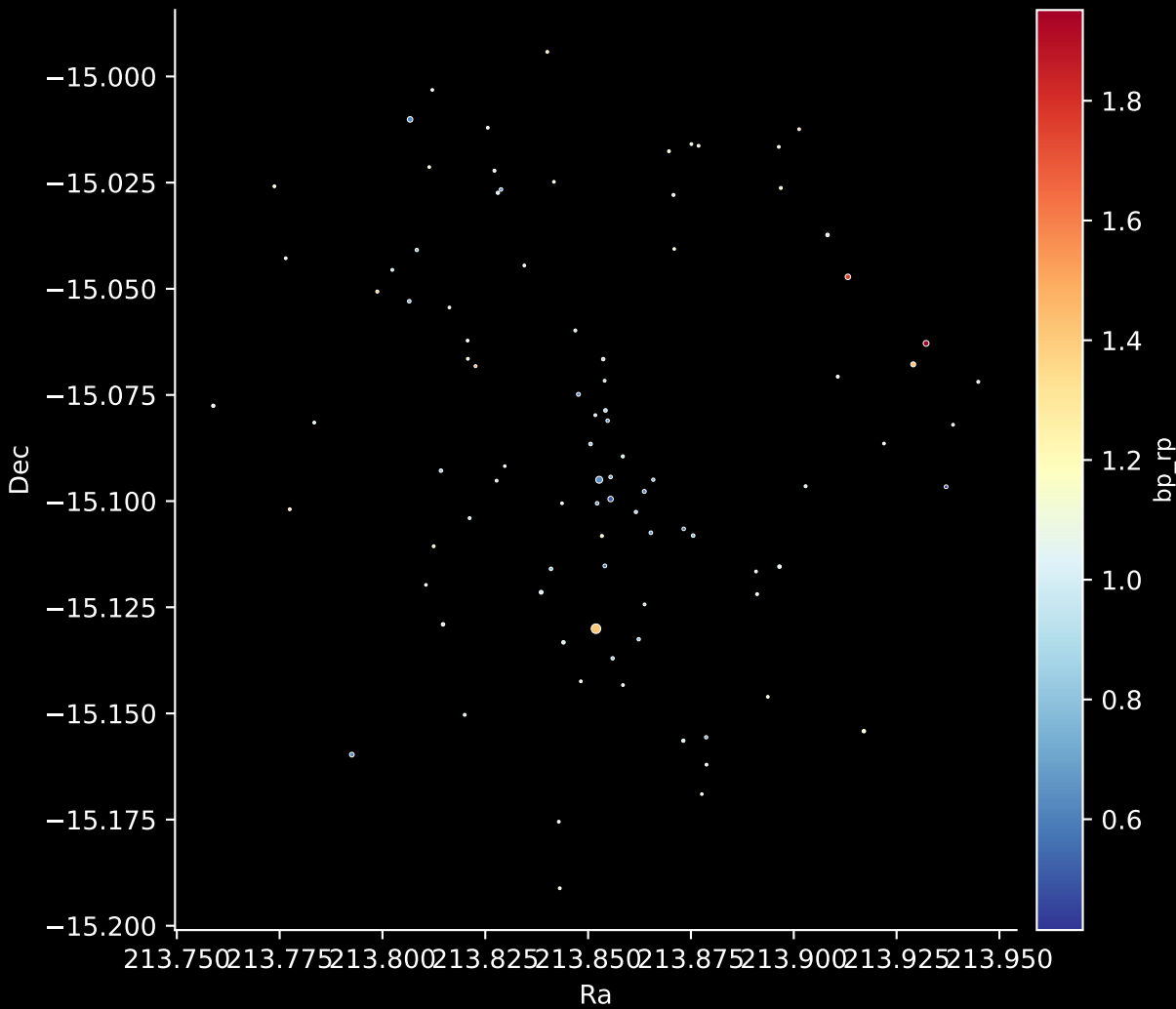
Gaia Cluster: [Alessi_17] Stars: 92
