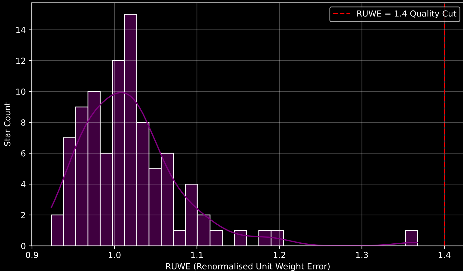
Gaia Cluster: [Alessi_17] RUWE Distribution (n= 92)
