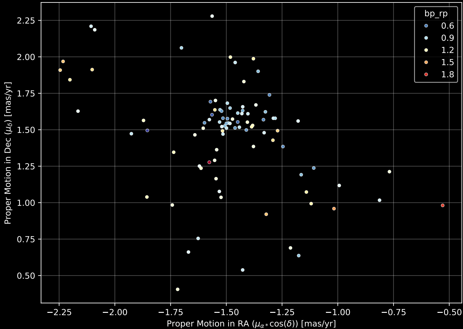
Gaia Cluster: [Alessi_17] Proper Motion Diagram (n= 92)
