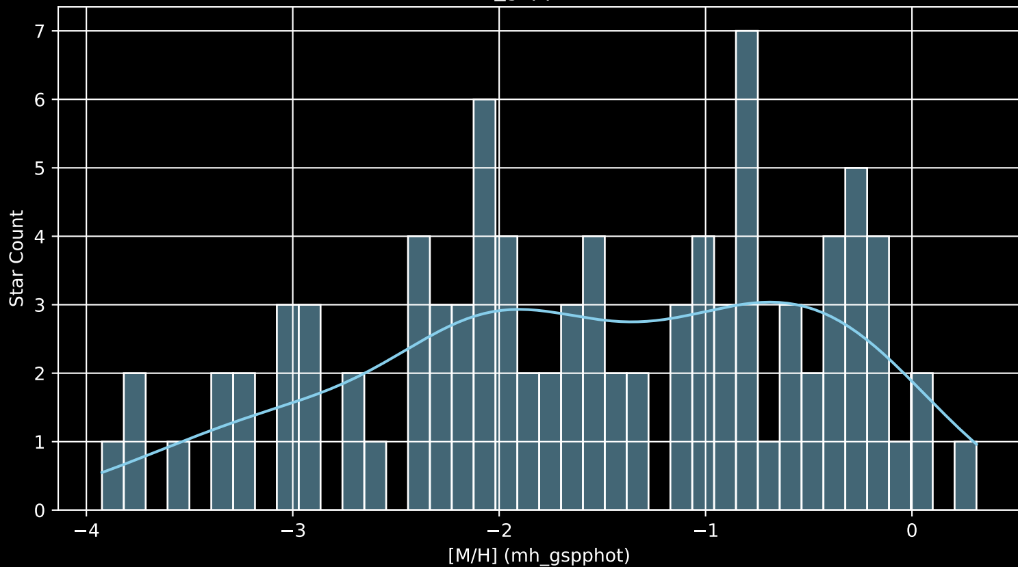
Gaia Cluster: [Alessi_17 [M/H] (mh_gspphot) (n= 92)
