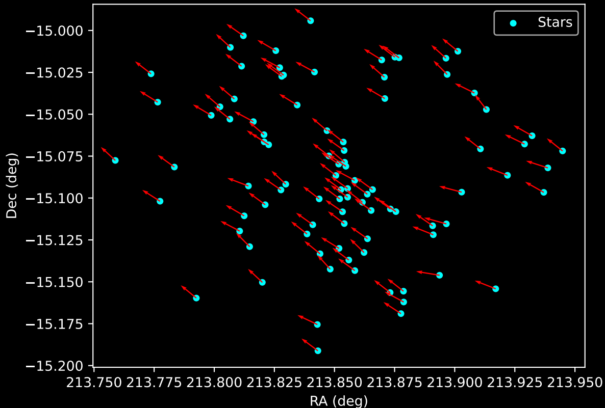
Gaia Cluster: [Alessi_17] Proper Motion Vectors for Gaia Star Field (n= 92)
