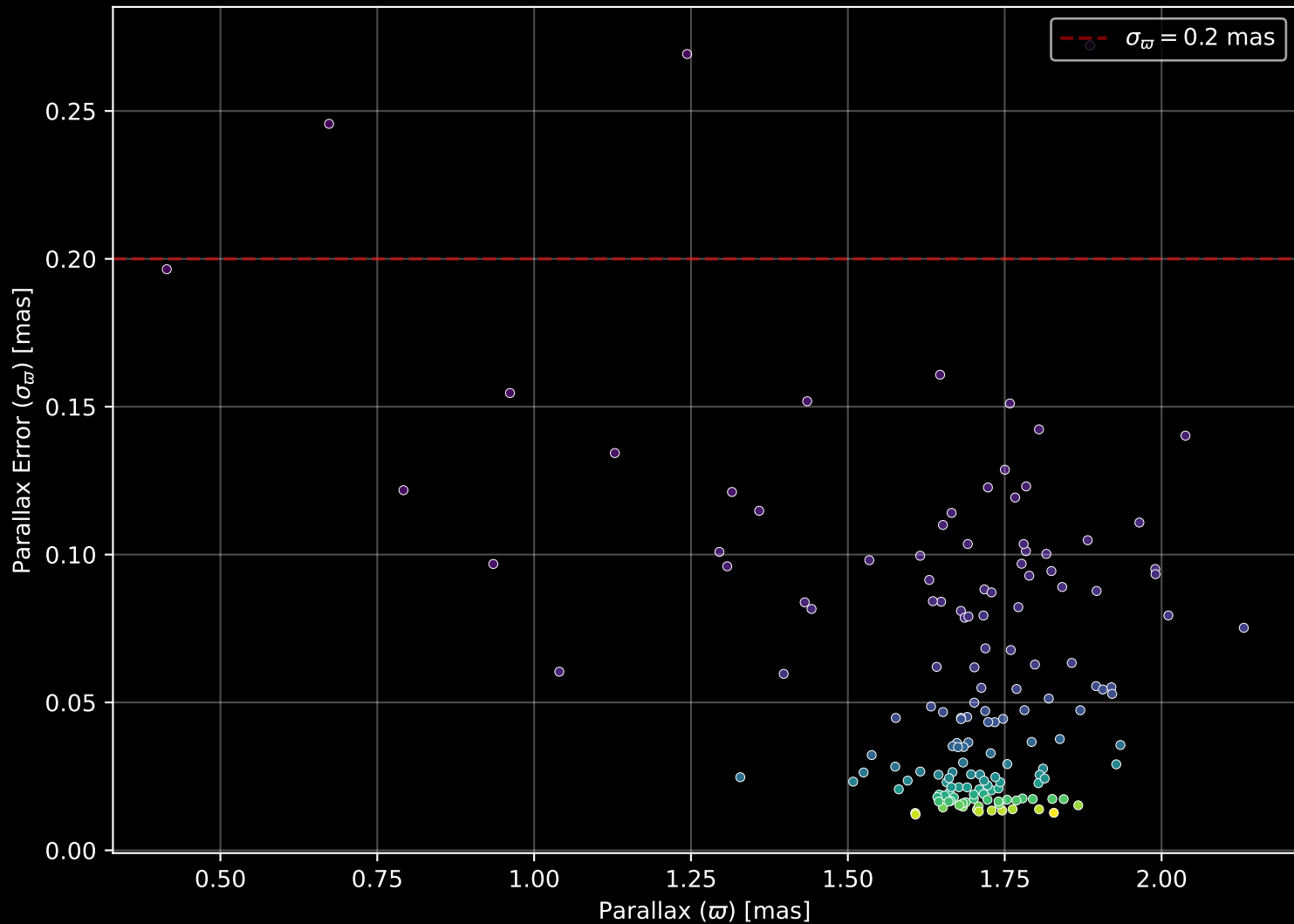
Gaia Cluster: [Alessi_19] Parallax Quality (n= 156)
