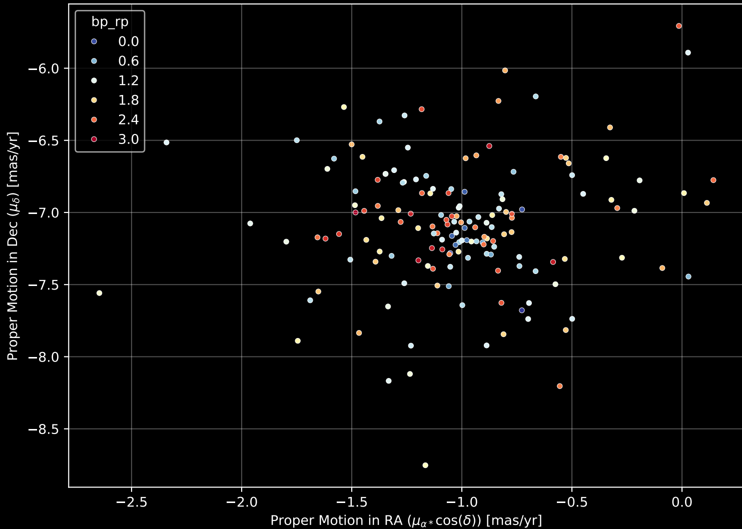
Gaia Cluster: [Alessi_19] Proper Motion Diagram (n= 156)
