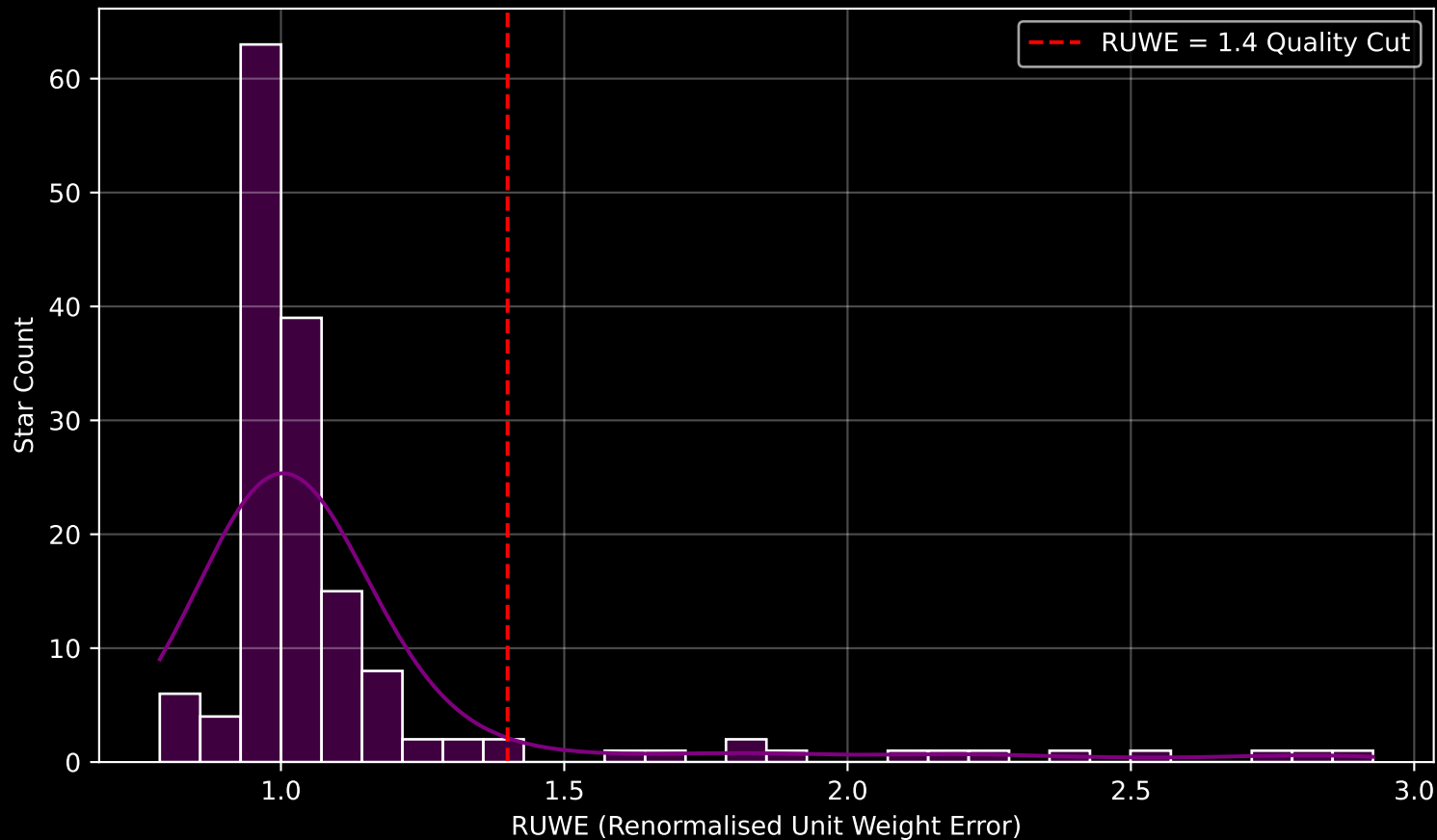
Gaia Cluster: [Alessi_19] RUWE Distribution (n= 154)
