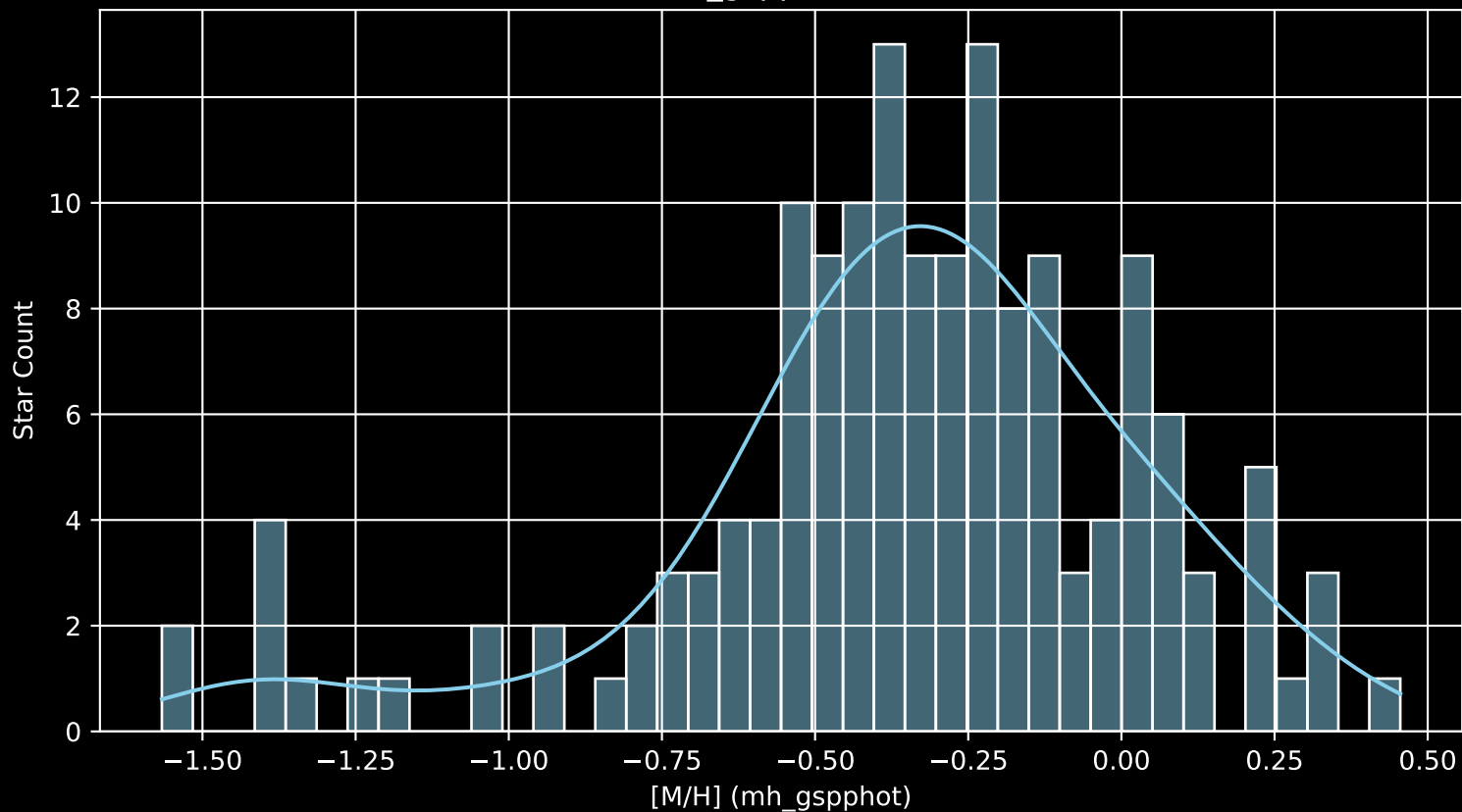
Gaia Cluster: [Alessi_19 [M/H] (mh_gspphot) (n= 155)
