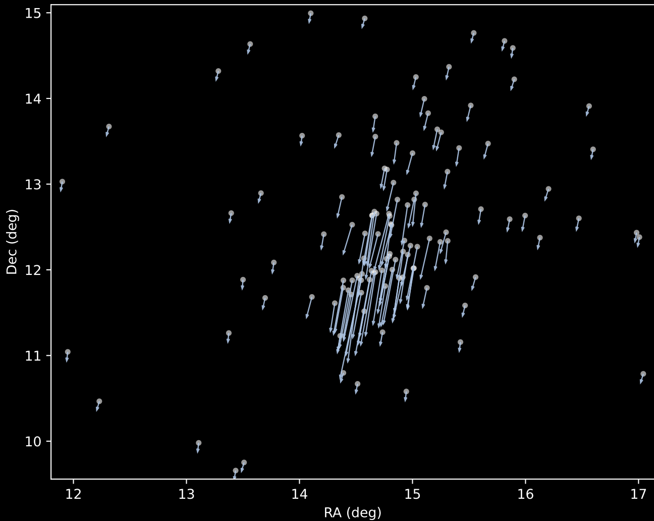
Gaia DR3 Cluster 1 Proper Motion Vectors (n=116)
