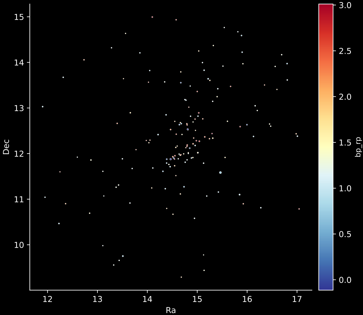
Gaia Cluster: [Alessi_19] Stars: 156
