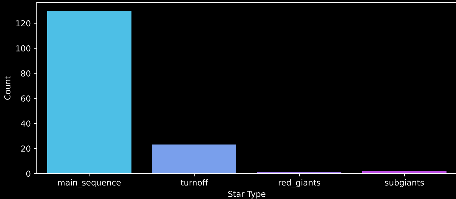
Gaia Cluster: [Alessi_19] Count plot of Star Type
