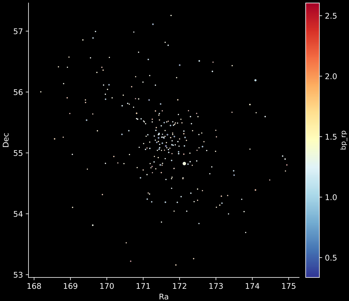
Gaia Cluster: [Alessi_2] Stars: 247
