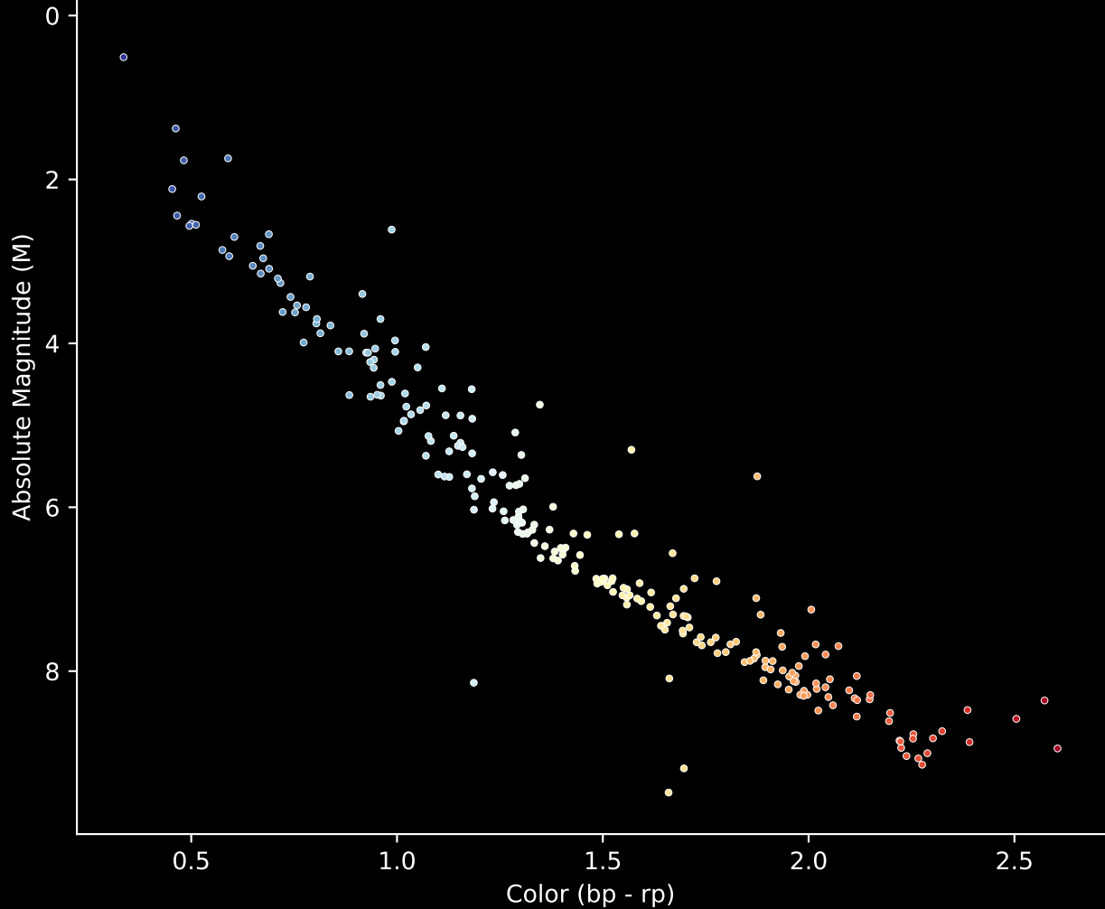
Gaia Cluster: [Alessi_2] Stars (n= 247) Hertzsprung-Russel Diagram
