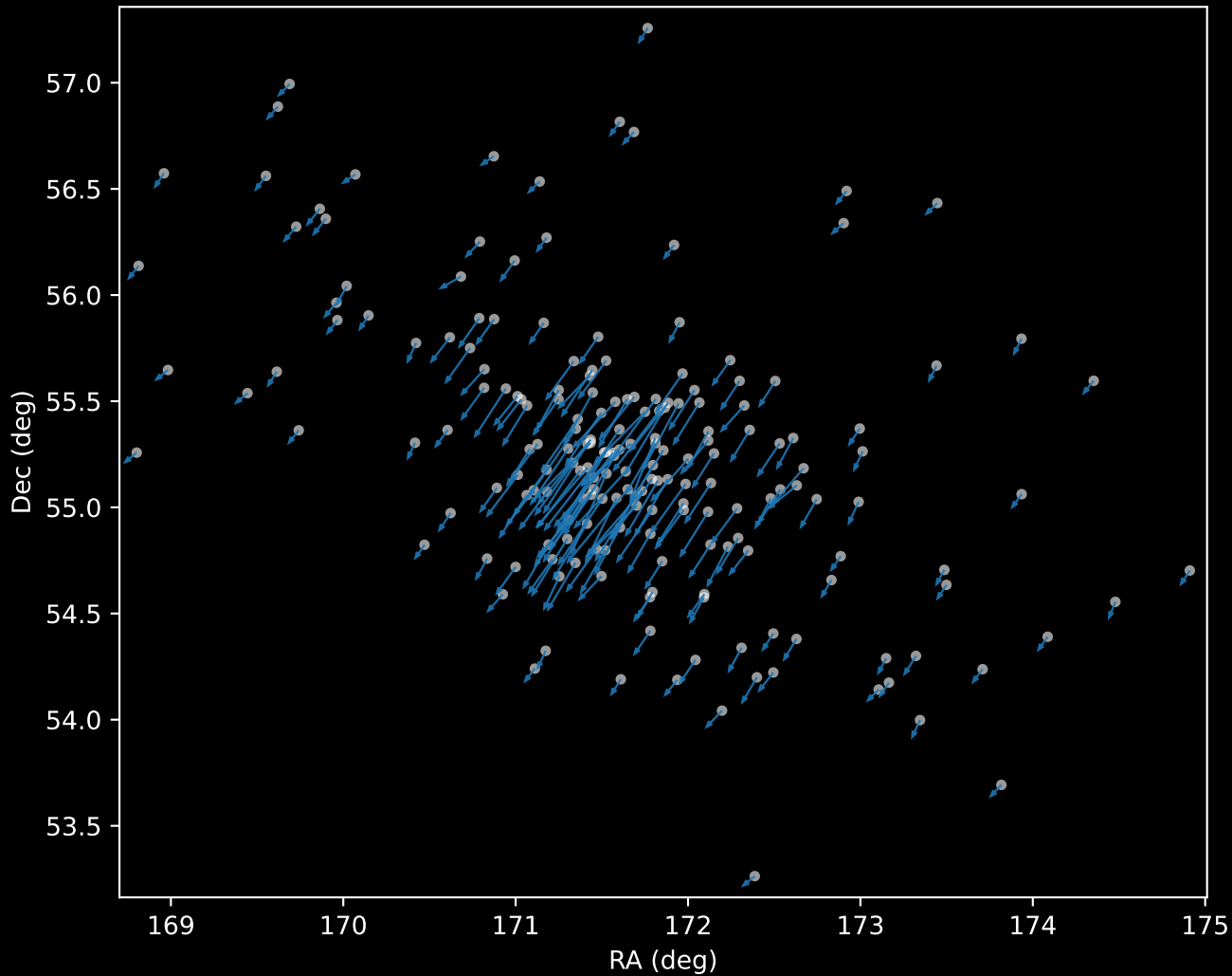
Gaia DR3 Cluster 0 Proper Motion Vectors (n=193)
