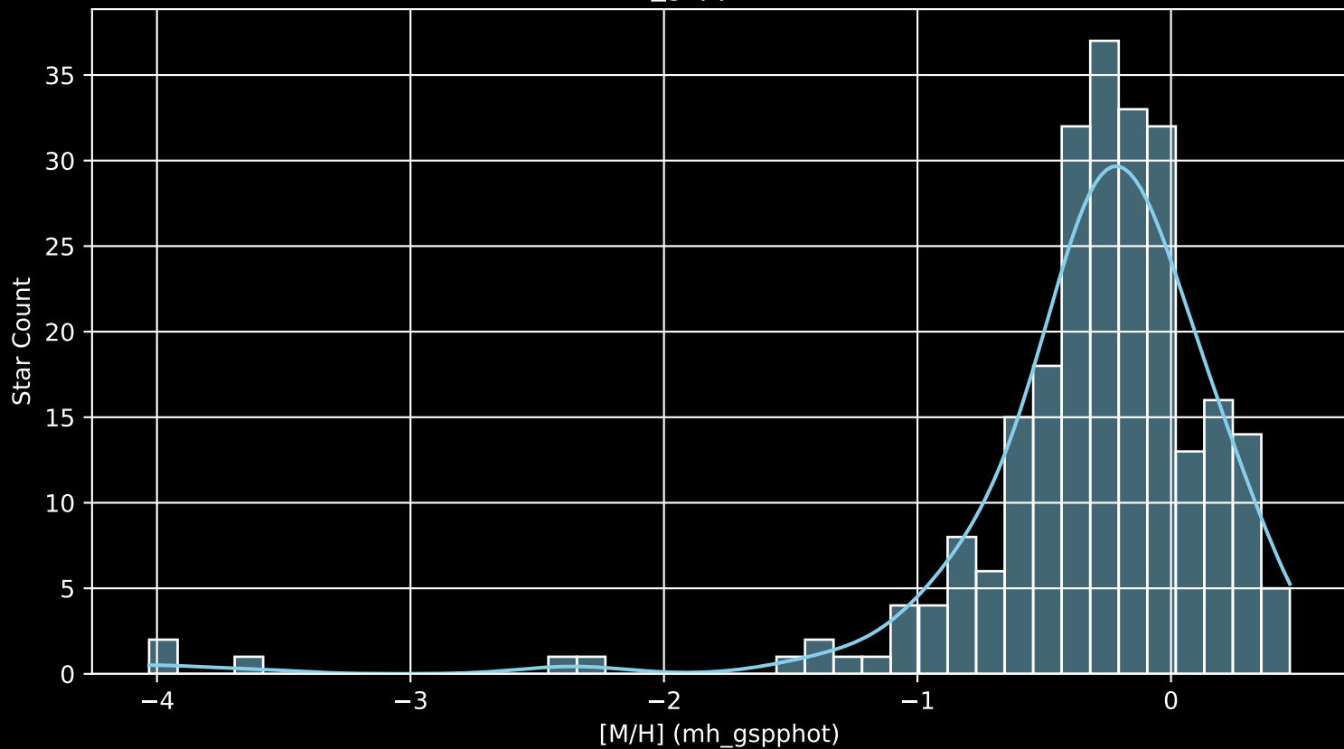
Gaia Cluster: [Alessi_2 [M/H] (mh_gspphot) (n= 247)
