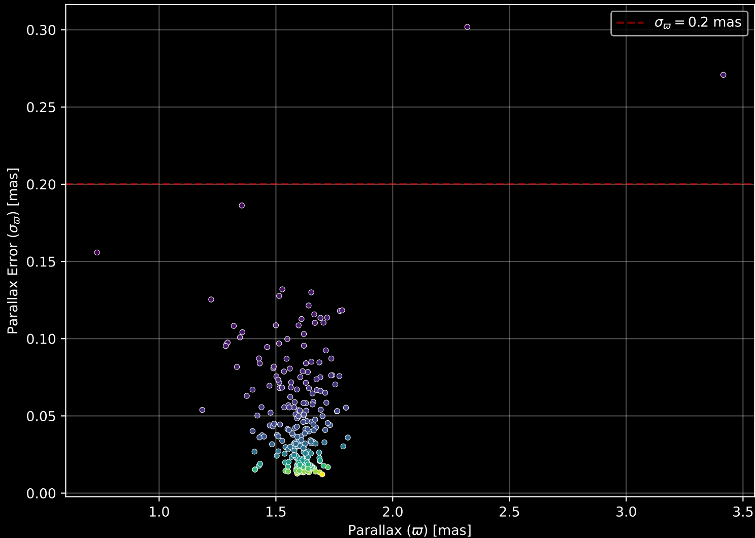
Gaia Cluster: [Alessi_2] Parallax Quality (n= 247)
