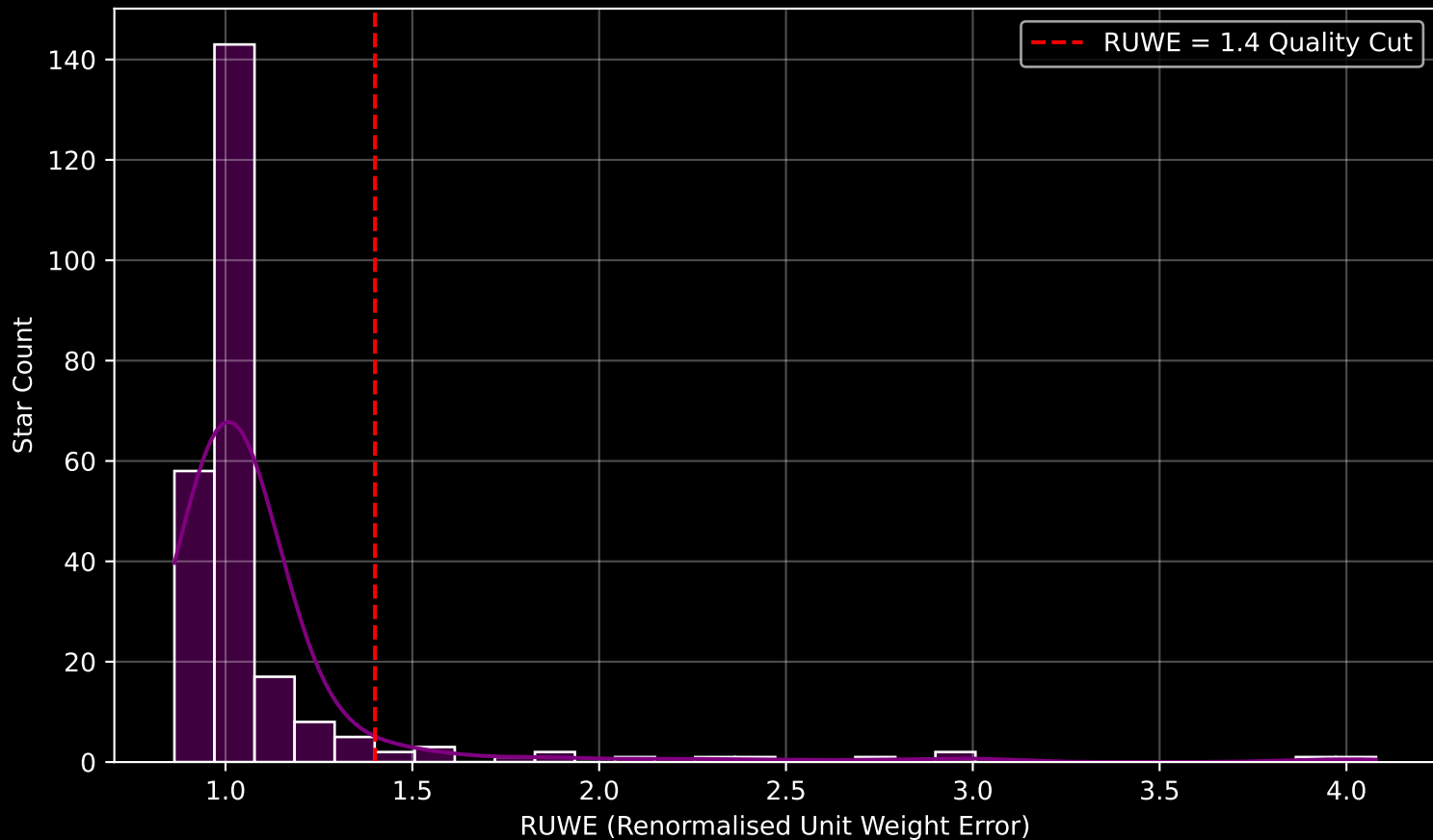
Gaia Cluster: [Alessi_2] RUWE Distribution (n= 247)
