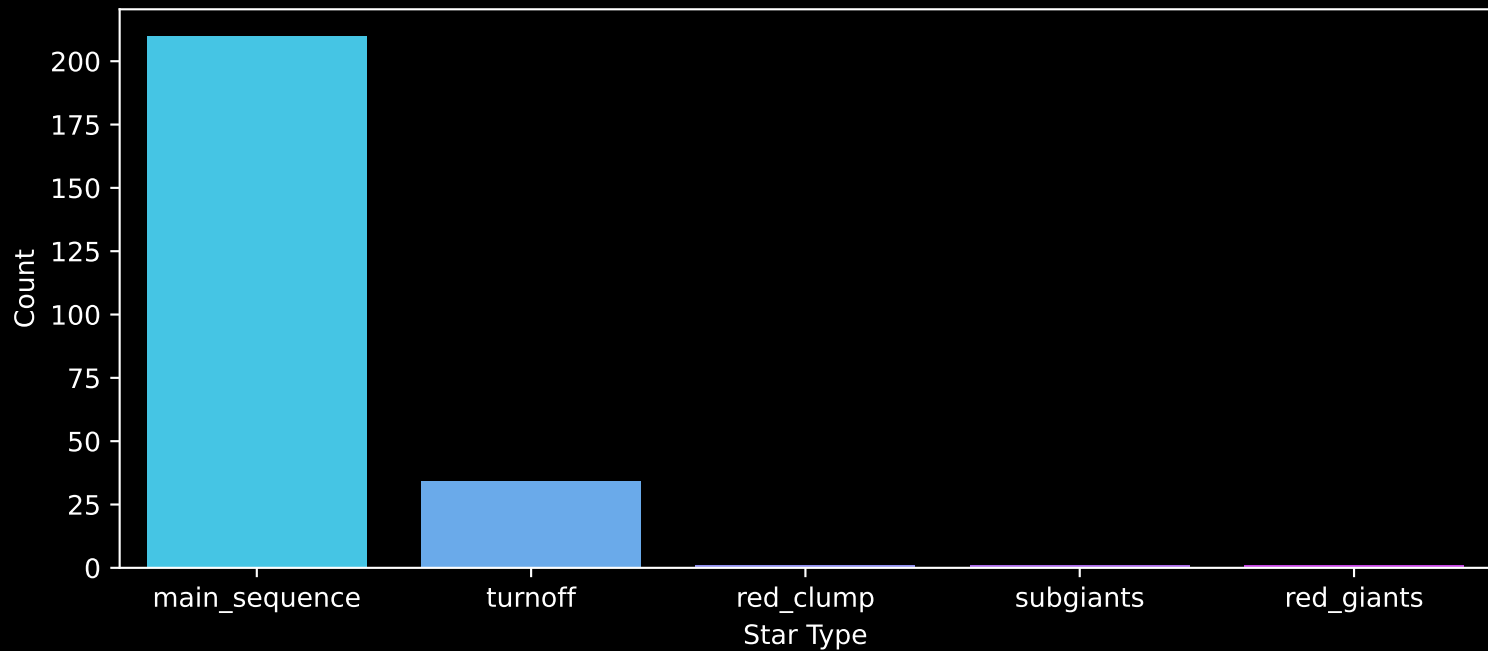
Gaia Cluster: [Alessi_2] Count plot of Star Type
