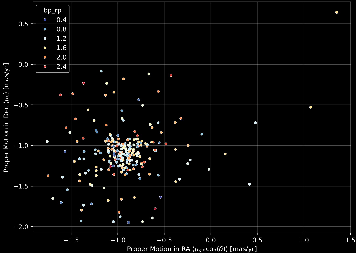
Gaia Cluster: [Alessi_2] Proper Motion Diagram (n= 247)
