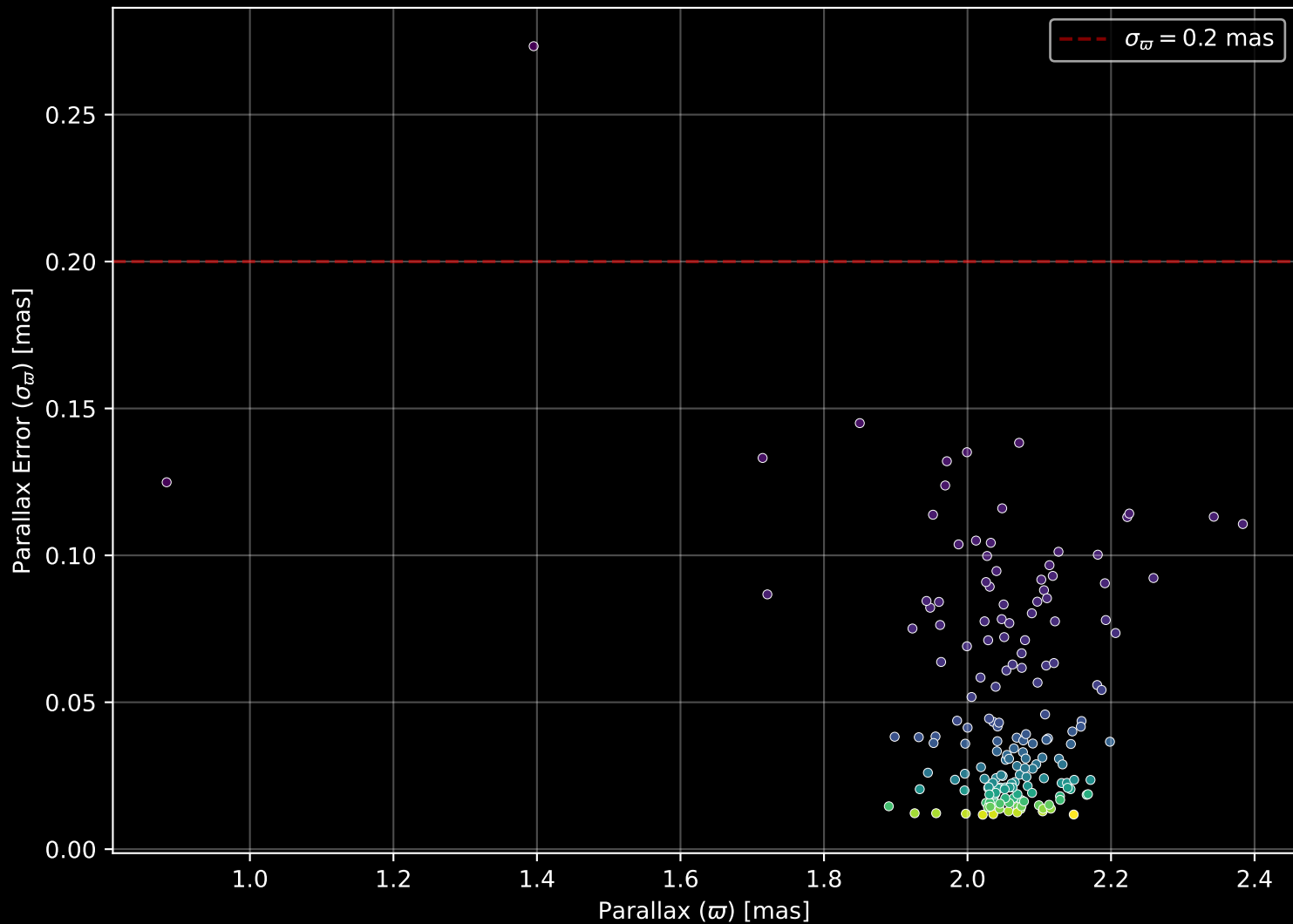
Gaia Cluster: [Alessi_24] Parallax Quality (n= 172)
