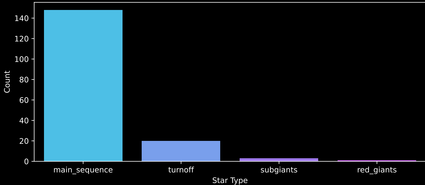
Gaia Cluster: [Alessi_24] Count plot of Star Type
