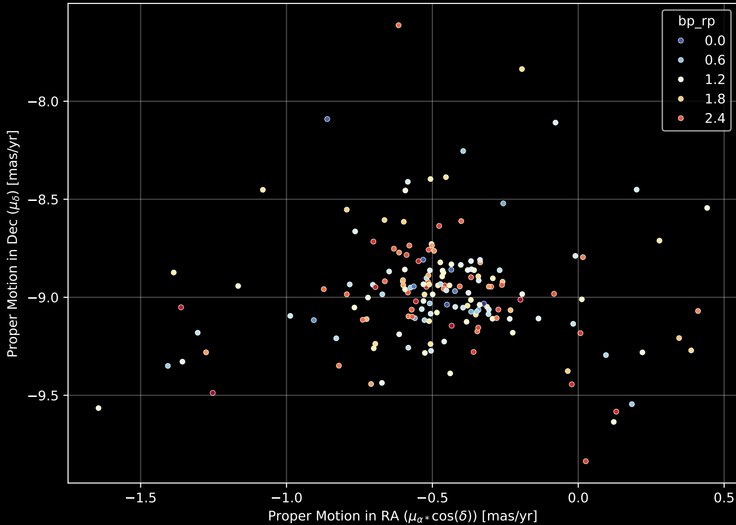
Gaia Cluster: [Alessi_24] Proper Motion Diagram (n= 172)
