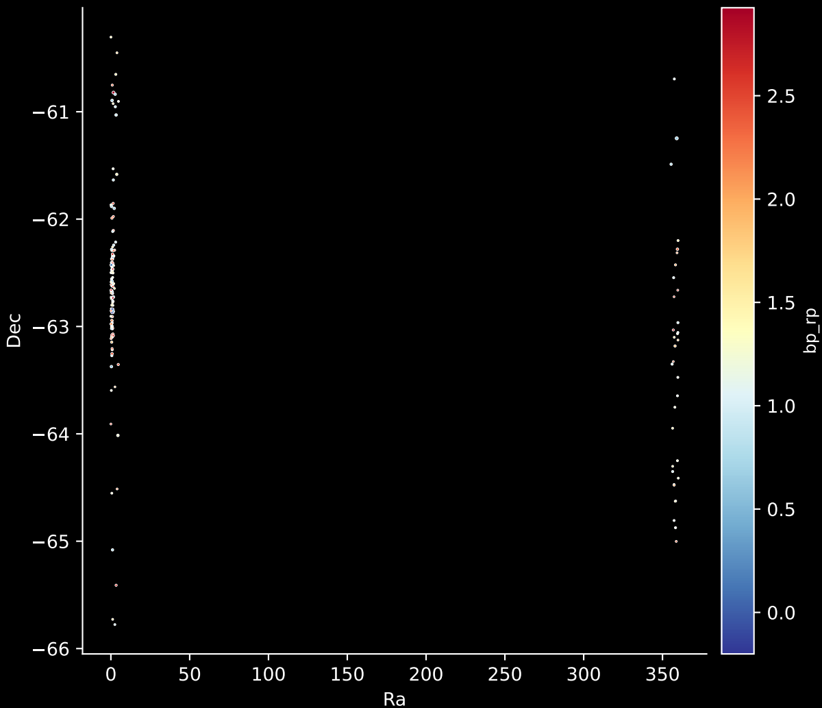
Gaia Cluster: [Alessi_24] Stars: 172
