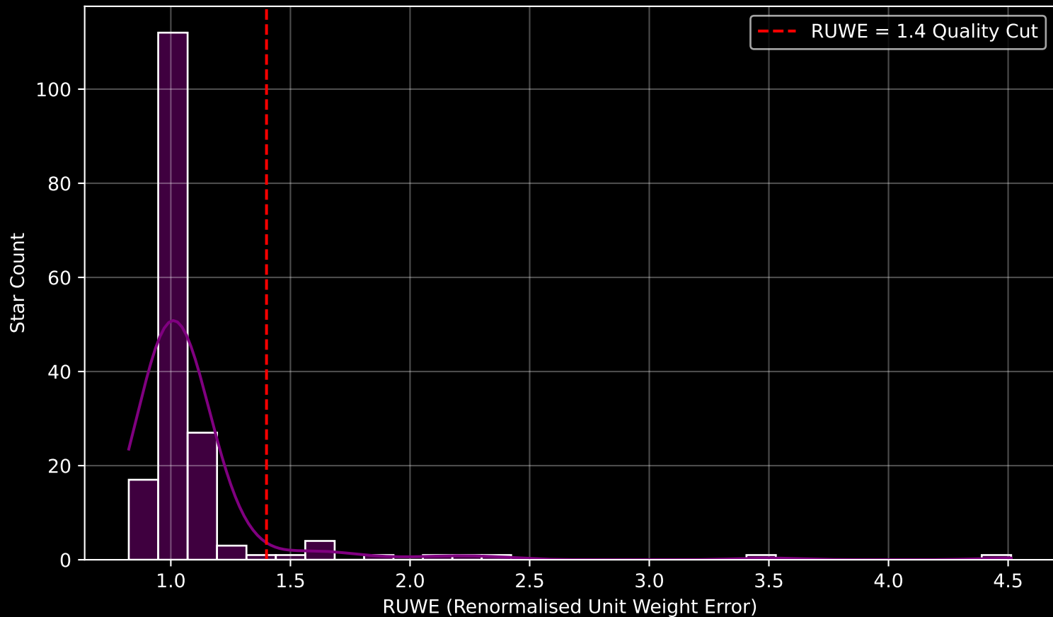
Gaia Cluster: [Alessi_24] RUWE Distribution (n= 171)
