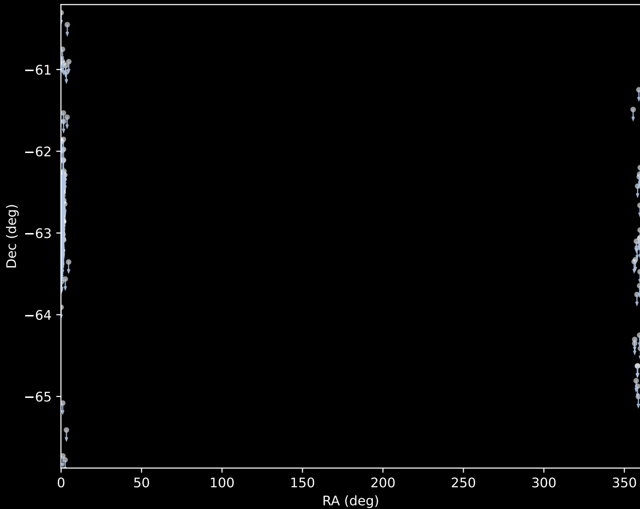
Gaia DR3 Cluster 1 Proper Motion Vectors (n=151)
