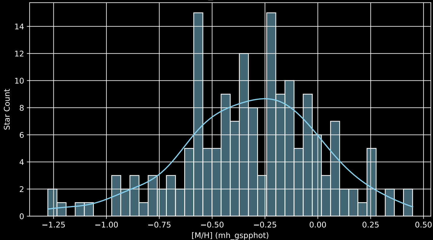
Gaia Cluster: [Alessi_24 [M/H] (mh_gspphot) (n= 171)
