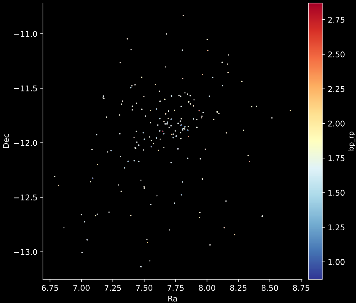
Gaia Cluster: [Alessi_31] Stars: 176
