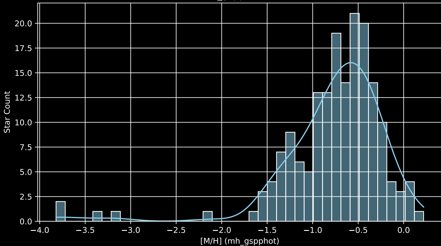
Gaia Cluster: [Alessi_31 [M/H] (mh_gspphot) (n= 176)
