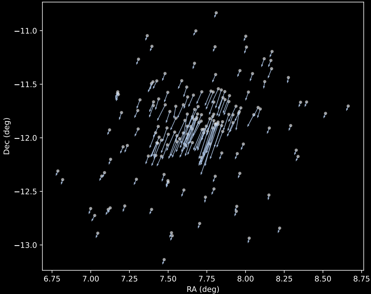
Gaia DR3 Cluster 1 Proper Motion Vectors (n=163)
