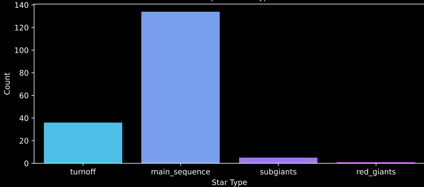
Gaia Cluster: [Alessi_31] Count plot of Star Type
