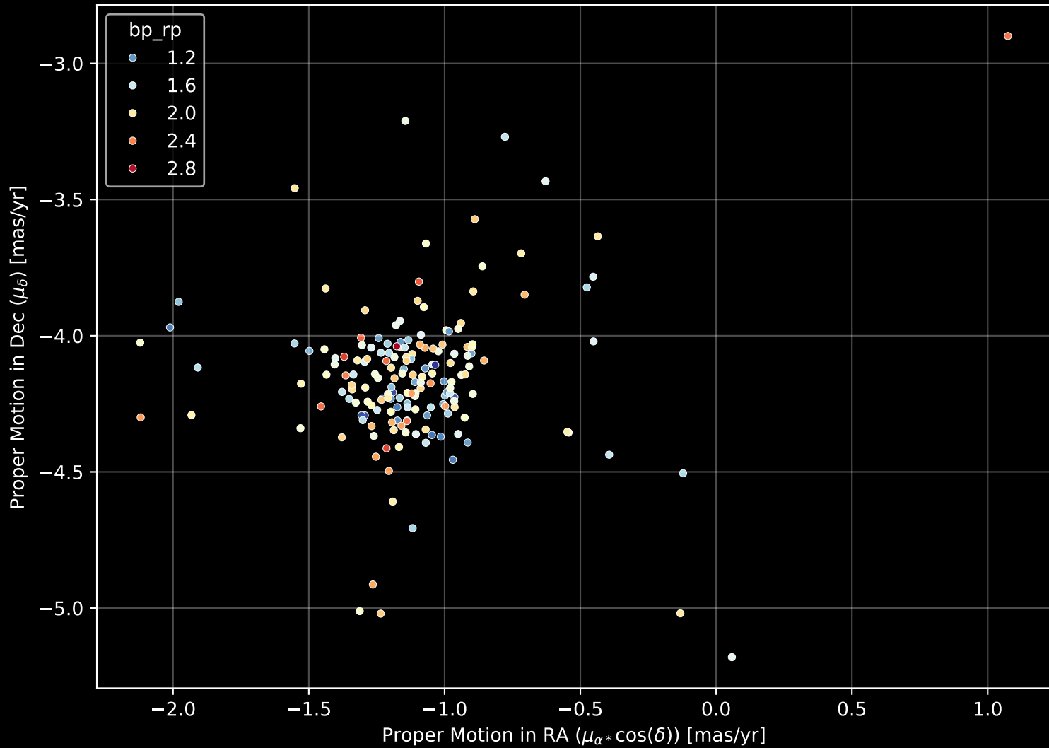
Gaia Cluster: [Alessi_31] Proper Motion Diagram (n= 176)
