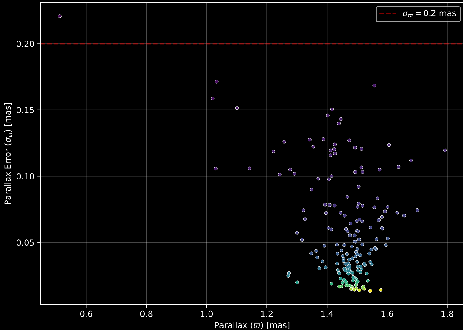
Gaia Cluster: [Alessi_31] Parallax Quality (n= 176)
