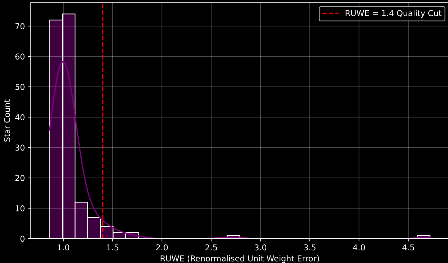
Gaia Cluster: [Alessi_31] RUWE Distribution (n= 175)
