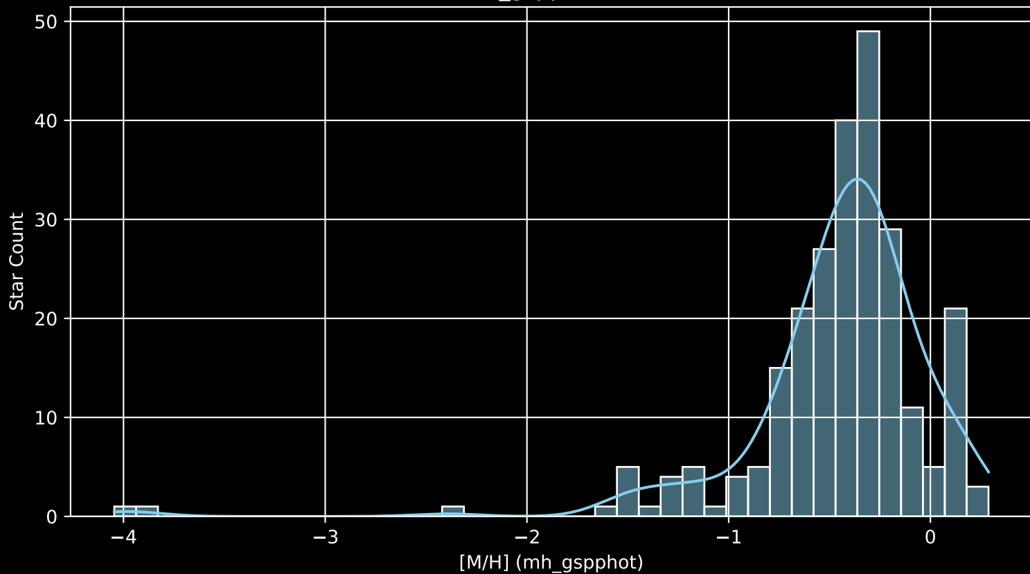
Gaia Cluster: [Alessi_5 [M/H] (mh_gspphot) (n= 250)
