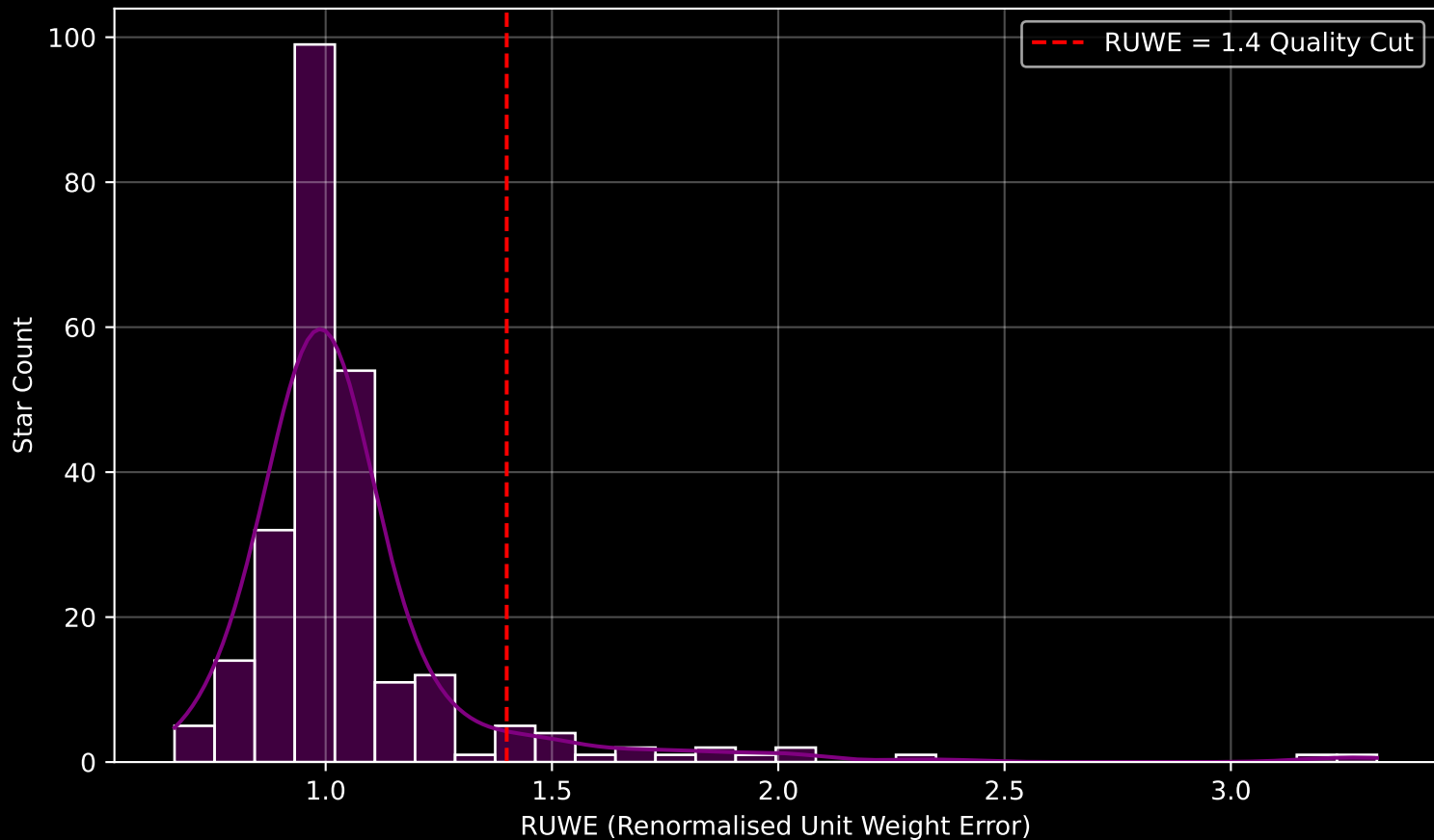
Gaia Cluster: [Alessi_5] RUWE Distribution (n= 249)
