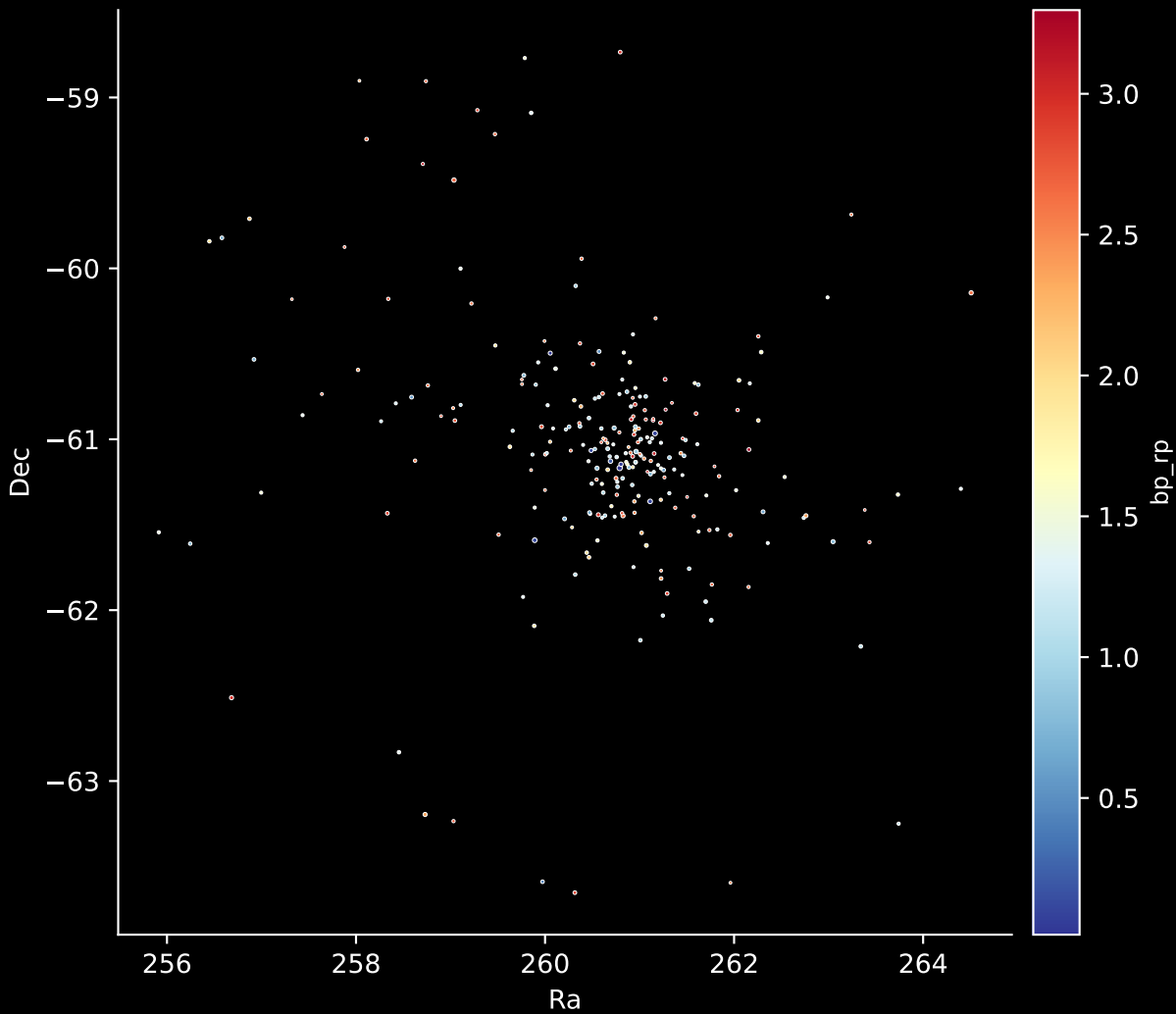
Gaia Cluster: [Alessi_5] Stars: 250
