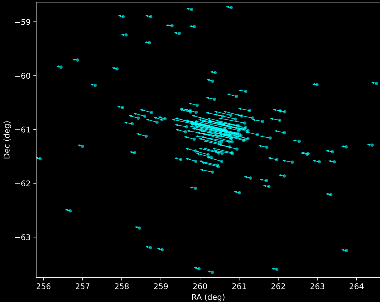
Gaia DR3 Noise Stream Proper Motion Vectors (n=131)
