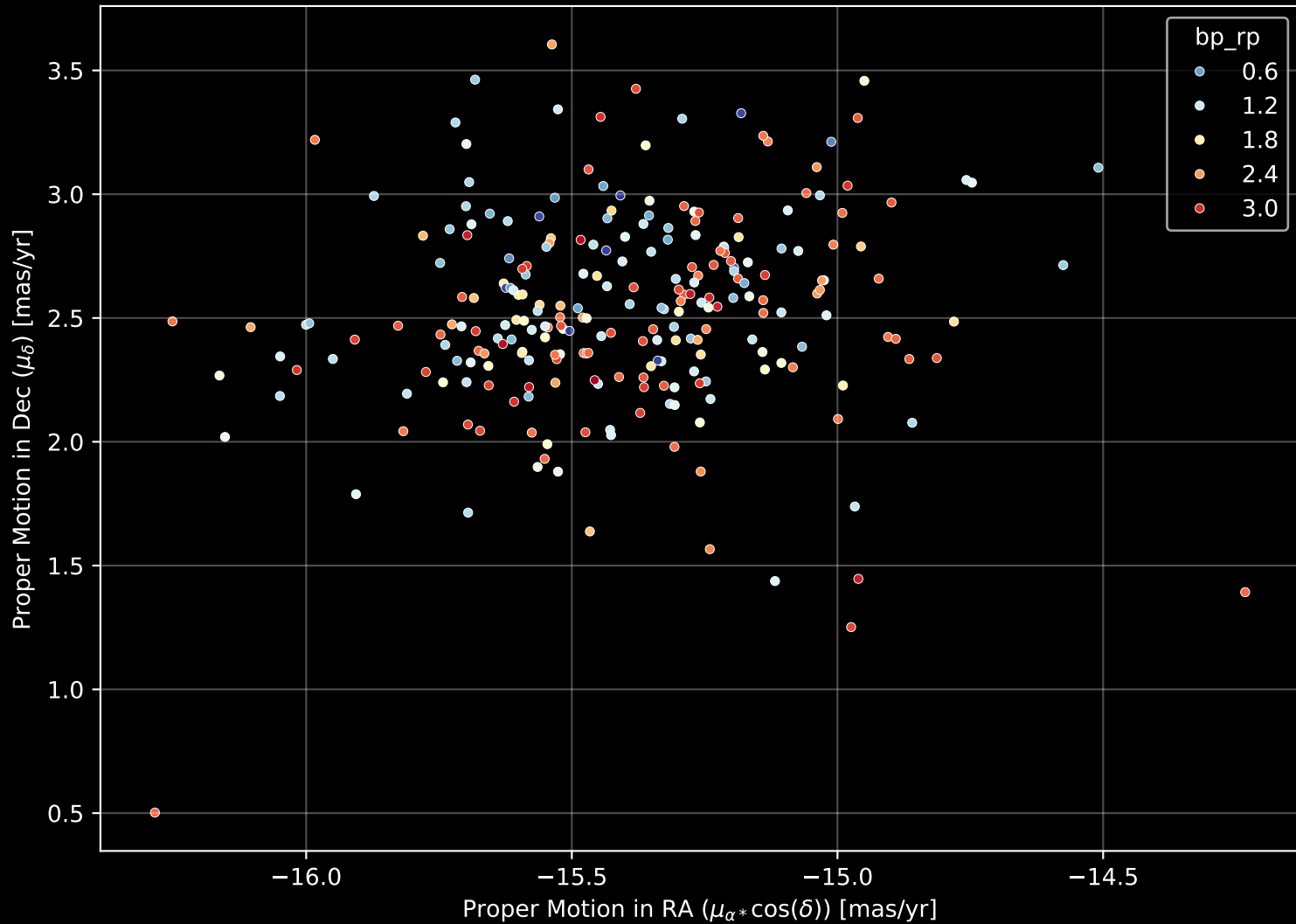
Gaia Cluster: [Alessi_5] Proper Motion Diagram (n= 250)
