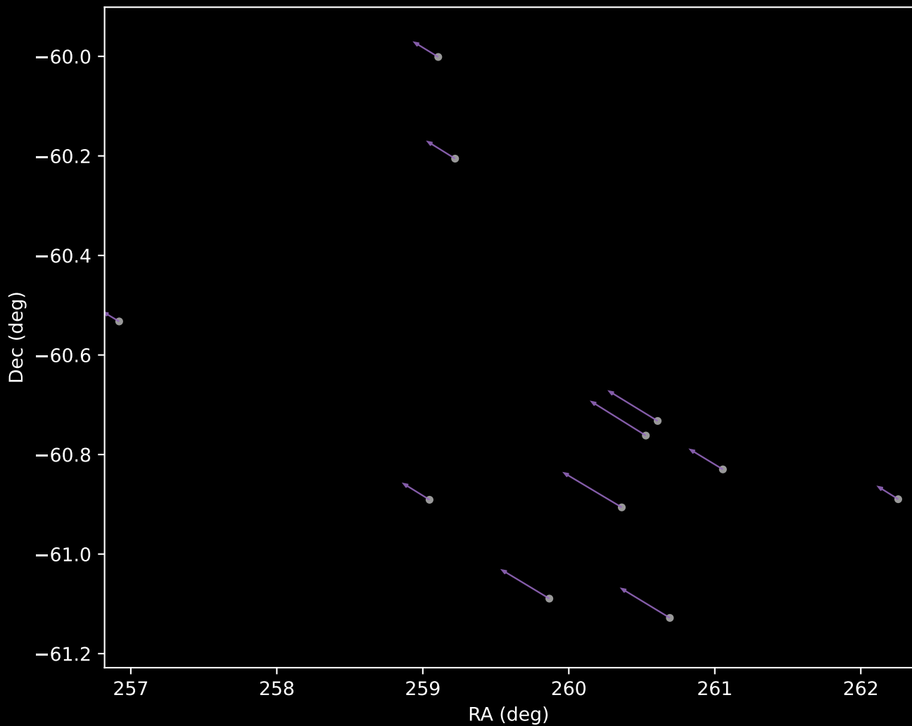
Gaia DR3 Cluster 8 Proper Motion Vectors (n=11)
