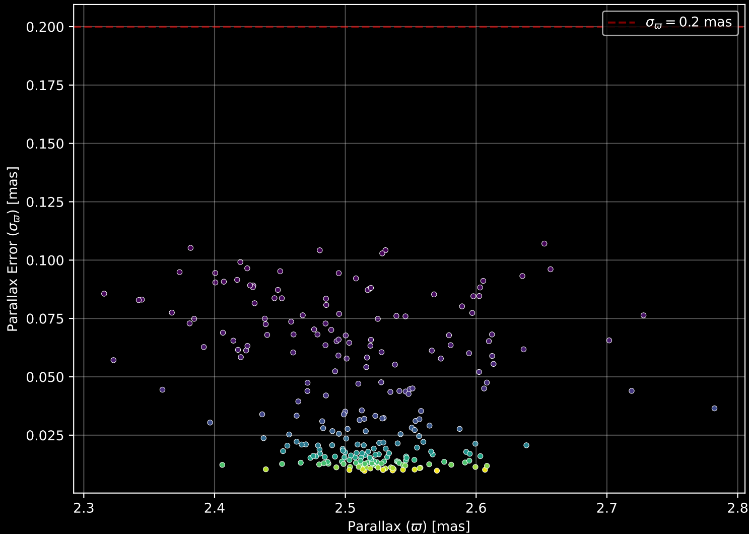
Gaia Cluster: [Alessi_5] Parallax Quality (n= 250)
