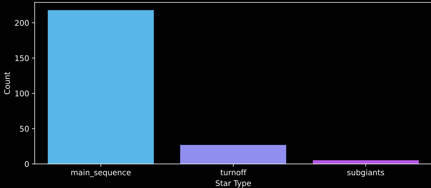
Gaia Cluster: [Alessi_5] Count plot of Star Type
