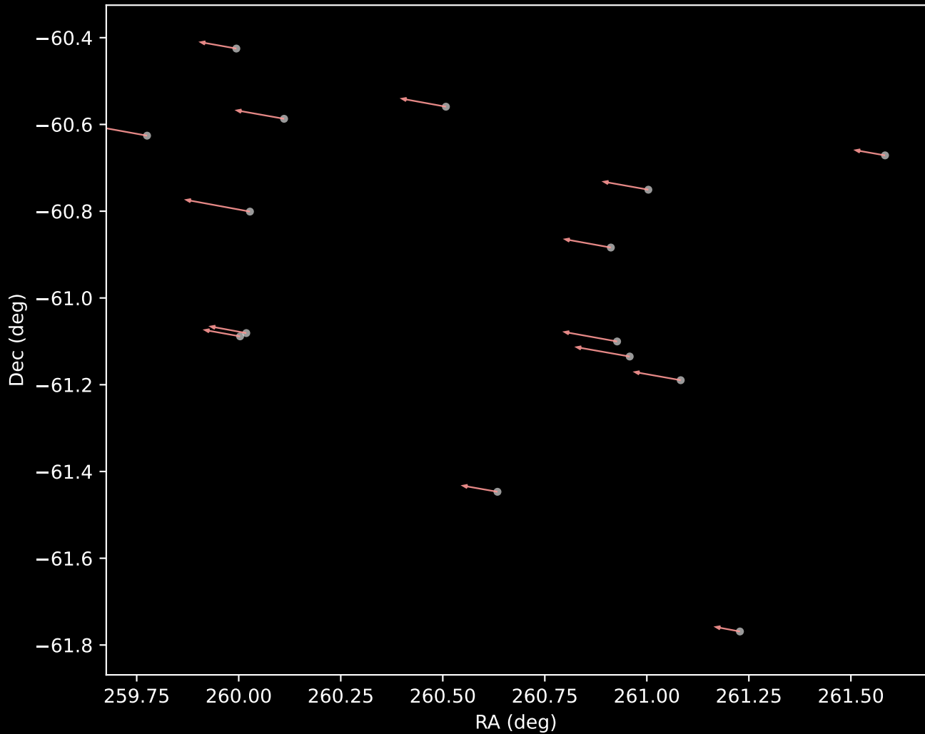
Gaia DR3 Cluster 7 Proper Motion Vectors (n=15)
