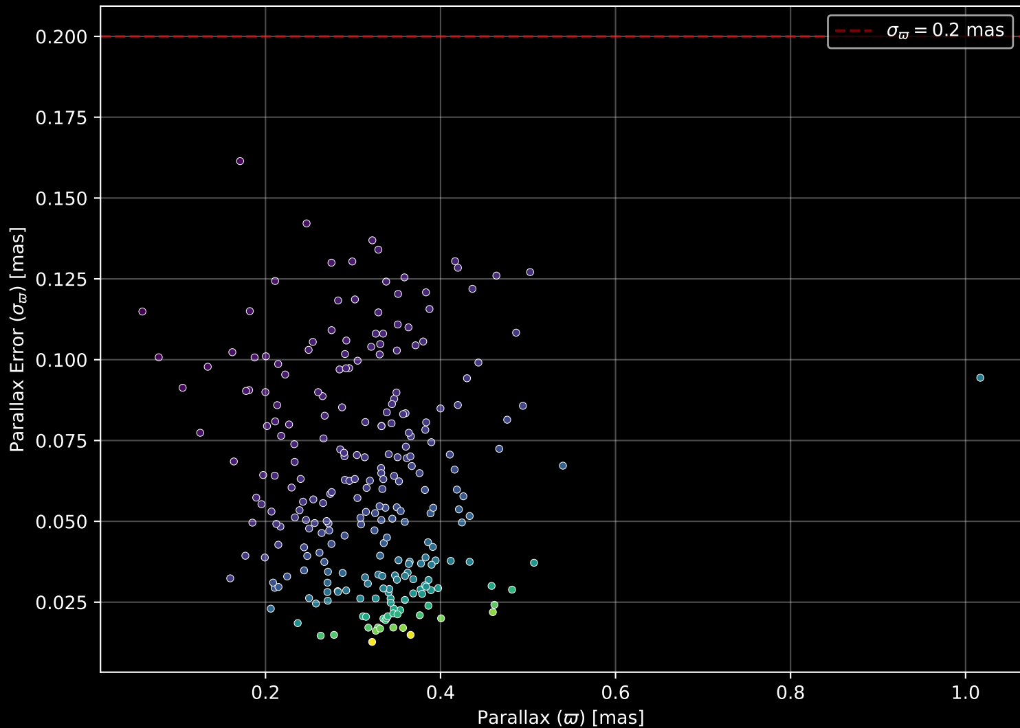
Gaia Cluster: [Alessi_60] Parallax Quality (n= 255)
