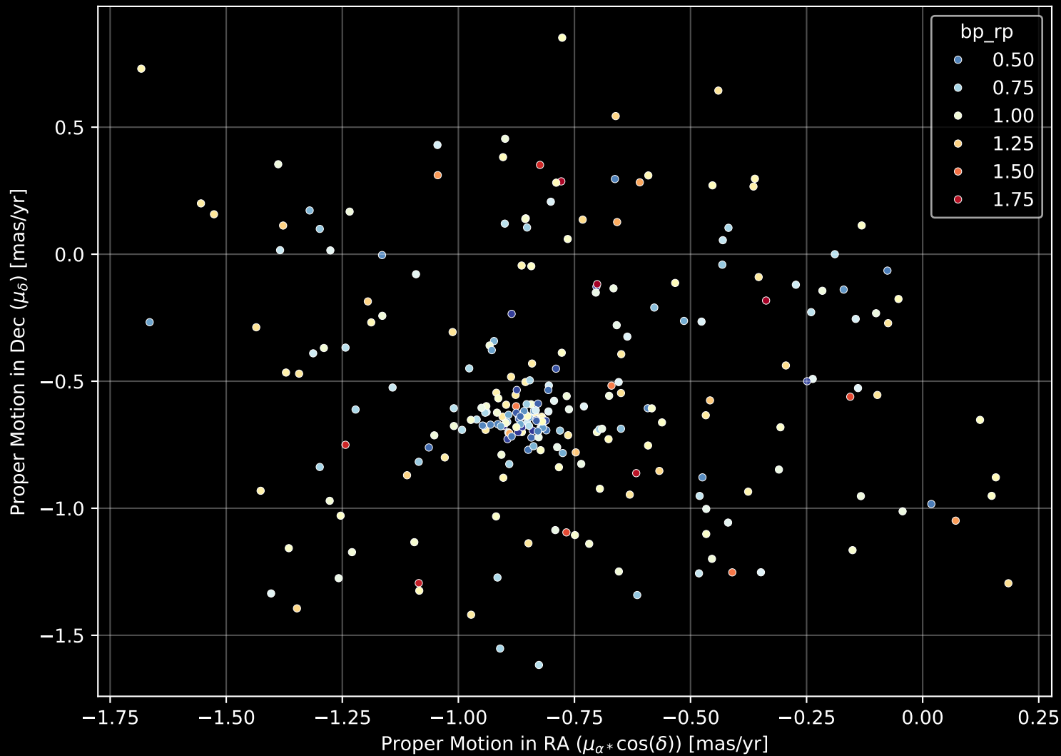
Gaia Cluster: [Alessi_60] Proper Motion Diagram (n= 255)
