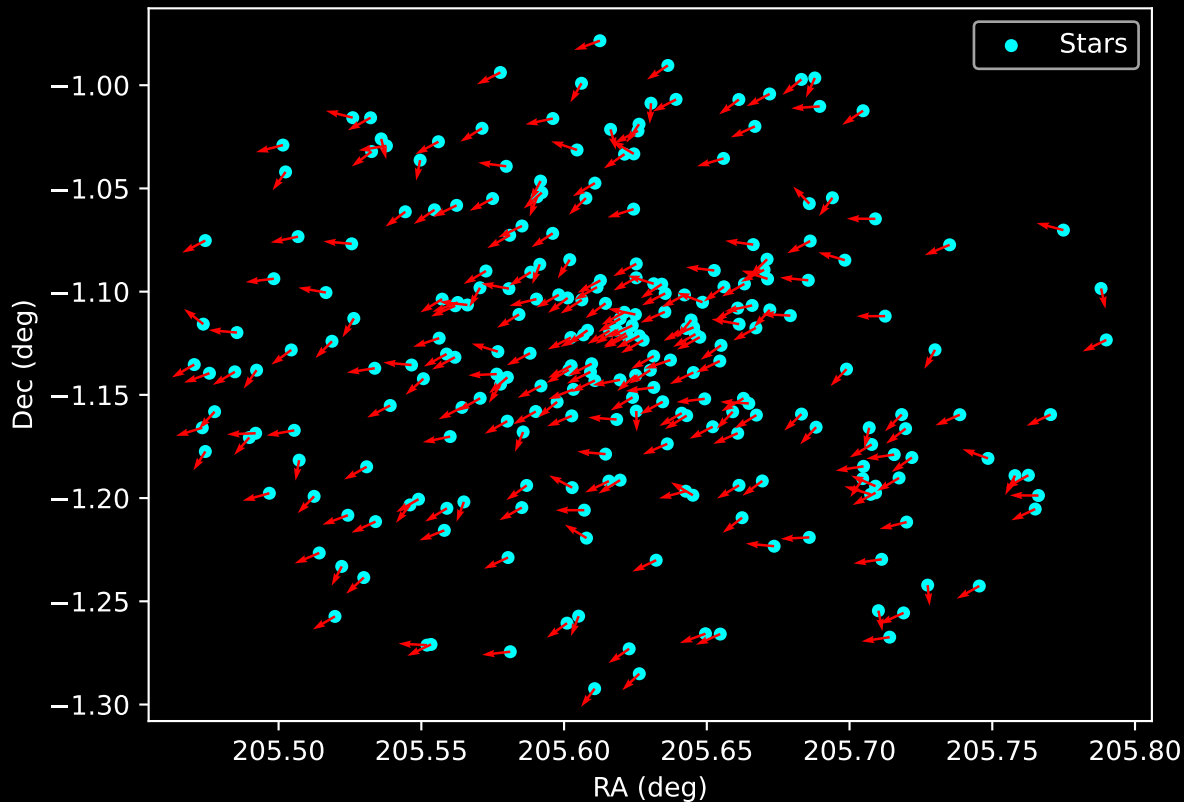
Gaia Cluster: [Alessi_60] Proper Motion Vectors for Gaia Star Field (n= 255)
