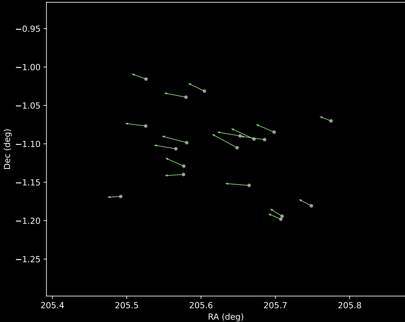
Gaia DR3 Cluster 5 Proper Motion Vectors (n=19)
