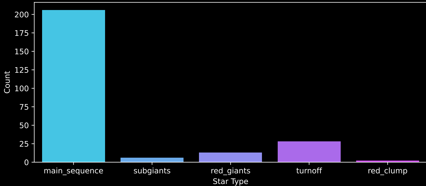
Gaia Cluster: [Alessi_60] Count plot of Star Type
