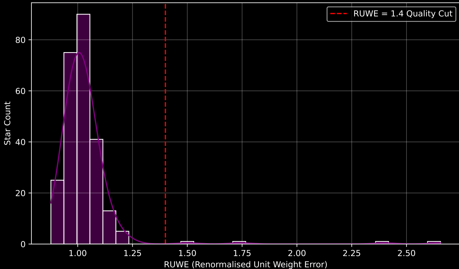
Gaia Cluster: [Alessi_60] RUWE Distribution (n= 253)
