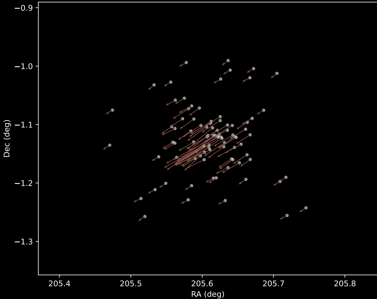
Gaia DR3 Cluster 10 Proper Motion Vectors (n=88)
