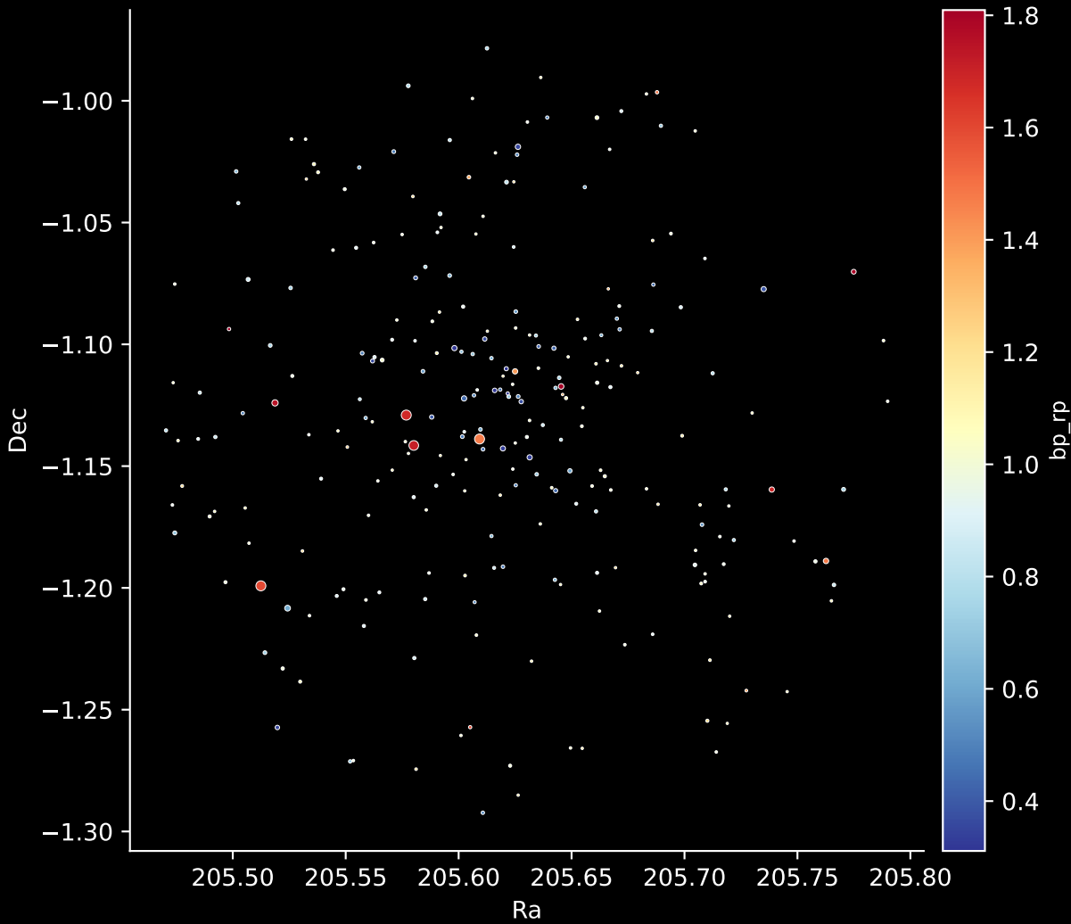
Gaia Cluster: [Alessi_60] Stars: 255
