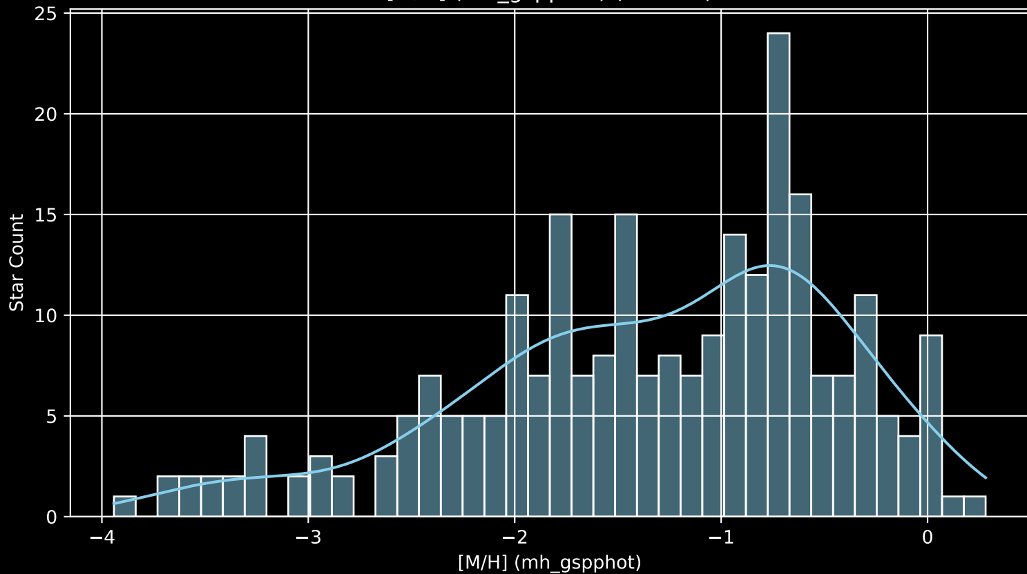
Gaia Cluster: [Alessi_60 [M/H] (mh_gspphot) (n= 255)
