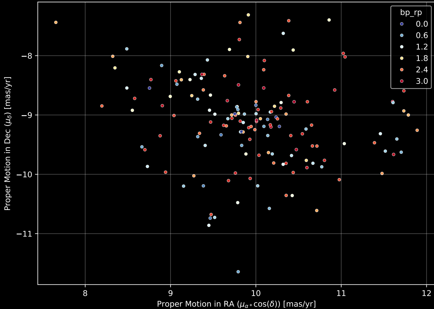
Gaia Cluster: [Alessi_9] Proper Motion Diagram (n= 157)
