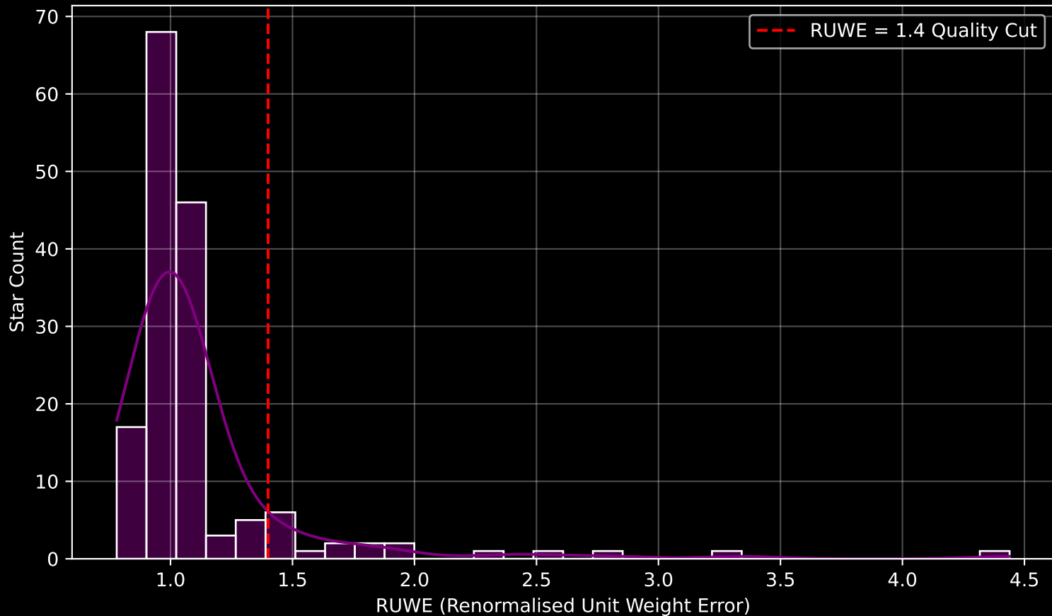
Gaia Cluster: [Alessi_9] RUWE Distribution (n= 157)
