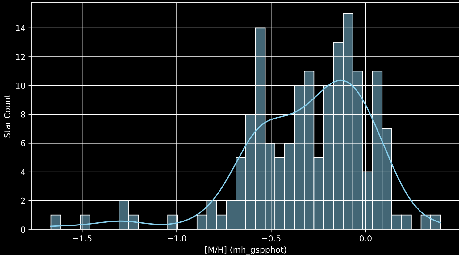
Gaia Cluster: [Alessi_9 [M/H] (mh_gspphot) (n= 157)
