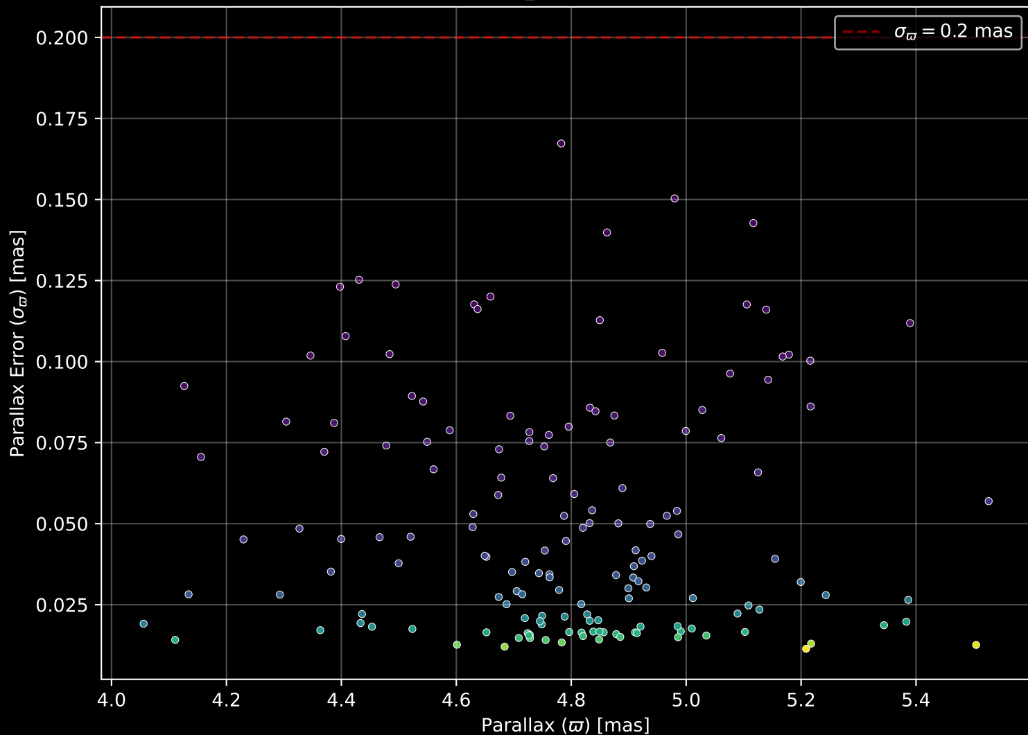
Gaia Cluster: [Alessi_9] Parallax Quality (n= 157)
