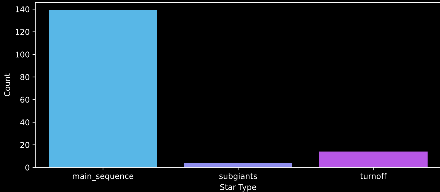
Gaia Cluster: [Alessi_9] Count plot of Star Type
