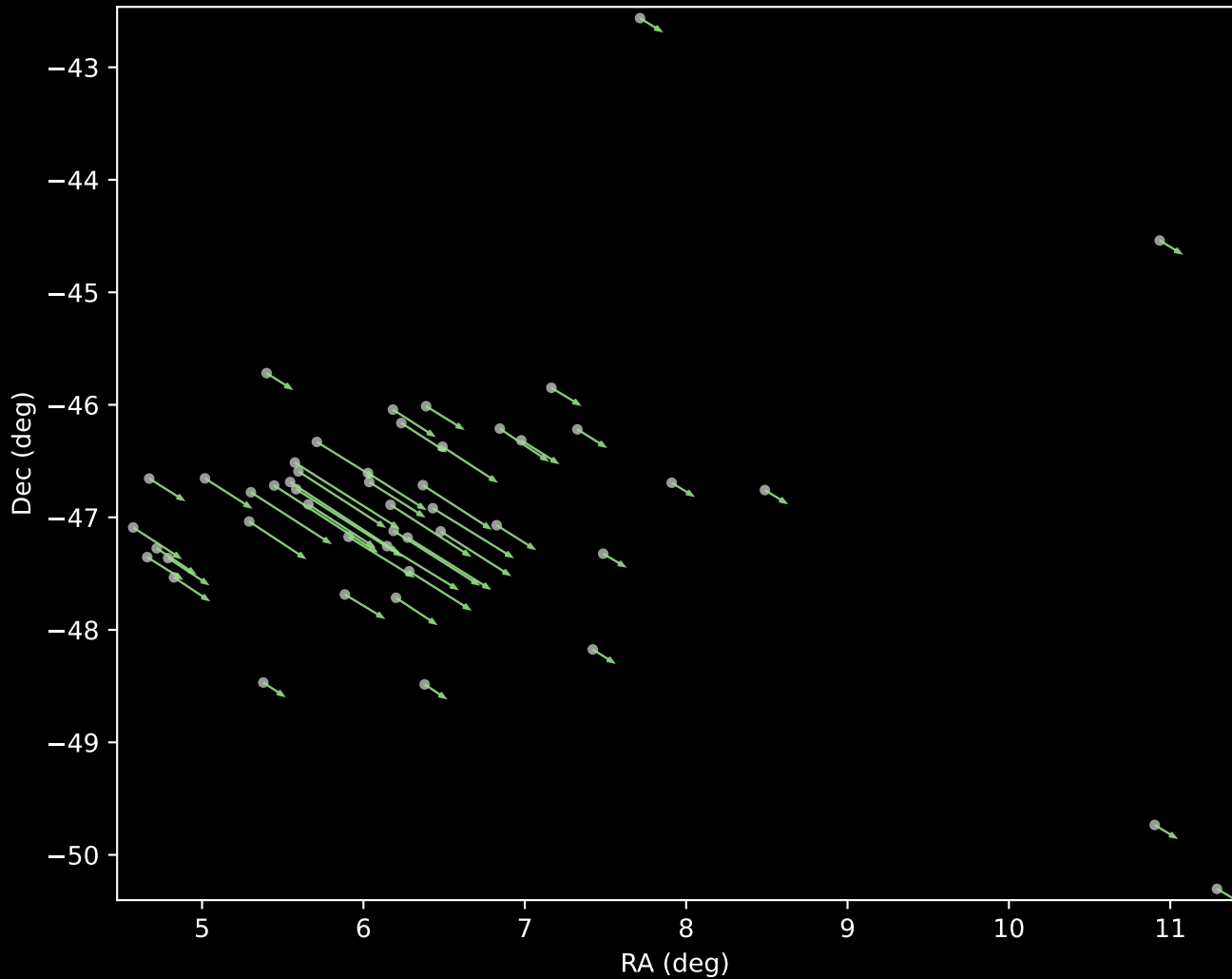
Gaia DR3 Cluster 5 Proper Motion Vectors (n=49)
