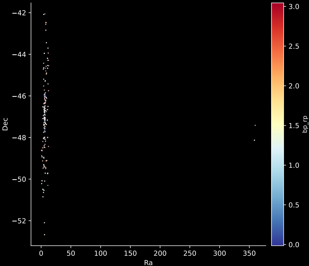
Gaia Cluster: [Alessi_9] Stars: 157
