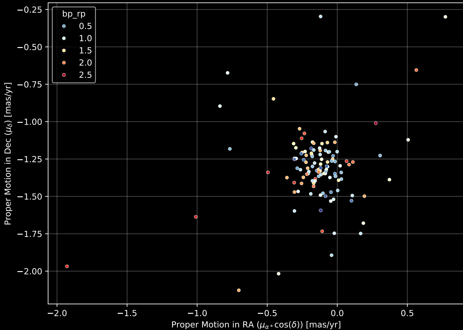
Gaia Cluster: [Alessi_Teutsch_11] Proper Motion Diagram (n= 118)
