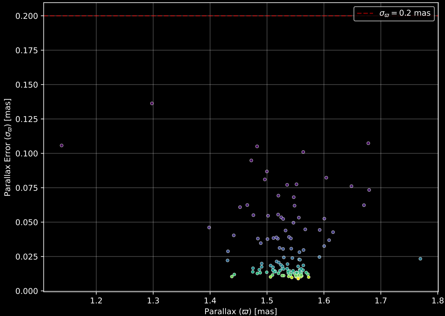
Gaia Cluster: [Alessi_Teutsch_11] Parallax Quality (n= 118)
