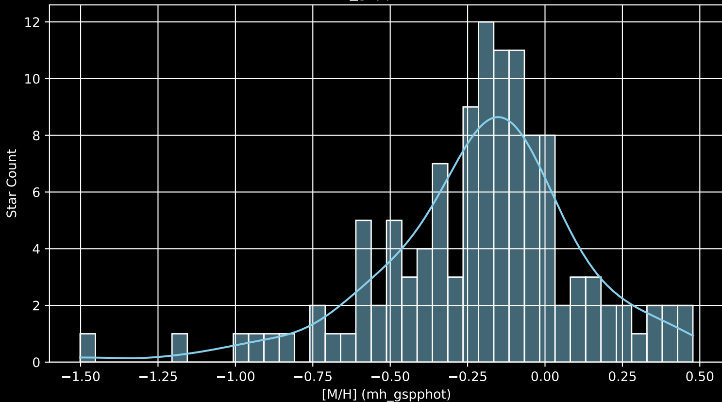
Gaia Cluster: [Alessi_Teutsch_11 [M/H] (mh_gspphot) (n= 117)
