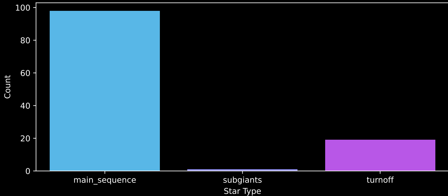
Gaia Cluster: [Alessi_Teutsch_11] Count plot of Star Type
