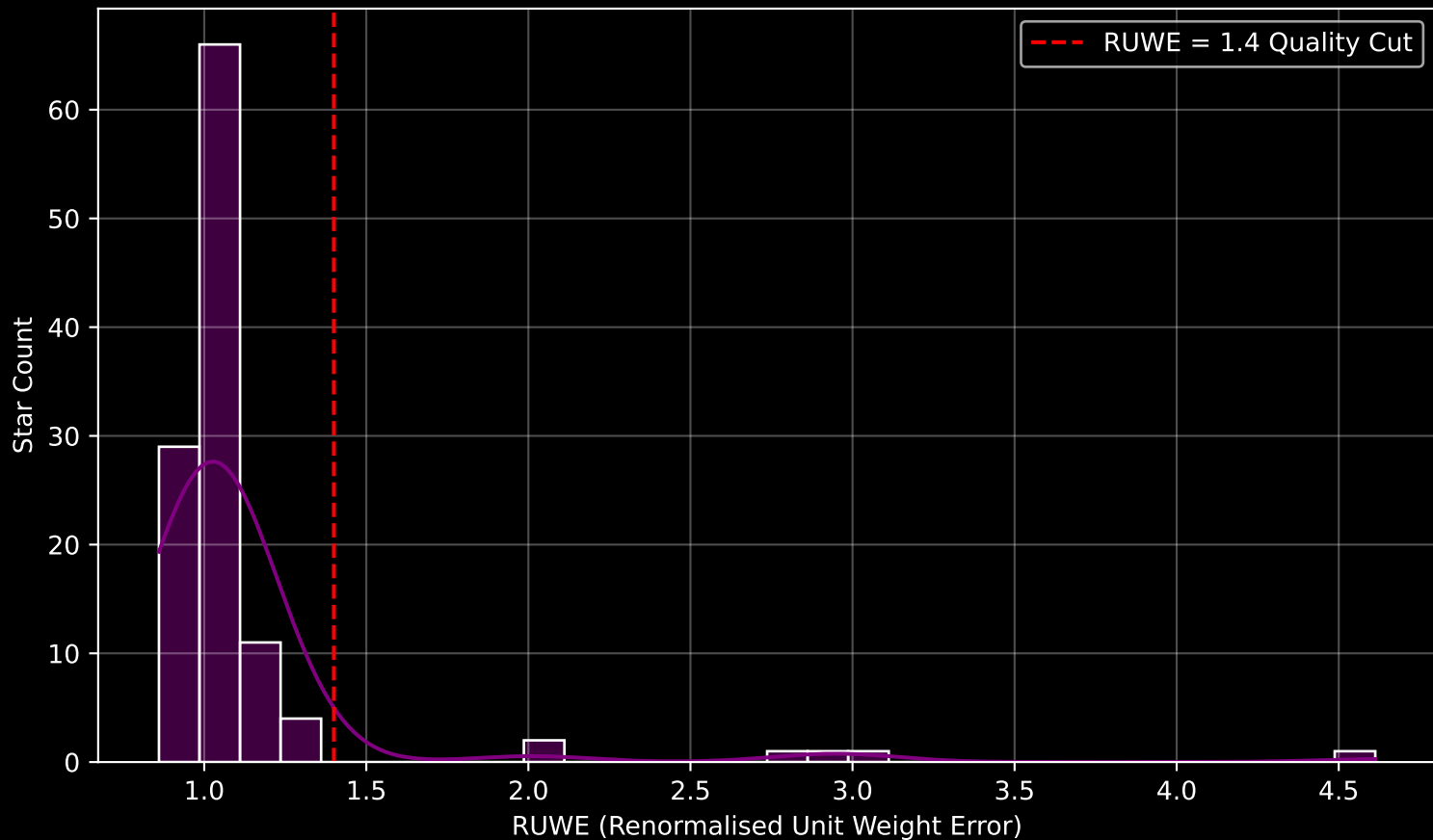
Gaia Cluster: [Alessi_Teutsch_11] RUWE Distribution (n= 116)
