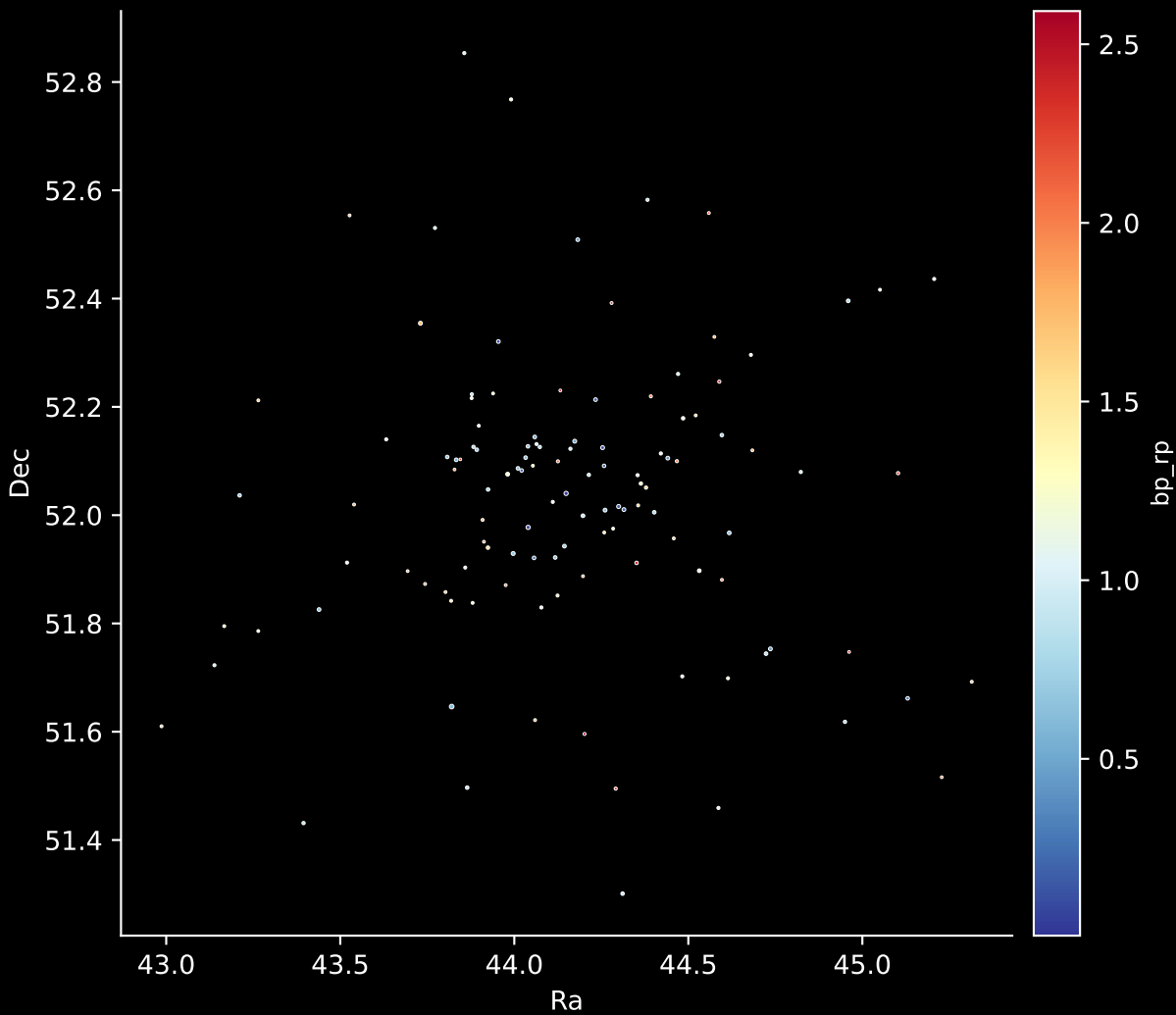
Gaia Cluster: [Alessi_Teutsch_11] Stars: 118
