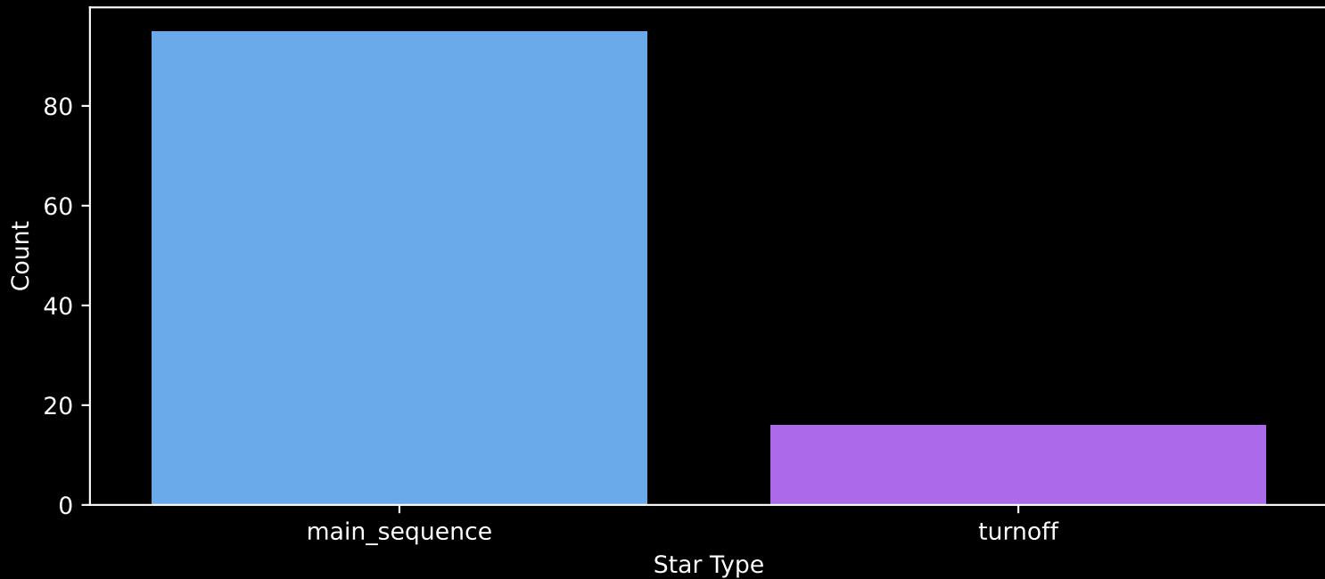
Gaia Cluster: [Alessi_Teutsch_3] Count plot of Star Type
