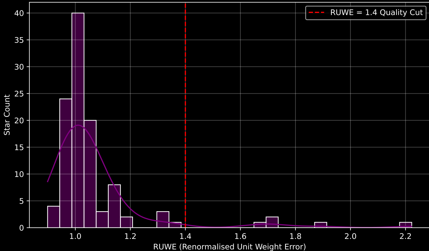
Gaia Cluster: [Alessi_Teutsch_3] RUWE Distribution (n= 110)
