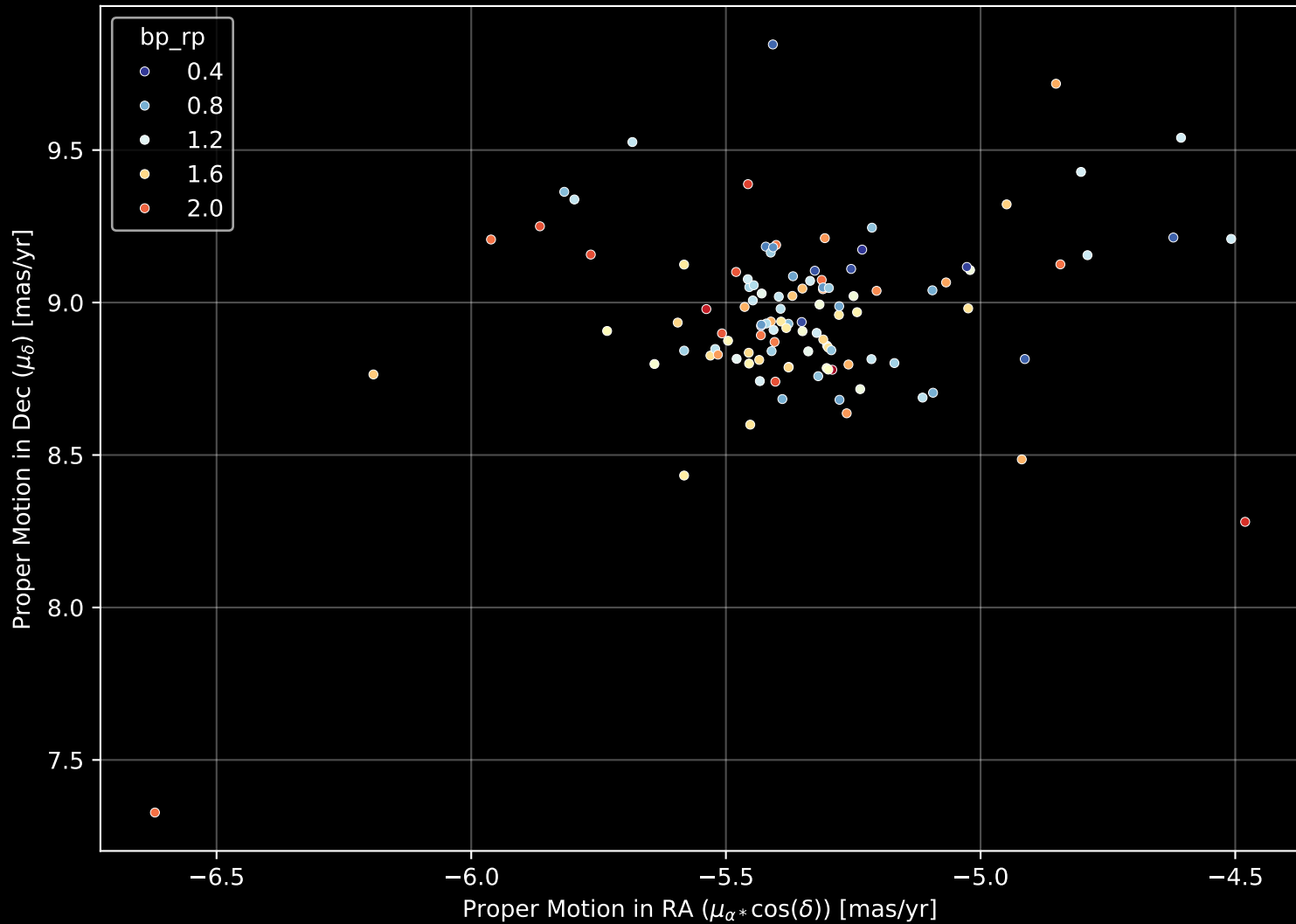
Gaia Cluster: [Alessi_Teutsch_3] Proper Motion Diagram (n= 111)
