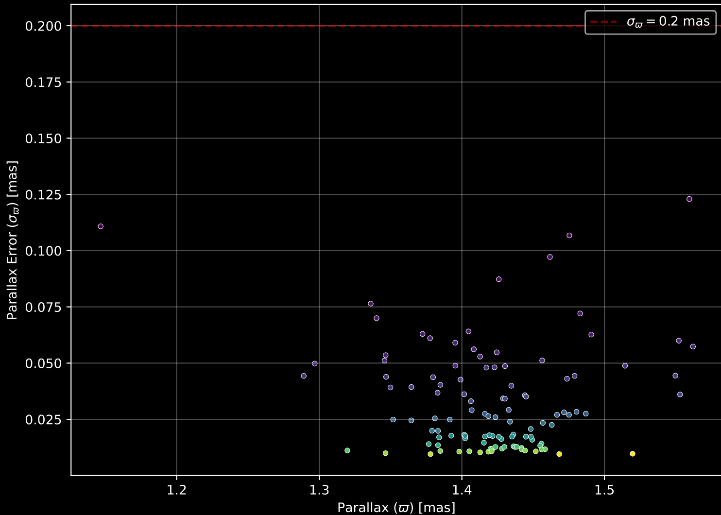
Gaia Cluster: [Alessi_Teutsch_3] Parallax Quality (n= 111)
