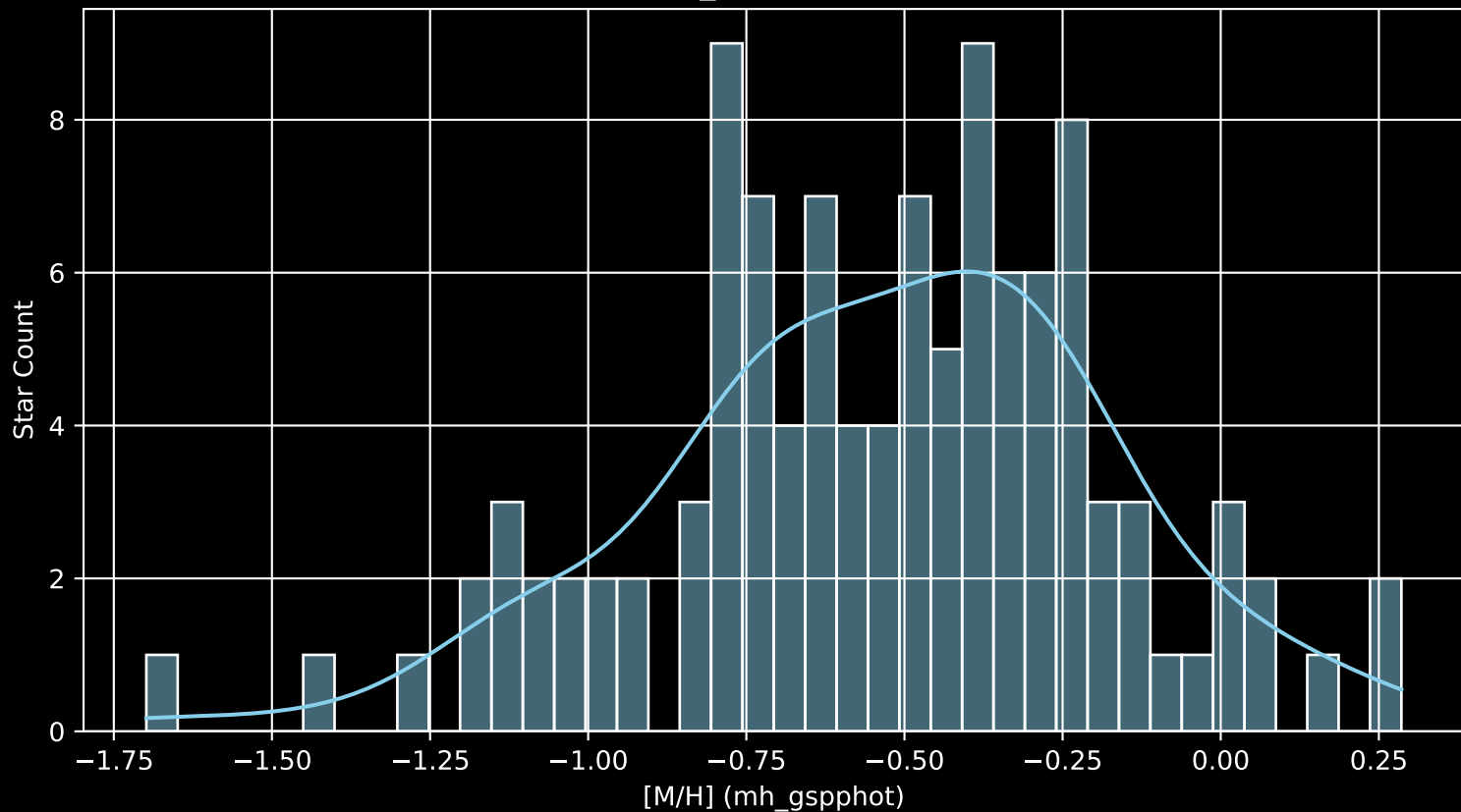
Gaia Cluster: [Alessi_Teutsch_3 [M/H] (mh_gspphot) (n= 111)
