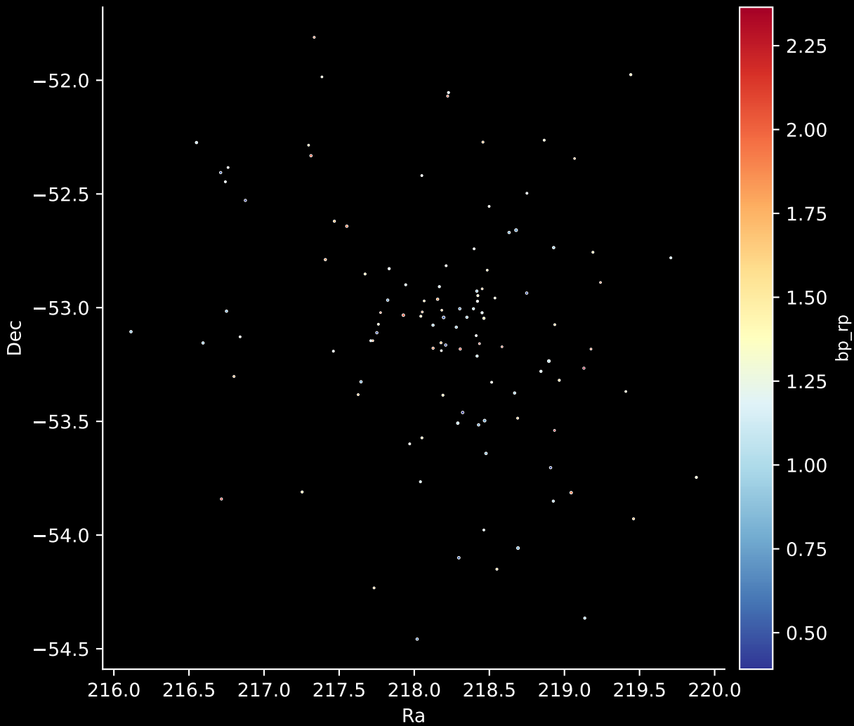
Gaia Cluster: [Alessi_Teutsch_3] Stars: 111
