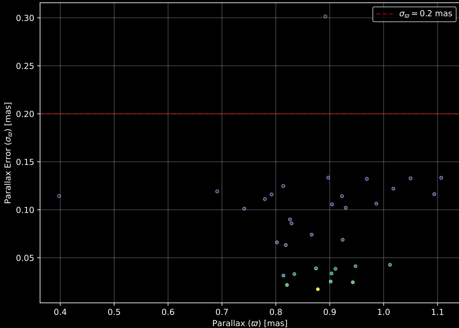
Gaia Cluster: [Antalova_2] Parallax Quality (n= 35)
