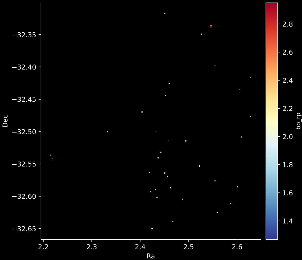
Gaia Cluster: [Antalova_2] Stars: 35
