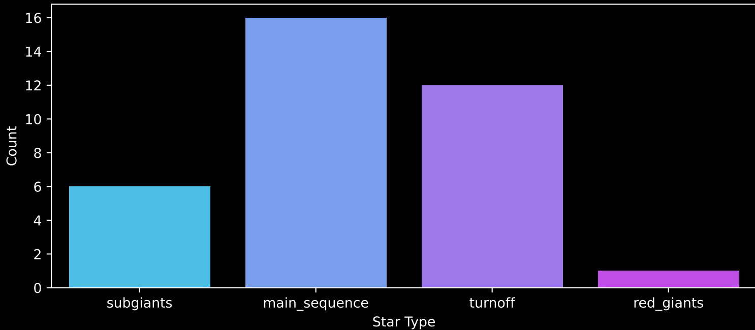
Gaia Cluster: [Antalova_2] Count plot of Star Type
