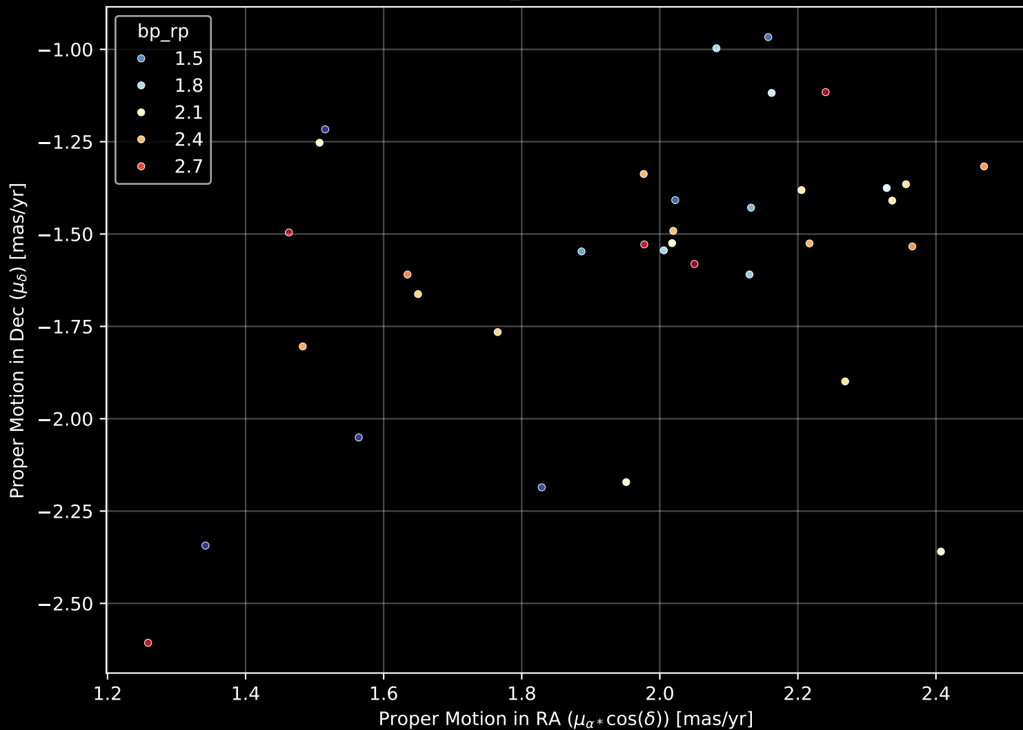
Gaia Cluster: [Antalova_2] Proper Motion Diagram (n= 35)
