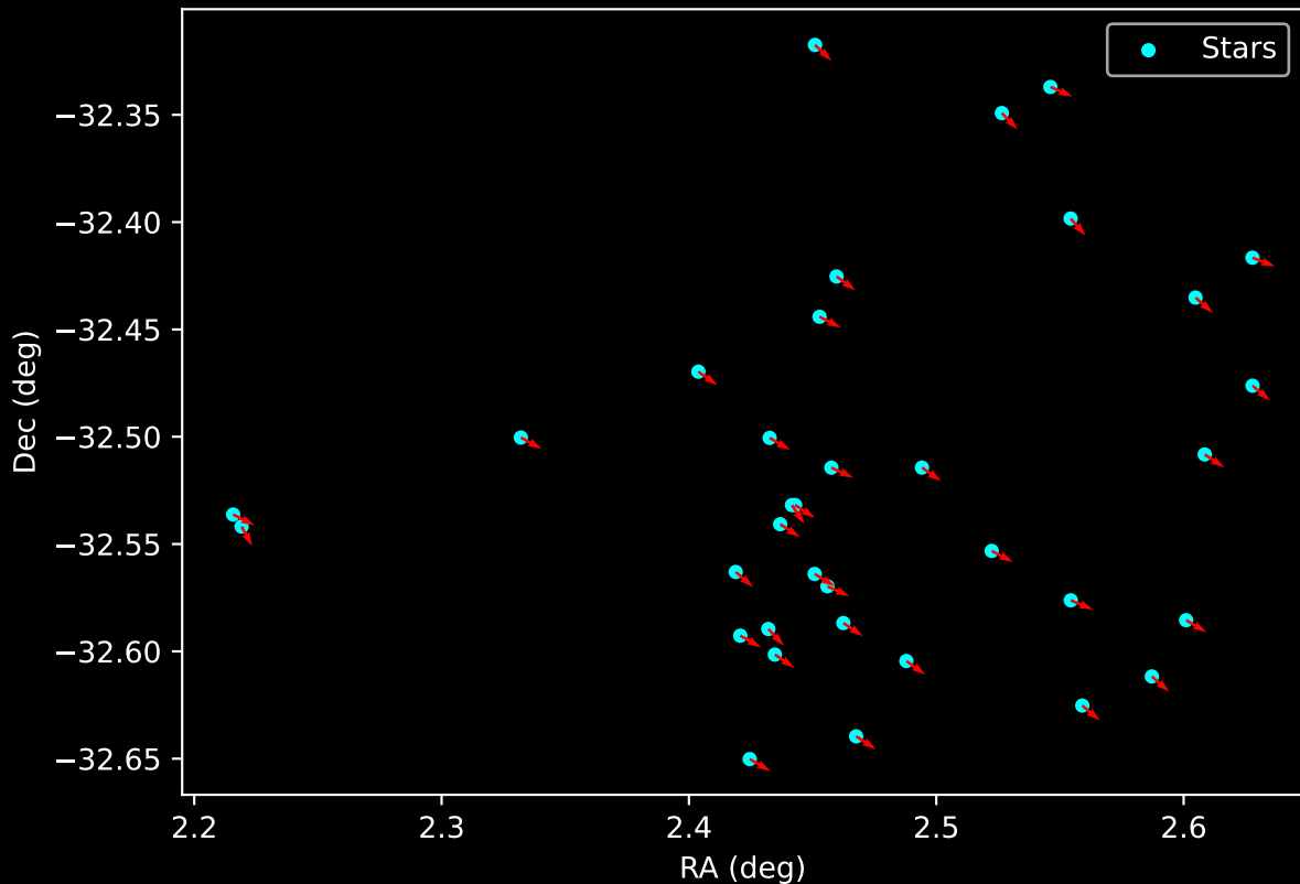
Gaia Cluster: [Antalova_2] Proper Motion Vectors for Gaia Star Field (n= 35)
