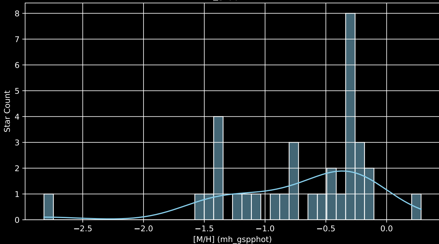
Gaia Cluster: [Antalova_2 [M/H] (mh_gspphot) (n= 34)
