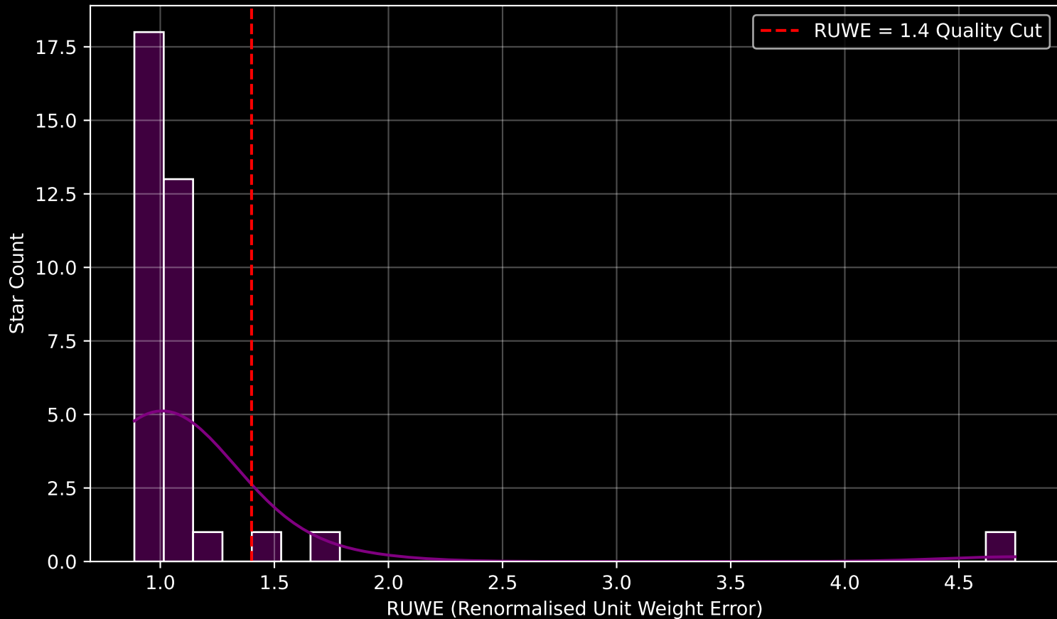
Gaia Cluster: [Antalova_2] RUWE Distribution (n= 35)
