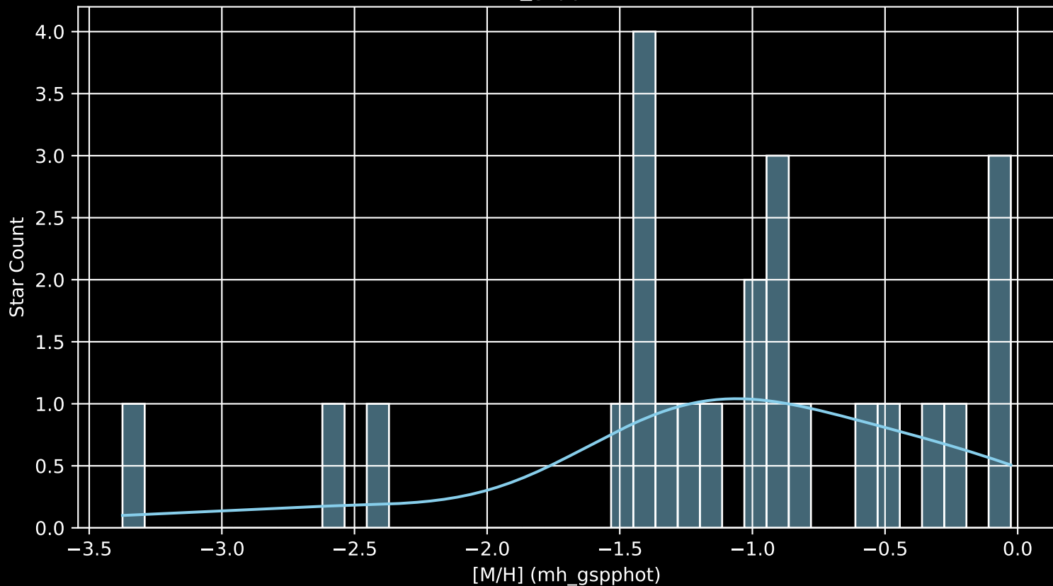
Gaia Cluster: [BDSB93 [M/H] (mh_gspphot) (n= 24)
