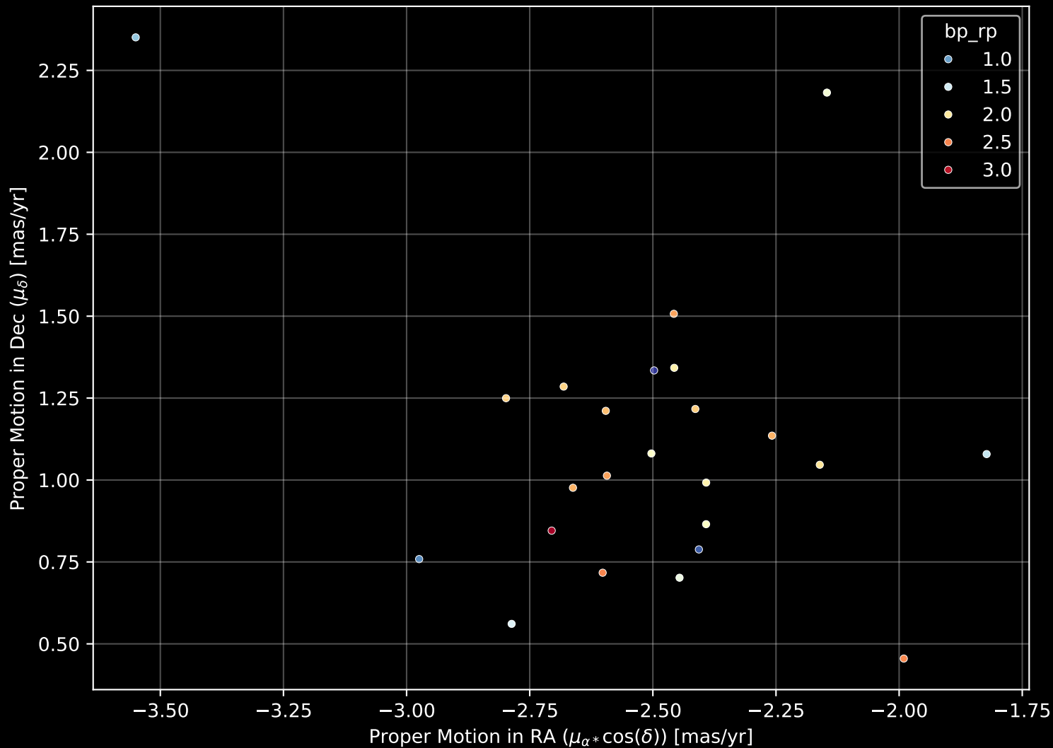
Gaia Cluster: [BDSB93] Proper Motion Diagram (n= 24)
