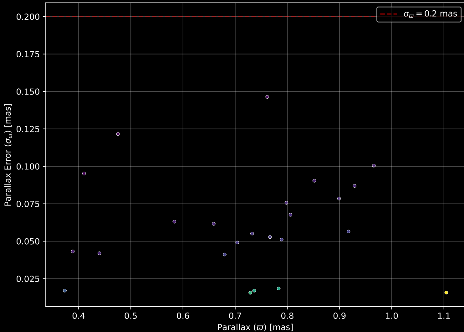
Gaia Cluster: [BDSB93] Parallax Quality (n= 24)
