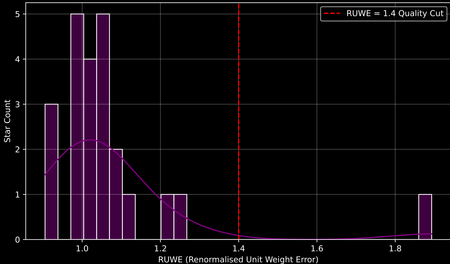
Gaia Cluster: [BDSB93] RUWE Distribution (n= 23)
