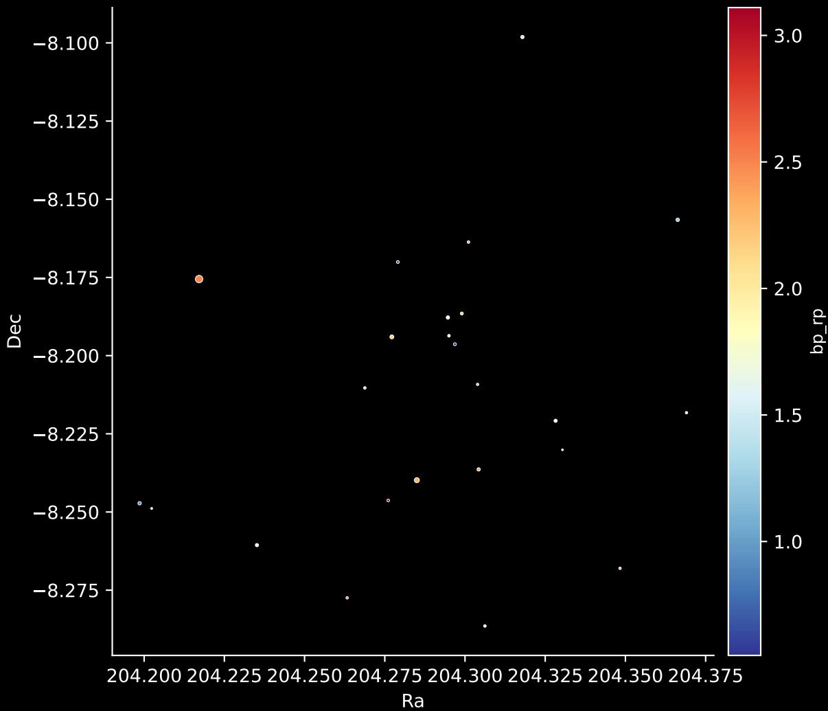
Gaia Cluster: [BDSB93] Stars: 24
