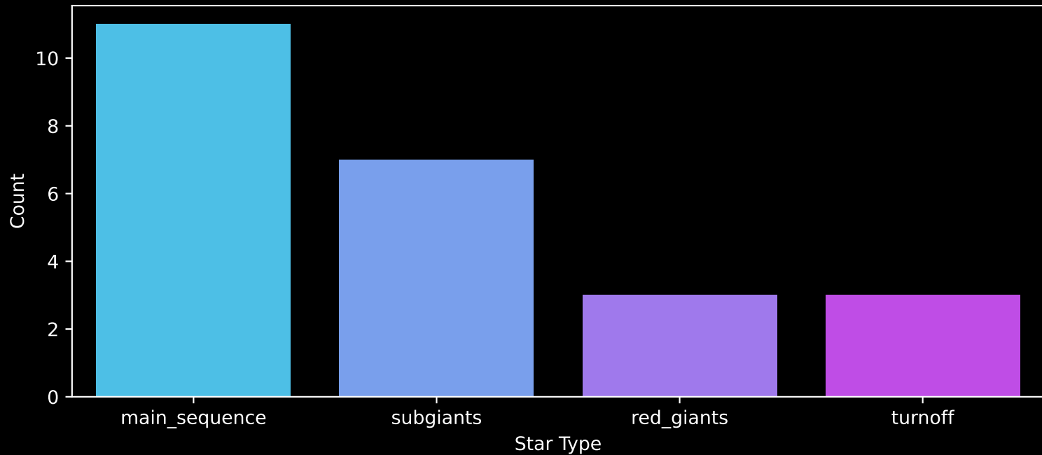
Gaia Cluster: [BDSB93] Count plot of Star Type
