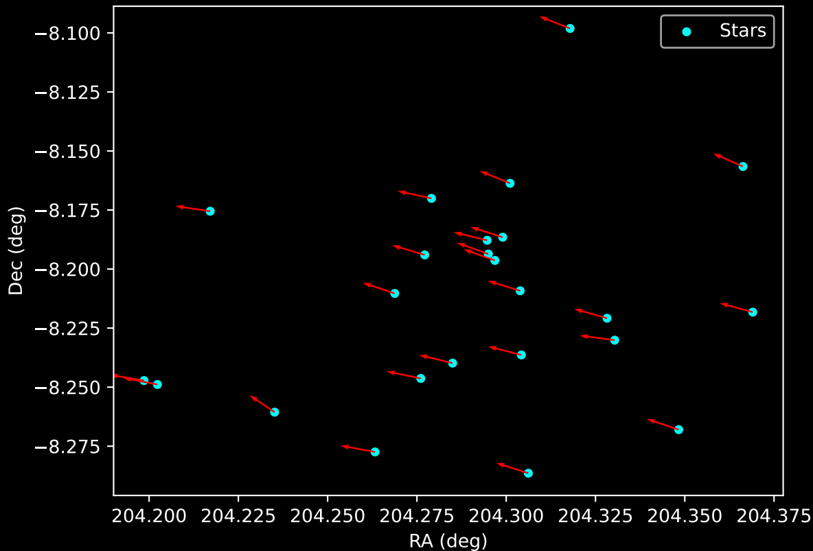
Gaia Cluster: [BDSB93] Proper Motion Vectors for Gaia Star Field (n= 24)
