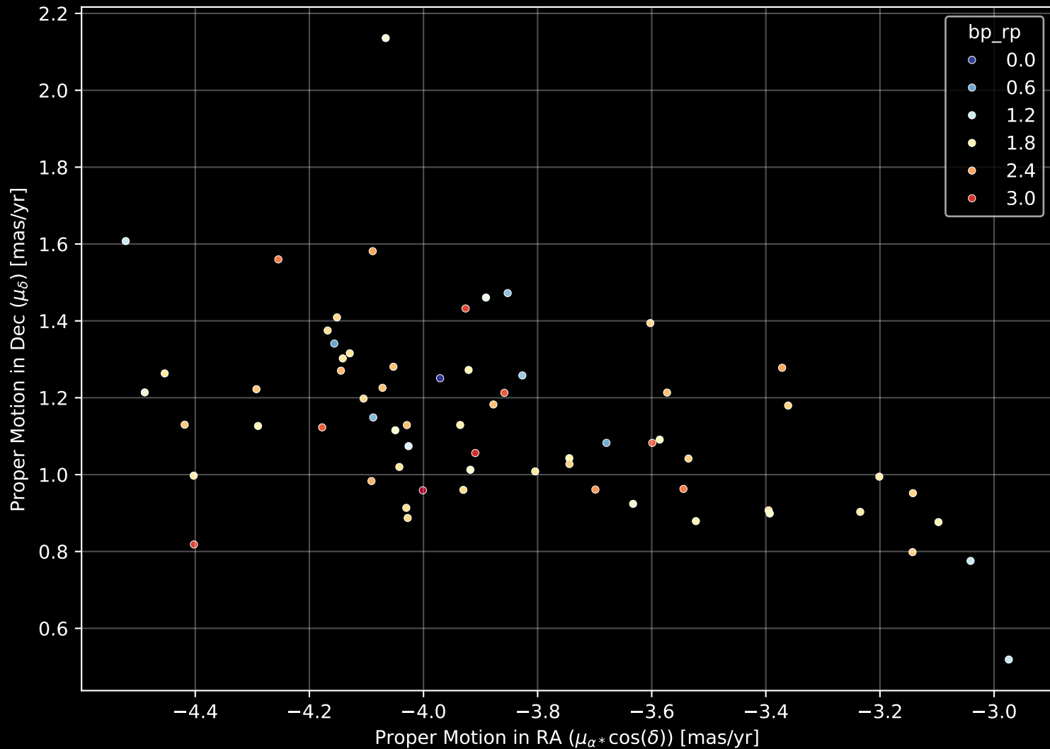
Gaia Cluster: [BDSB96] Proper Motion Diagram (n= 66)
