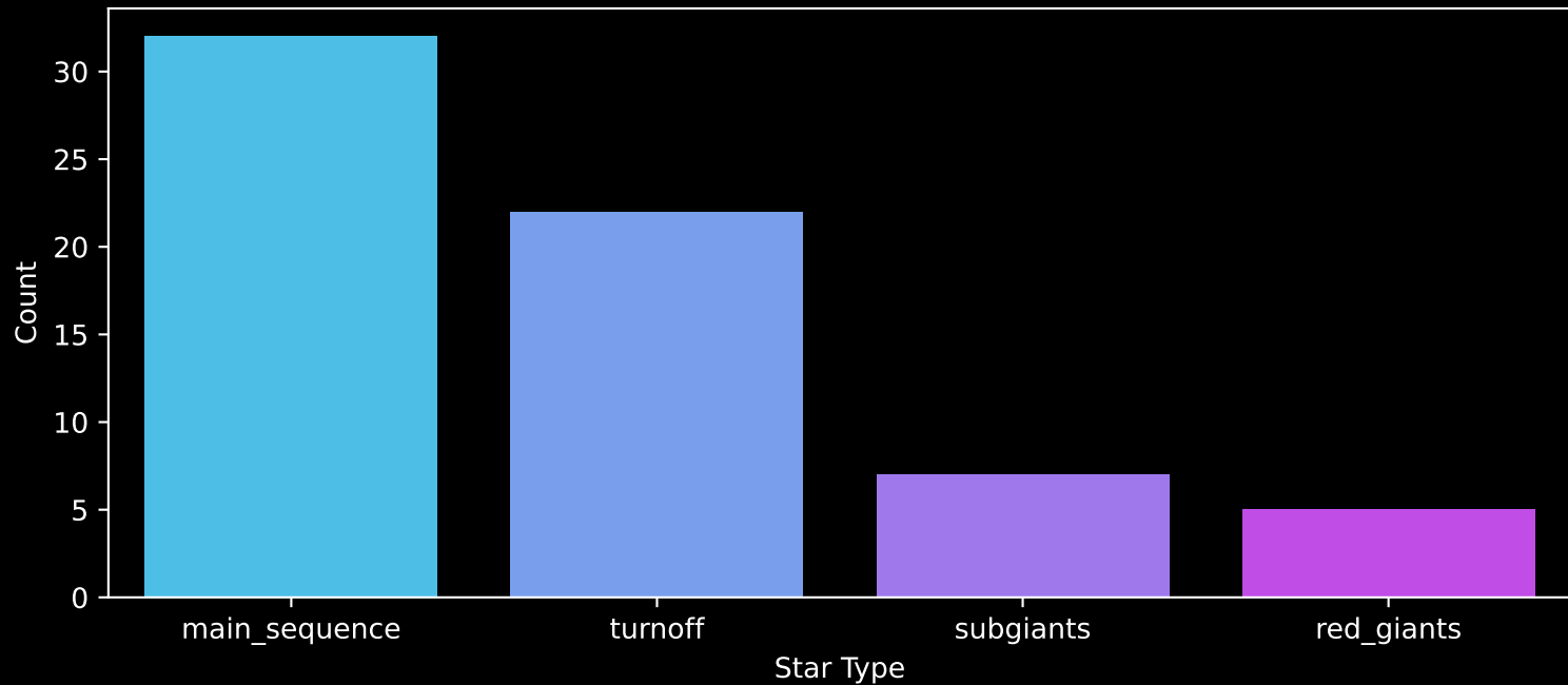
Gaia Cluster: [BDSB96] Count plot of Star Type
