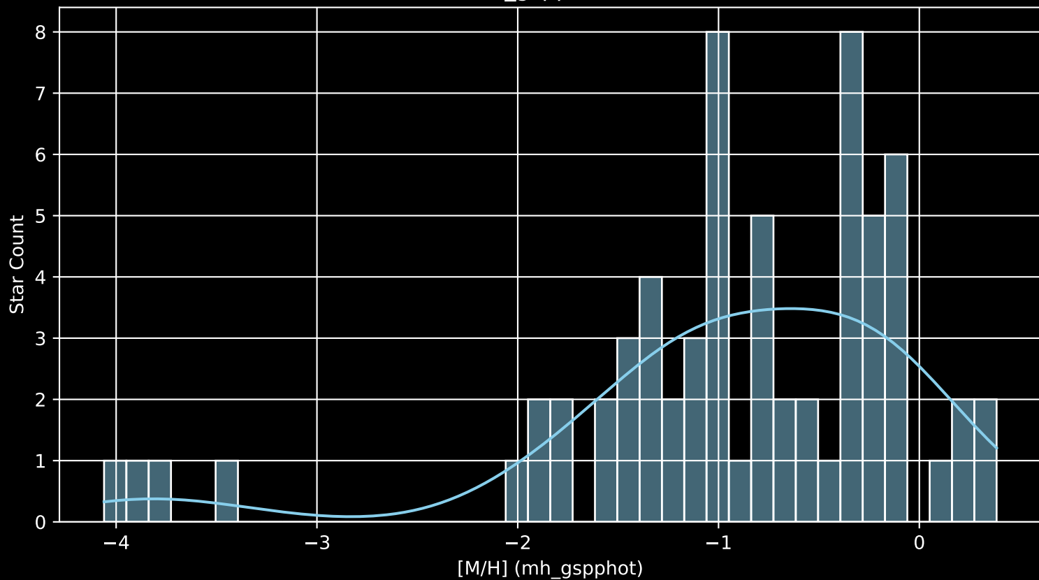
Gaia Cluster: [BDSB96 [M/H] (mh_gspphot) (n= 66)
