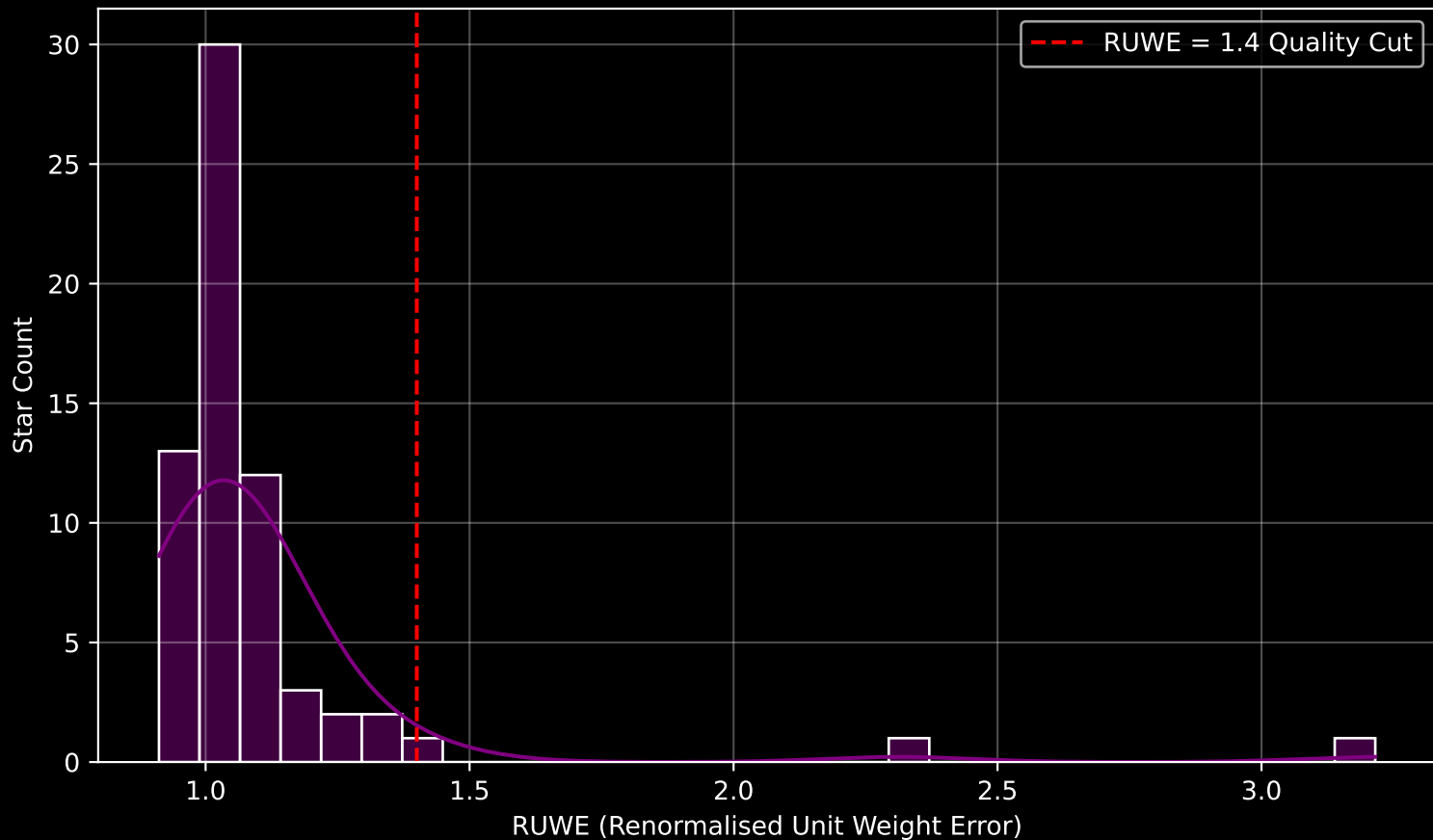
Gaia Cluster: [BDSB96] RUWE Distribution (n= 65)
