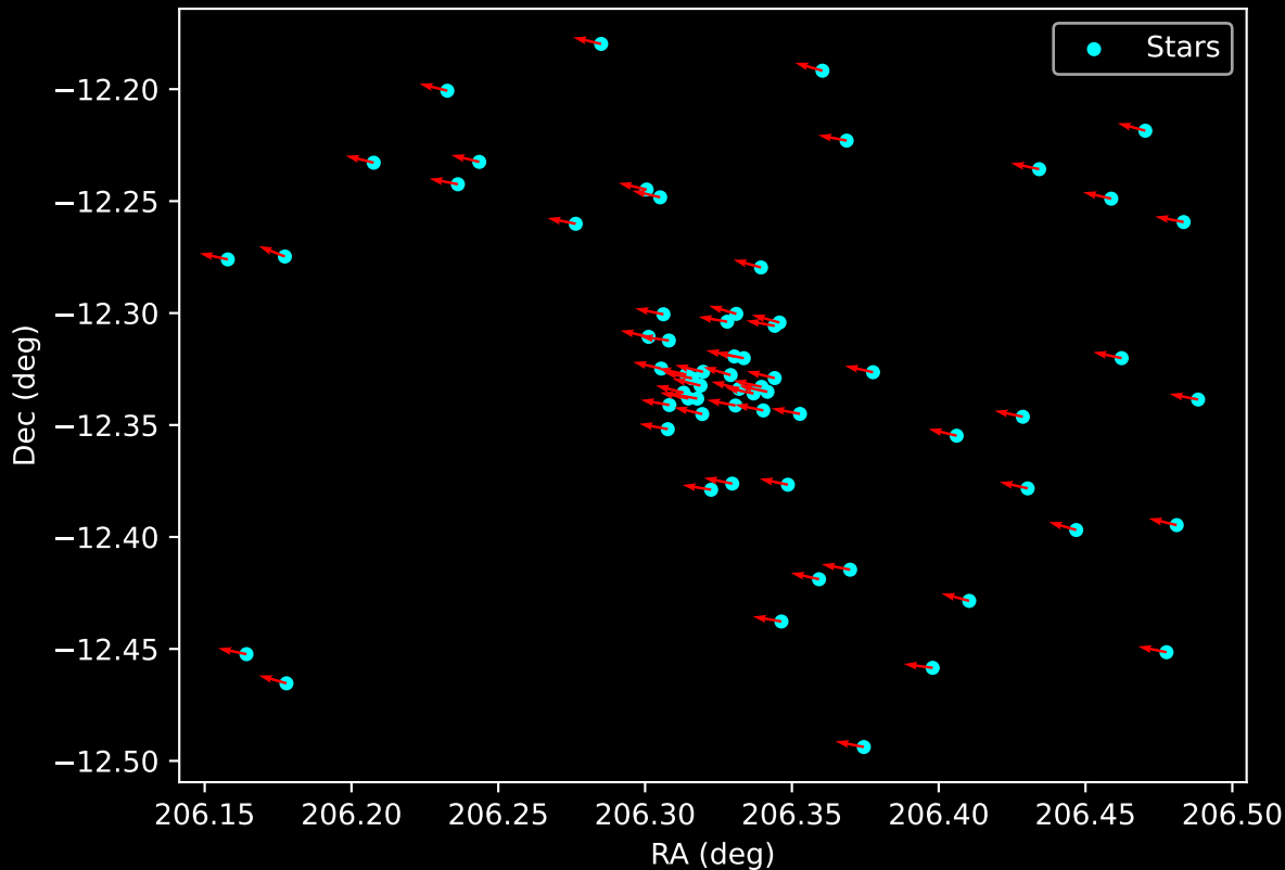
Gaia Cluster: [BDSB96] Proper Motion Vectors for Gaia Star Field (n= 66)
