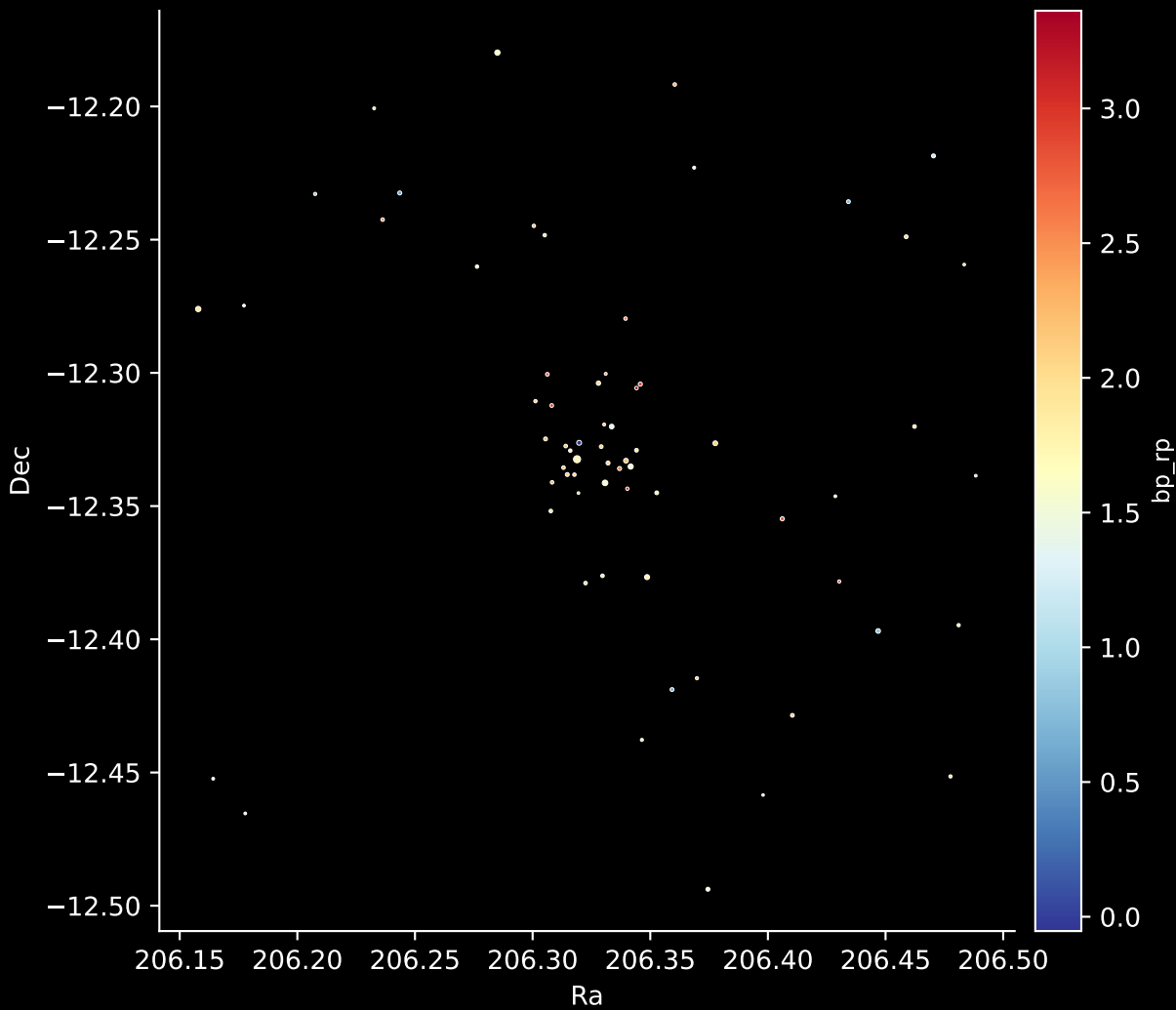
Gaia Cluster: [BDSB96] Stars: 66
