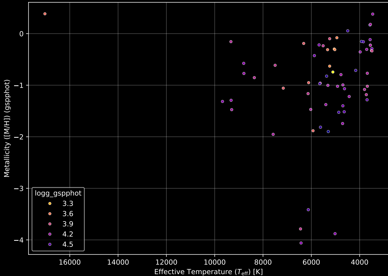
Gaia Cluster: [BDSB96] Stellar Population Parameters (n= 66)
