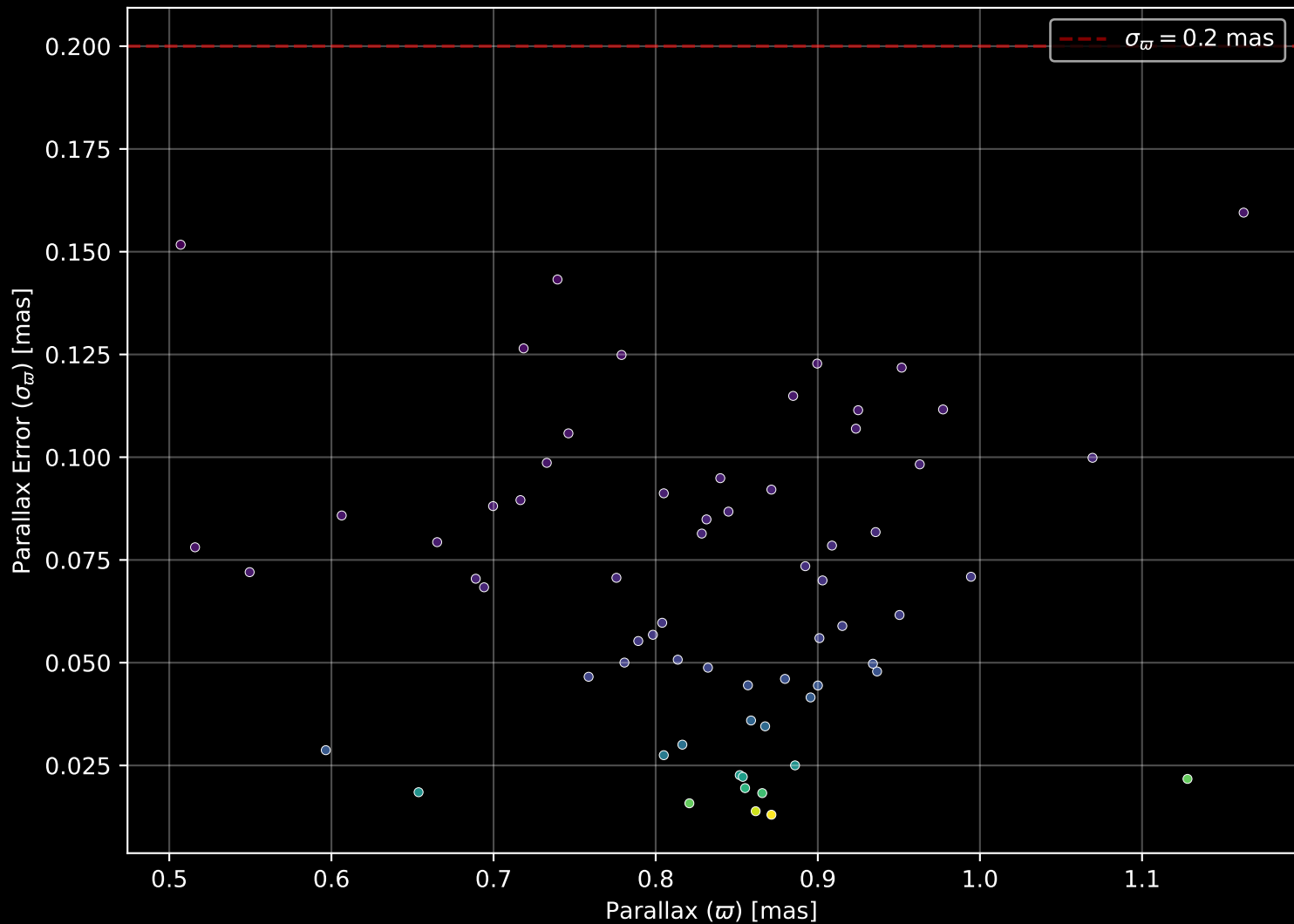
Gaia Cluster: [BDSB96] Parallax Quality (n= 66)
