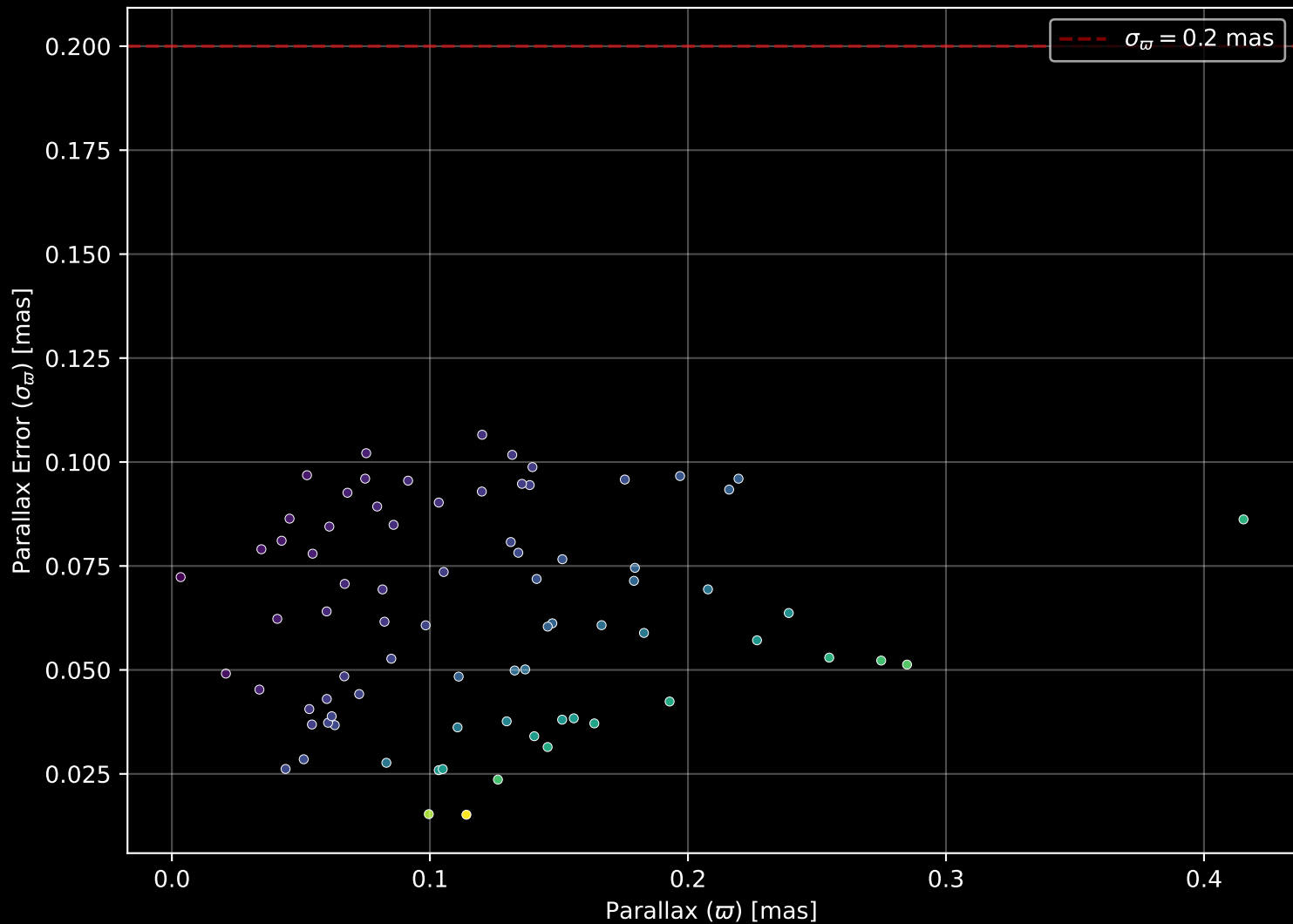
Gaia Cluster: [BH_118] Parallax Quality (n= 78)
