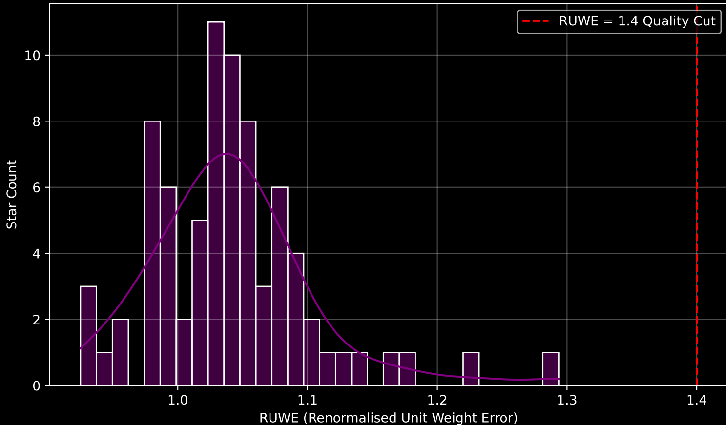
Gaia Cluster: [BH_118] RUWE Distribution (n= 78)
