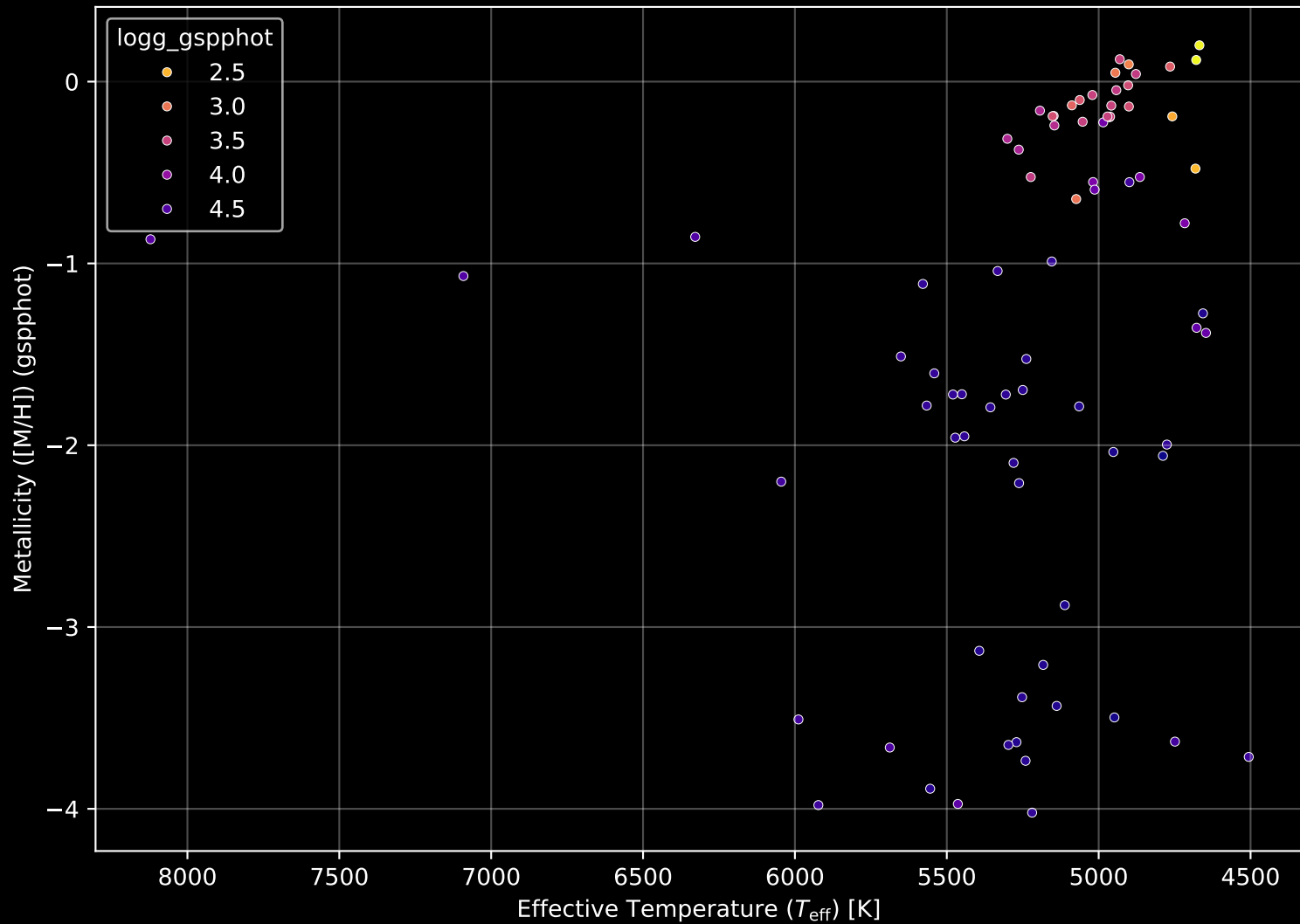
Gaia Cluster: [BH_118] Stellar Population Parameters (n= 78)
