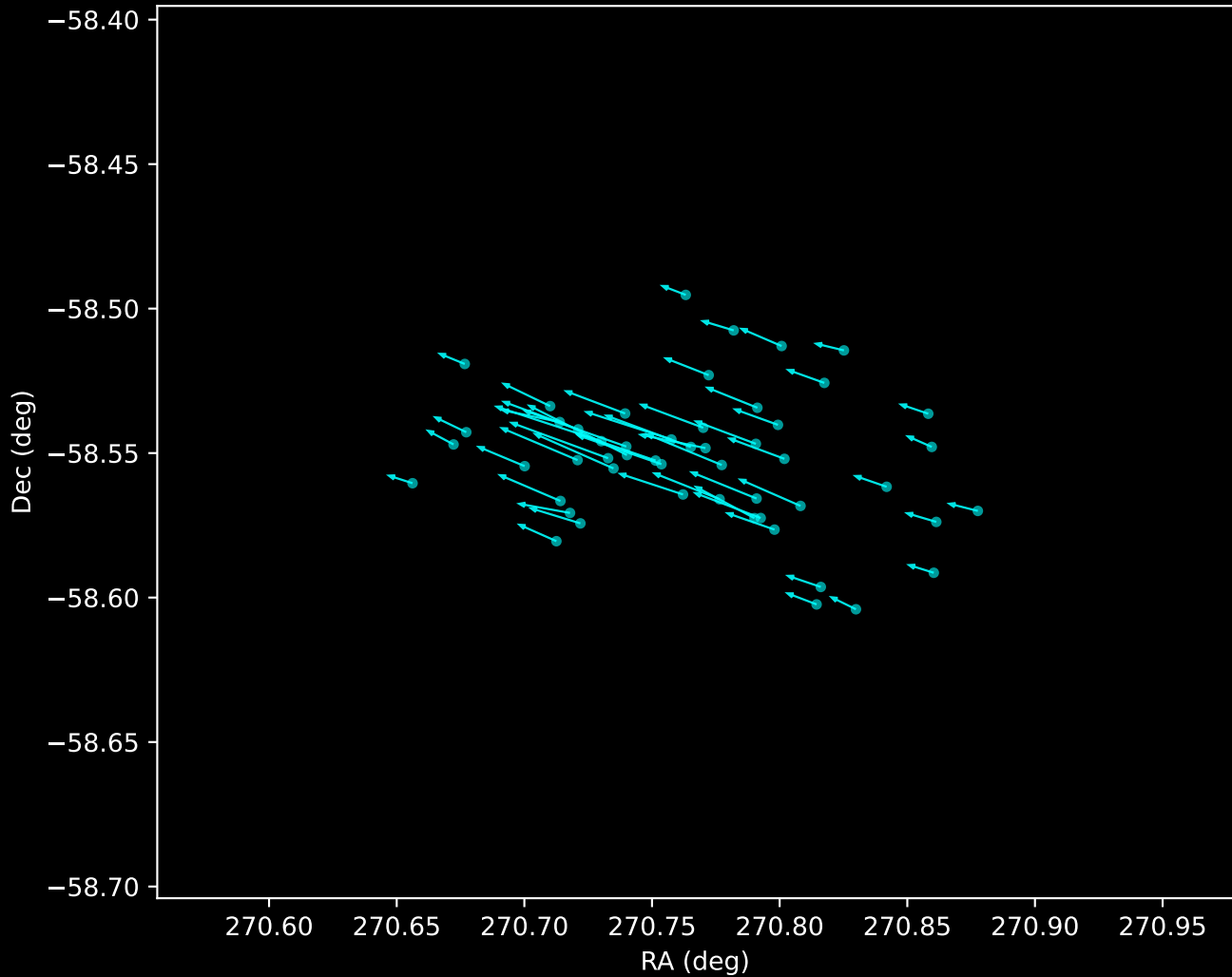
Gaia DR3 Noise Stream Proper Motion Vectors (n=52)
