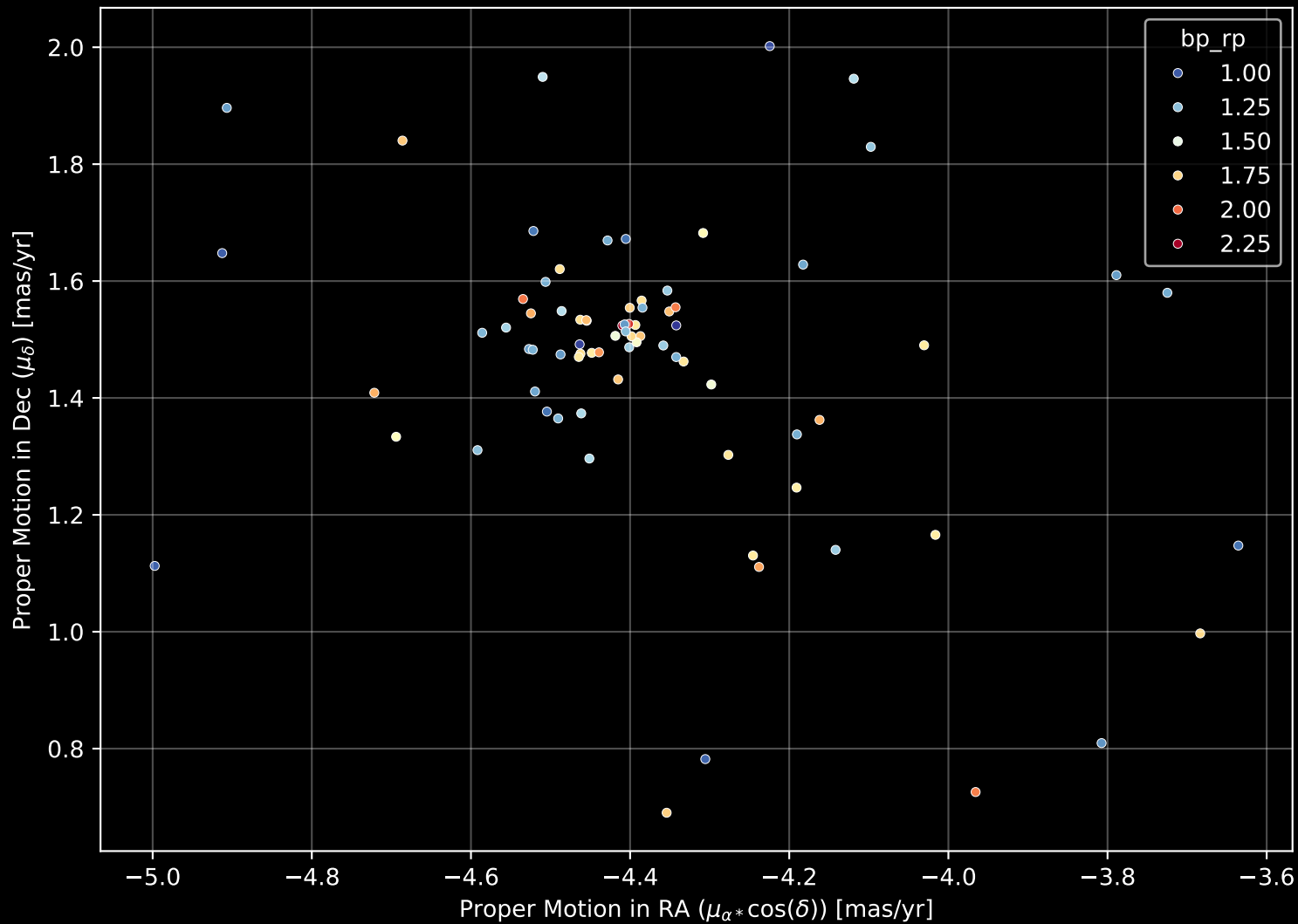
Gaia Cluster: [BH_118] Proper Motion Diagram (n= 78)
