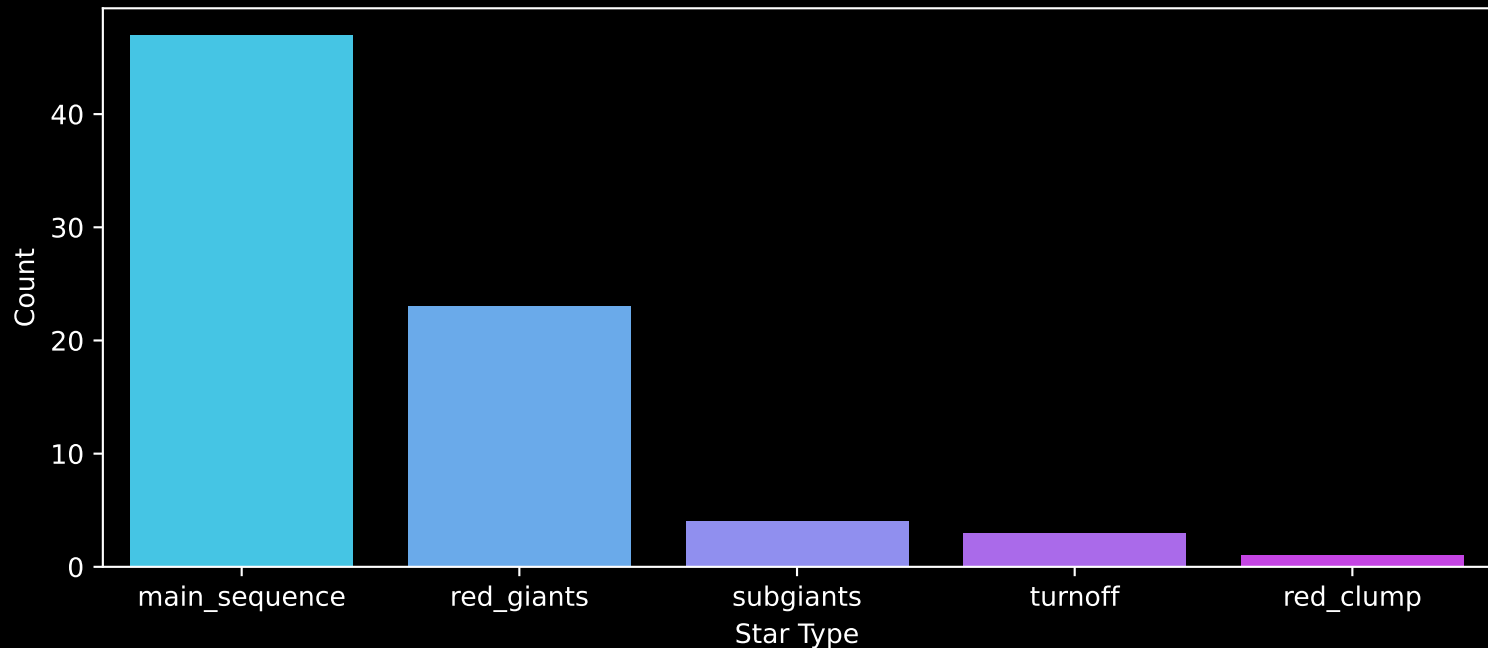
Gaia Cluster: [BH_118] Count plot of Star Type
