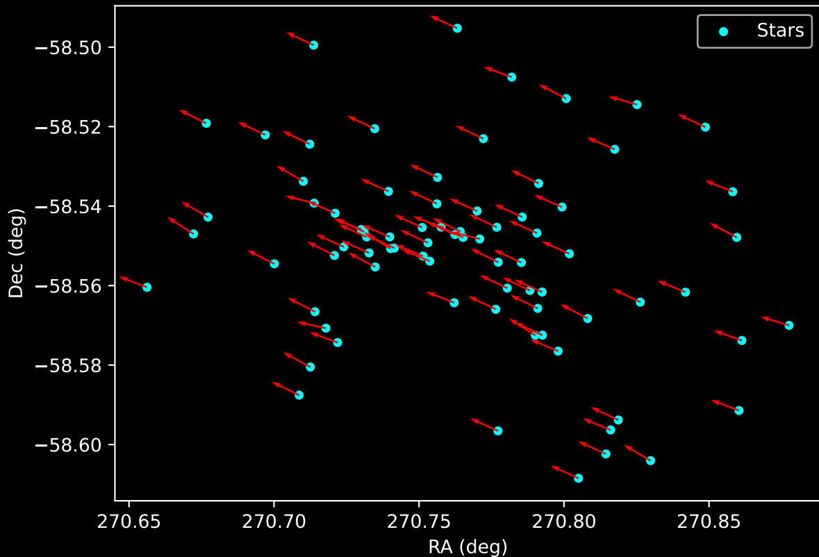
Gaia Cluster: [BH_118] Proper Motion Vectors for Gaia Star Field (n= 78)
