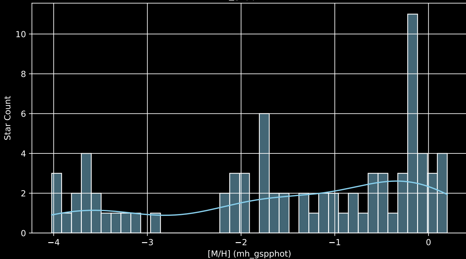
Gaia Cluster: [BH_118 [M/H] (mh_gspphot) (n= 78)
