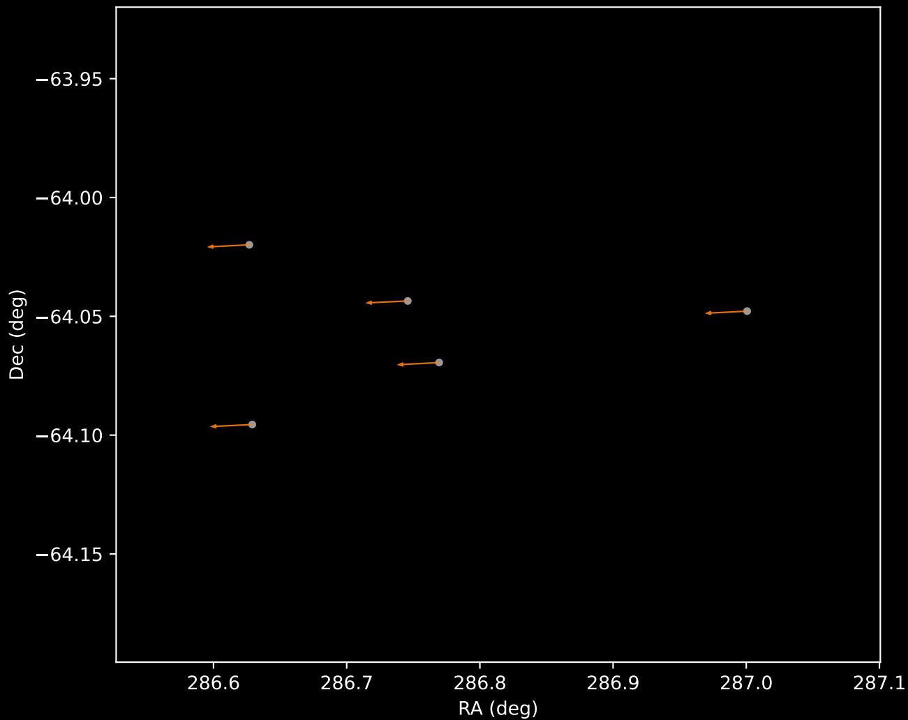
Gaia DR3 Cluster 2 Proper Motion Vectors (n=5)
