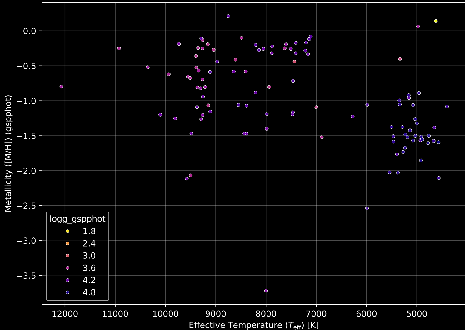
Gaia Cluster: [BH_132] Stellar Population Parameters (n= 108)
