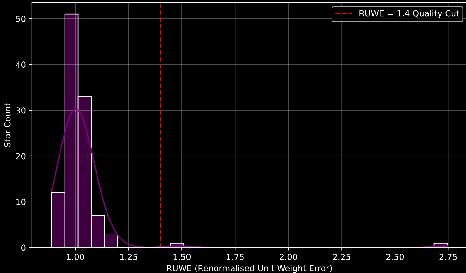
Gaia Cluster: [BH_132] RUWE Distribution (n= 108)
