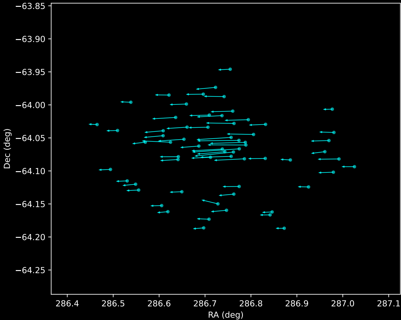
Gaia DR3 Noise Stream Proper Motion Vectors (n=64)
