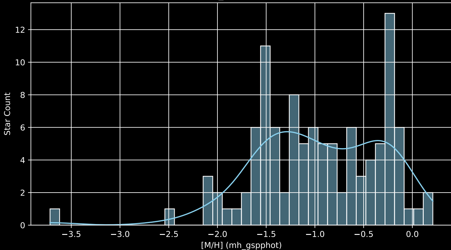
Gaia Cluster: [BH_132 [M/H] (mh_gspphot) (n= 108)
