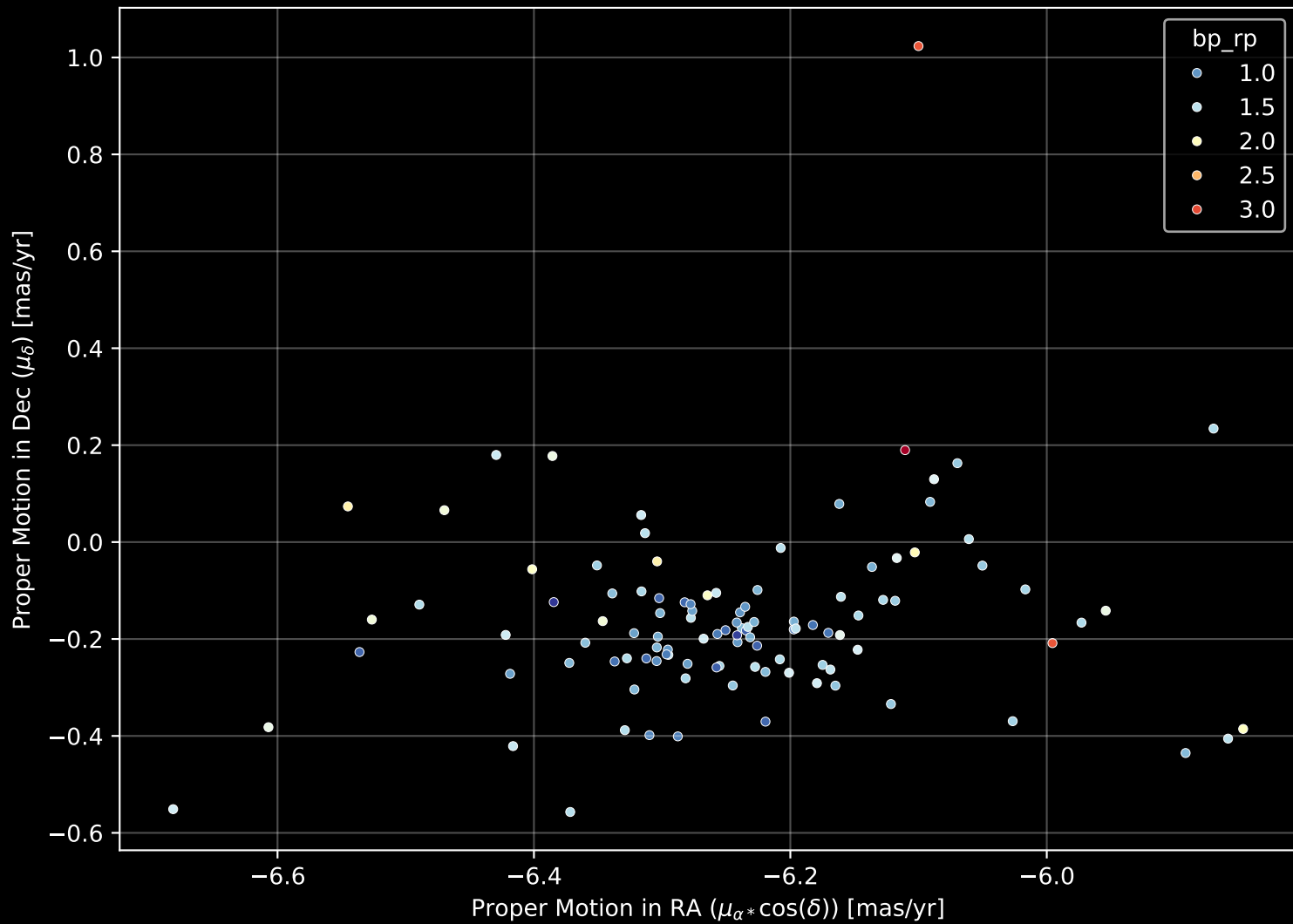
Gaia Cluster: [BH_132] Proper Motion Diagram (n= 108)
