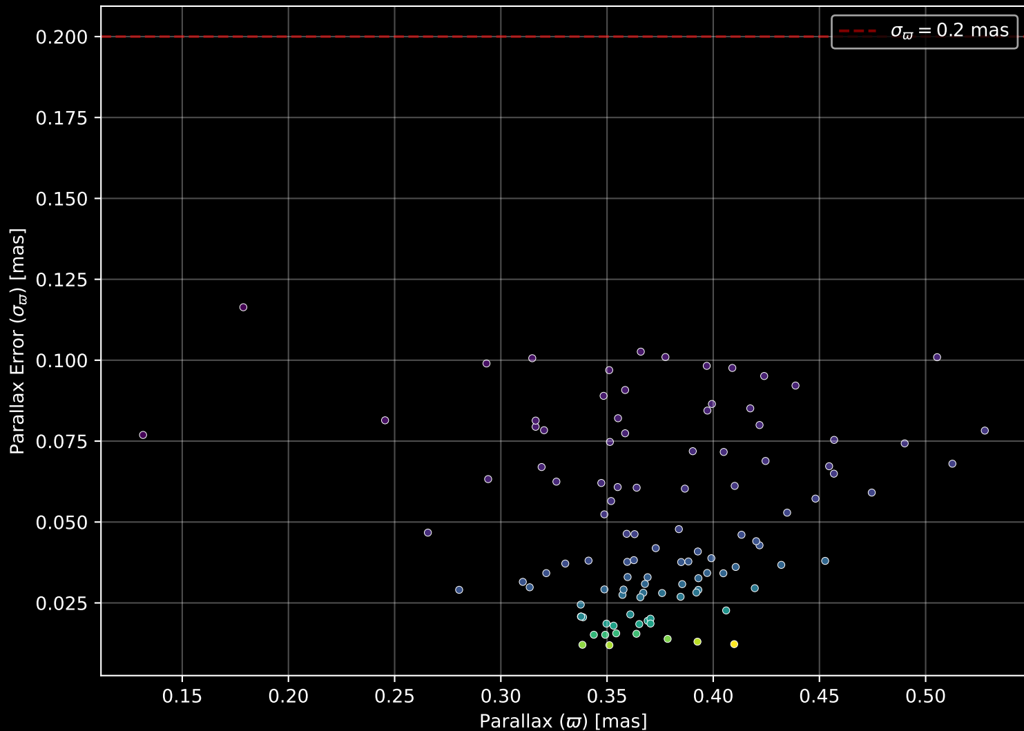
Gaia Cluster: [BH_132] Parallax Quality (n= 108)
