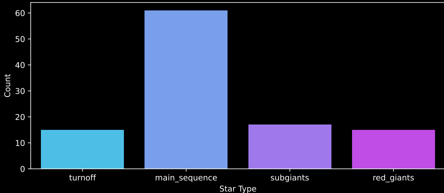
Gaia Cluster: [BH_132] Count plot of Star Type
