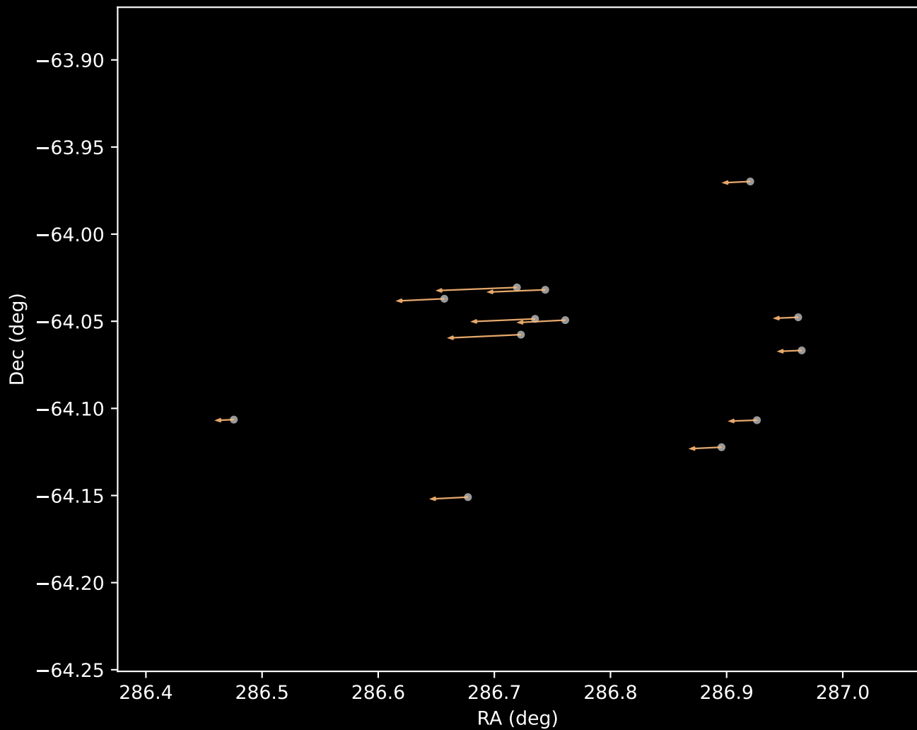
Gaia DR3 Cluster 3 Proper Motion Vectors (n=13)
