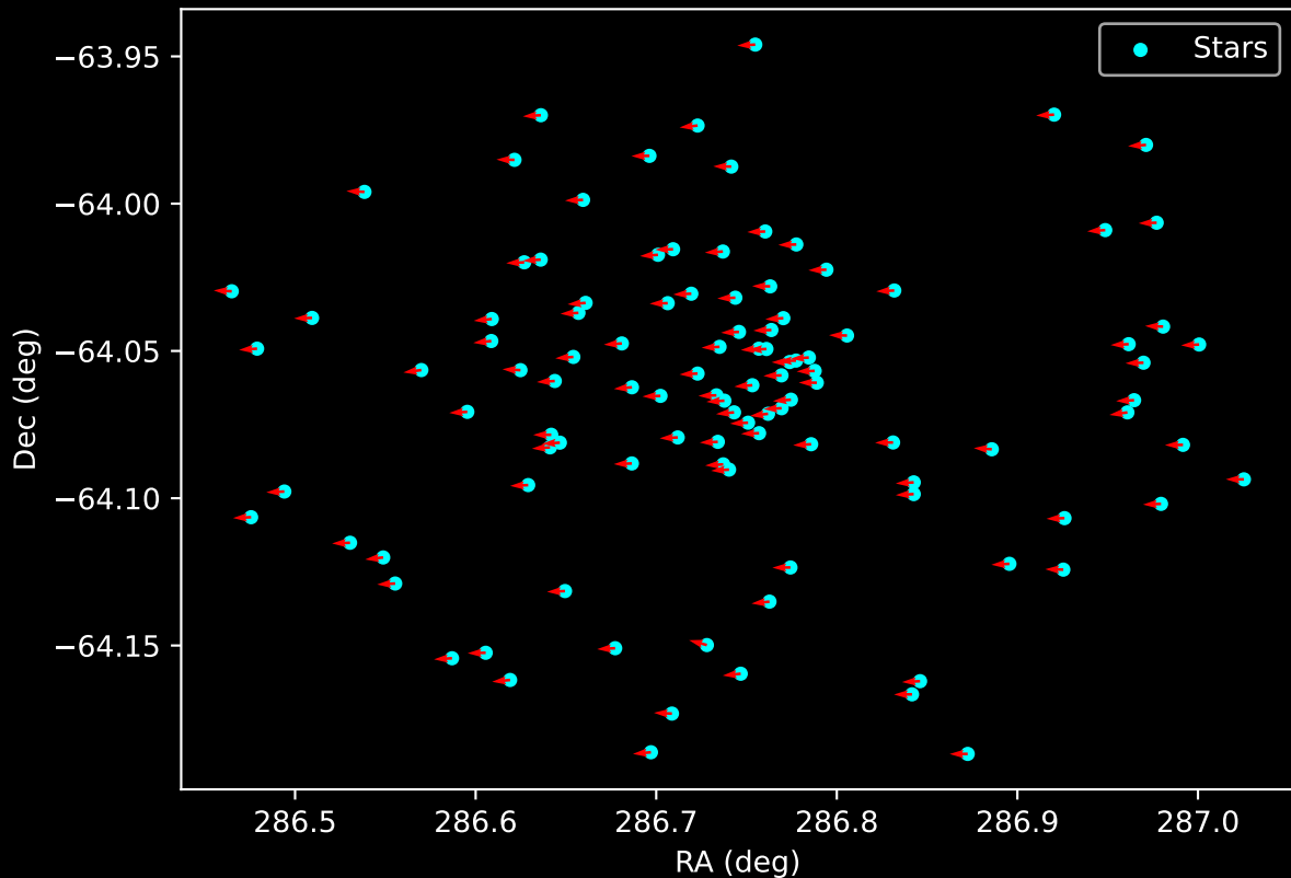
Gaia Cluster: [BH_132] Proper Motion Vectors for Gaia Star Field (n= 108)
