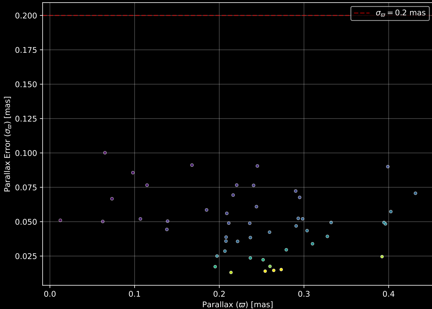
Gaia Cluster: [BH_151] Parallax Quality (n= 50)
