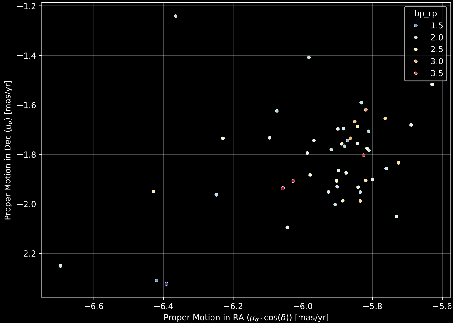
Gaia Cluster: [BH_151] Proper Motion Diagram (n= 50)
