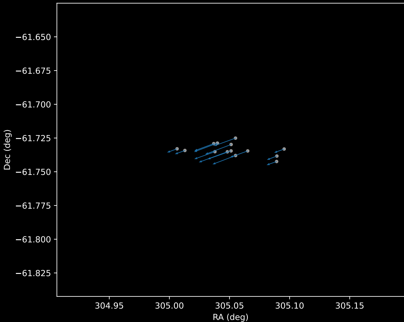
Gaia DR3 Cluster 0 Proper Motion Vectors (n=14)
