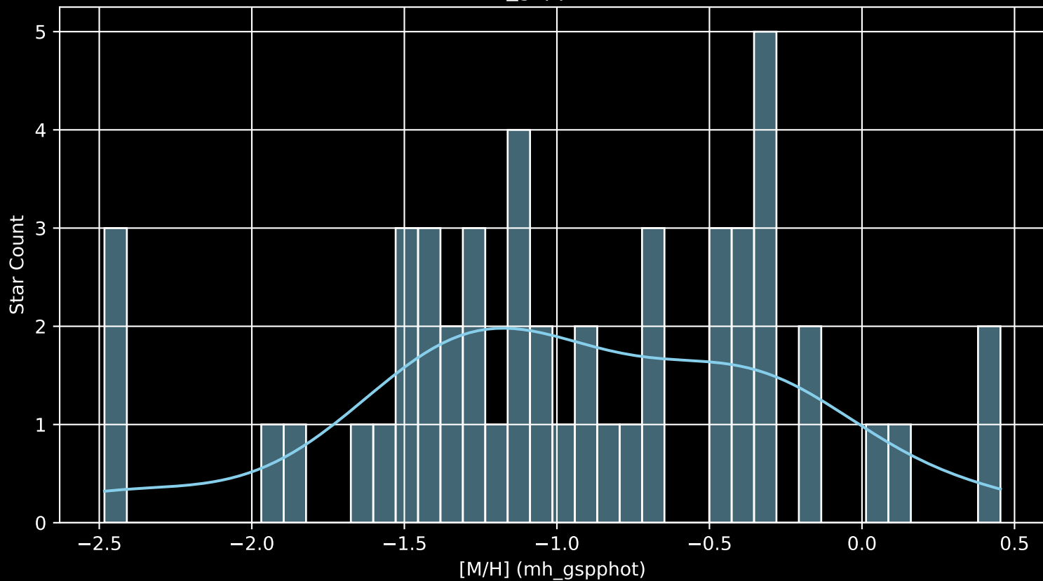
Gaia Cluster: [BH_151 [M/H] (mh_gspphot) (n= 50)
