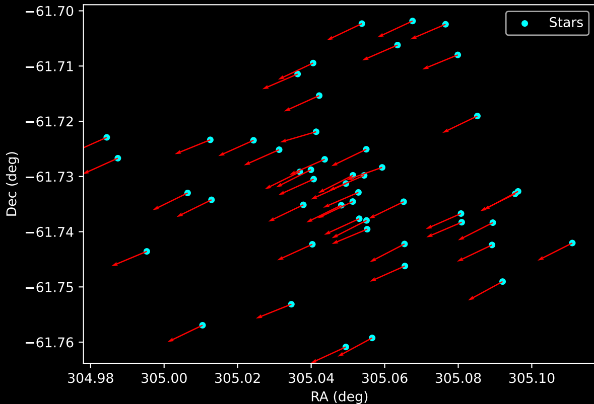
Gaia Cluster: [BH_151] Proper Motion Vectors for Gaia Star Field (n= 50)
