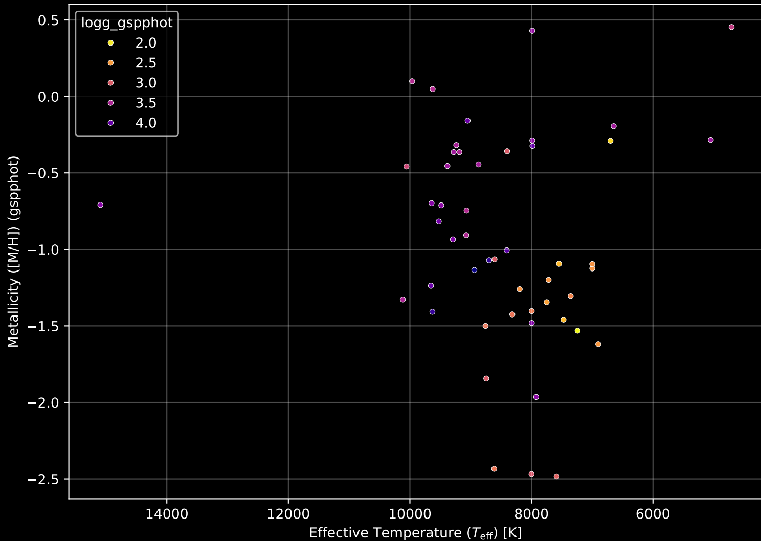
Gaia Cluster: [BH_151] Stellar Population Parameters (n= 50)
