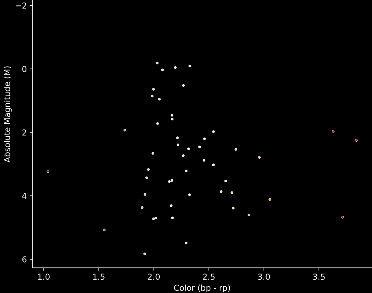
Gaia Cluster: [BH_151] Stars (n= 50) Hertzsprung-Russel Diagram
