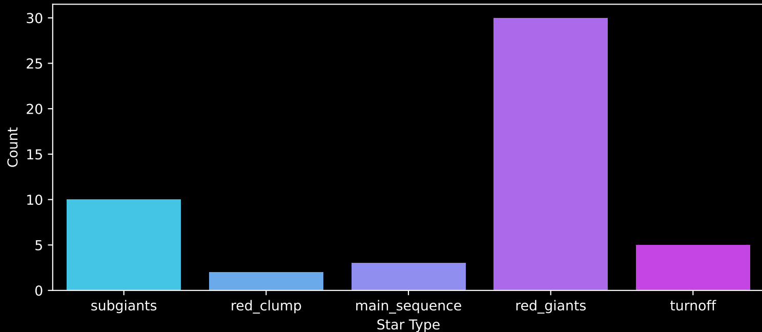
Gaia Cluster: [BH_151] Count plot of Star Type
