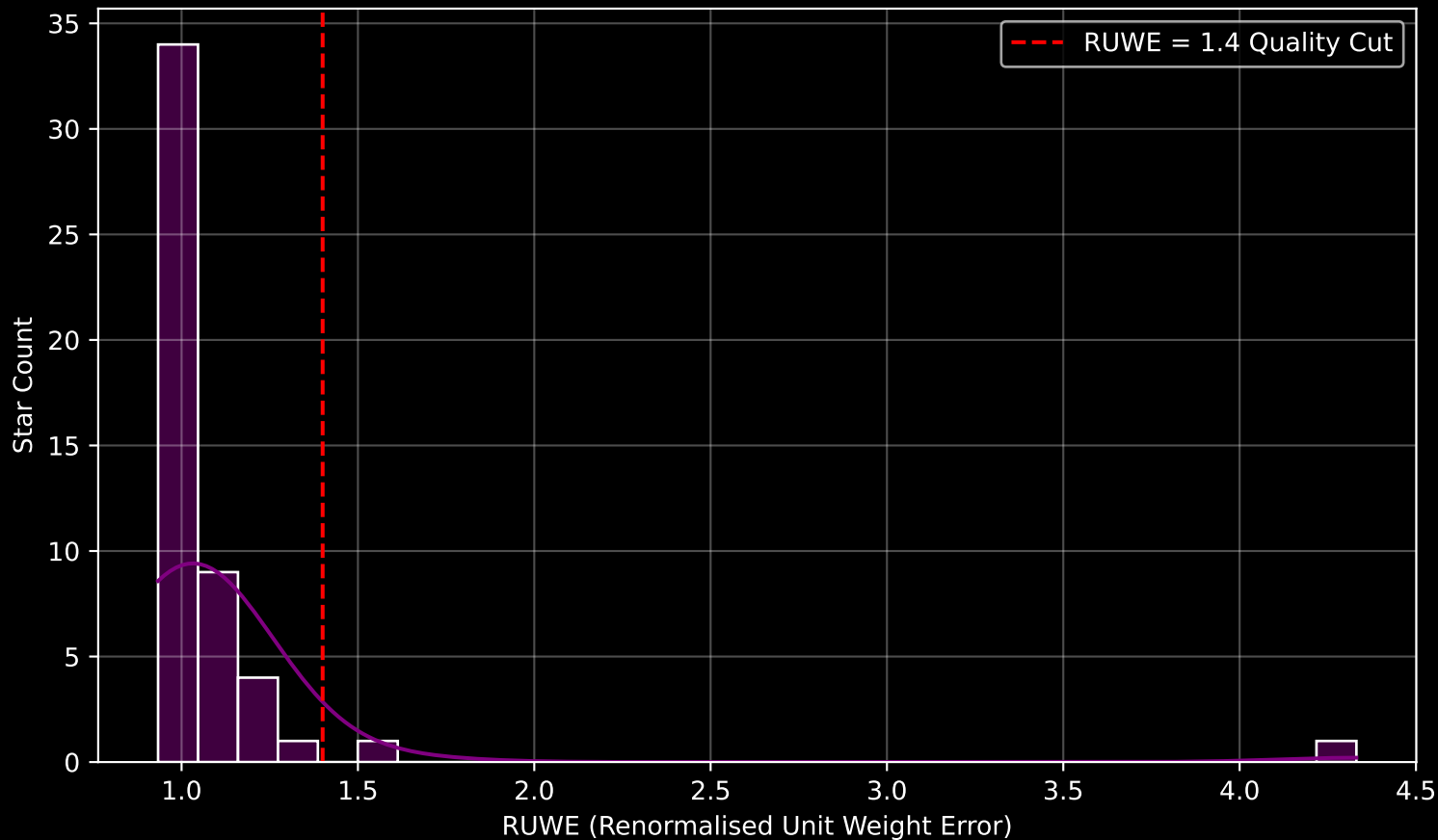
Gaia Cluster: [BH_151] RUWE Distribution (n= 50)
