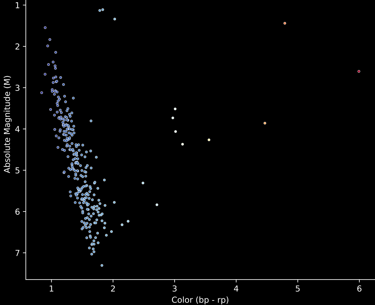
Gaia Cluster: [BH_202] Stars (n= 273) Hertzsprung-Russel Diagram
