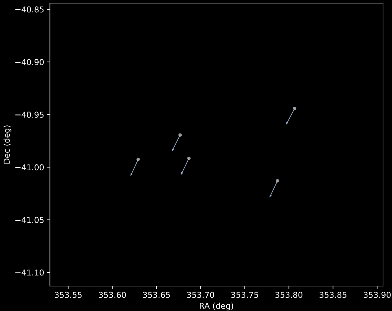
Gaia DR3 Cluster 1 Proper Motion Vectors (n=5)
