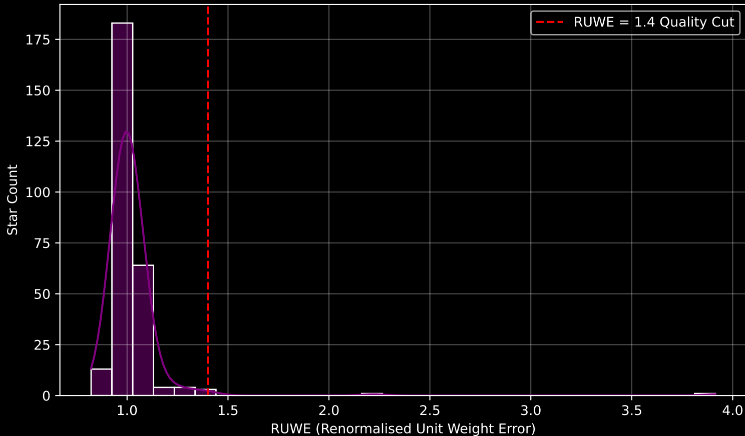
Gaia Cluster: [BH_202] RUWE Distribution (n= 273)
