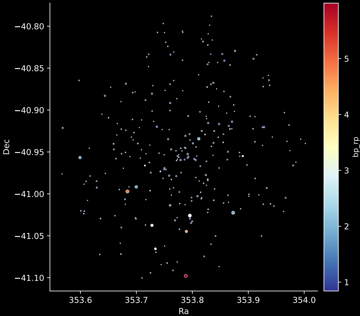
Gaia Cluster: [BH_202] Stars: 273
