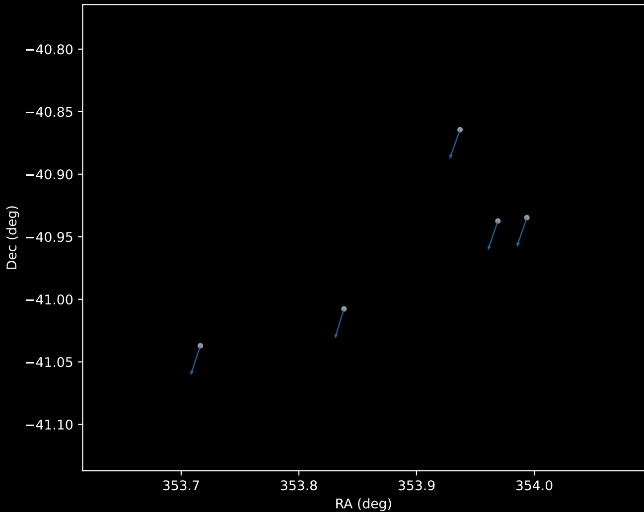
Gaia DR3 Cluster 0 Proper Motion Vectors (n=5)
