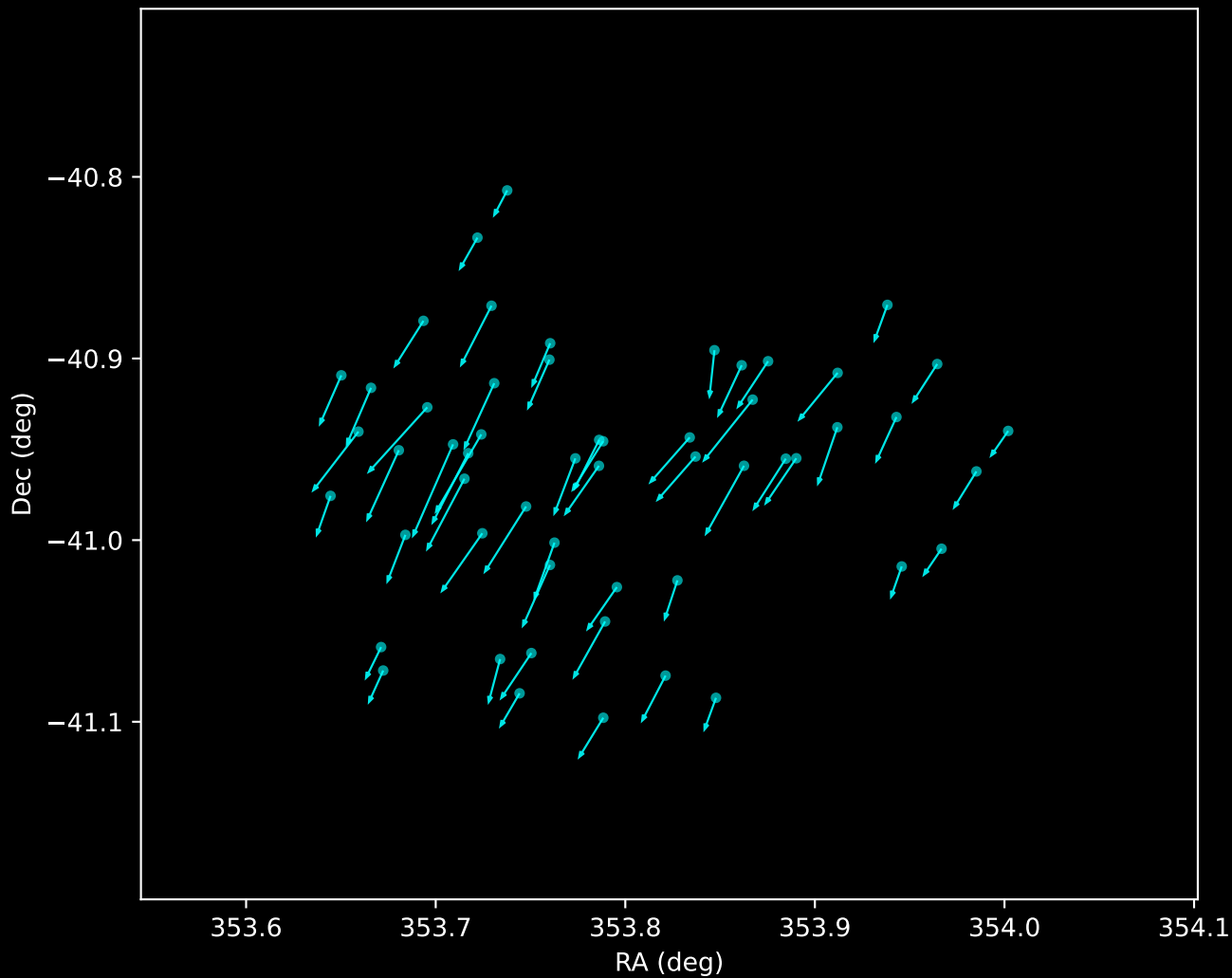
Gaia DR3 Noise Stream Proper Motion Vectors (n=55)
