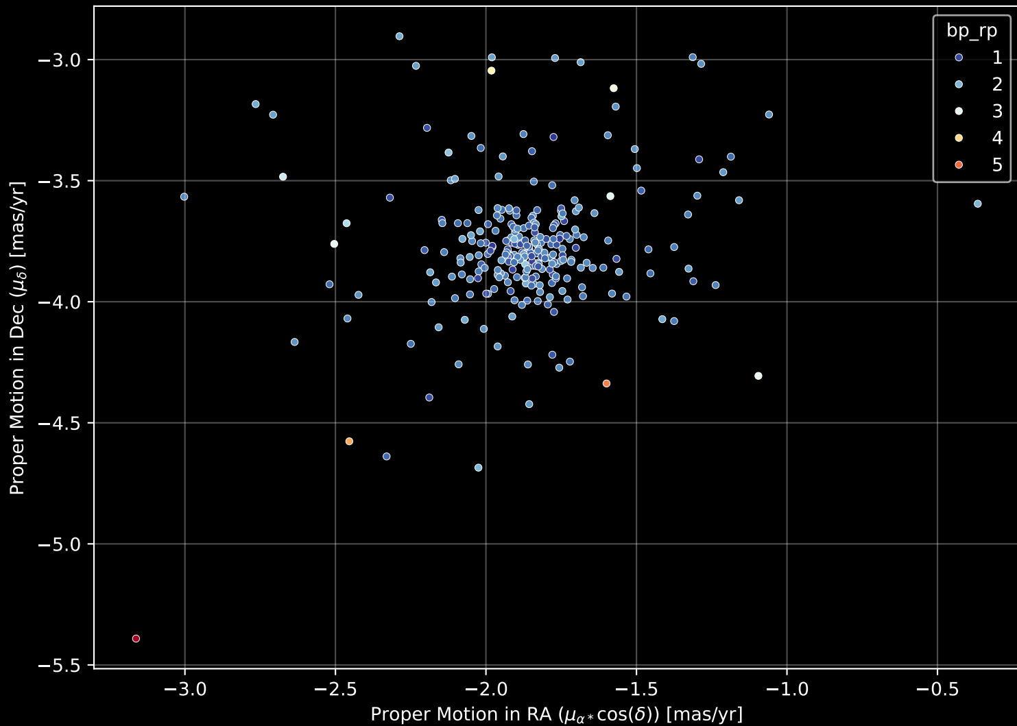
Gaia Cluster: [BH_202] Proper Motion Diagram (n= 273)
