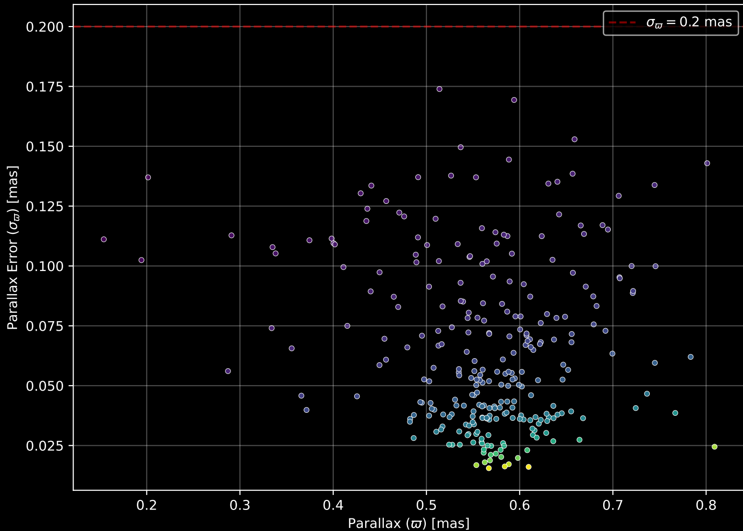
Gaia Cluster: [BH_202] Parallax Quality (n= 273)
