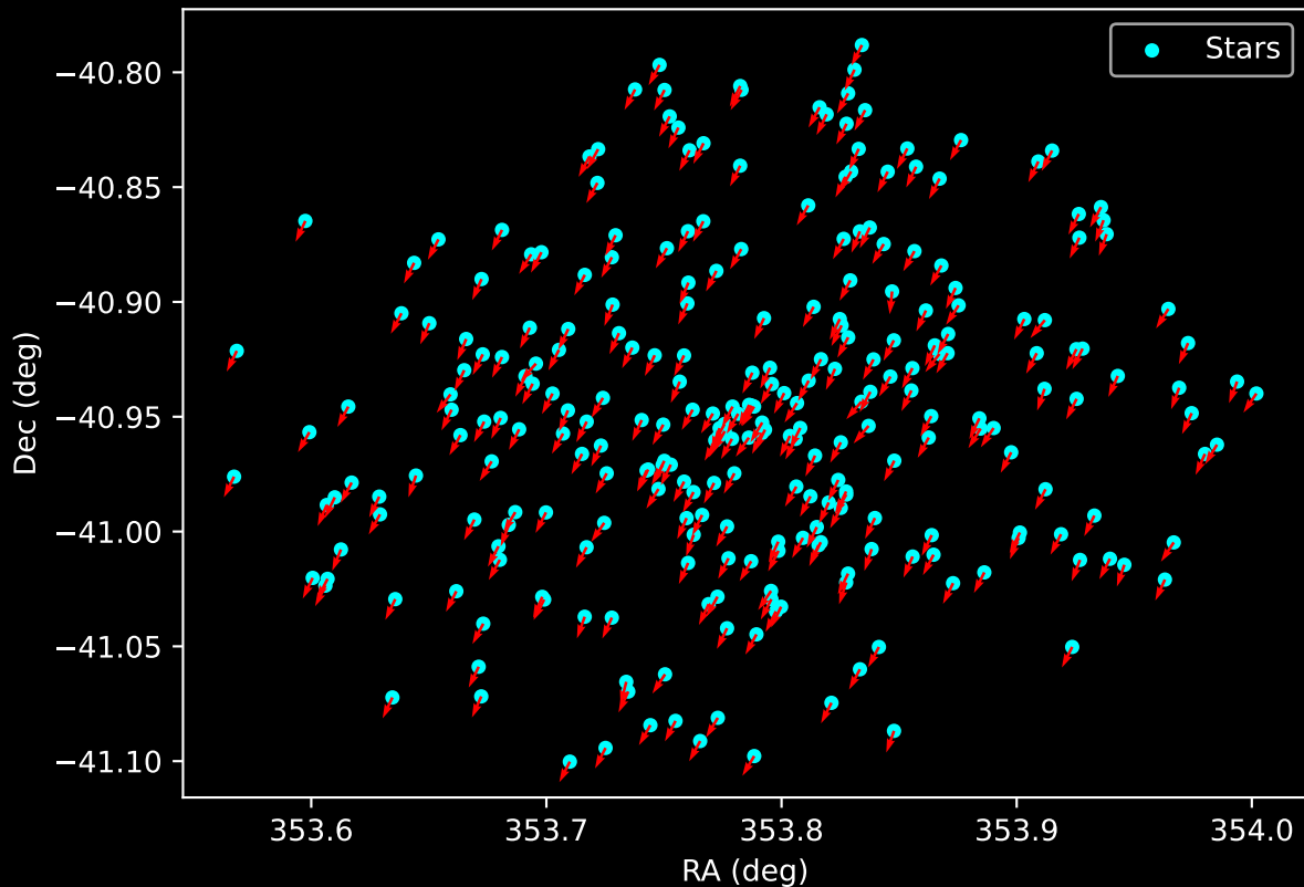
Gaia Cluster: [BH_202] Proper Motion Vectors for Gaia Star Field (n= 273)
