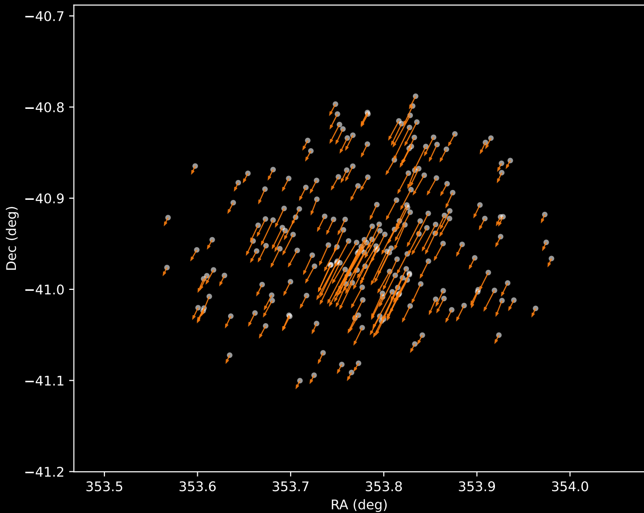
Gaia DR3 Cluster 2 Proper Motion Vectors (n=208)
