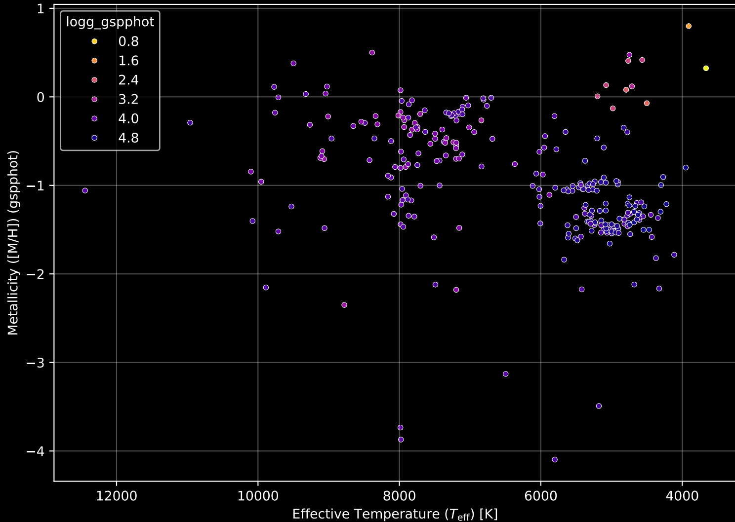
Gaia Cluster: [BH_202] Stellar Population Parameters (n= 273)
