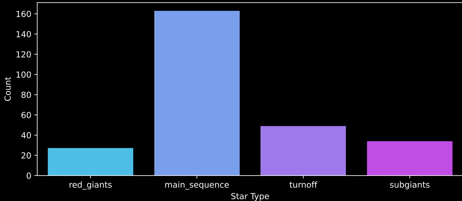
Gaia Cluster: [BH_202] Count plot of Star Type
