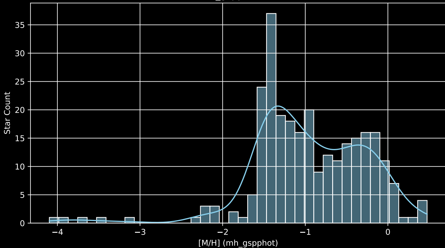
Gaia Cluster: [BH_202 [M/H] (mh_gspphot) (n= 271)
