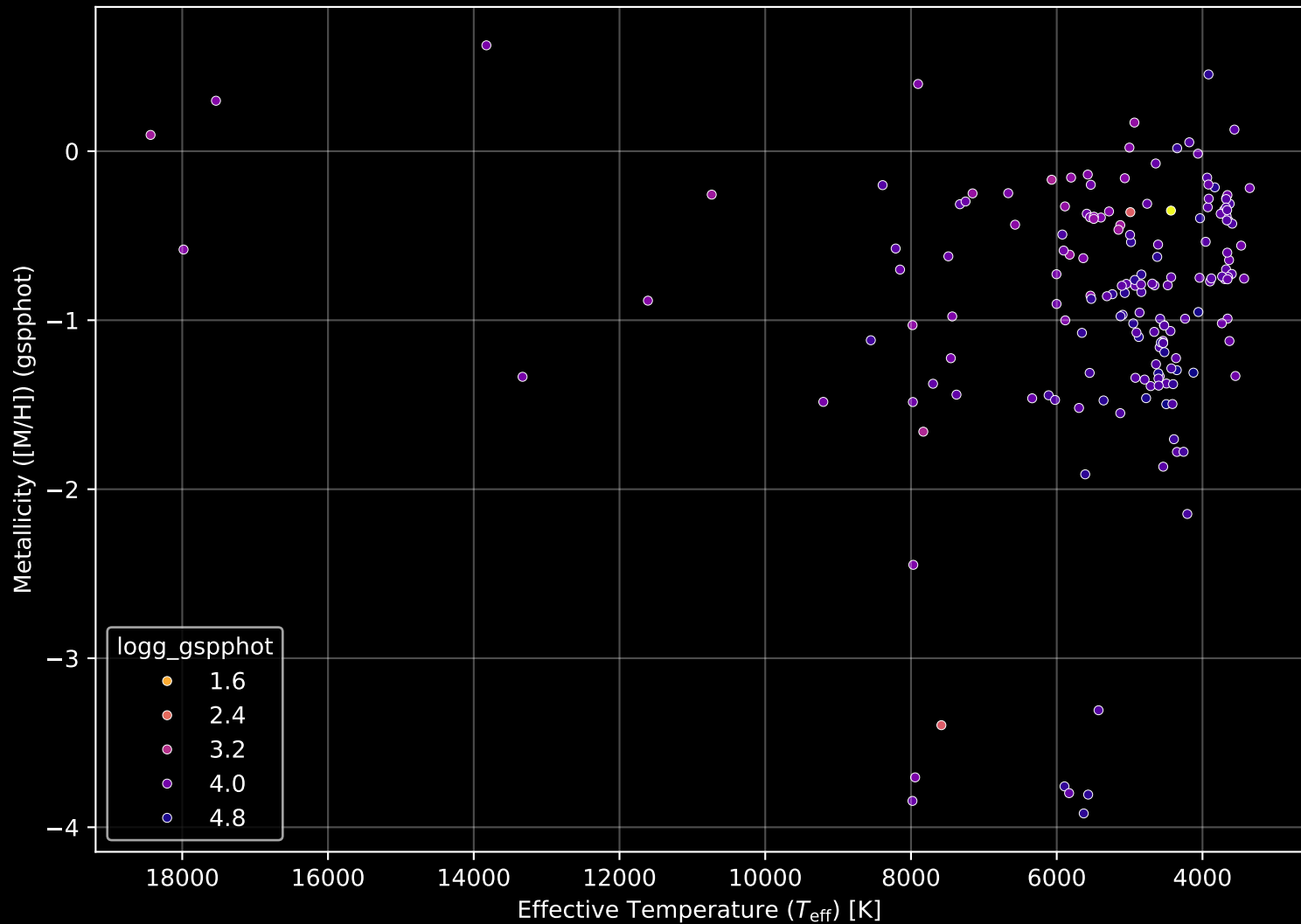
Gaia Cluster: [BH_221] Stellar Population Parameters (n= 175)
