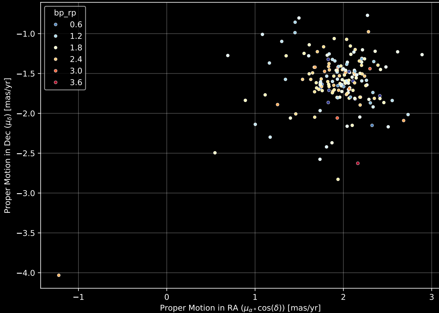
Gaia Cluster: [BH_221] Proper Motion Diagram (n= 175)
