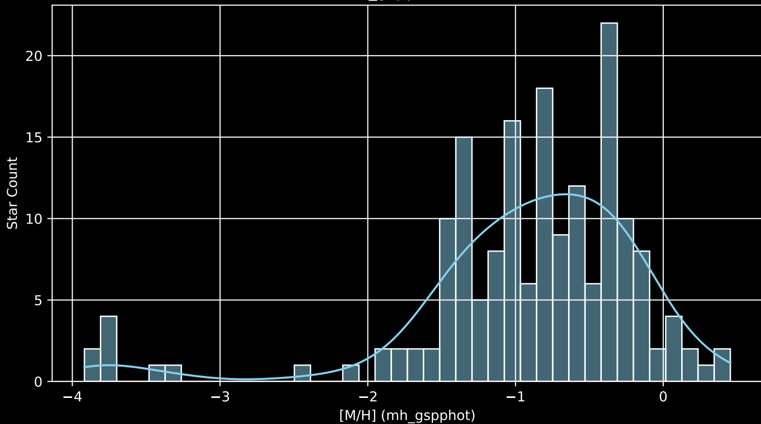
Gaia Cluster: [BH_221 [M/H] (mh_gspphot) (n= 174)
