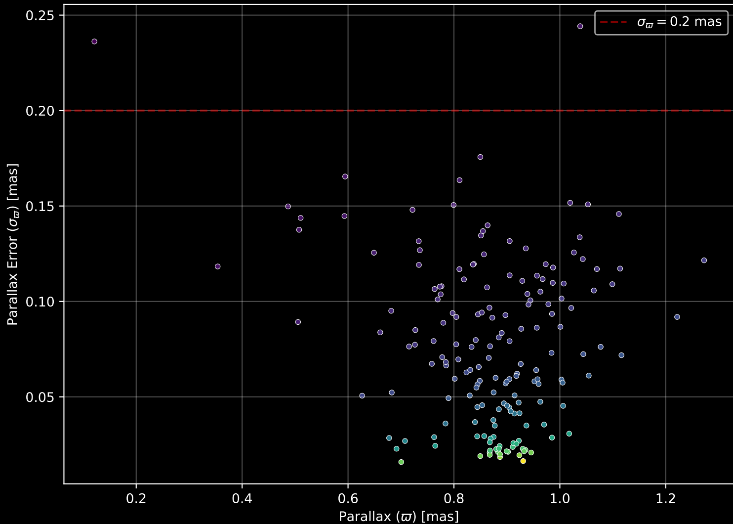
Gaia Cluster: [BH_221] Parallax Quality (n= 175)
