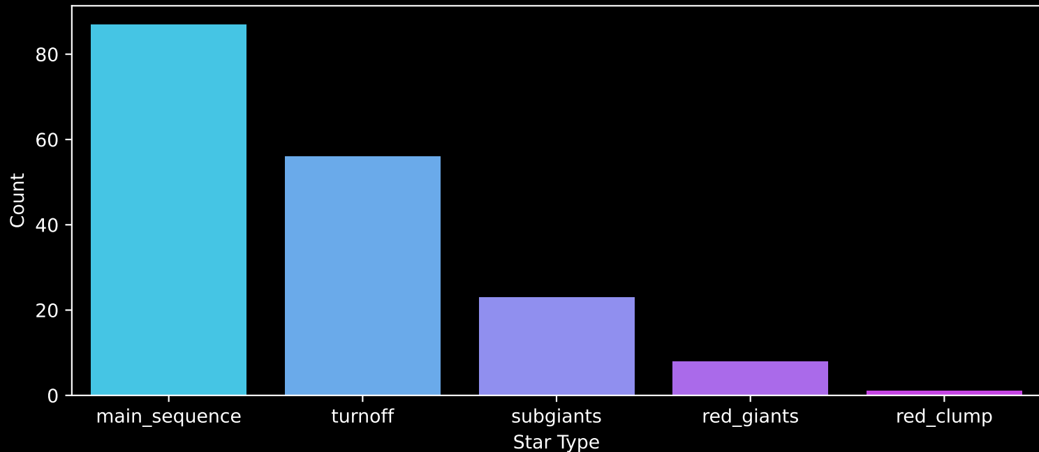
Gaia Cluster: [BH_221] Count plot of Star Type
