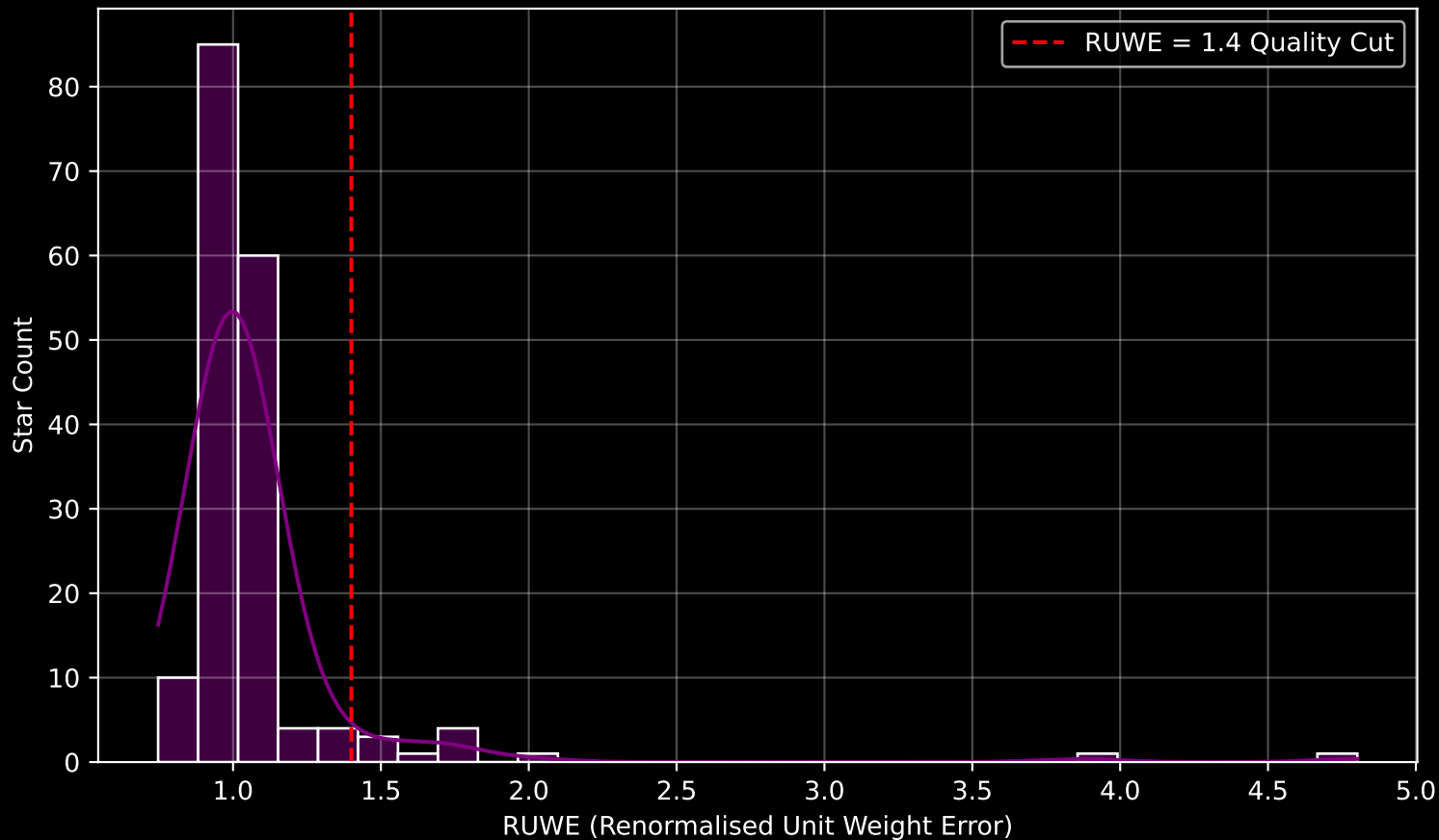
Gaia Cluster: [BH_221] RUWE Distribution (n= 174)
