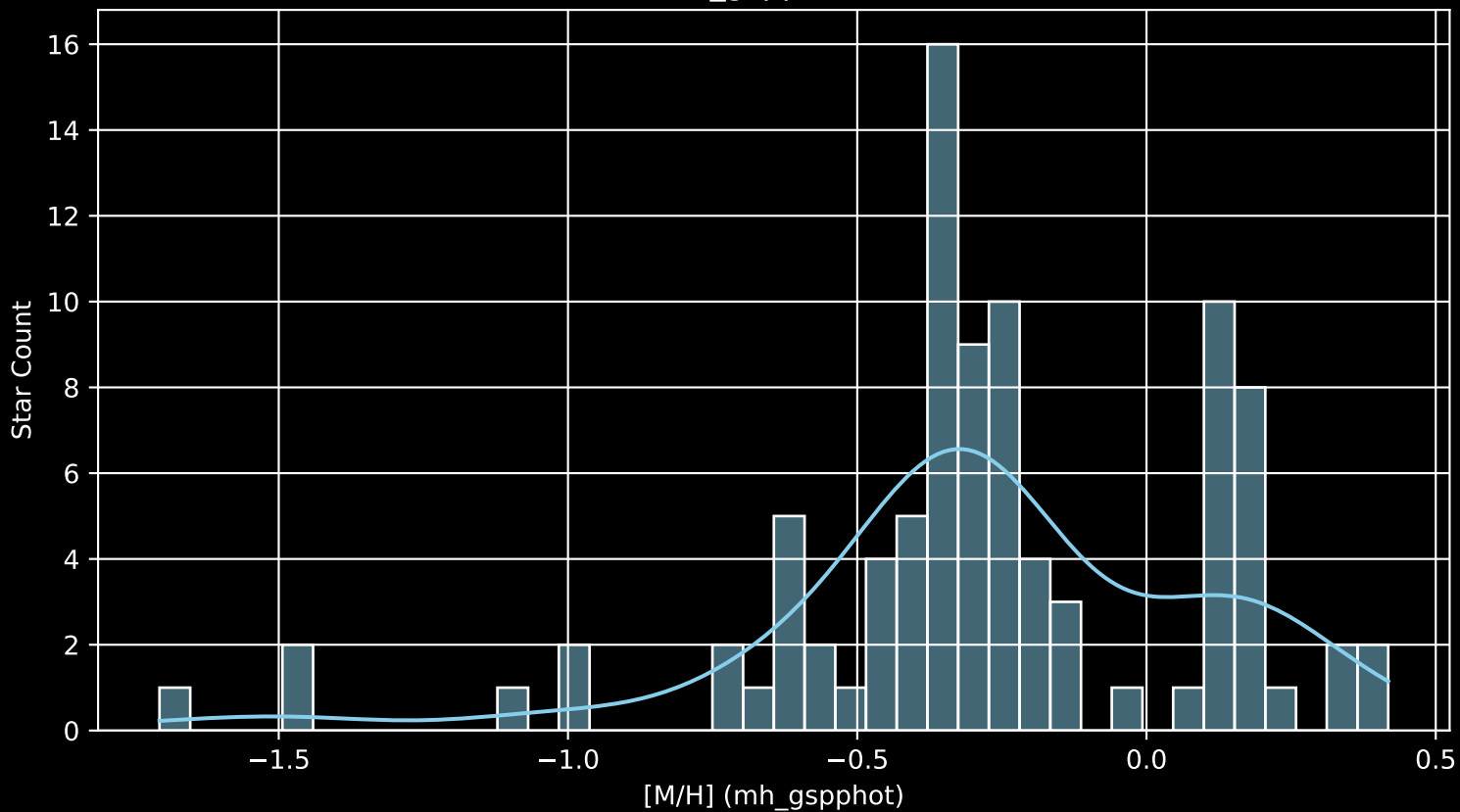
Gaia Cluster: [BH_23 [M/H] (mh_gspphot) (n= 93)
