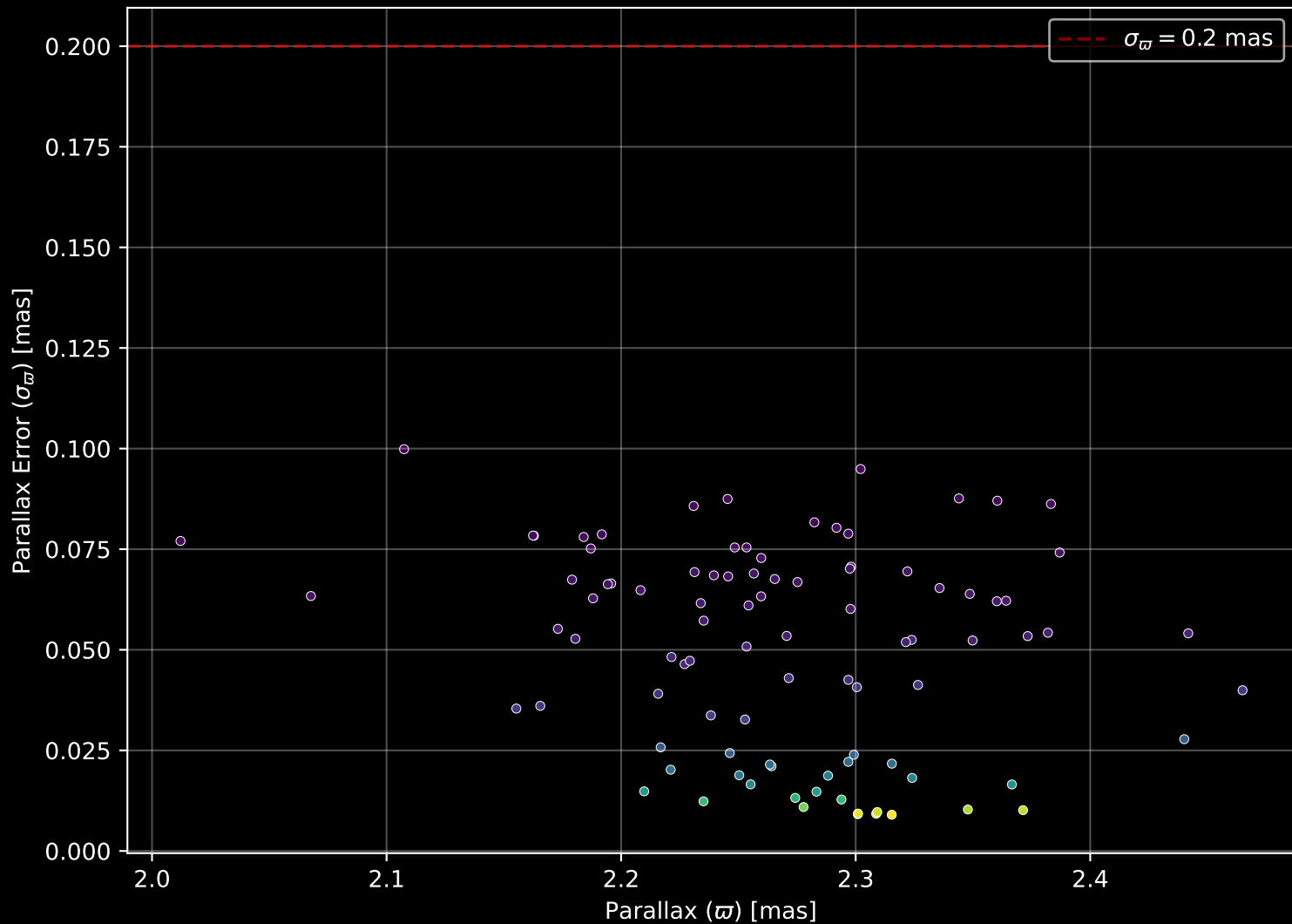
Gaia Cluster: [BH_23] Parallax Quality (n= 94)
