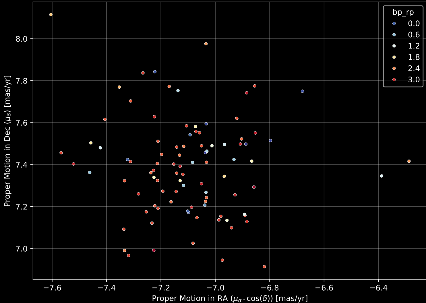
Gaia Cluster: [BH_23] Proper Motion Diagram (n= 94)
