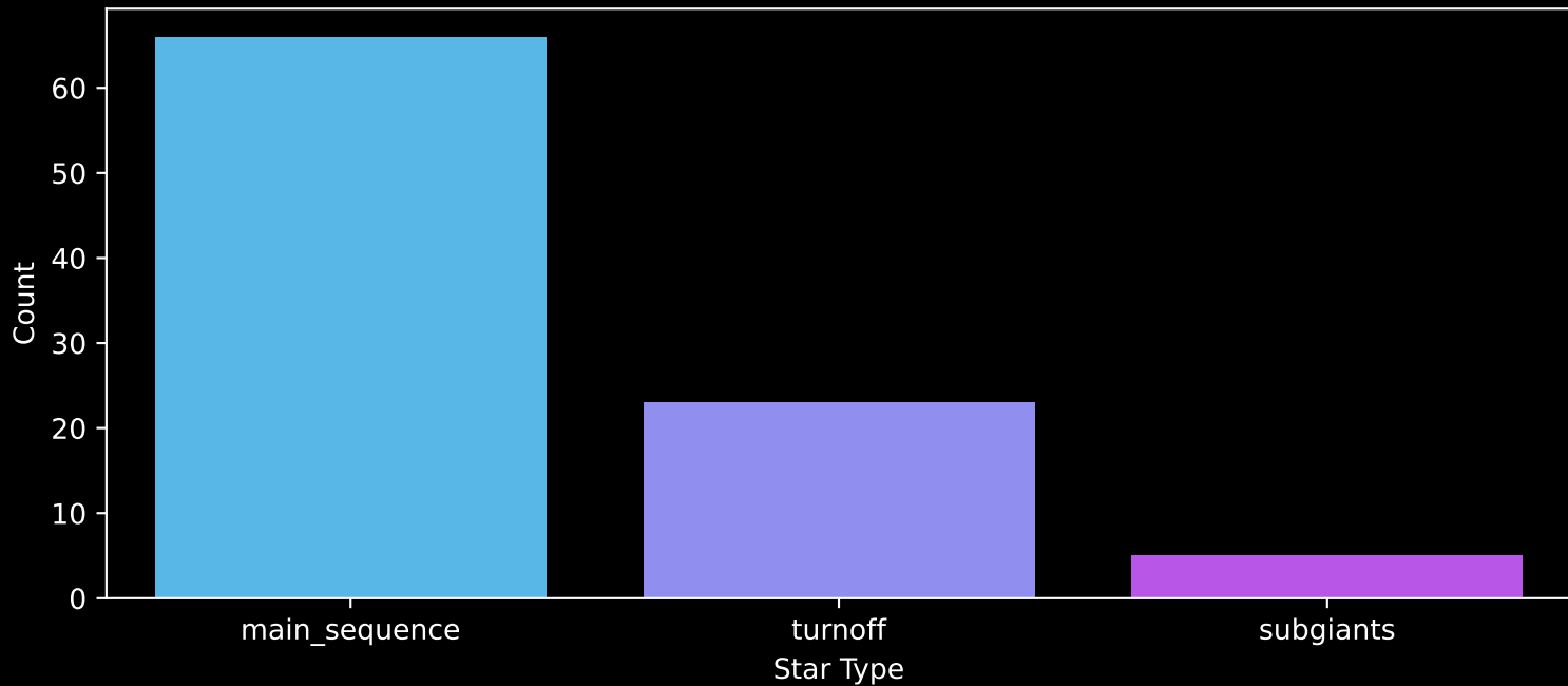
Gaia Cluster: [BH_23] Count plot of Star Type
