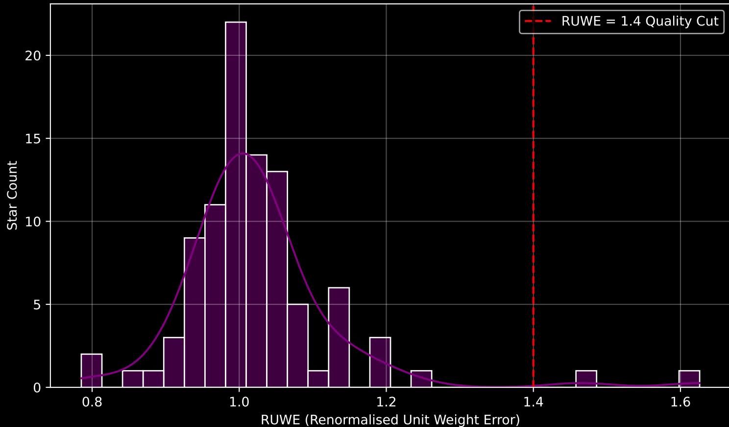
Gaia Cluster: [BH_23] RUWE Distribution (n= 94)
