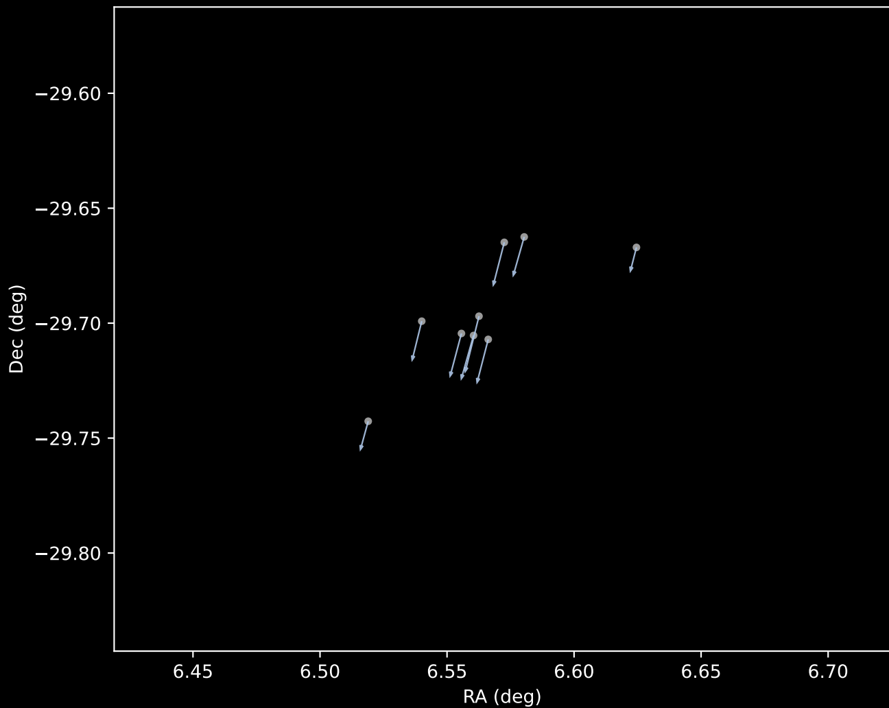
Gaia DR3 Cluster 1 Proper Motion Vectors (n=9)
