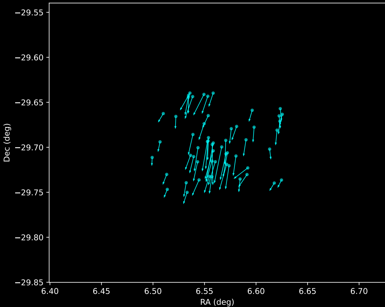
Gaia DR3 Noise Stream Proper Motion Vectors (n=56)
