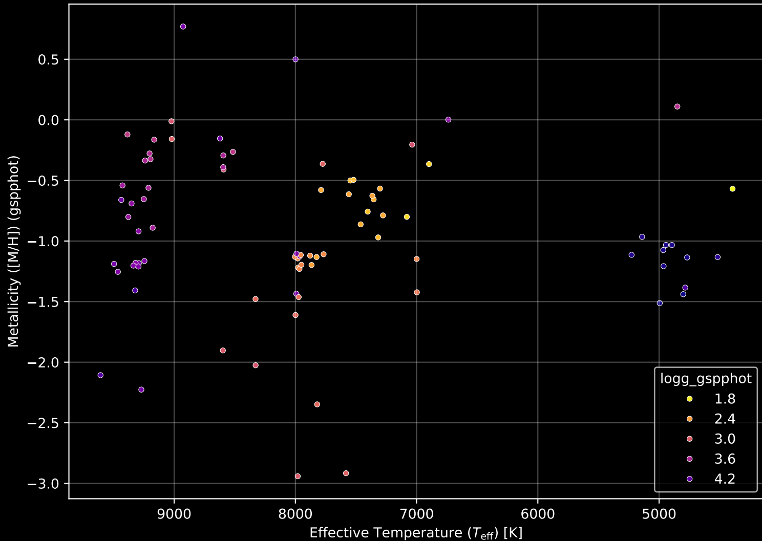
Gaia Cluster: [BH_245] Stellar Population Parameters (n= 84)
