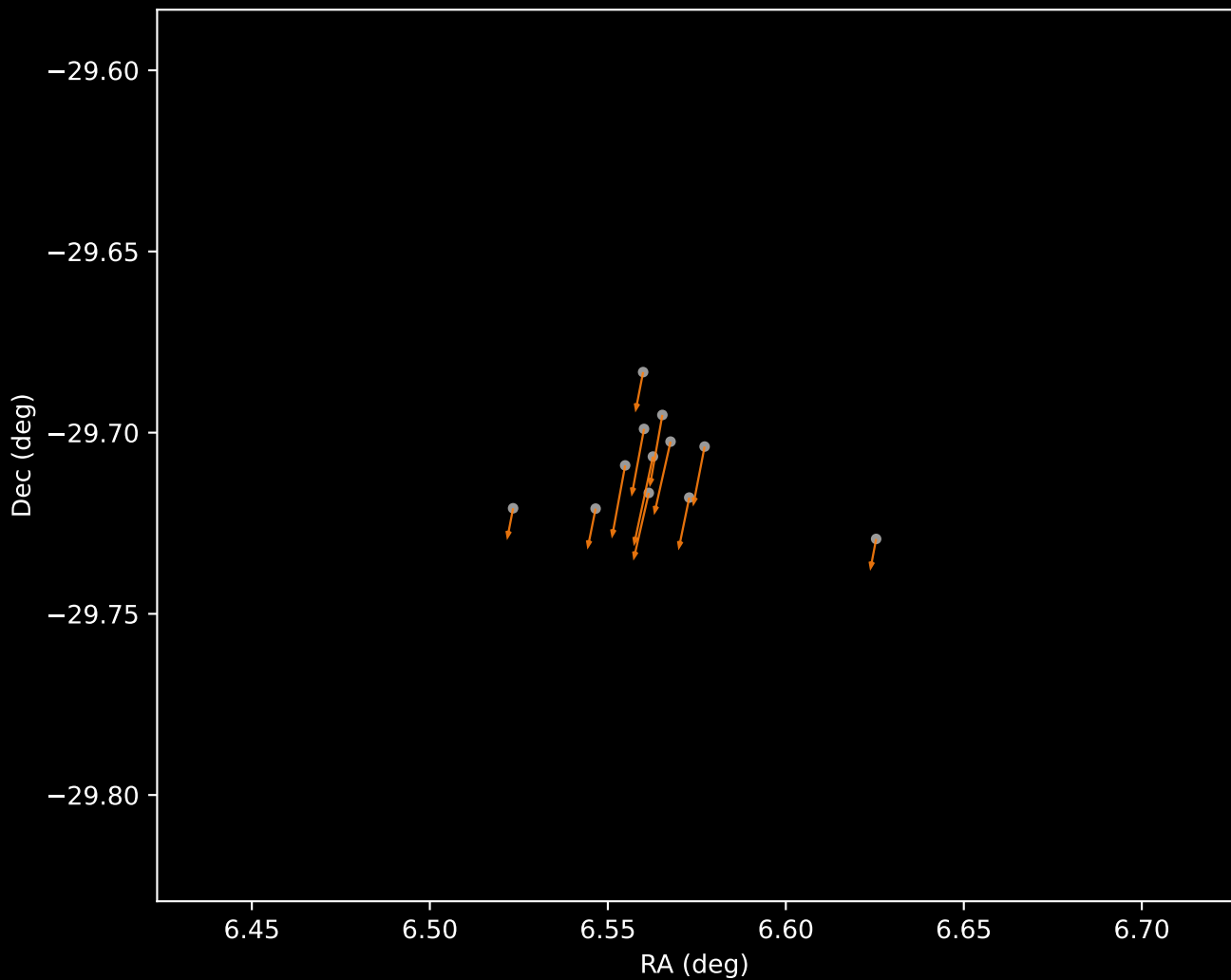
Gaia DR3 Cluster 2 Proper Motion Vectors (n=12)
