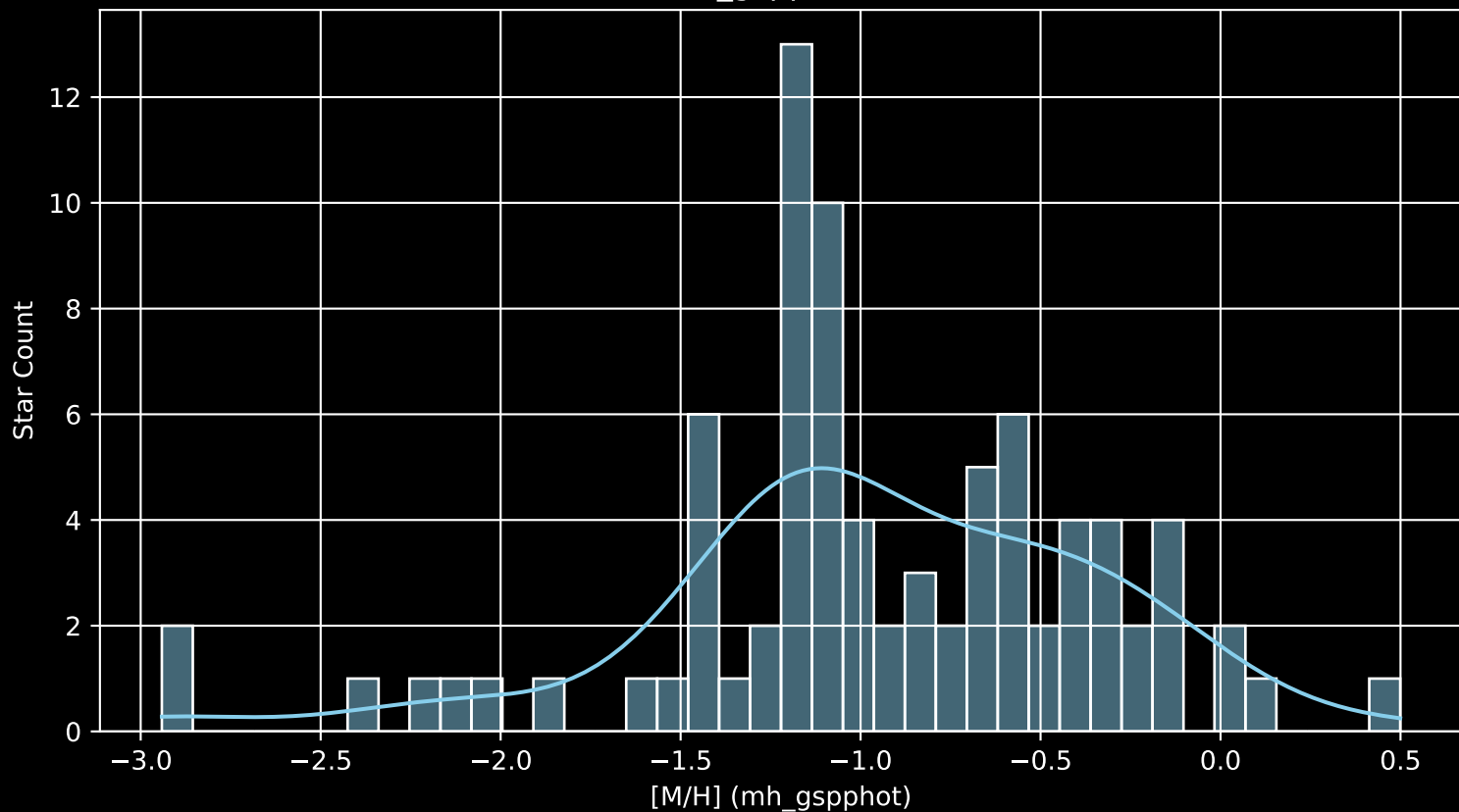
Gaia Cluster: [BH_245 [M/H] (mh_gspphot) (n= 83)
