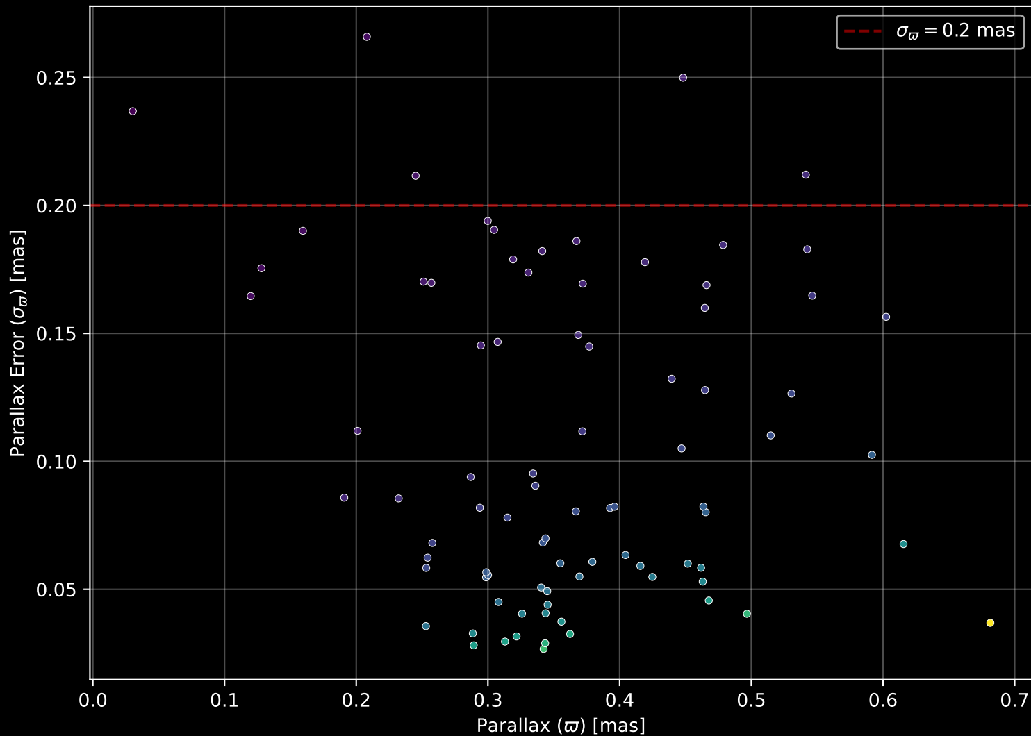
Gaia Cluster: [BH_245] Parallax Quality (n= 84)
