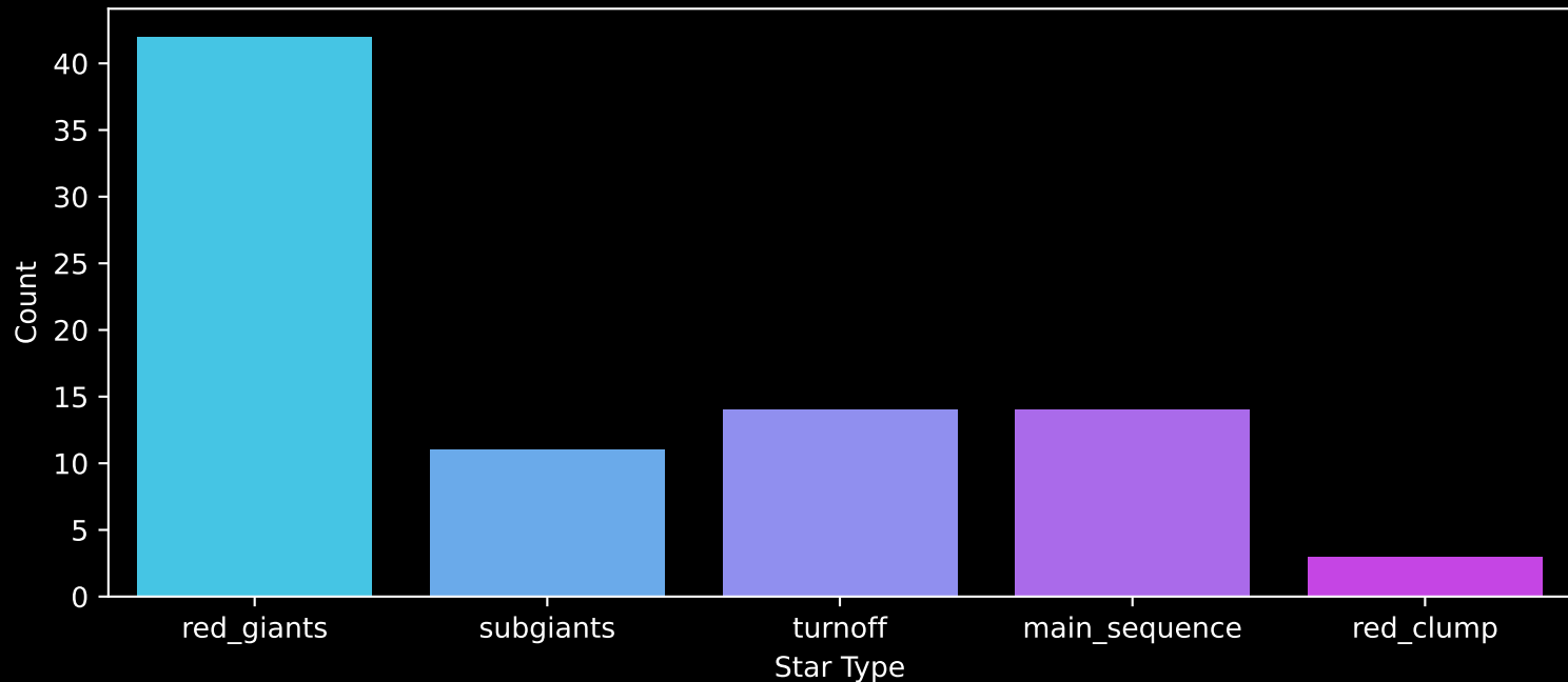
Gaia Cluster: [BH_245] Count plot of Star Type
