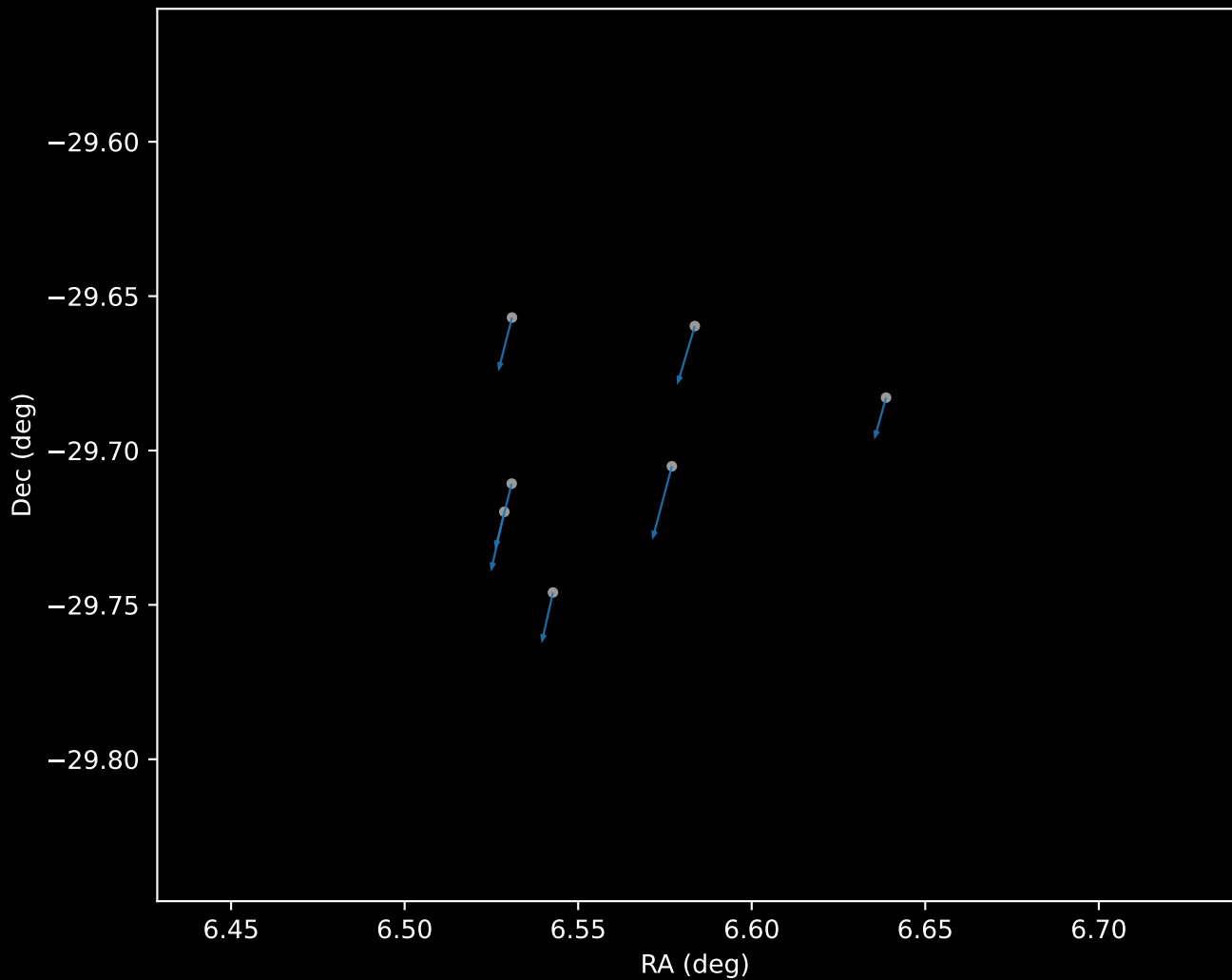
Gaia DR3 Cluster 0 Proper Motion Vectors (n=7)
