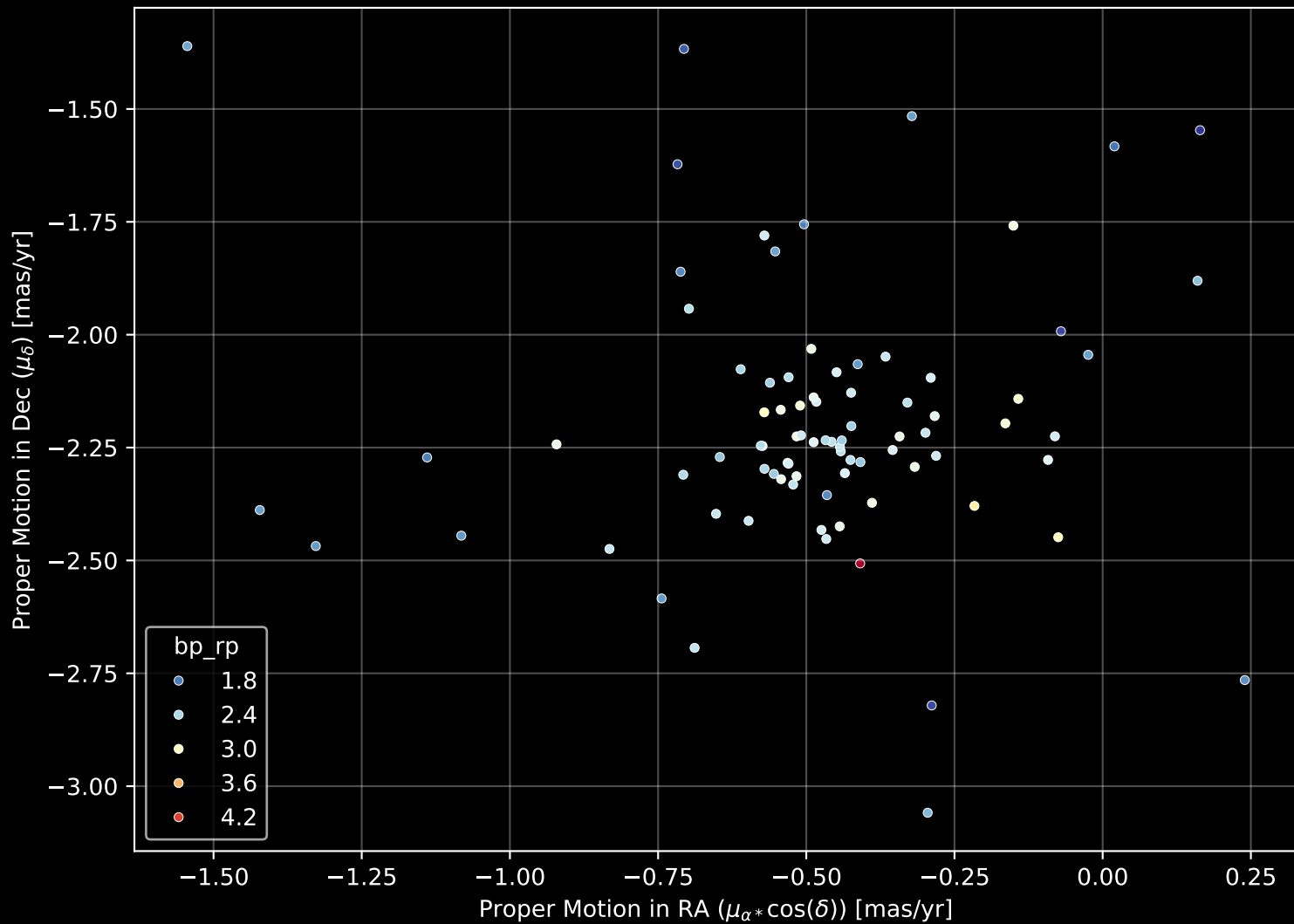
Gaia Cluster: [BH_245] Proper Motion Diagram (n= 84)
