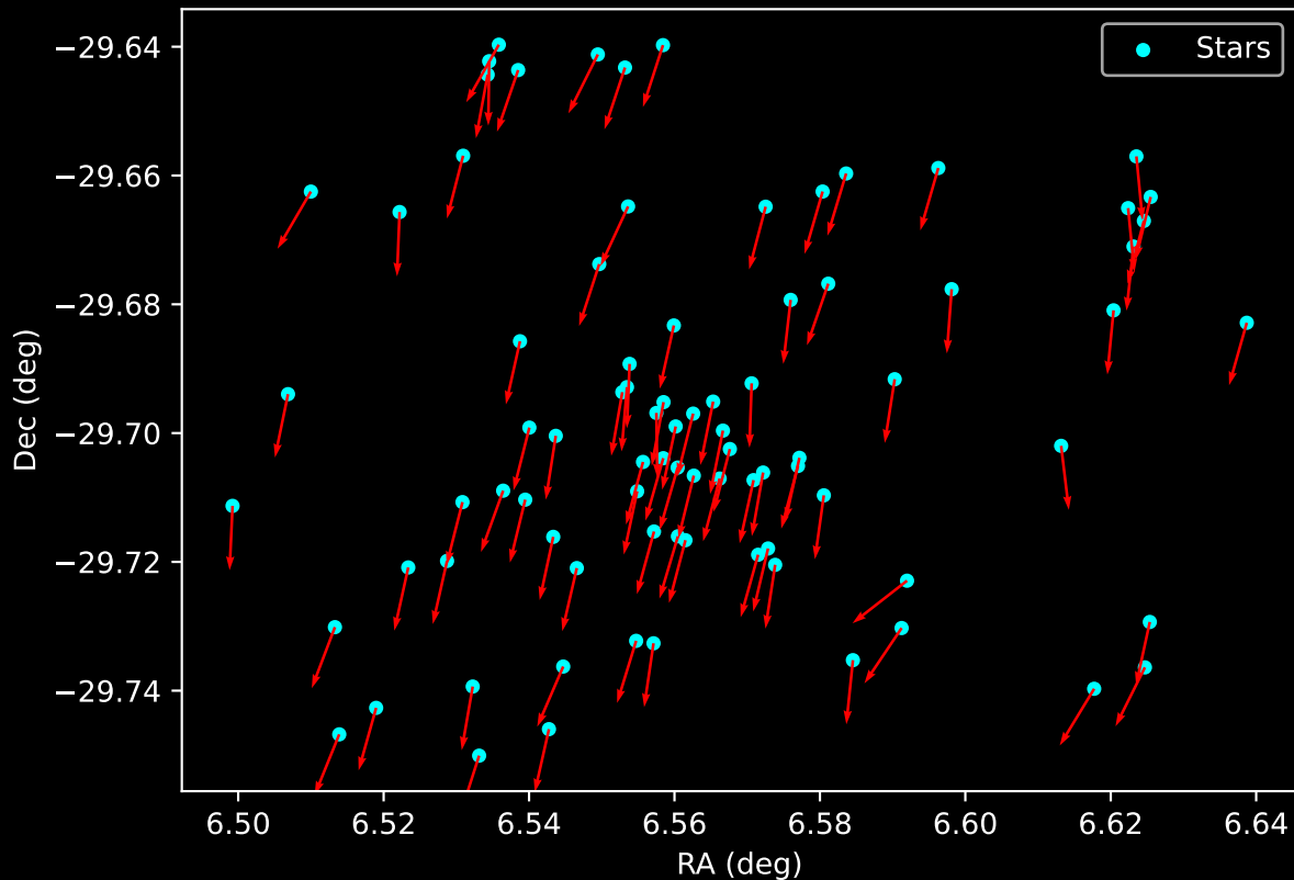
Gaia Cluster: [BH_245] Proper Motion Vectors for Gaia Star Field (n= 84)
