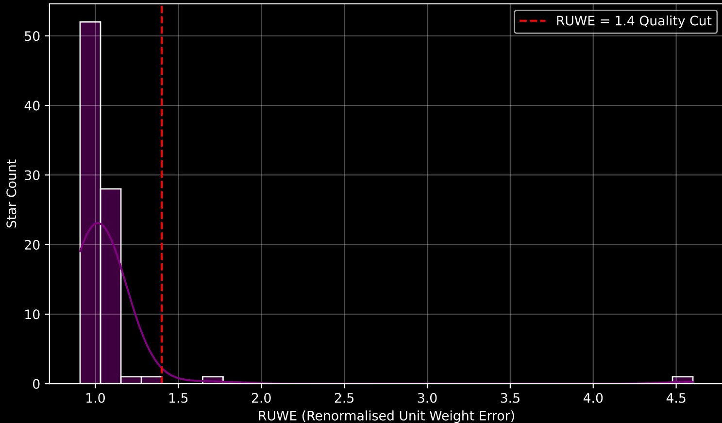
Gaia Cluster: [BH_245] RUWE Distribution (n= 84)
