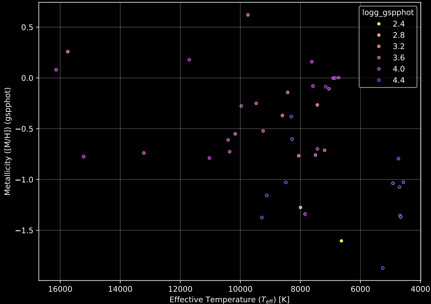
Gaia Cluster: [BH_54] Stellar Population Parameters (n= 42)
