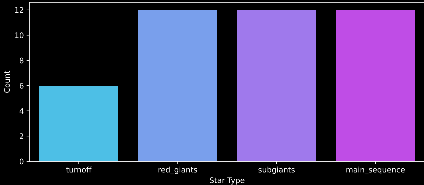
Gaia Cluster: [BH_54] Count plot of Star Type
