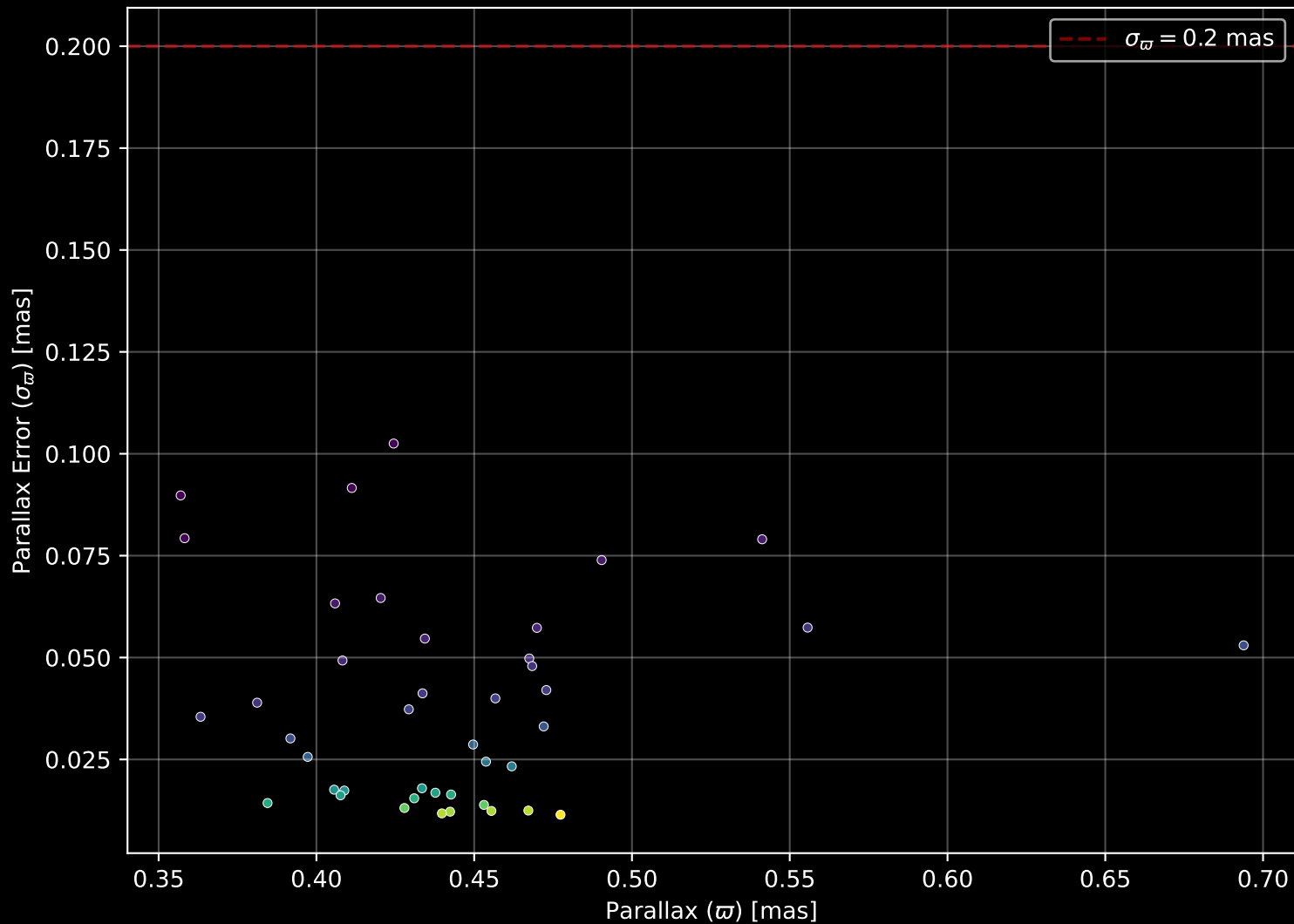
Gaia Cluster: [BH_54] Parallax Quality (n= 42)
