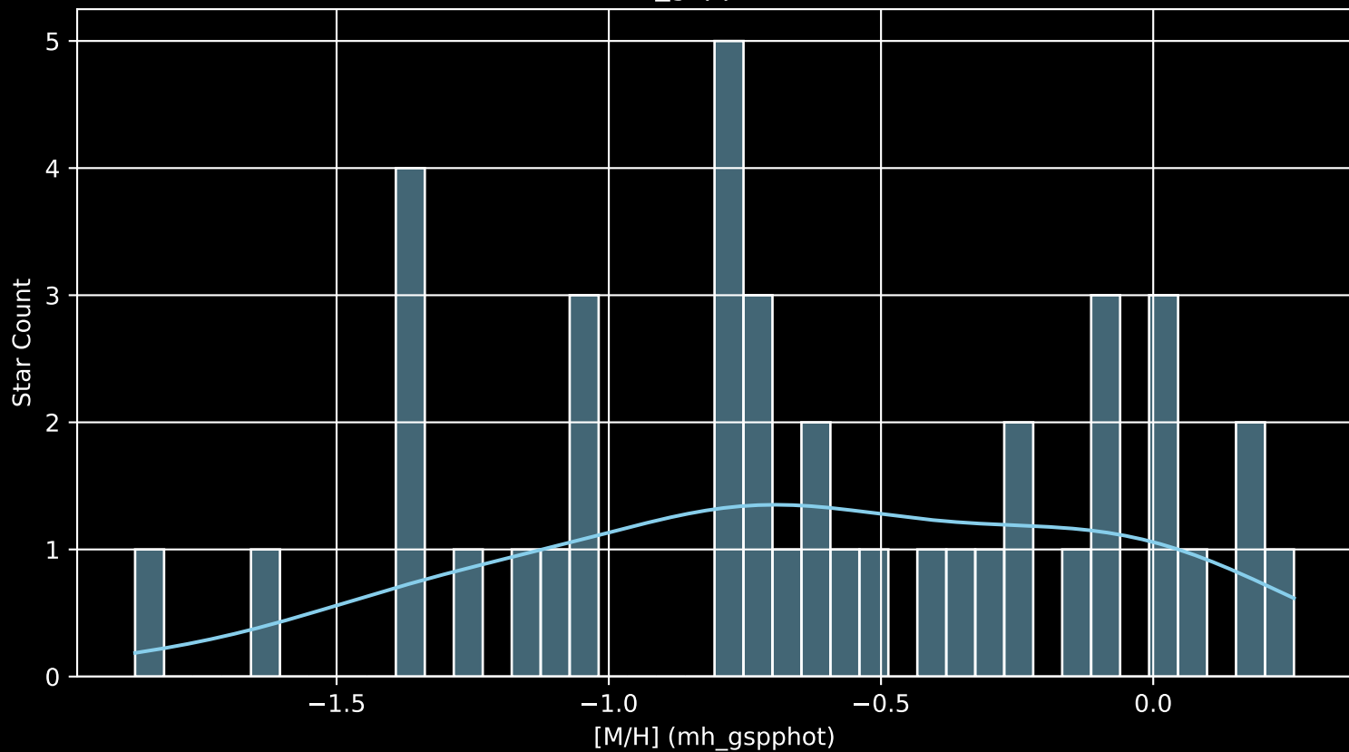
Gaia Cluster: [BH_54 [M/H] (mh_gspphot) (n= 41)
