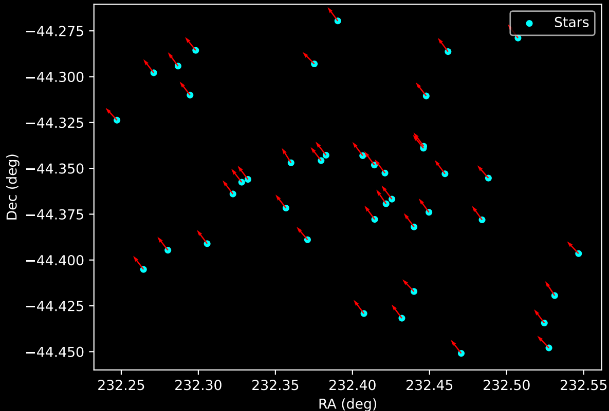
Gaia Cluster: [BH_54] Proper Motion Vectors for Gaia Star Field (n= 42)
