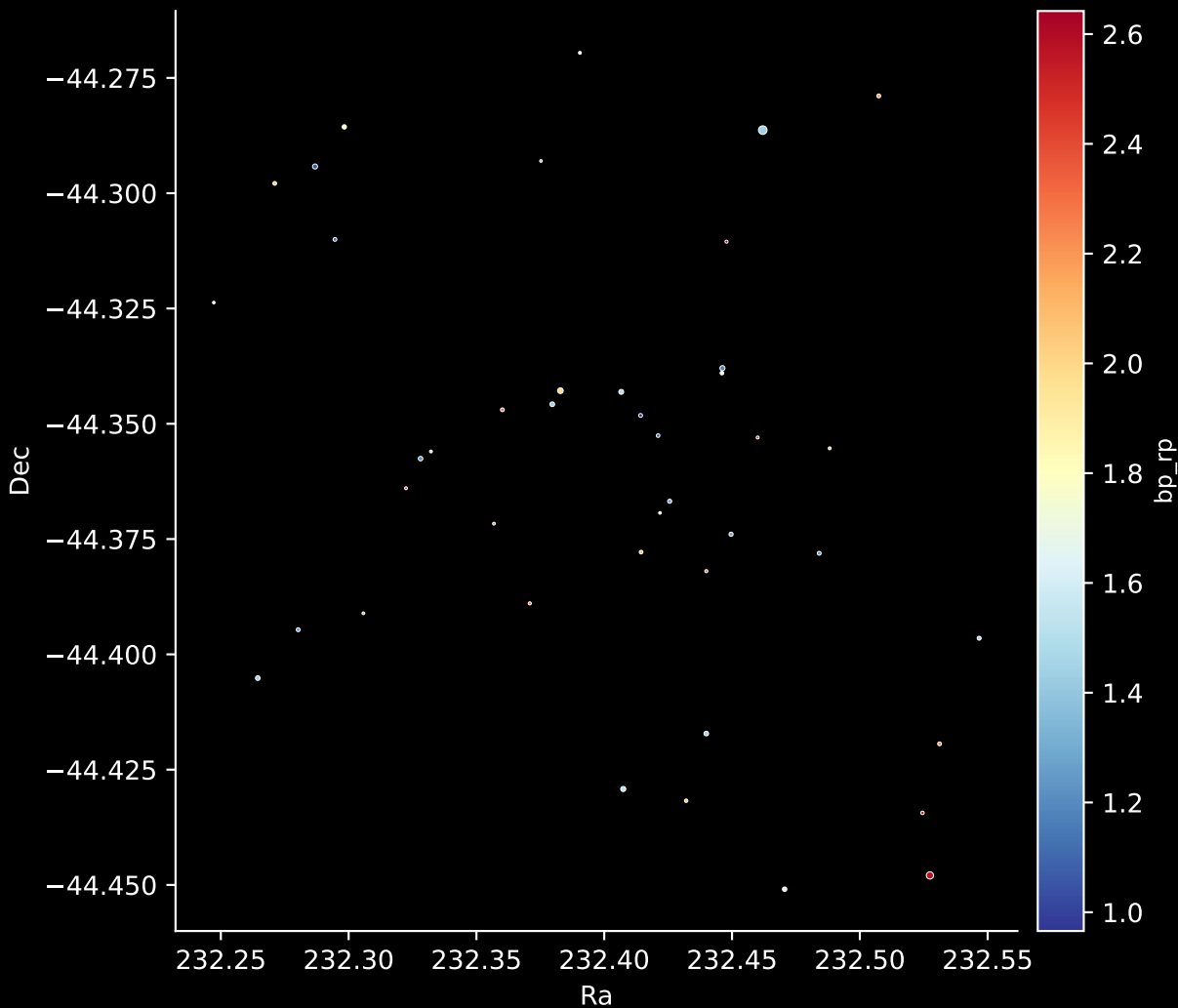
Gaia Cluster: [BH_54] Stars: 42
