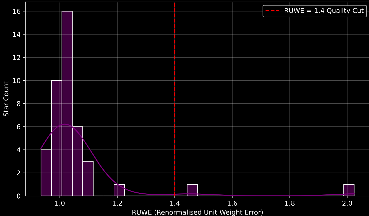
Gaia Cluster: [BH_54] RUWE Distribution (n= 42)
