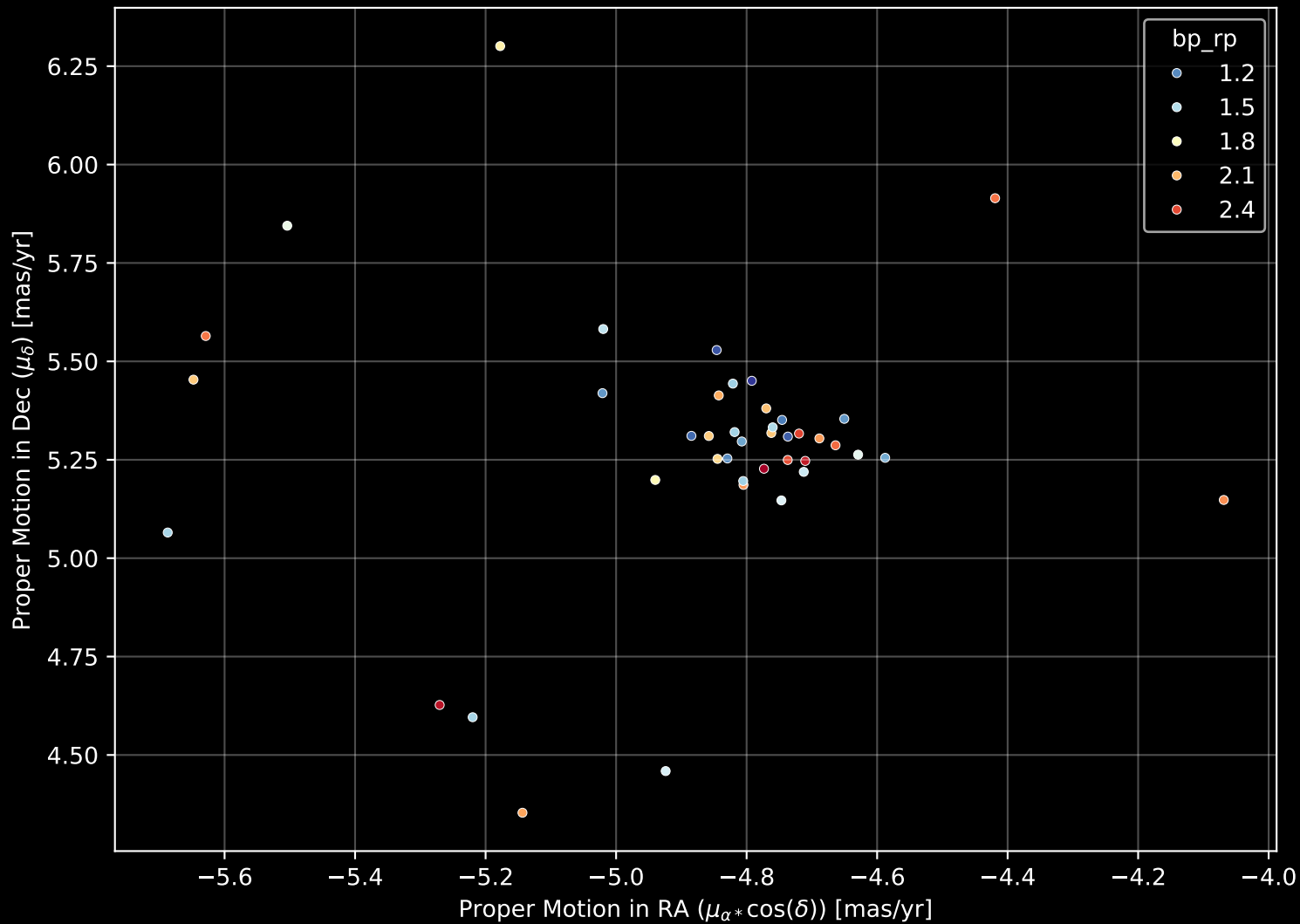
Gaia Cluster: [BH_54] Proper Motion Diagram (n= 42)
