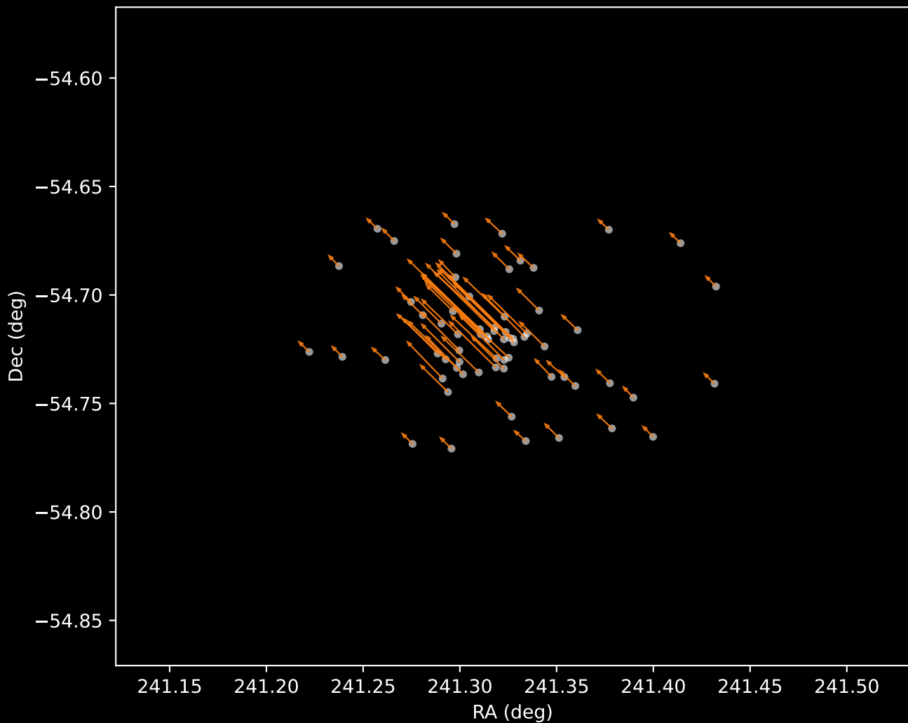
Gaia DR3 Cluster 2 Proper Motion Vectors (n=66)
