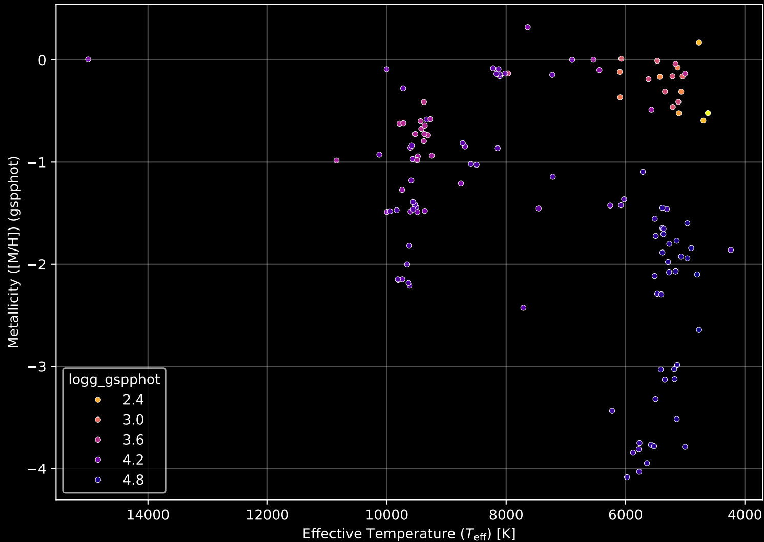
Gaia Cluster: [BH_66] Stellar Population Parameters (n= 128)
