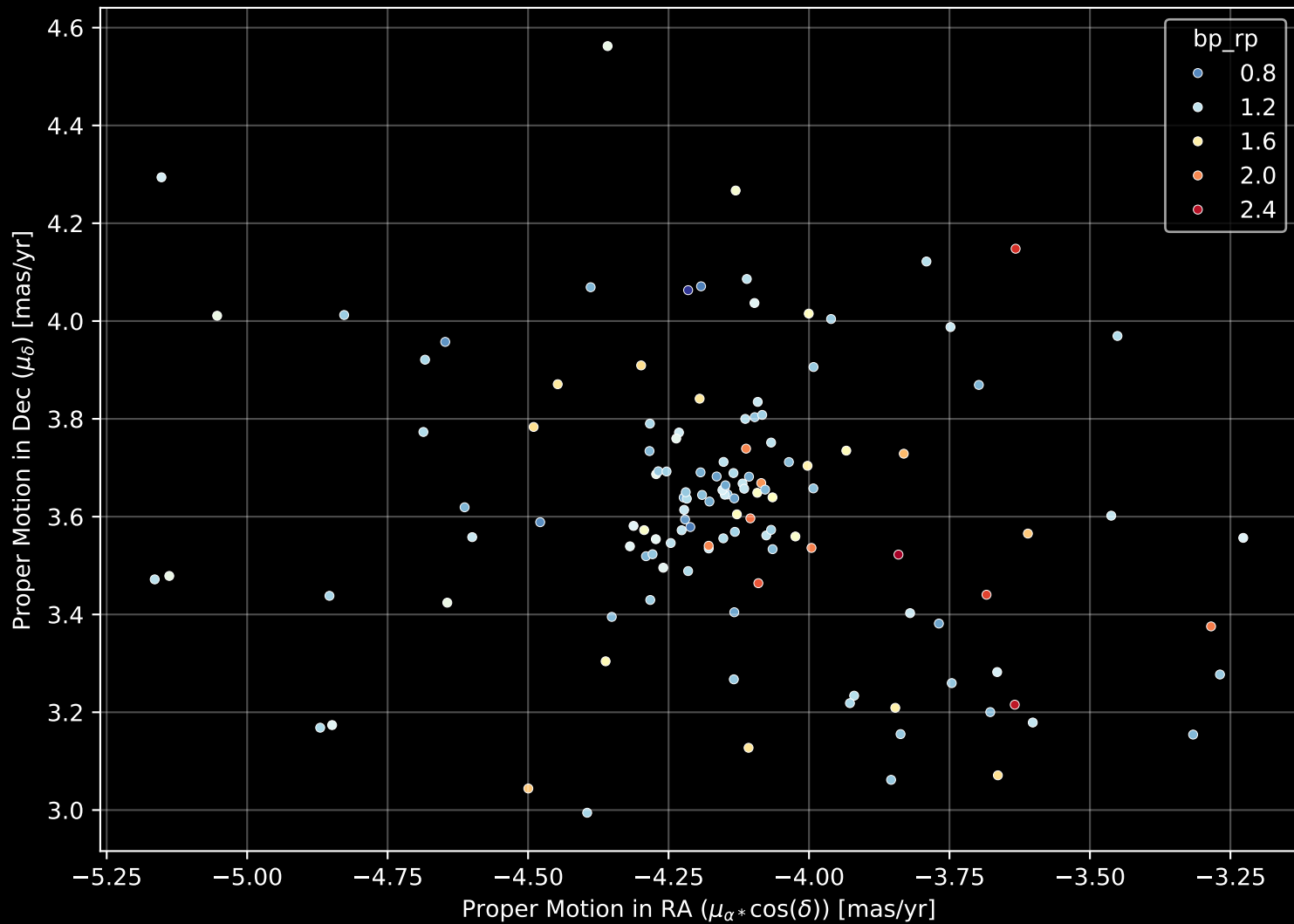
Gaia Cluster: [BH_66] Proper Motion Diagram (n= 128)
