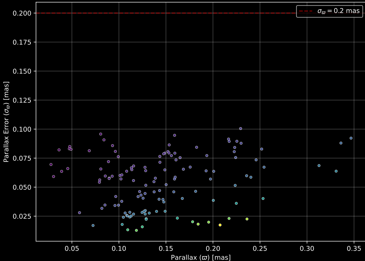
Gaia Cluster: [BH_66] Parallax Quality (n= 128)
