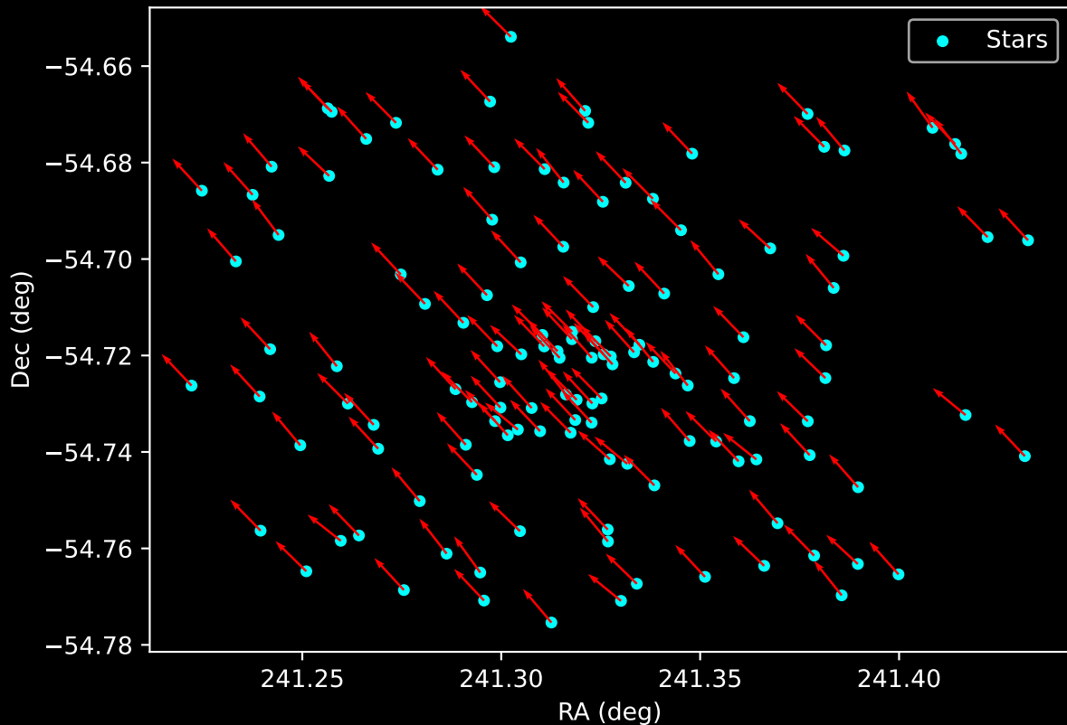
Gaia Cluster: [BH_66] Proper Motion Vectors for Gaia Star Field (n= 128)
