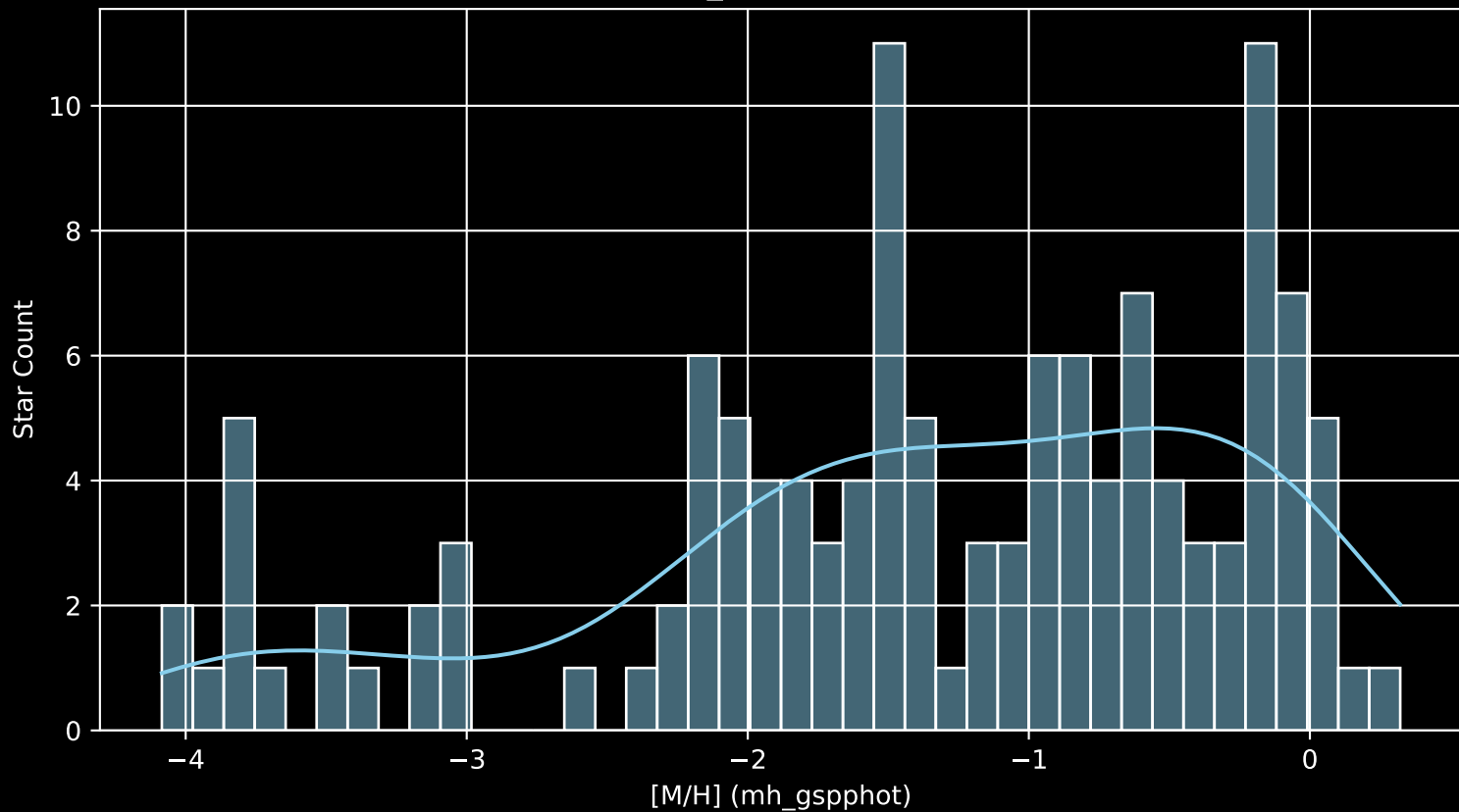
Gaia Cluster: [BH_66 [M/H] (mh_gspphot) (n= 128)
