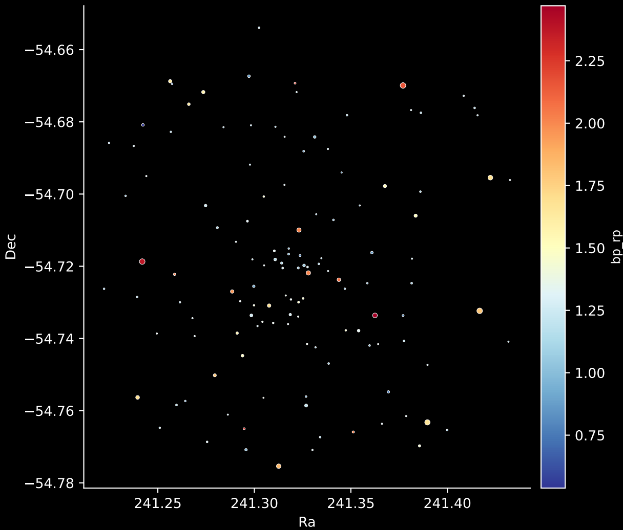
Gaia Cluster: [BH_66] Stars: 128
