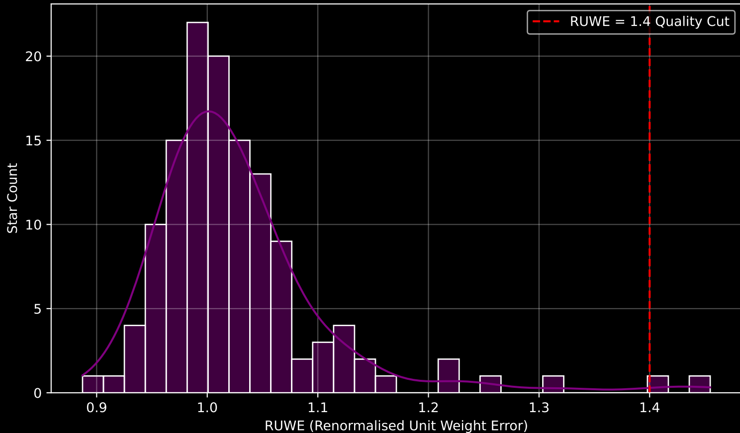
Gaia Cluster: [BH_66] RUWE Distribution (n= 128)
