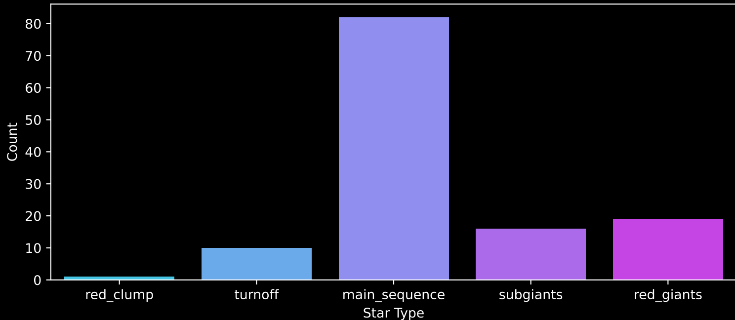
Gaia Cluster: [BH_66] Count plot of Star Type
